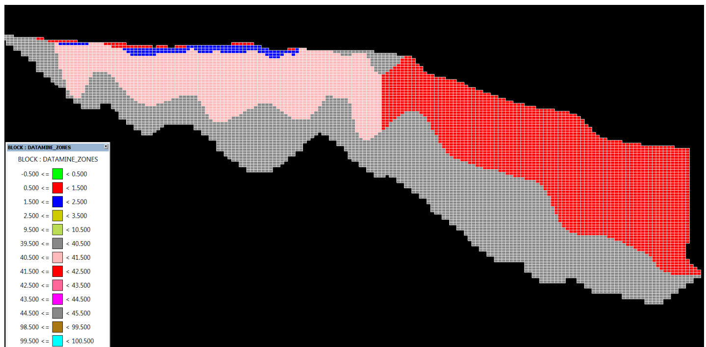
Figure 14-10: Pebble Deposit Copper Grade Domains
