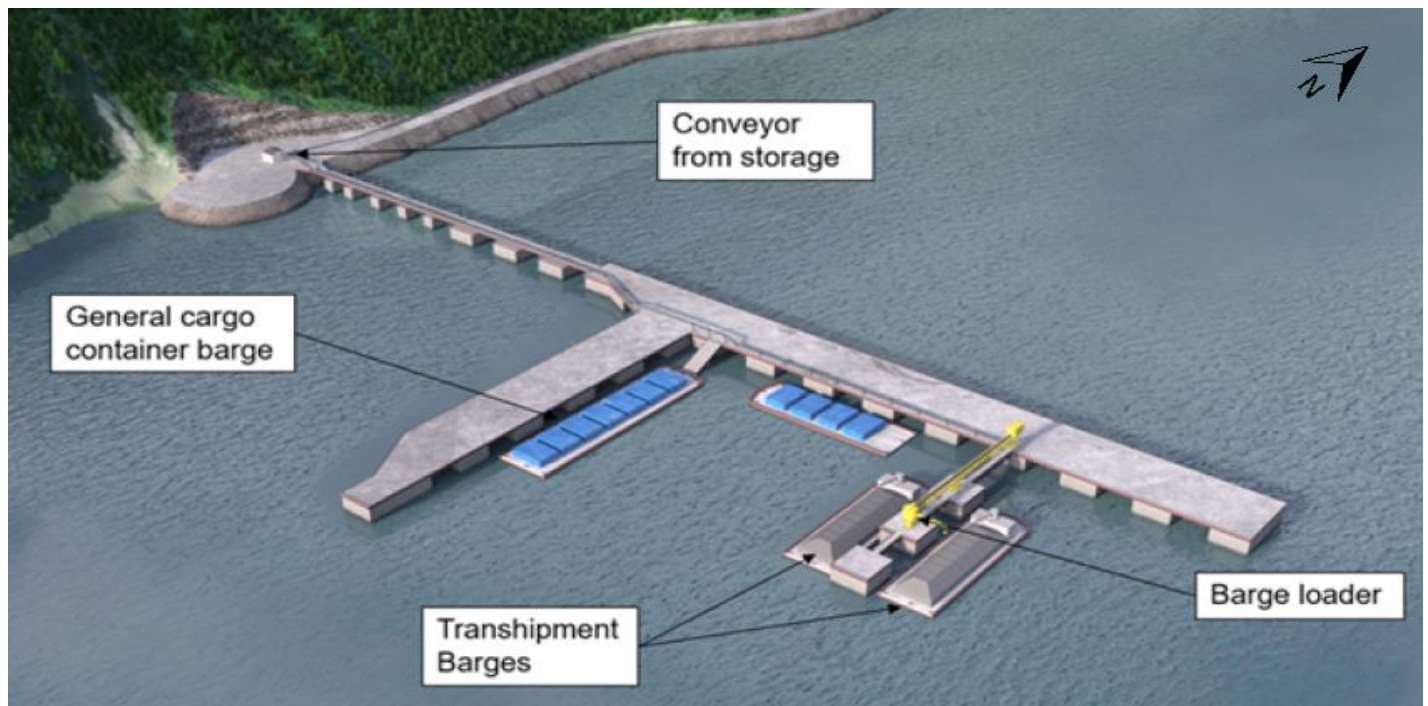
Figure 18-7: Schematic Rendering of the Marine Facilities
