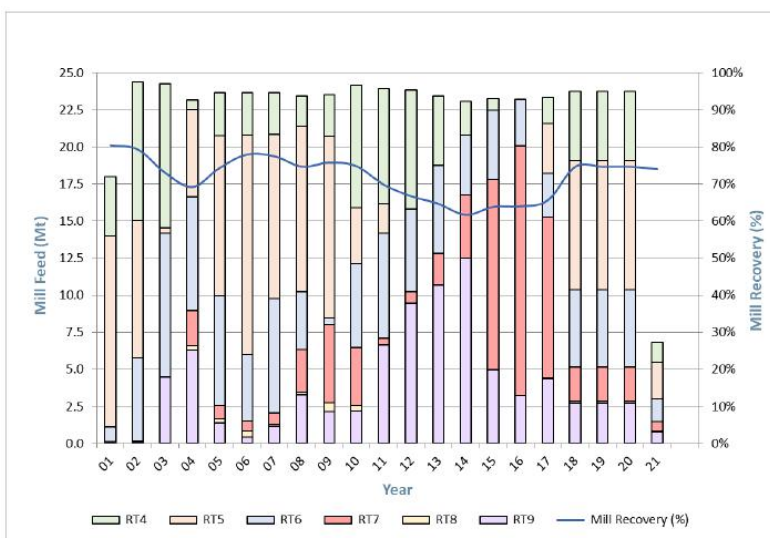
Figure 13-9: Mill feed
