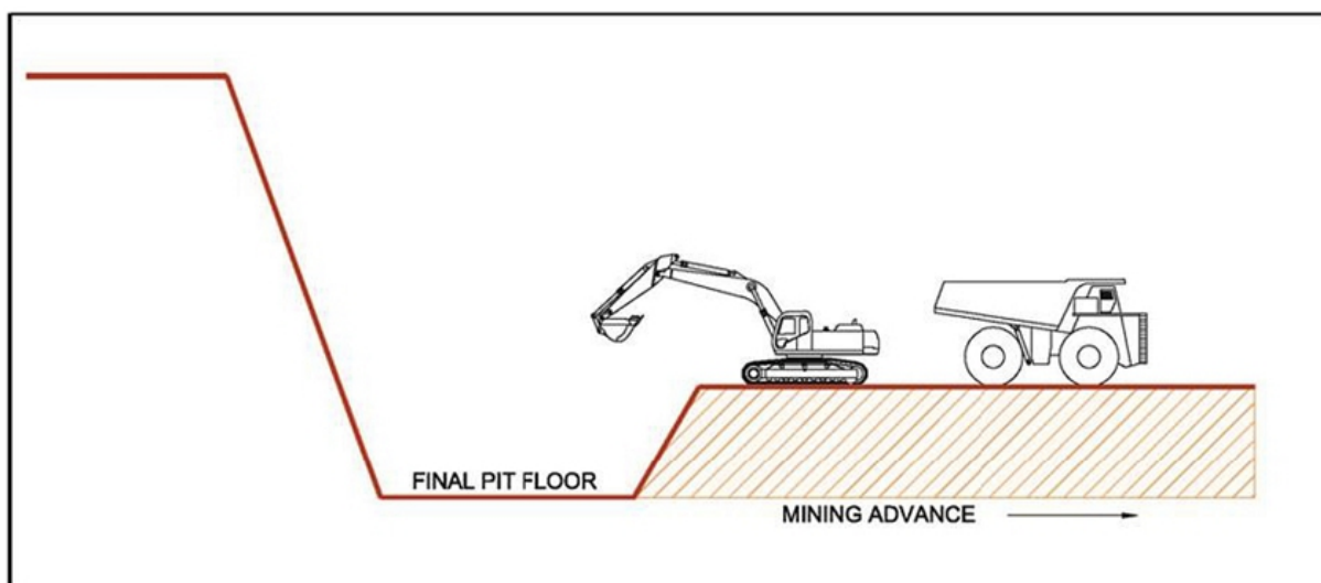
Figure 12-6: Final bench access
