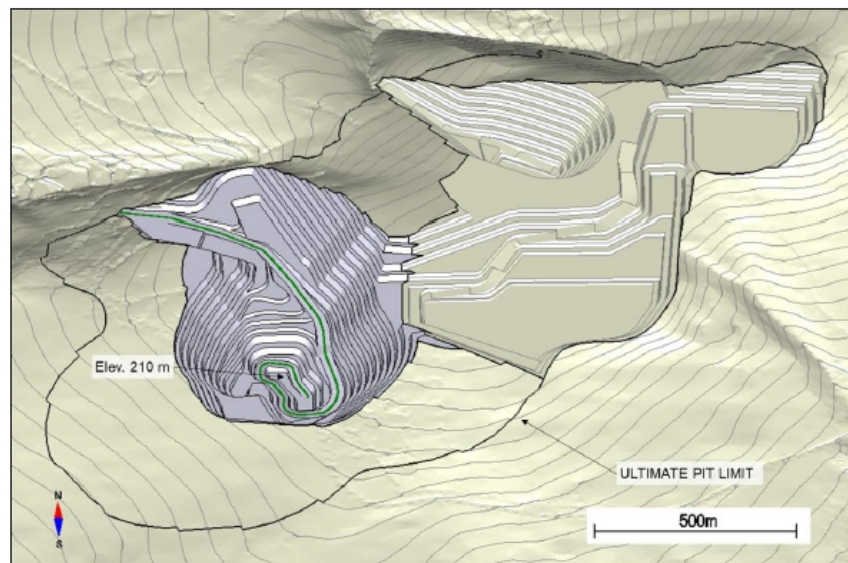
Figure 13-4: Phase 3 design
