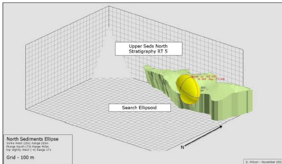
Figure 11-9: Upper Sediments North search ellipse
