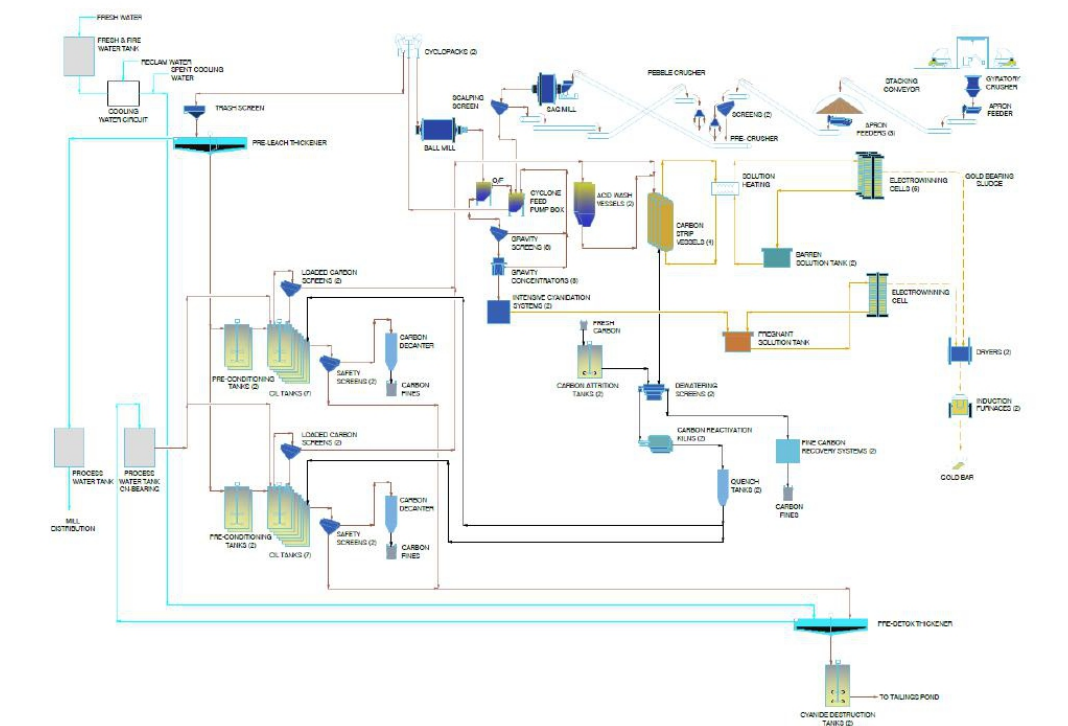
Figure 14-2: Conceptual process flowsheet
