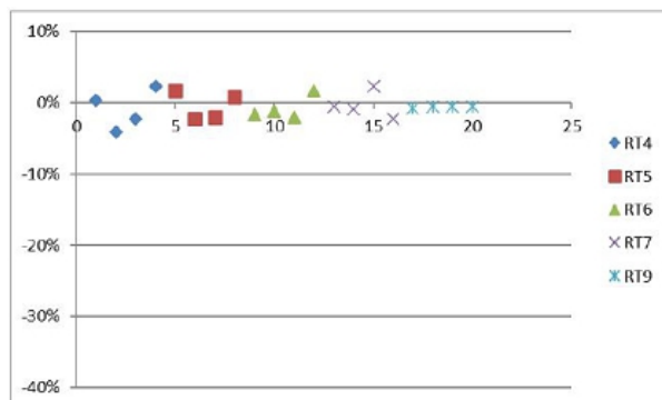
Figure 10-29: % Au gain preg-robbing level (2021 PFS – Phase 9a)
