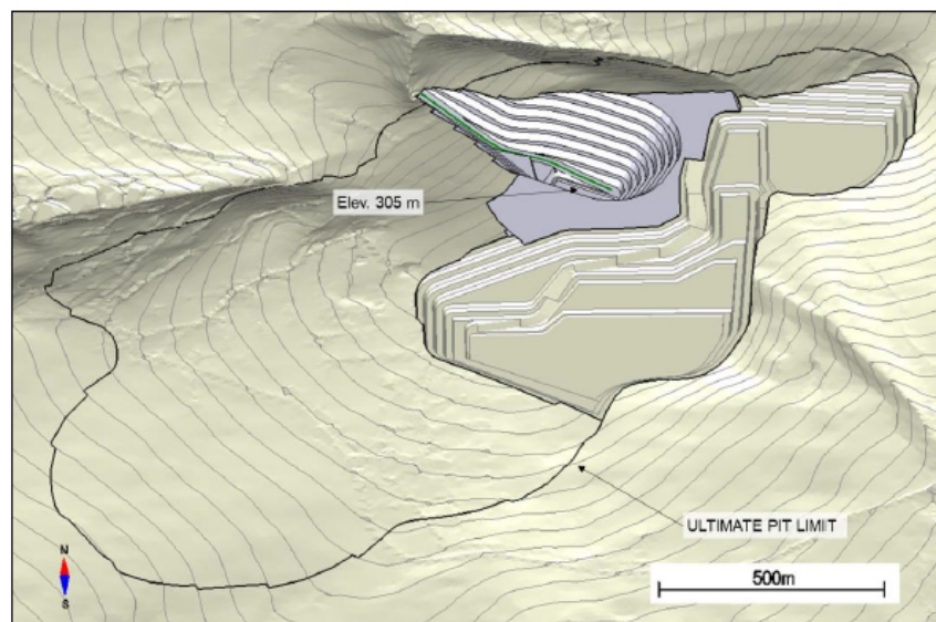
Figure 13-3: Phase 2 design
