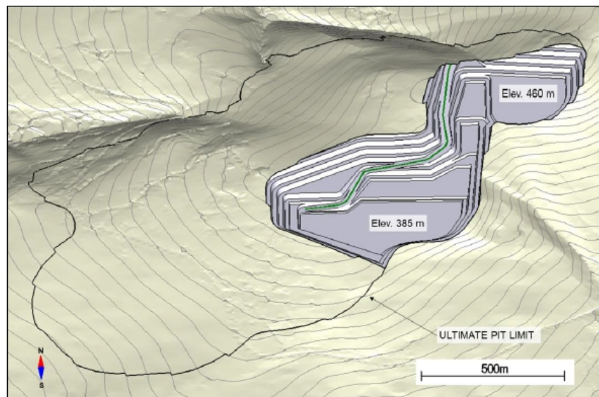
Figure 13-2: Phase 1 design
