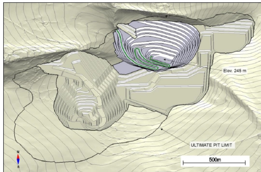
Figure 13-5: Phase 4 design
