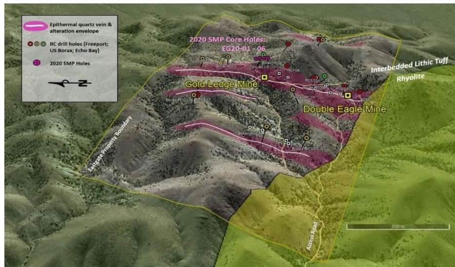
Eastgate Gold Project: Property Geology (Oblique View to East)
