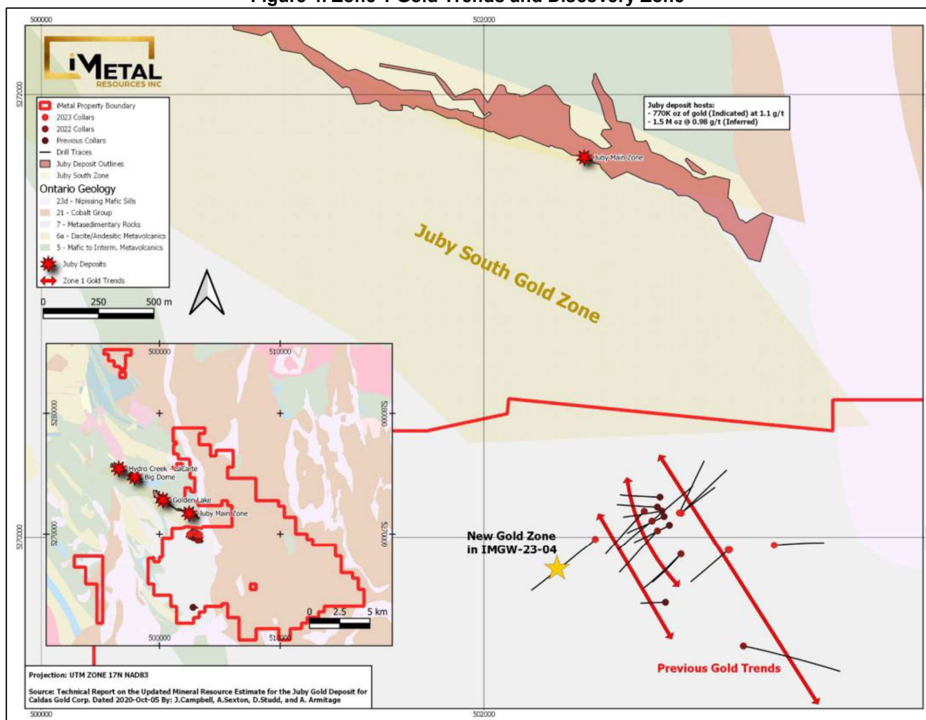
Figure 4. Zone 1 Gold Trends and Discovery Zone
