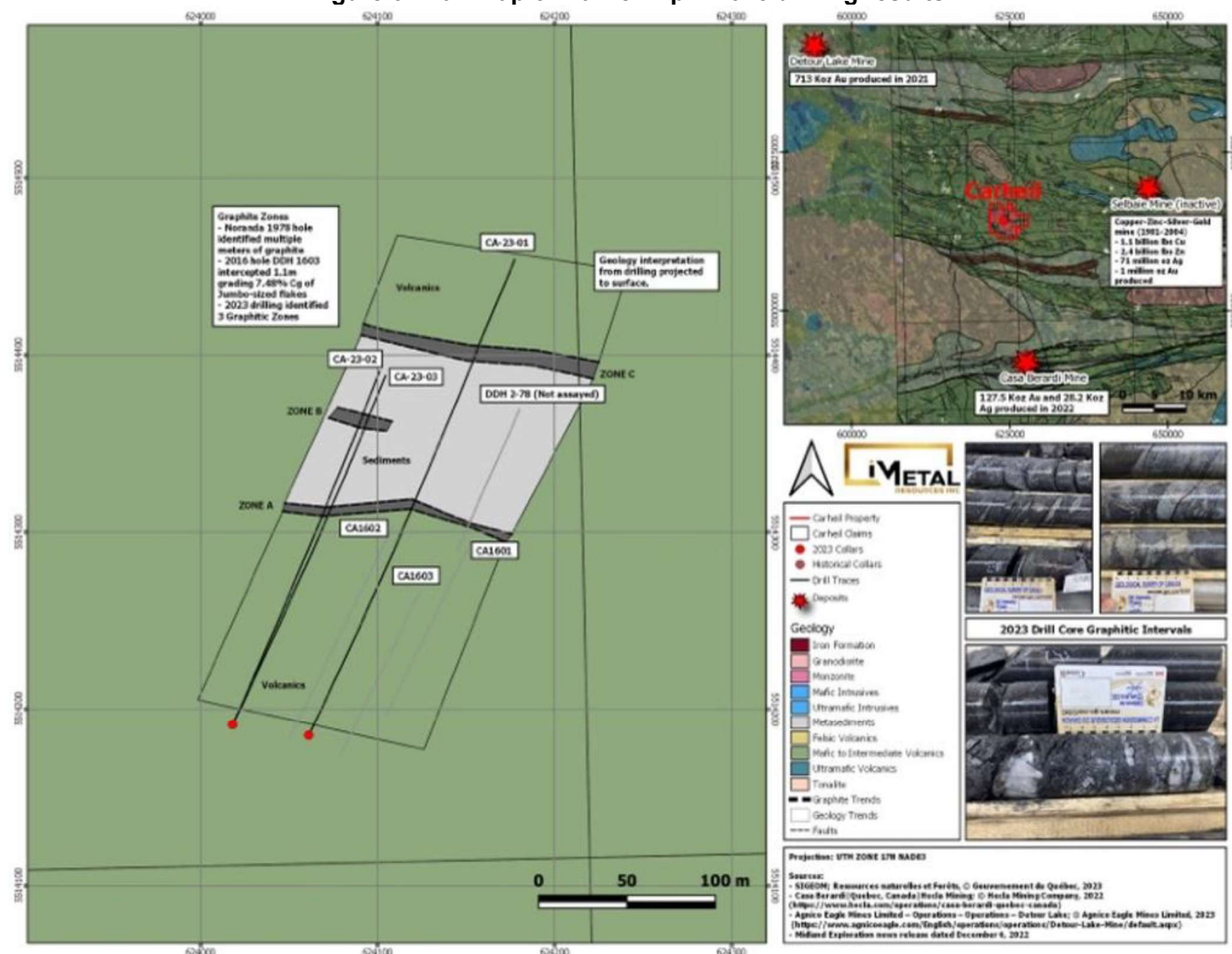
Figure 6. Plan Map of Carheil April 2023 drilling results
