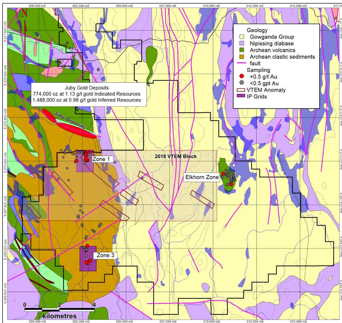
Figure 2. Geology and Current Exploration Focus
