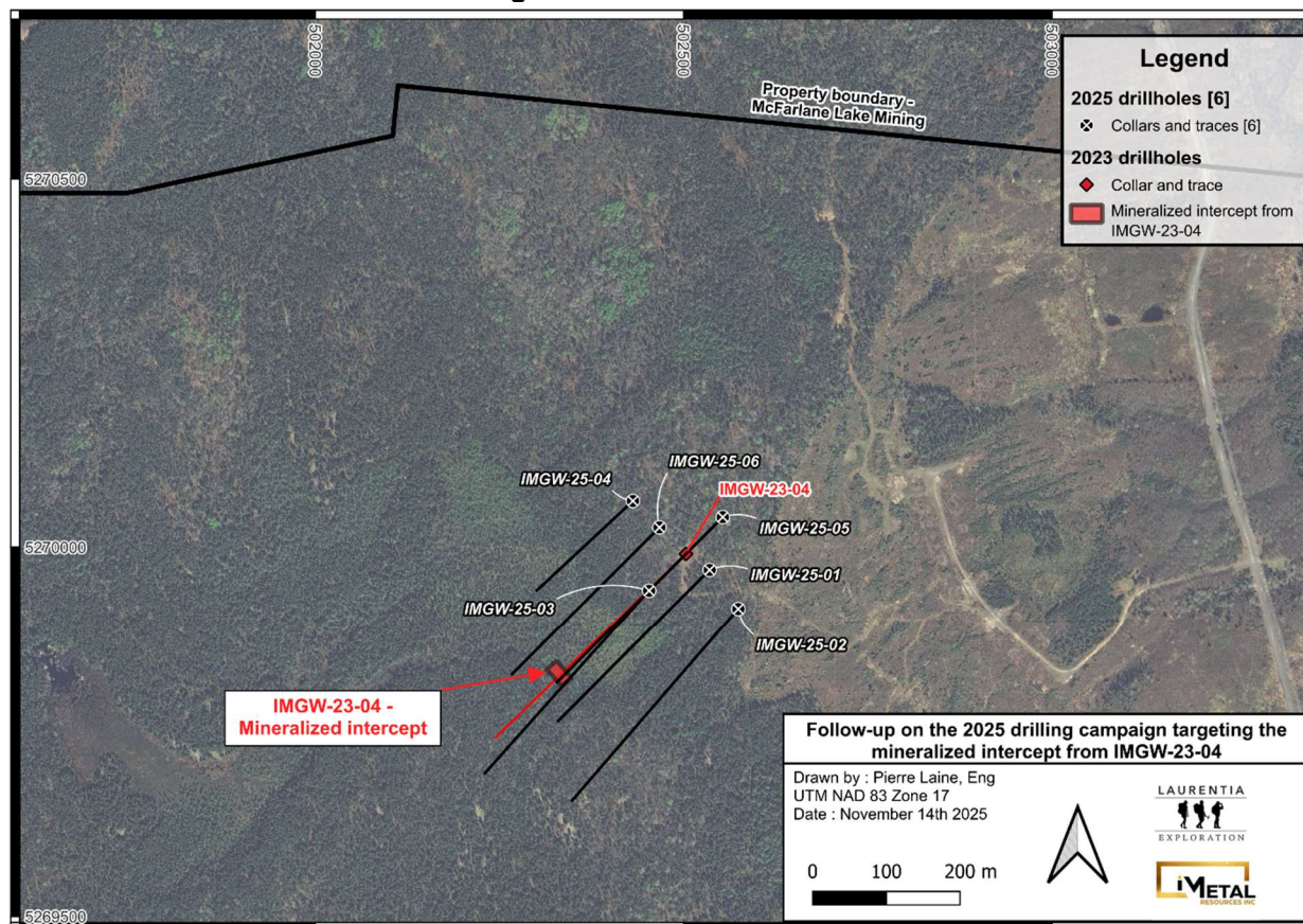
Figure 6. 2026 Drill Hole Locations
