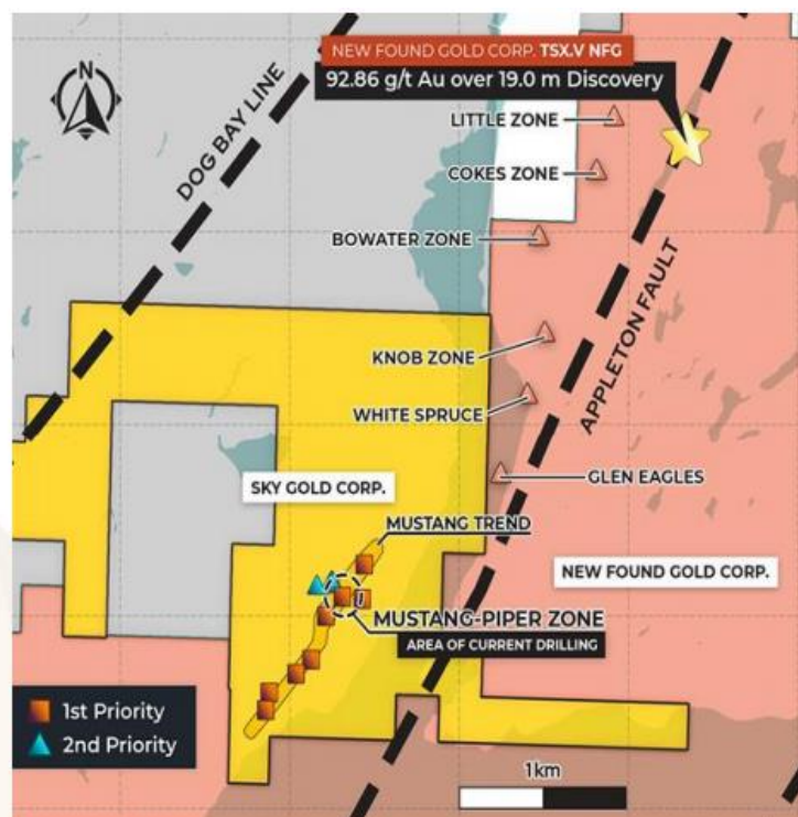
Figure 2: Location of drill holes completed on the Mustang Property in 2020-2021.
