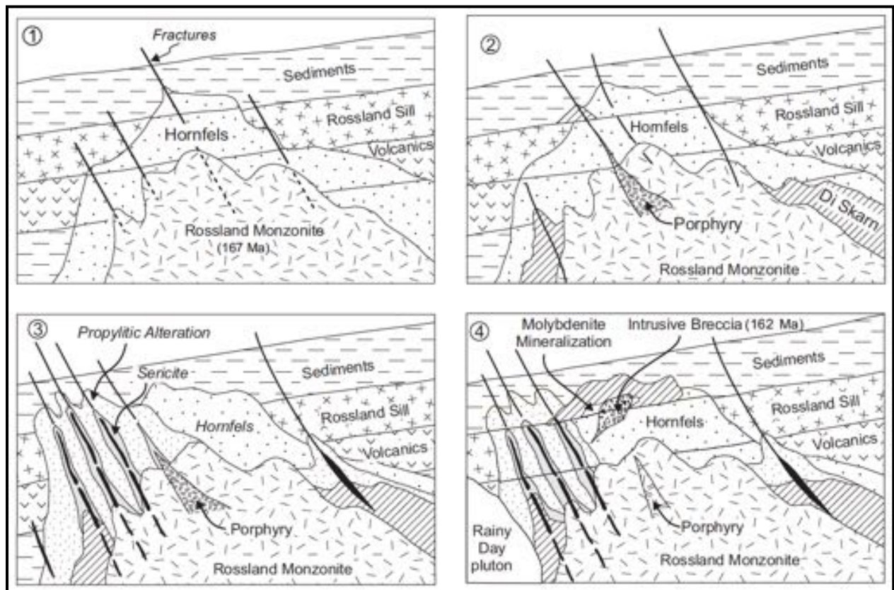
Figure 39: Model showing proposed evolution of gold-copper, and polymetallic veins, and molybdenite breccia/skarn deposits of the Rossland district, related to the intrusion of the Rossland monzonite and diorite porphyry at circa 167 Ma (frames 2 & 3) and molybdenite to intrusion of the circa Rainy Day pluton and associated dikes at 162-163 Ma (frame 4) (from Hoy & Dunne, 2001)
