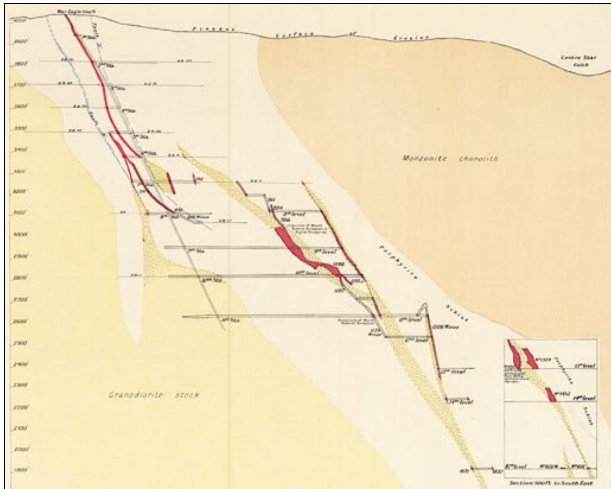
Figure 33: Cross-section through the War Eagle mine (from Geological Survey of Canada, circa 1915)
