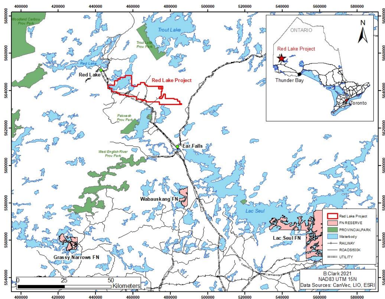
Figure 1: Regional Location Map of Dixie Gold's Project
