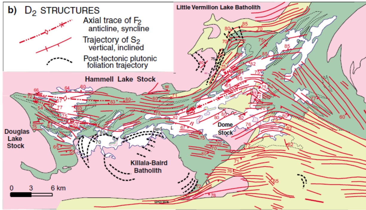
Figure 4: D2 Structures in the Red Lake Greenstone Belt
