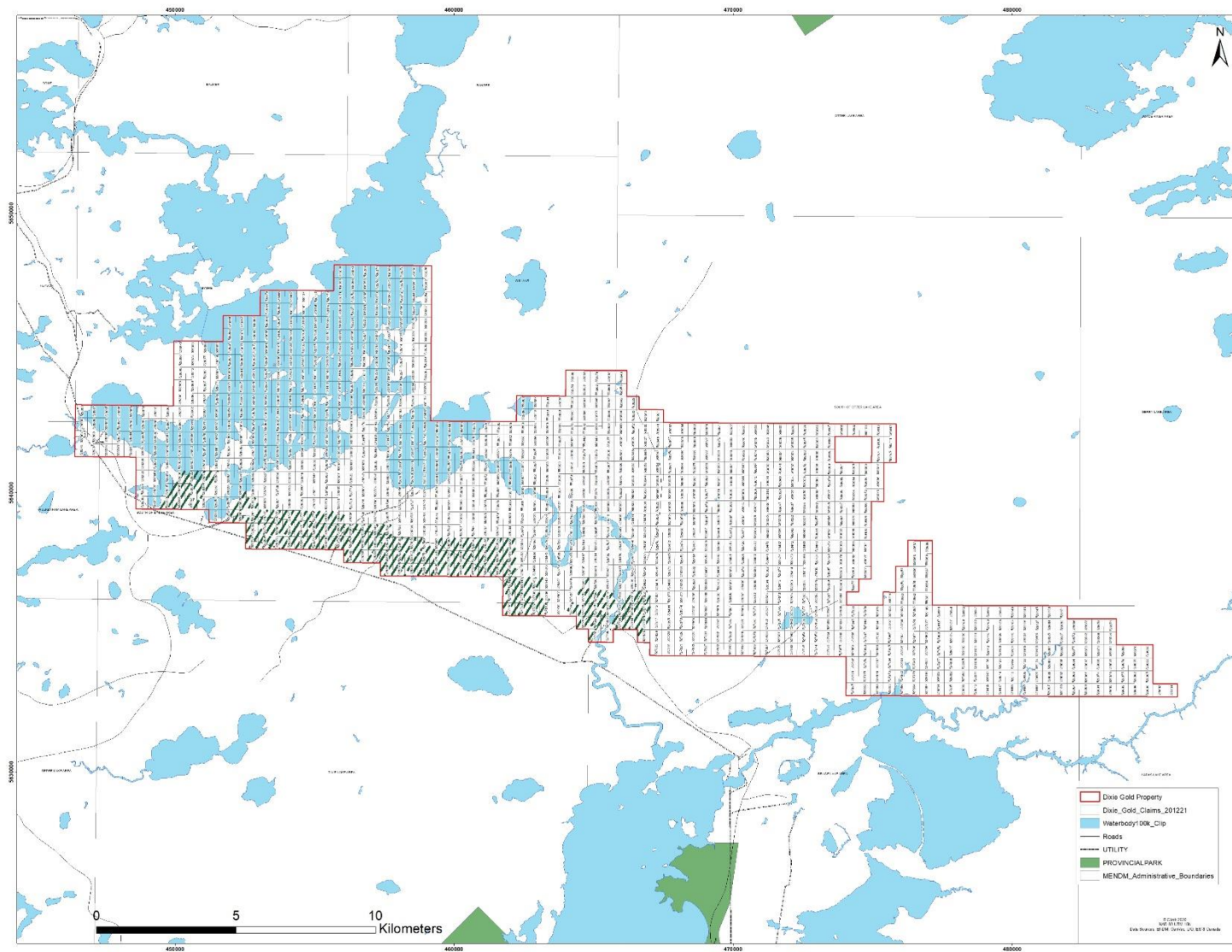
Figure 9: Location of SGH Samples in Relation to Dixie Gold's Project (Full View).
