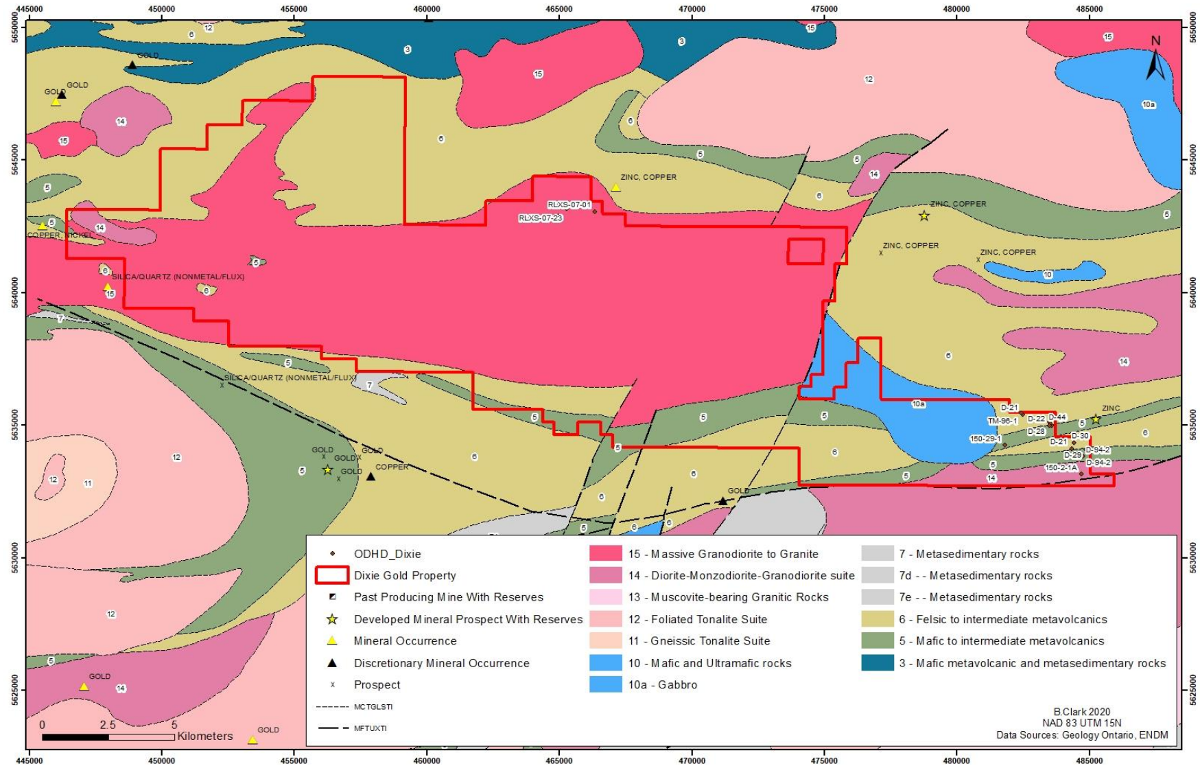
Figure 6: Property Geology (above)
