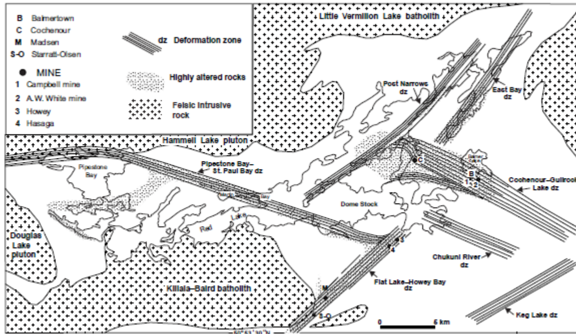
Figure 5: System of belt-scale transcurrent shear zones
