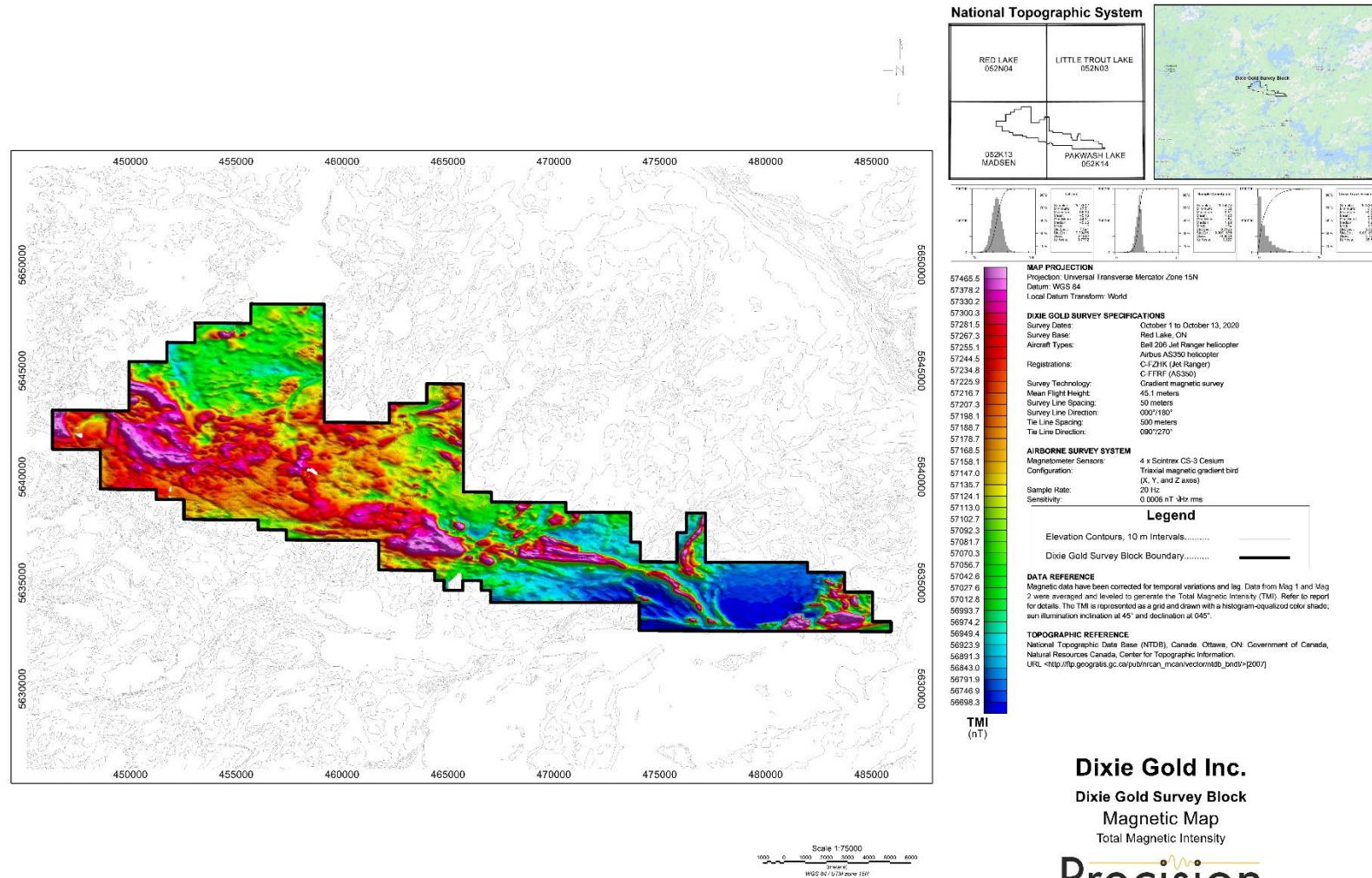
Figure 12: Dixie Gold Inc. - Property Total Field Magnetics ( above )
