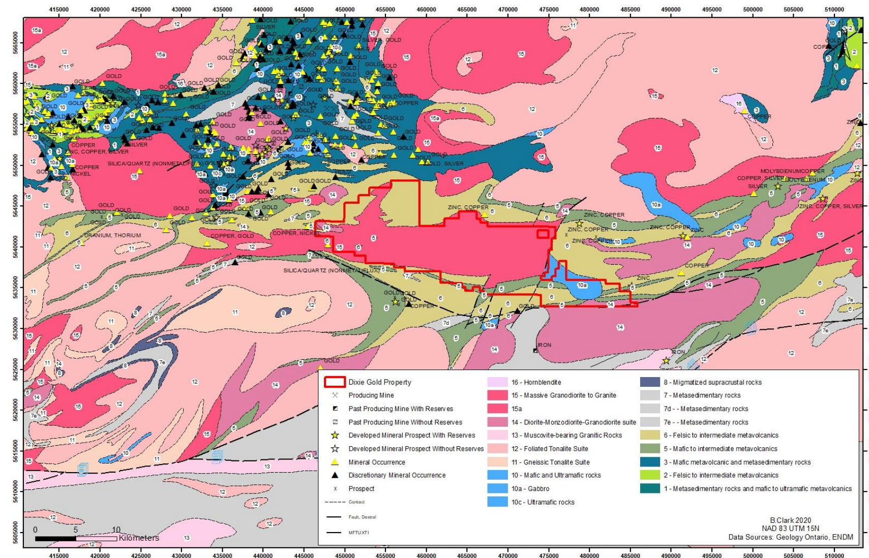
Figure 3: Geology of the Red Lake Greenstone Belt (above)
