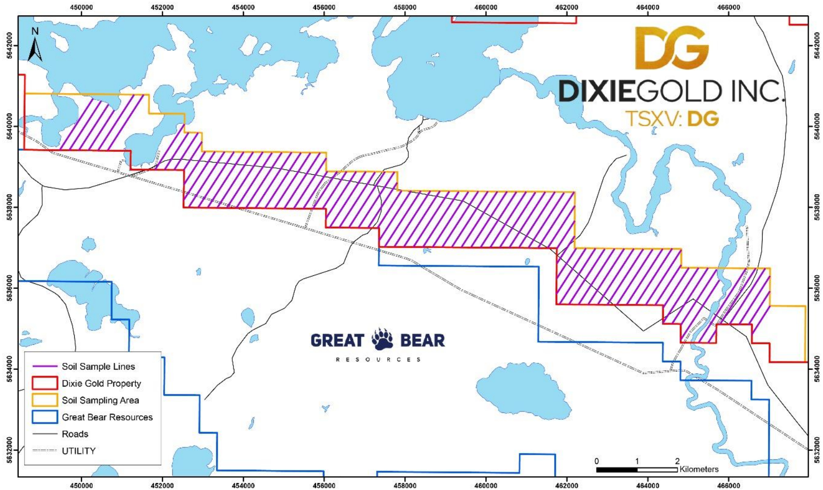
Figure 8: Location of Dixie Gold's SGH Sampling Lines (Fall 2020)
