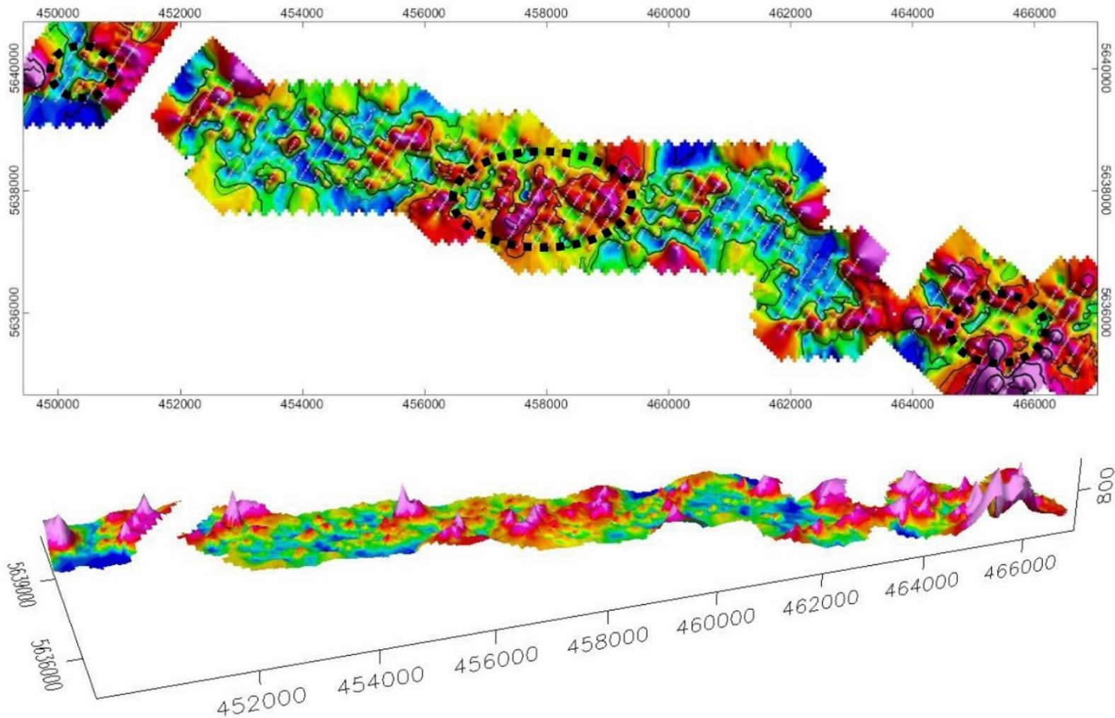
Figure 10: Dixie Gold Inc. SGH “Redox” Pathfinder Class Map (Halo Anomalies Illustrating Possible Presence of Redox Zones) (Brown 2020)
