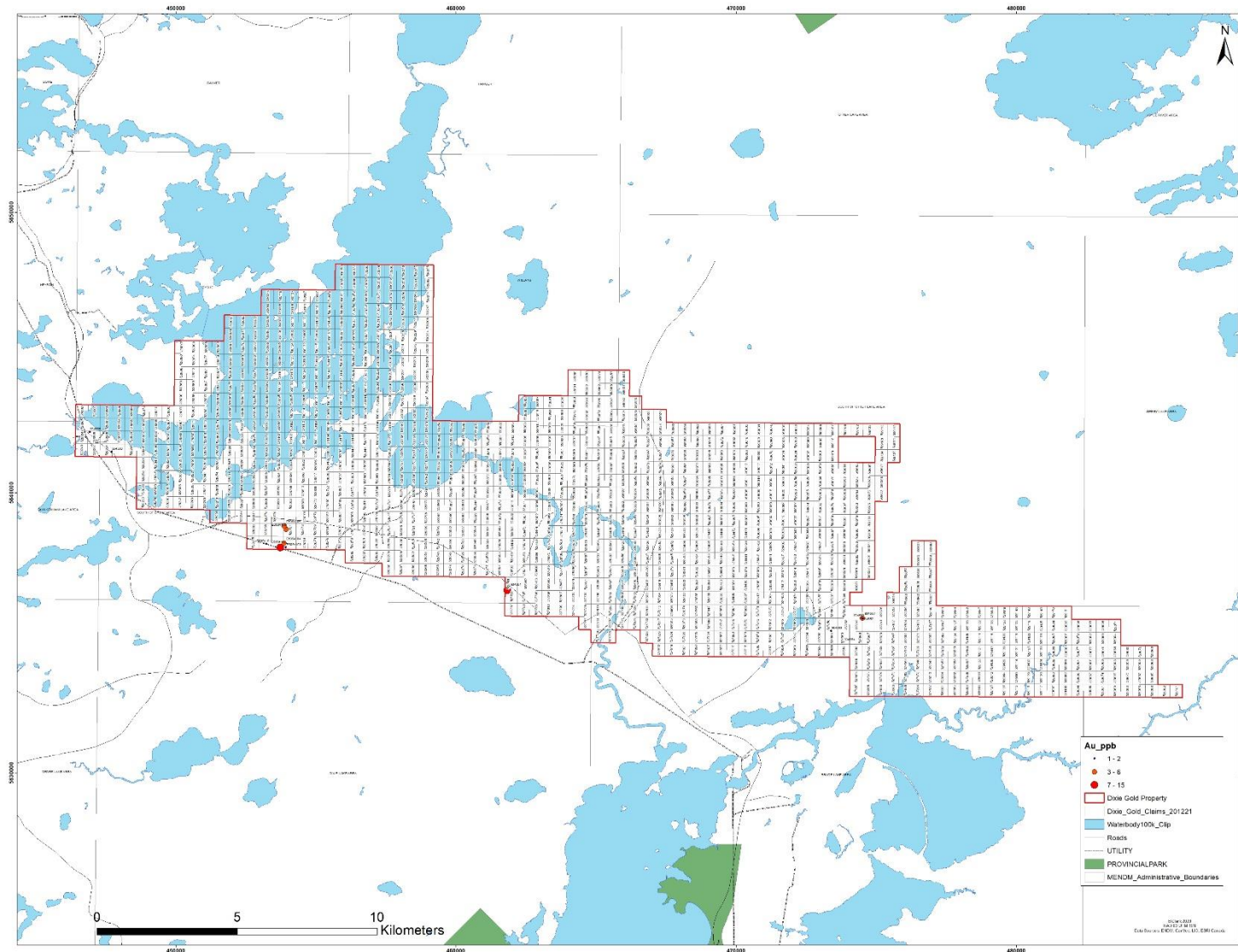
Figure 7: Location of Prospecting Samples
