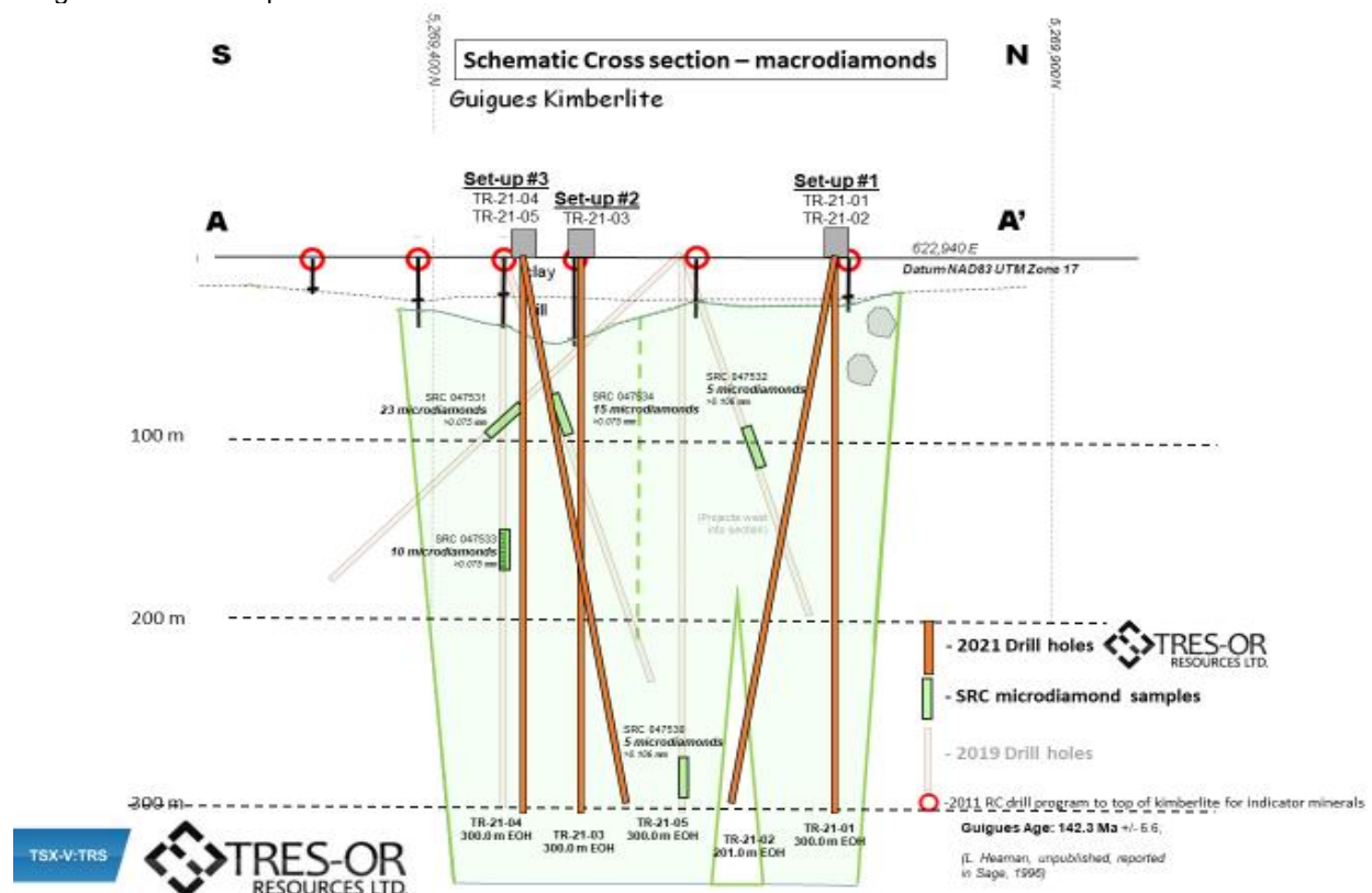
Figure 1: Schematic Cross Section presenting the November 2021 drilling program for macrodiamond testing of the Guigues Kimberlite Pipe.
