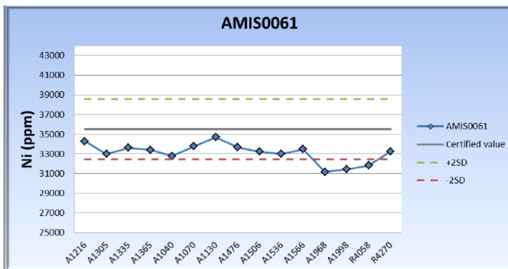
Figure 11-2: Performance of AMIS0061 for TNi.
