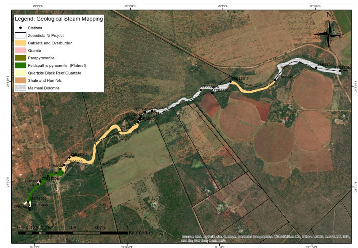
Figure 9-5: Geological field mapping results and station locations along the Rooisloot River, (McCreesh et al. , 2019).
