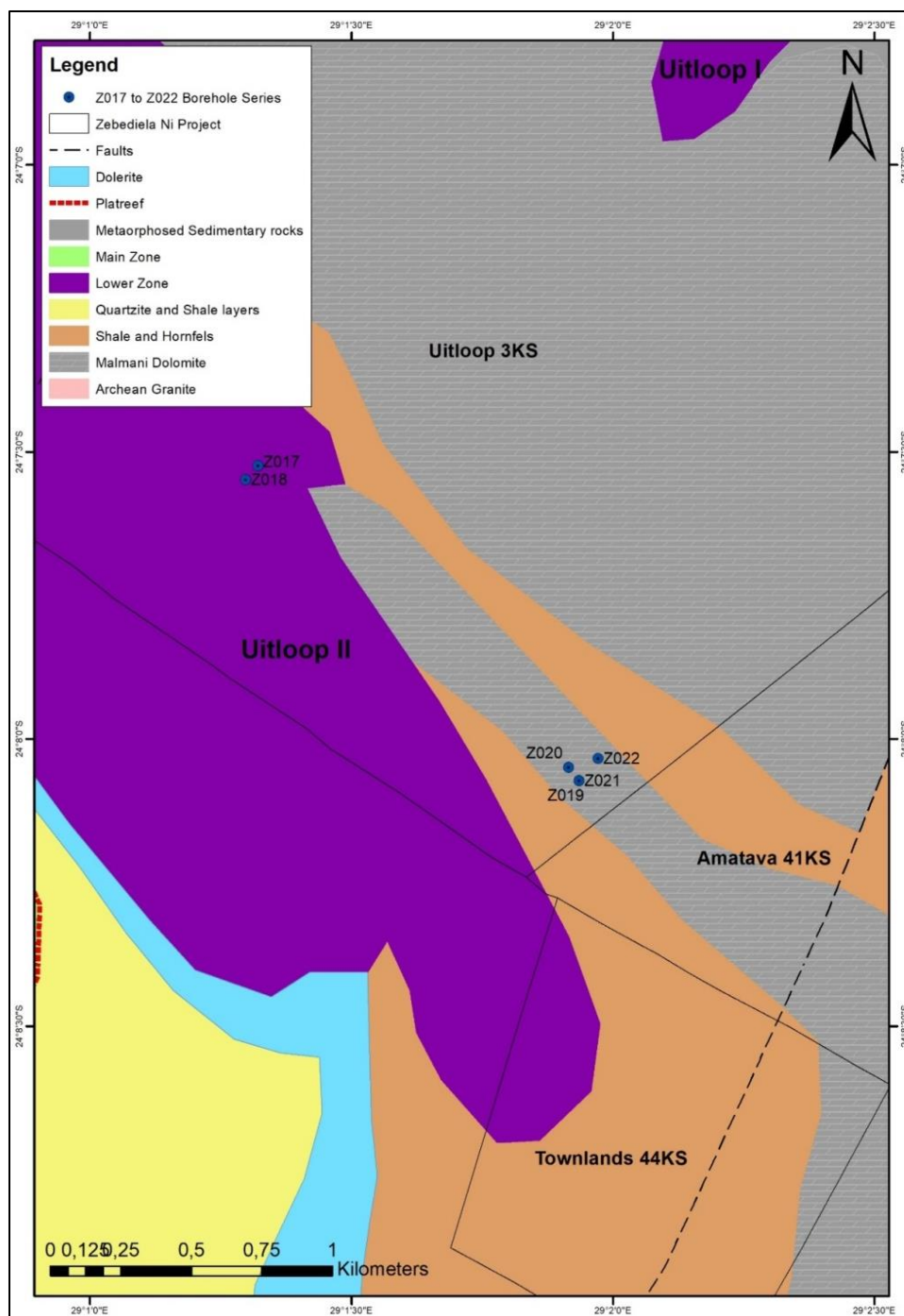
Figure 10-7: Locations of the 2017 to 2022 borehole series collars which targeted the Platreef contact-style mineralisation/ massive sulfides (Z017 and Z018) and Platreef strata-bound mineralisation (Z019 to Z022) (base geological map modified after van der Merwe, 1978).
