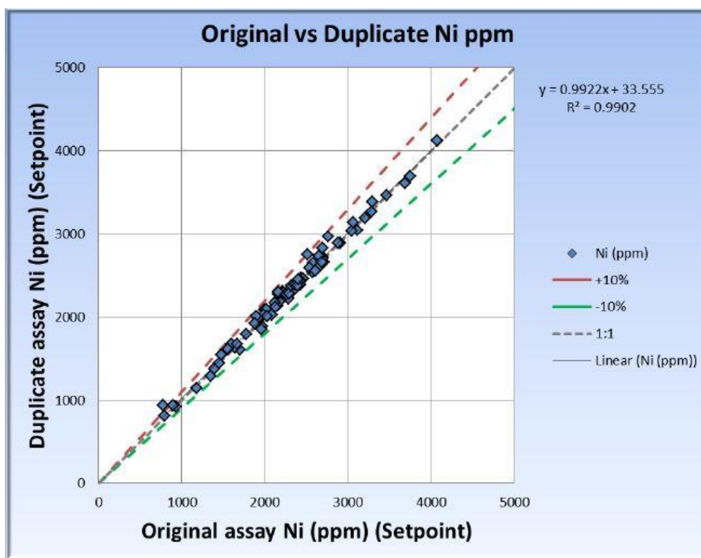
Figure 11-6: Original vs Duplicate plot (TNi).
