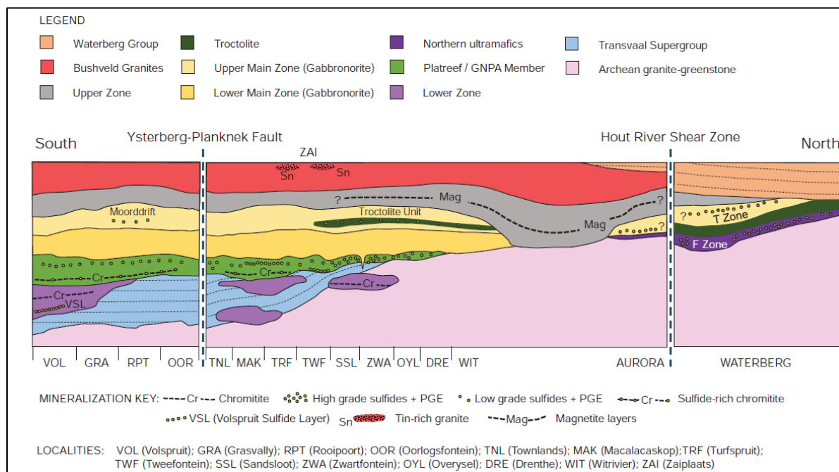
Figure 7-6: Schematic longitudinal section through the Northern Limb of the Bushveld Igneous Complex over the entire strike length (Kinnaird and McDonald, 2018). Note the positions of major east-west or NE-SW-trending structures such as the Ysterberg-Planknek fault and the Hout River Shear Zone the compartmentalise the Northern Limb.
