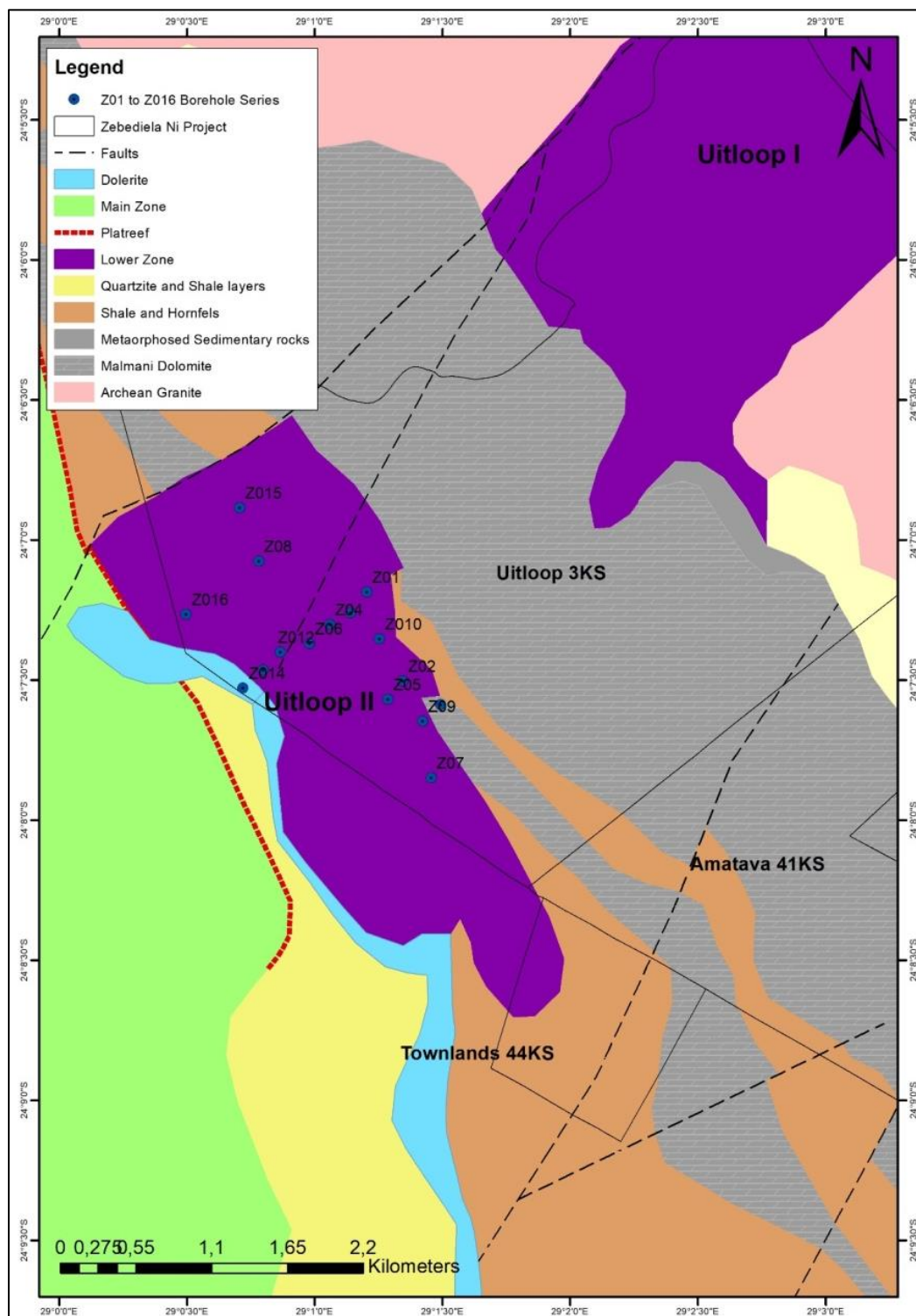
Figure 10-6: Locations of the Z01-2016 borehole series collars, which targeted the low-grade, disseminated Ni sulfide deposit associated with the Lower Zone Uitloop II body (base geological map modified after van der Merwe, 1978).
