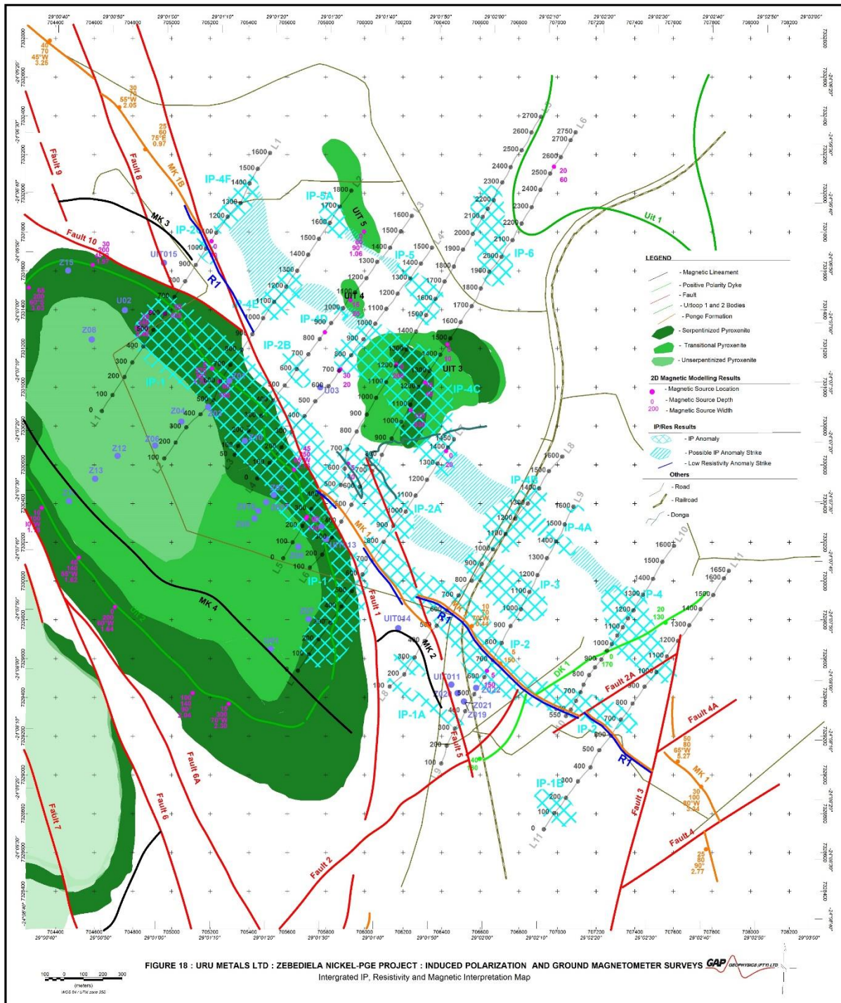
Figure 9-7: Interpreted and integrated induced polarization, resistivity, and ground magnetics surveys showing IP anomalies (light blue cross-hatching) and a low resistivity anomaly (solid dark blue line), from work completed in 2018 (Boitshepo et al. , 2018).
