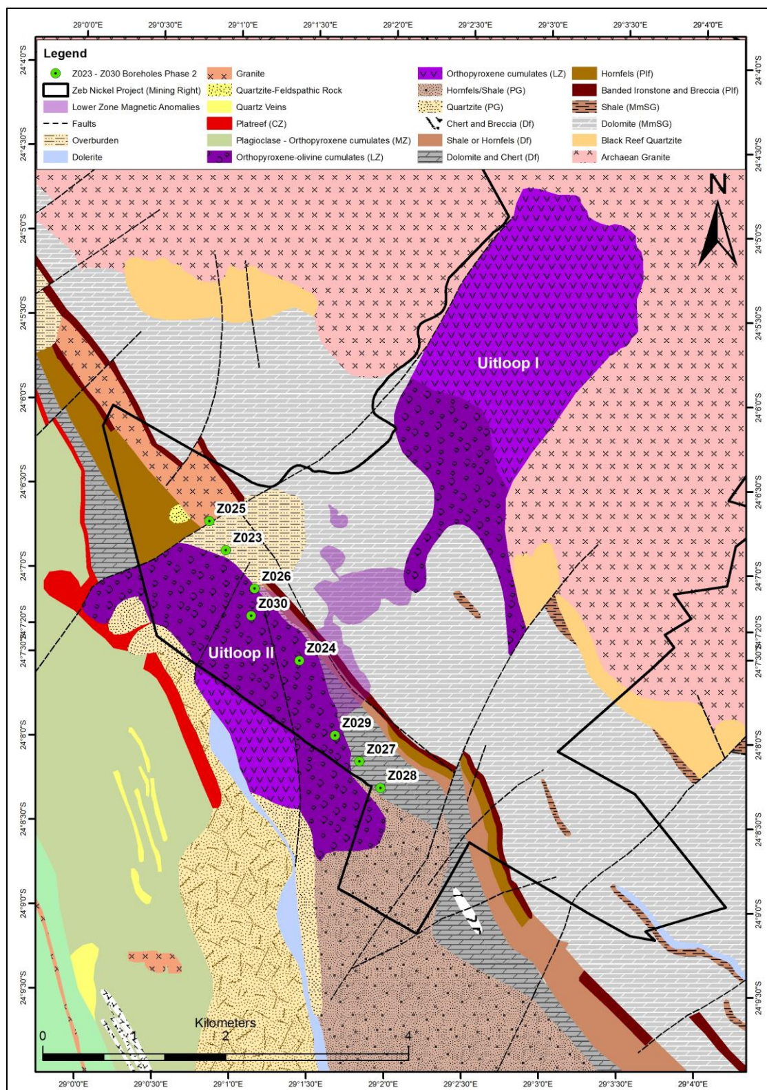
Figure 10-8: Locations of the 2023 to 2030 borehole series collars overlain on 2022 geological map.
