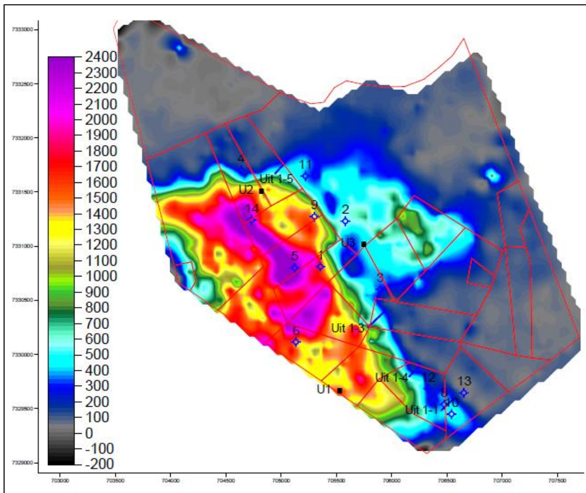
Figure 9-3: Soil geochemistry contours showing ppm nickel results and approximate positions of historical UIT series (labelled Uit) and UL series (numbered blue 4 point stars) boreholes and 2007 U series (black squares) boreholes.
