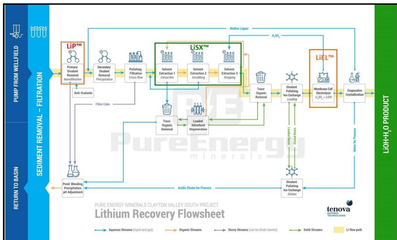
Figure 19. Flow Diagram outlining the Tenova extraction process from Pure Energy (2017).
