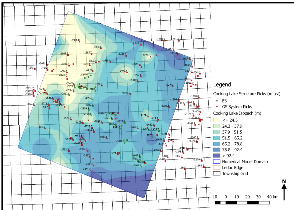
Figure 21. Isopach map of the Cooking Lake Formation
