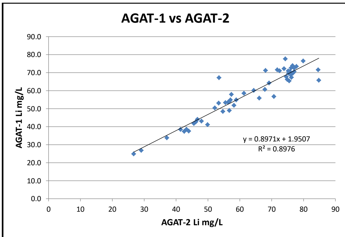
Figure 15. Scatter plot of duplicate Li-brine well sample analyses from AGAT laboratory.
