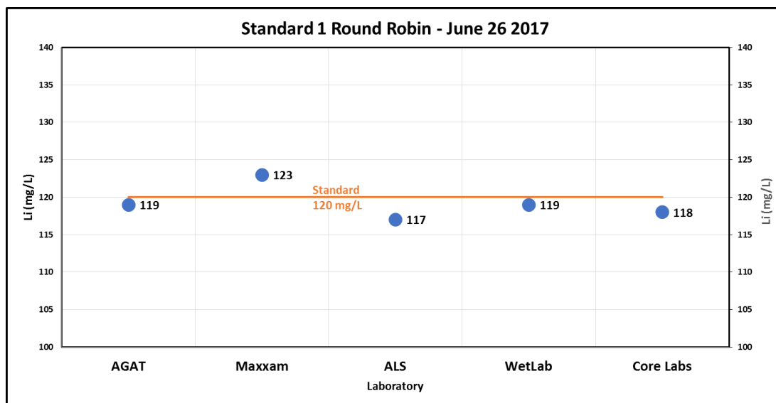
Figure 14. Results of lithium standard analyses from five laboratories.
