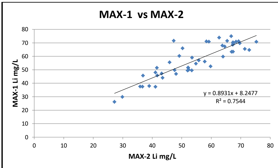
Figure 16. Scatter plot of duplicate Li-brine well brine sample analyses from Maxxam laboratory.
