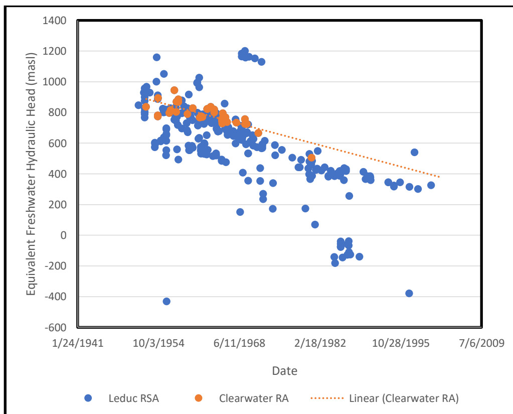
Figure 25. CCRA DST derived hydraulic heads over time as compared to regional data.
