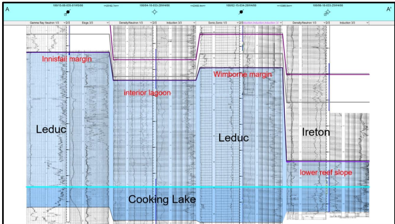
Figure 9: Geological stratigraphic cross section of the CCRA, line A-A' (Fig. 8) using a Cooking Lake Datum (E3 Metals Corp. using GeoLOGIC Systems). This cross section demonstrates the reservoir continuity across the Clearwater area Leduc platform. It highlights the relative thickness of the Leduc reef margins at Innisfail and Wimborne to the thinner interior platform lagoon and the lower reef slope towards the basin on the east side.
