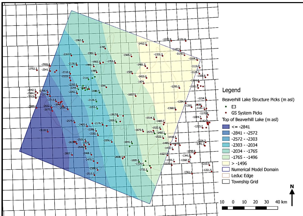
Figure 24. Top of the Beaverhill Lake Group
