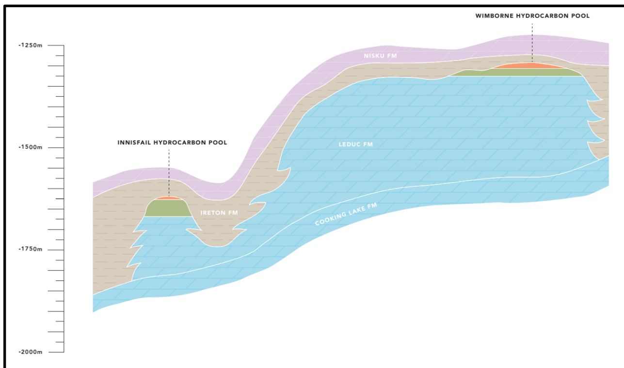
Figure 10: Schematic representation of the CCRA (to scale with vertical exaggeration) highlighting the current relationships of the geology, structure, and hydrocarbon pools. (E3 Metals, 2017)
