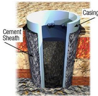
Figure 16-8. Example of cemented casing strings and cement sheath (Ref: 3m.com)
