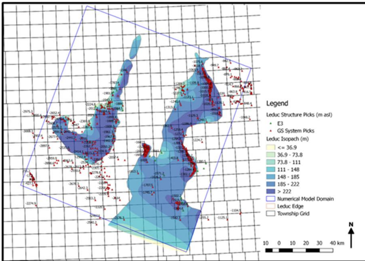
Figure 14-1. Isopach map of the Leduc Aquifer
