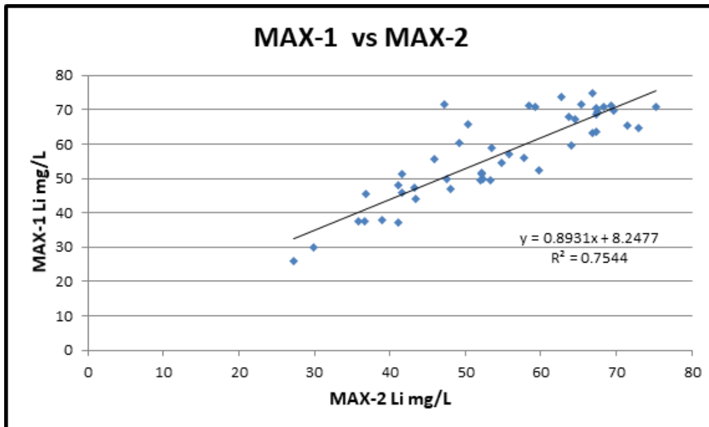
Figure 11-3. Scatter plot of duplicate Li-brine well sample analyses from Maxxam laboratory.
