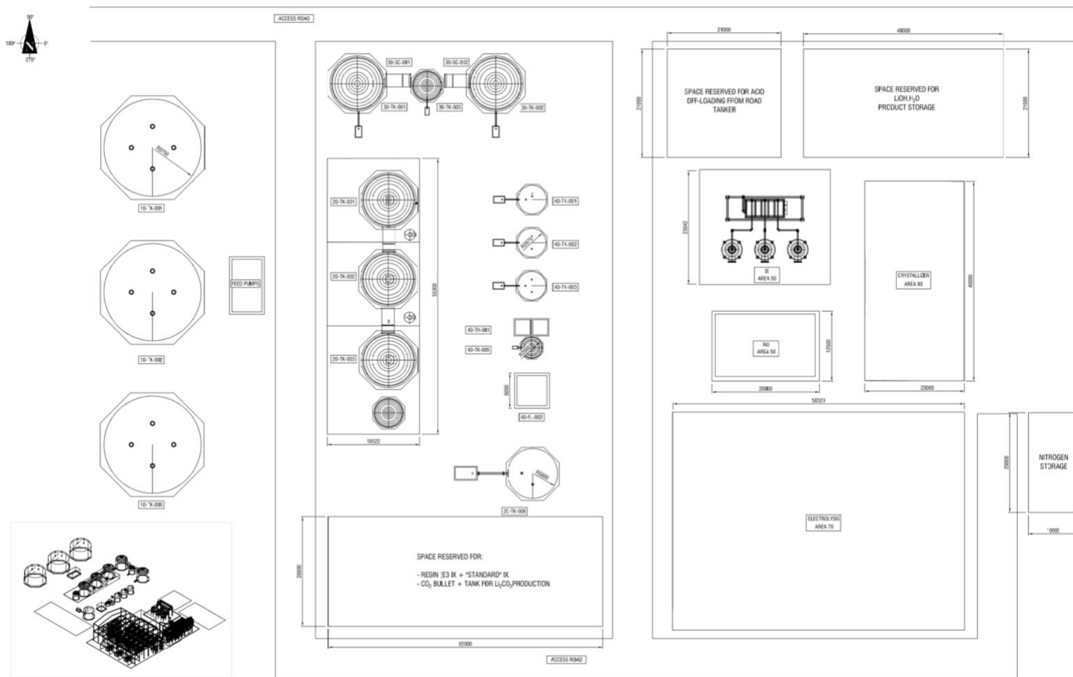
Figure 17-4. Overall lithium processing plant conceptual layout
