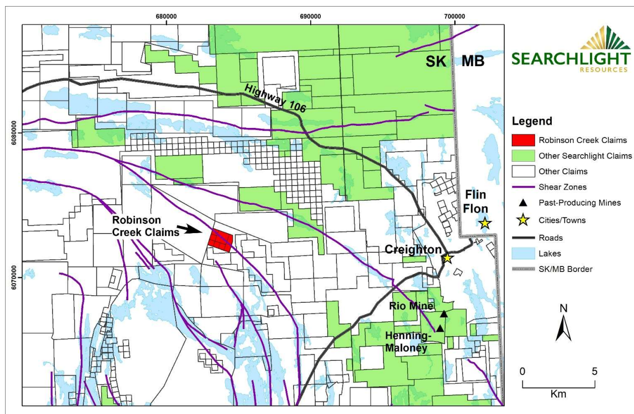
Map 3 – Location of Robinson Creek claims
