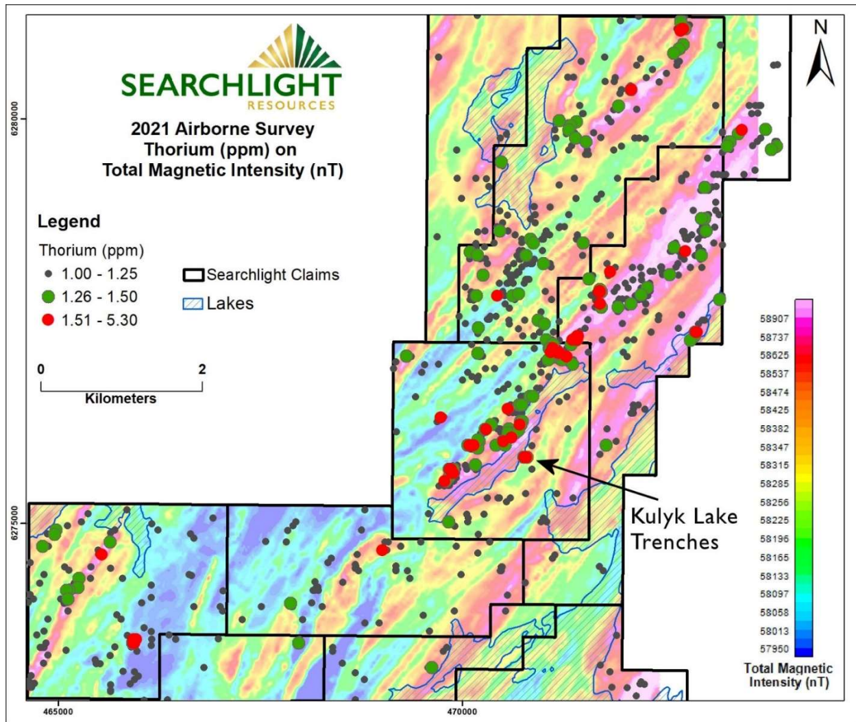
Map 6. Thorium (ppm) overlaid on Total Magnetic Intensity (nT), 2021 Airborne Survey, Kulyk Lake Project
