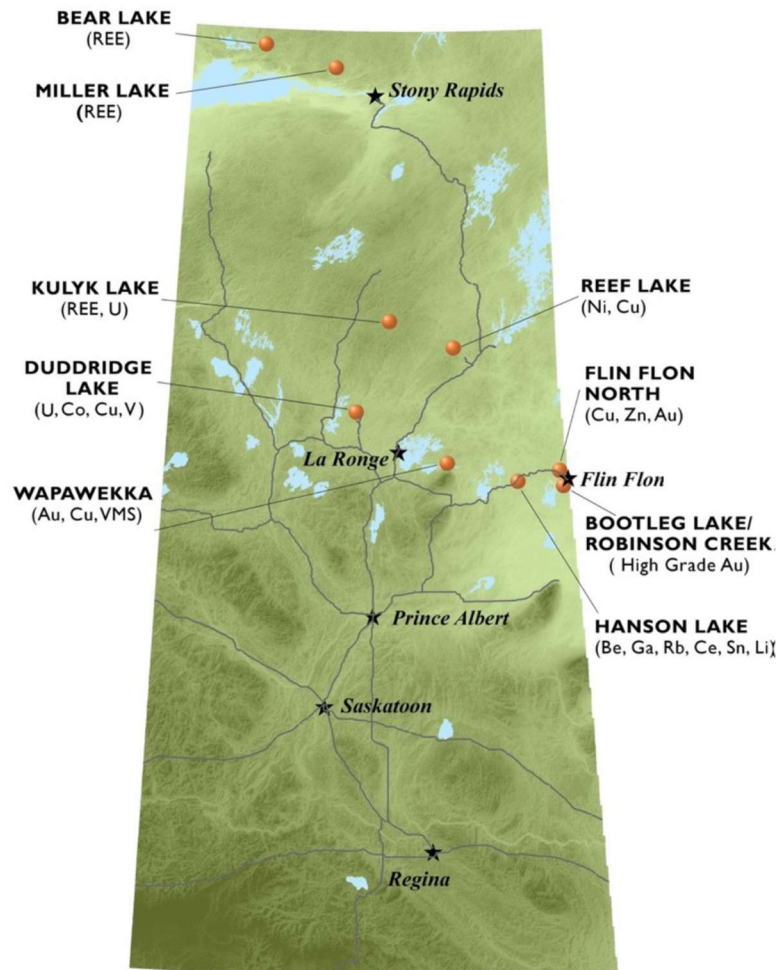
Map 1 – Location of Searchlight Resources Projects in Saskatchewan
