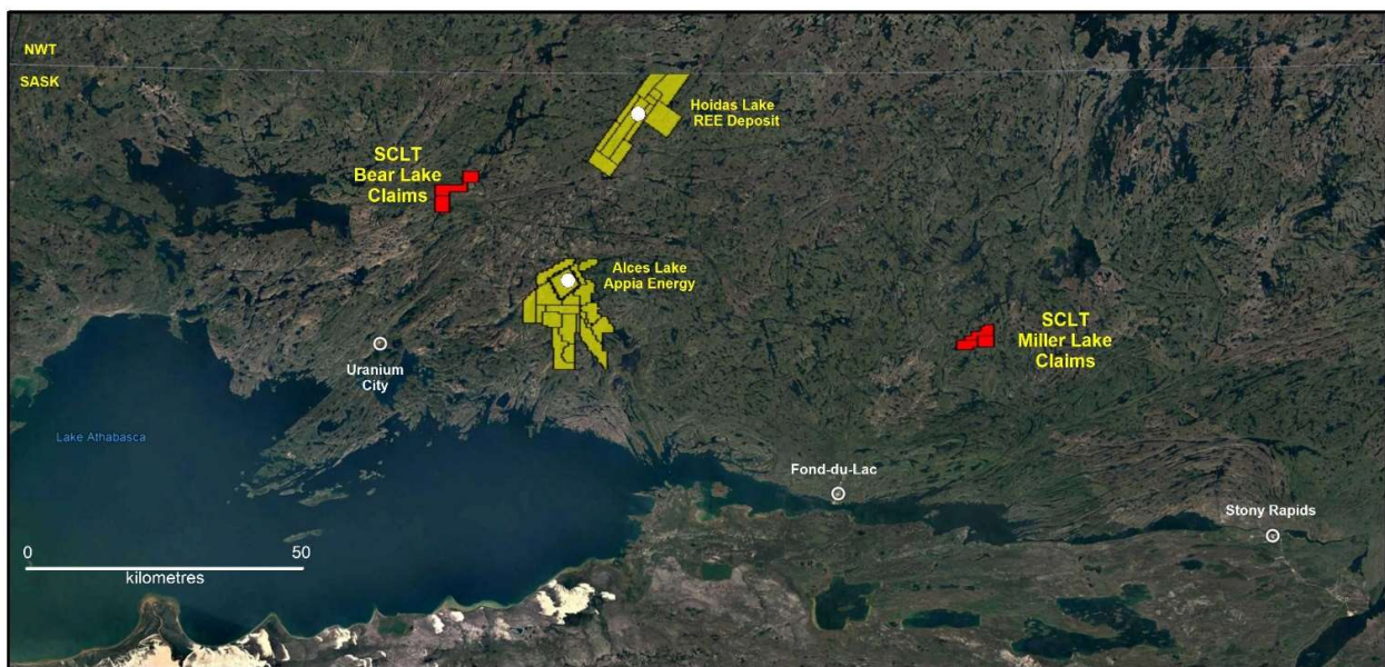
Map 2 – Location of Bear Lake and Miller Lake Rare earth project
