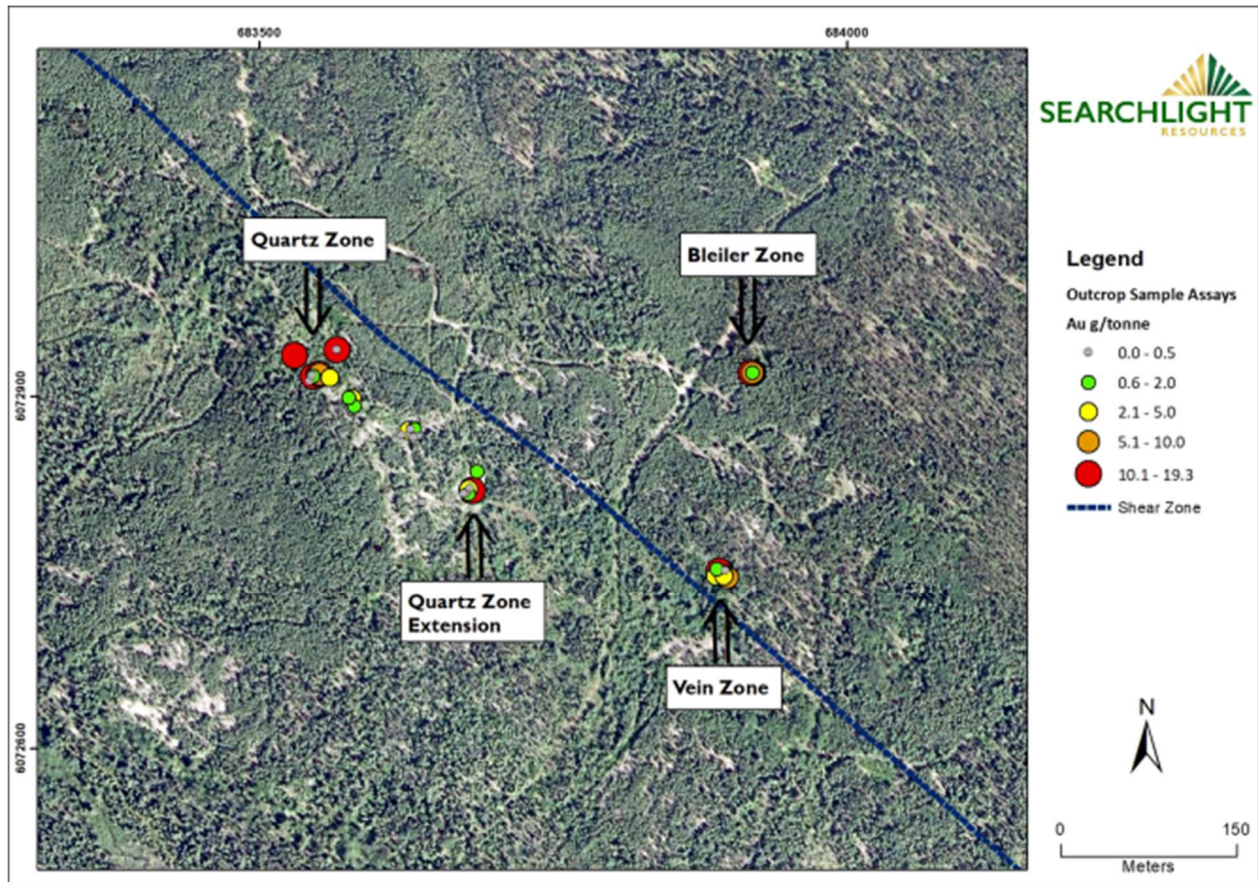
Map 4. Gold Assays (g/t) from Outcrop Samples from the Robinson Creek Mineralized Zones
