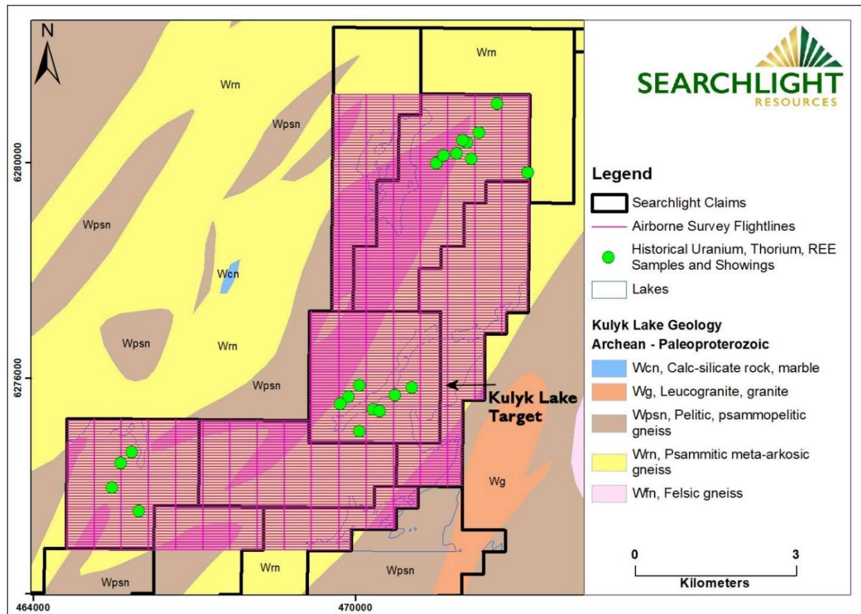
Map 5. Flightlines for 2021 Airborne Magnetic and Radiometric Surveys, Kulyk Lake Project, with Historical Showings
