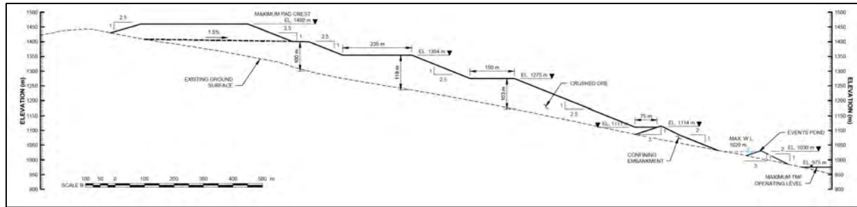
Figure 18-9: Heap Leach Facility Cross-Section (KP, 2021)
