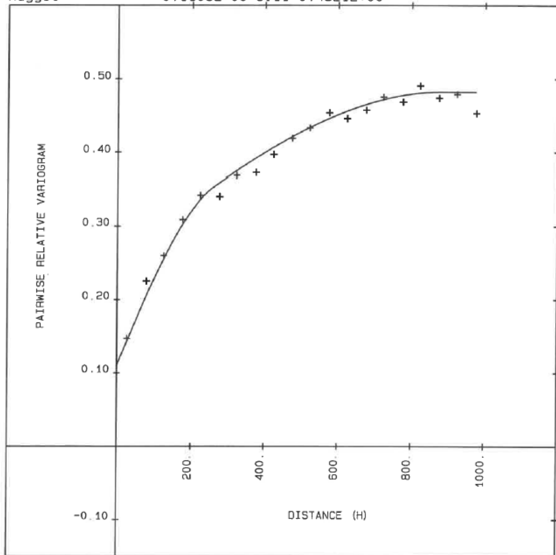
Figure 14-9: Total Copper Variogram – Supergene Sulphide
