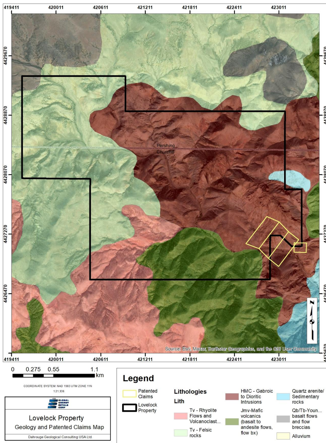
Figure 7-2 Lovelock Cobalt Mine Property Geology Map
