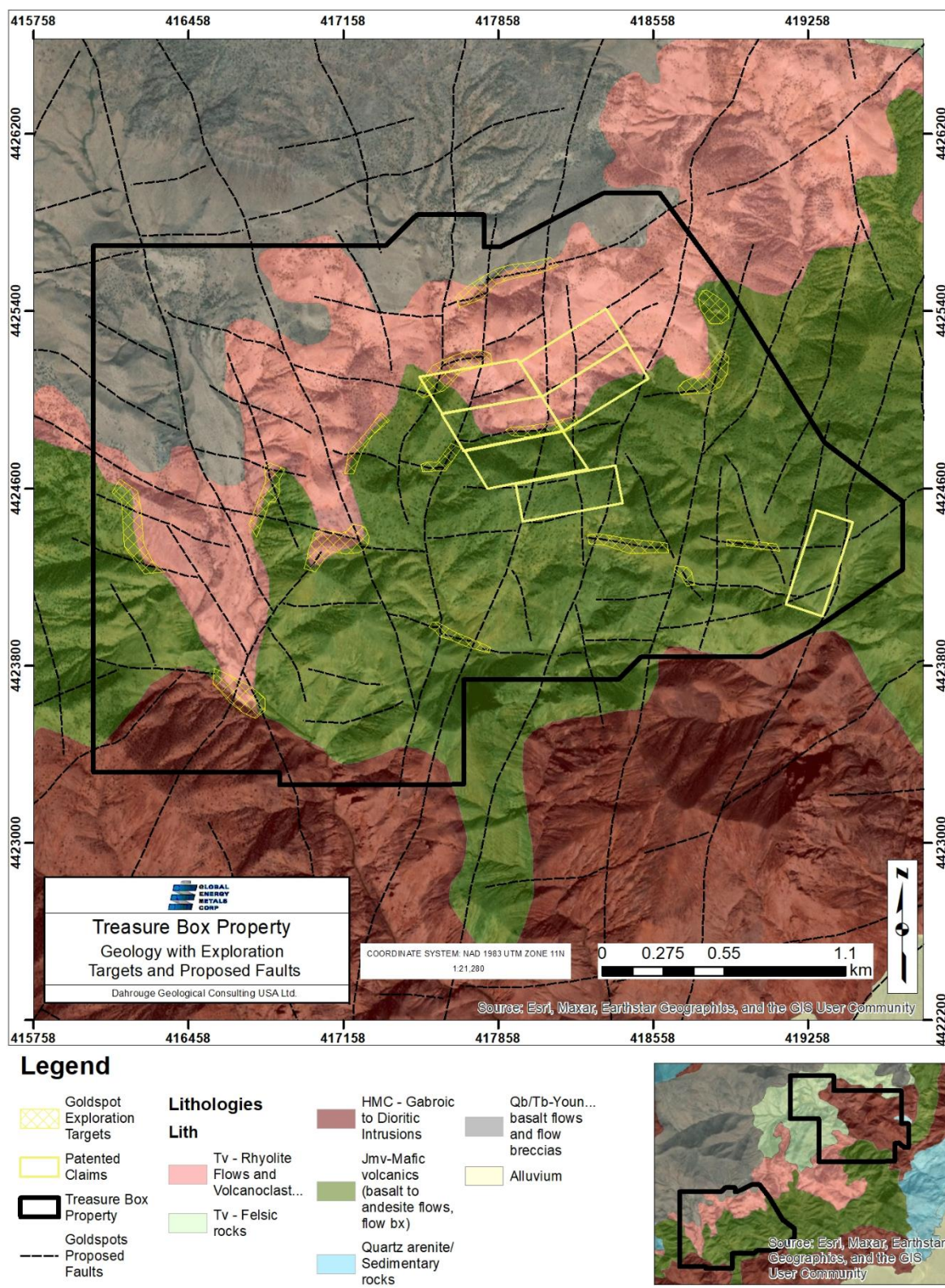
Figure 9-9 Treasure Box Mine Property Targets with Interpreted Faults and Geology
