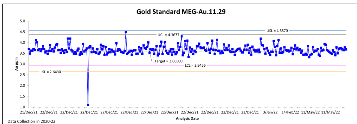
Figure 11-5. Control Chart for Gold CRM MED-Au.11.29.
