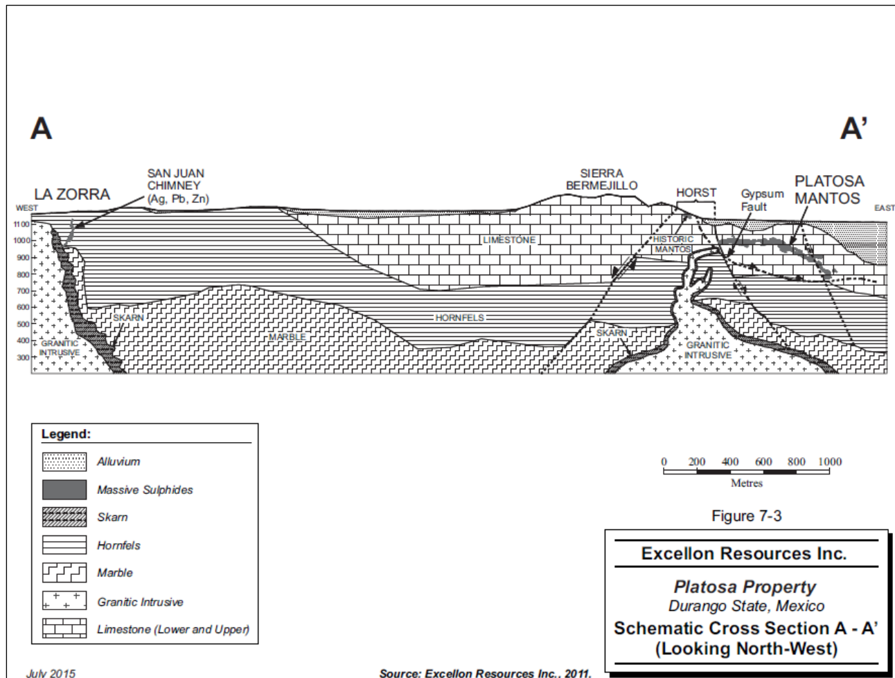
Figure 8: General Stratigraphic Cross-Section of the Platosa Mine Area
