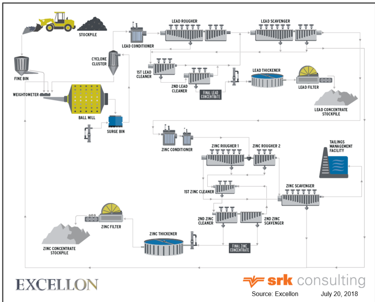
Figure 32: Flowsheet for the Miguel Auza Concentrator
