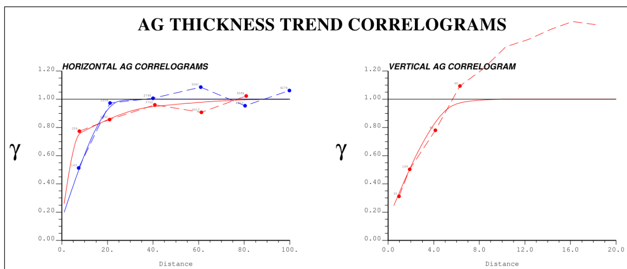
Figure 26: Silver Correlogram for Platosa Mine
