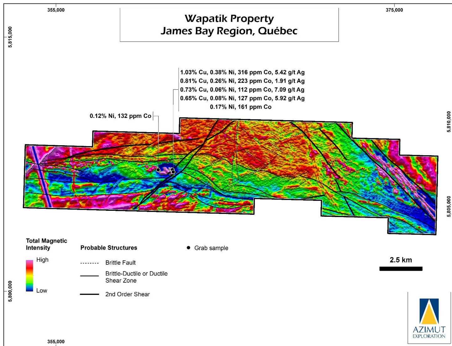
Figure 10: Magnetic map of the Wapatik Property showing structures and the locations of known mineralization.
