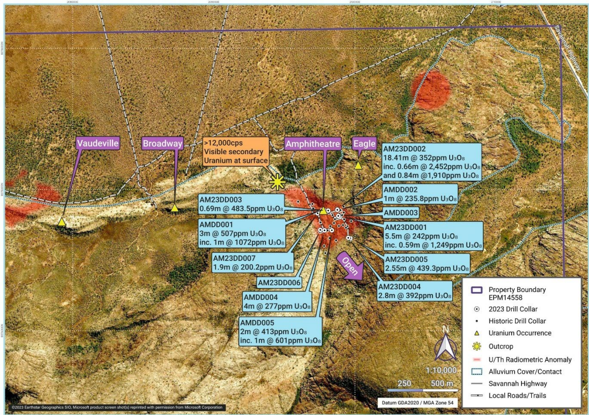
Figure 10.14 Summary of drilling results at Amphitheatre
