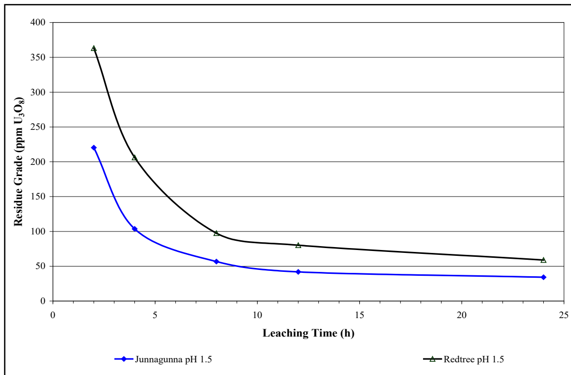
Figure 13.1 ANSTO Base Case Conventional Leach Test Kinetics
