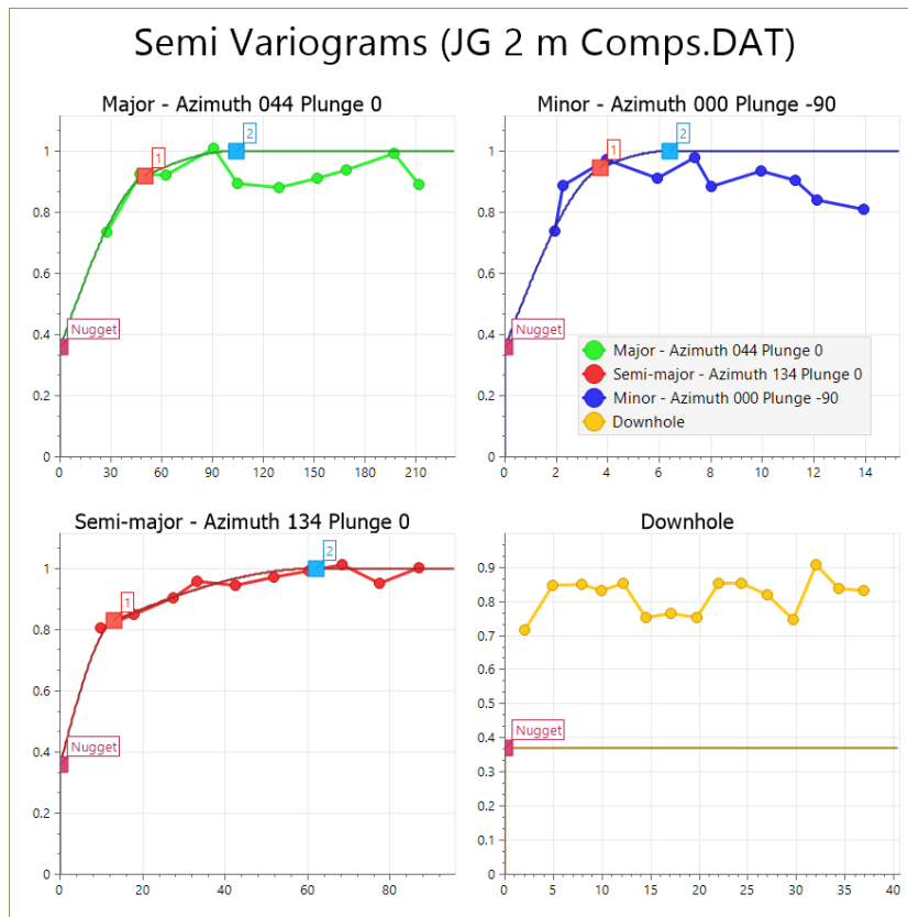
Figure 14.13 Junnagunna semi-variograms.
