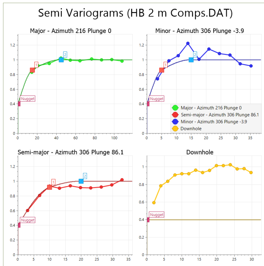
Figure 14.12 Huarabagoo semi-variograms.
