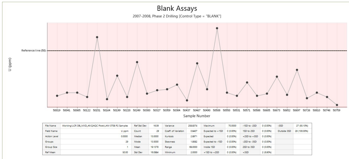
Figure 11.11 Phase 2, Drilling 2007 – 2008, Blank Assay Results
