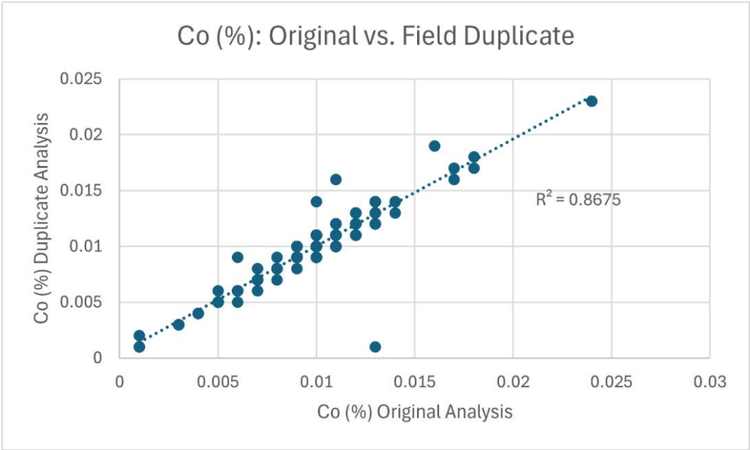
Figure 11-9. Plot of Absolute Concentrations of Pairs of Duplicate Samples Analyzed for Cobalt (Co) (Caracle Creek, 2024).
