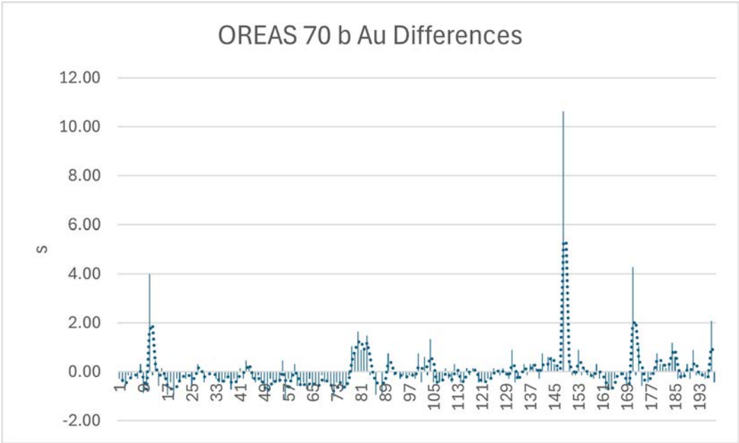
Figure 11-3. CRM OREAS 70b – Number of Standard Deviations Difference for Au Analysis from the Average Value for Various Analytical Runs (Caracle Creek, 2024).
