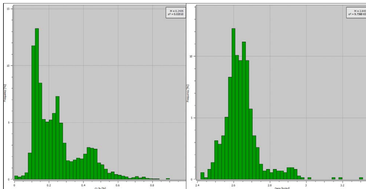
Figure 14-10. Multimodal histograms for EST Domain Chromium grades (left) and density values (right) (Caracle Creek, 2024).
