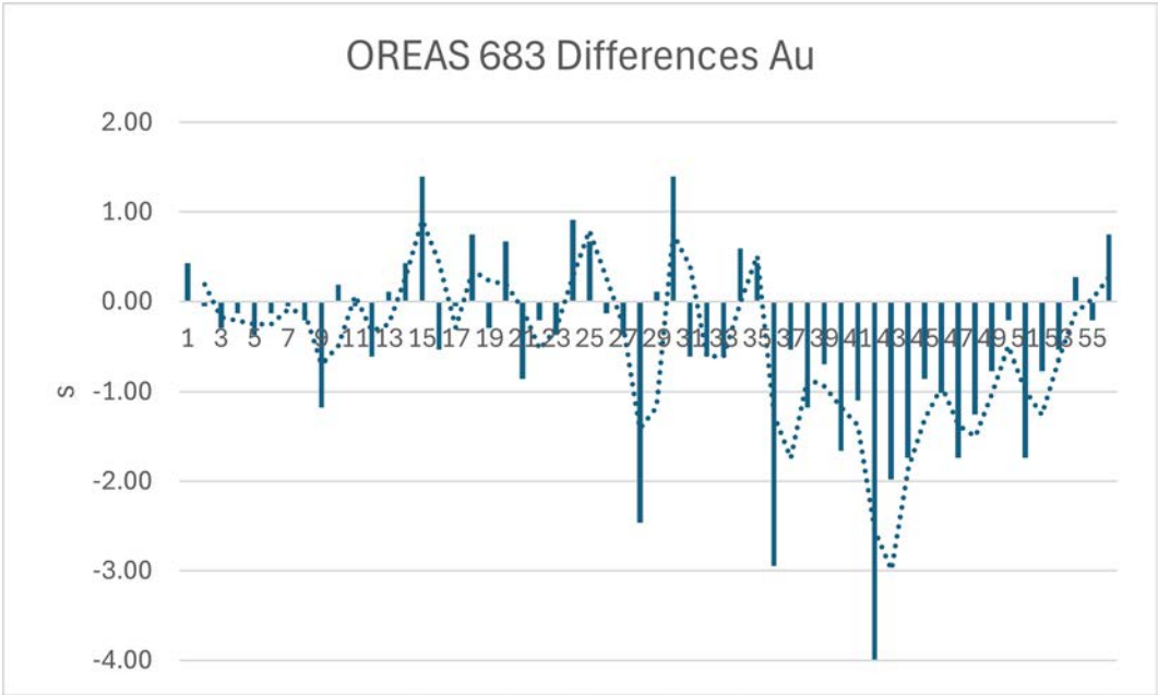
Figure 11-6. CRM OREAS 683 – Distribution of Standard Deviations Difference for Au Analysis from the Average Value for Various Analytical Runs (Caracle Creek, 2024).
