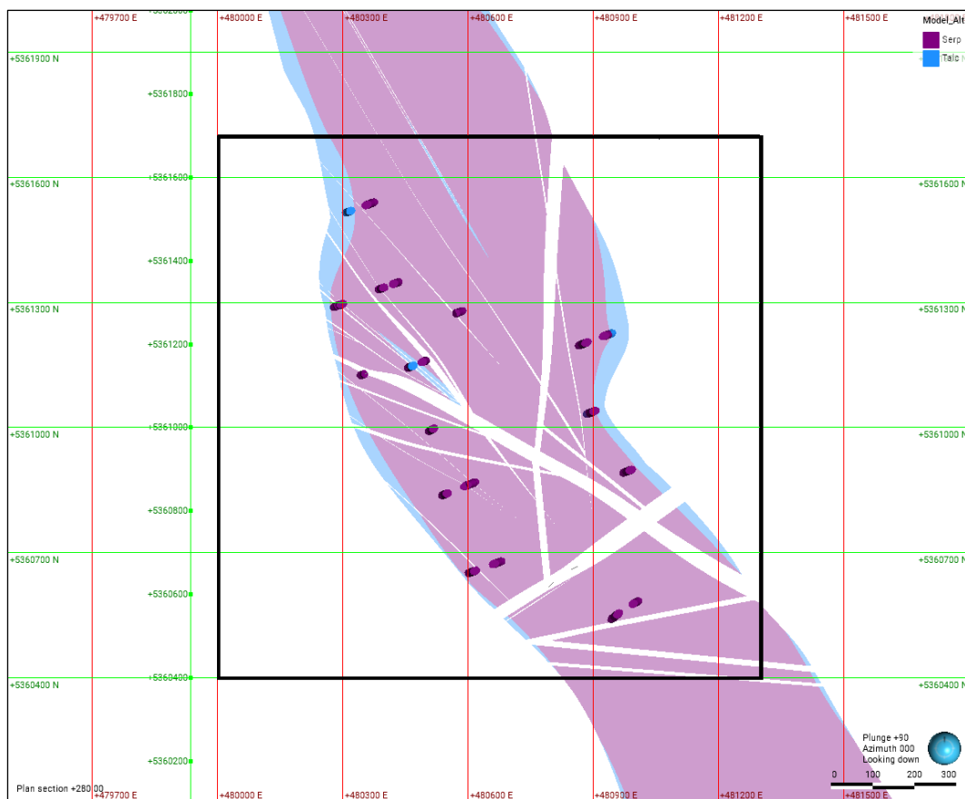
Figure 14-6. Plan section (280 m level) of the Extended Alteration Model with CNC drill hole Intercepts. The black square represents the current resource boundary and main modelling area (Caracle Creek, 2024).
