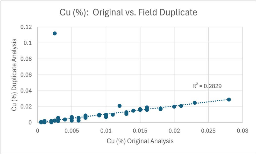
Figure 11-13. Plot of Absolute Concentrations of Pairs of Duplicate Samples Analyzed for Copper (Cu) (Caracle Creek, 2024).
