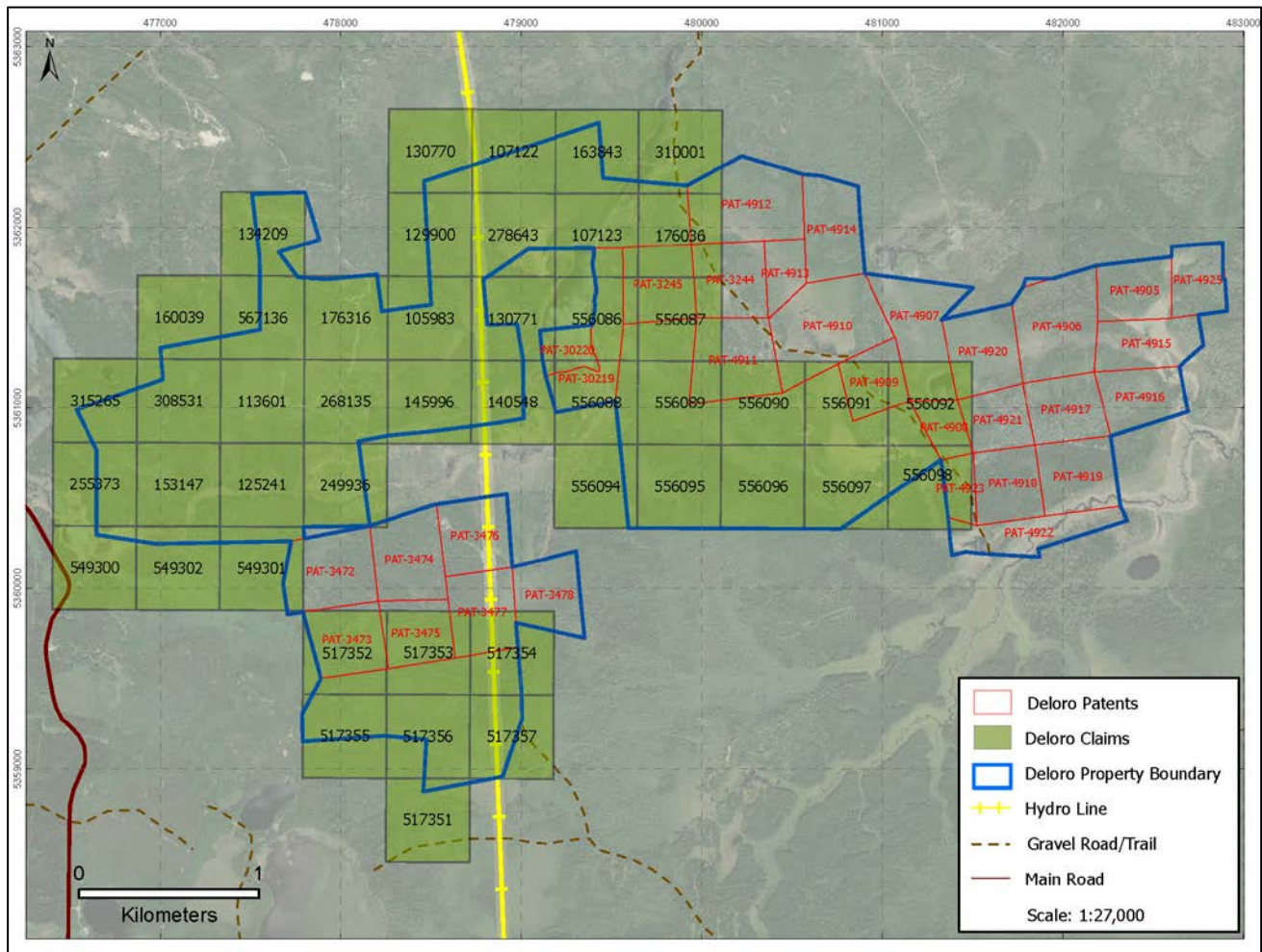
Figure 4-2. Land tenure of the Deloro Project showing the unpatented mining claims and Crown Patents. The Property comprises the Crown Patents (red boundaries) and the unpatented mining claims (blue boundary), the latter which does not encompass entire SCMC claim units (green) (Canada Nickel, 2024).
