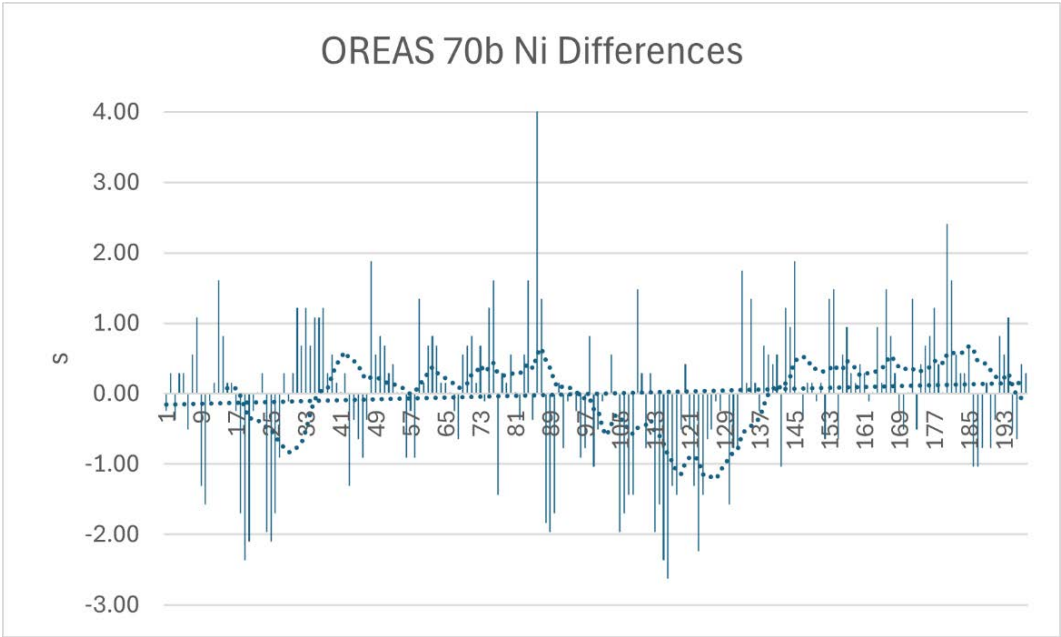
Figure 11-1. CRM OREAS 70b – Number of Standard Deviations Difference for Ni Analysis from the Average Value for Various Analytical Runs (Caracle Creek, 2024).
