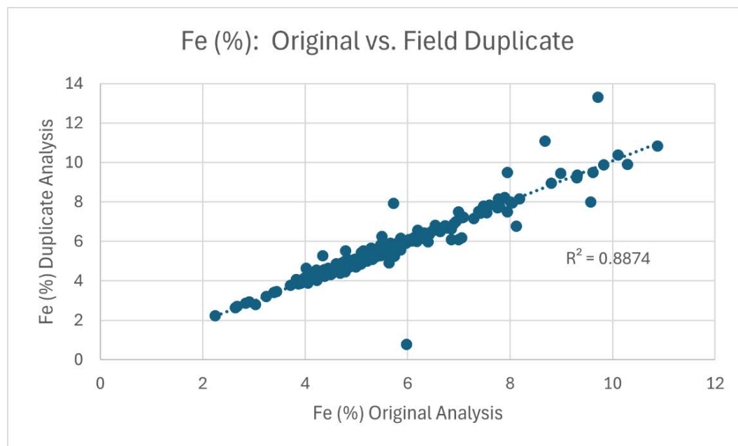
Figure 11-14. Plot of Absolute Concentrations of Pairs of Duplicate Samples Analyzed for Iron (Fe) (Caracle Creek, 2024).
