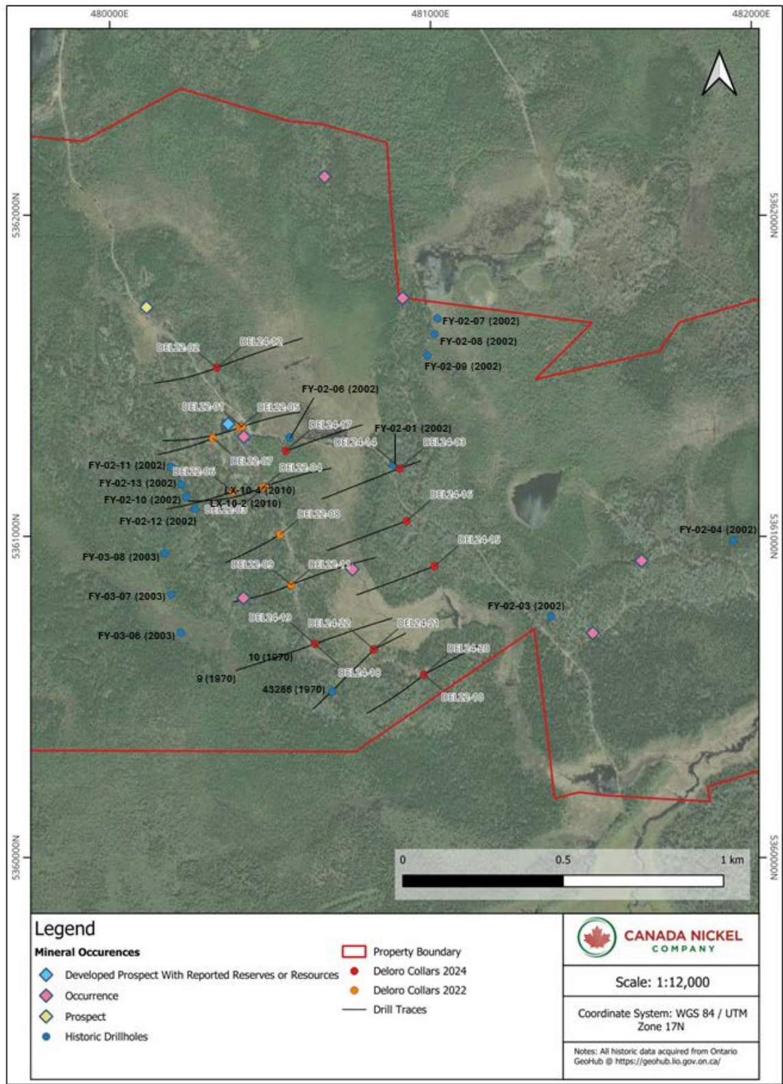
Figure 6-3. Location of historical drill holes, prospects and mineral occurrences, and collars and traces from the 2022 and 2024 drill holes completed by CNC, within the Deloro Property (see also Figure 6-2) (Canada Nickel, 2024).
