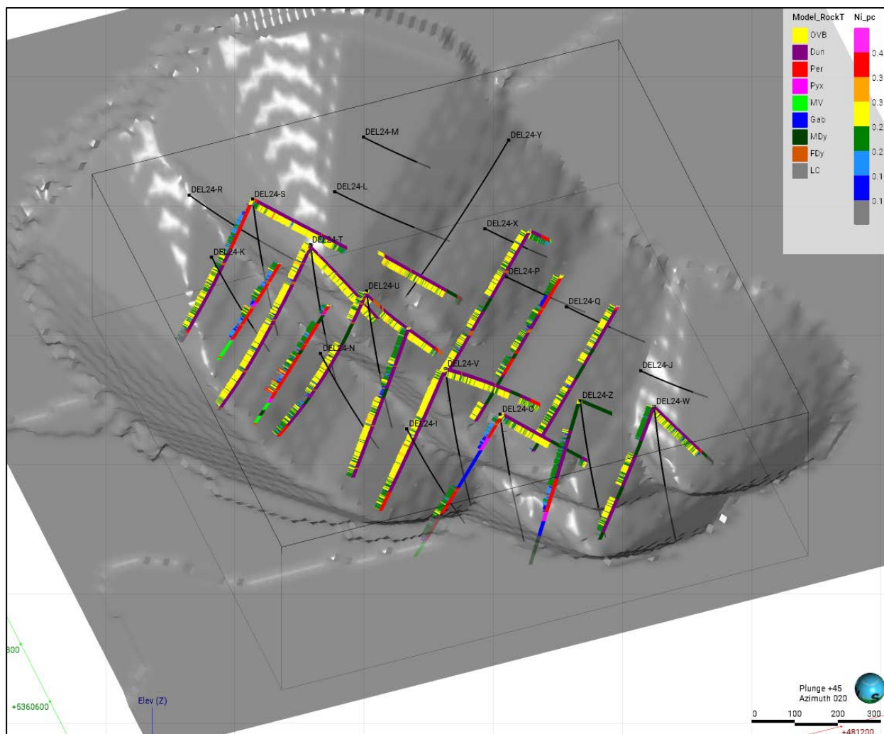
Figure 26-2. Isometric view of the 18 proposed diamond drill holes (black traces) within shaded area of the optimized pit shell and unlabelled drill holes (with Ni% and lithologies) used in the current mineral resource estimate, Deloro Project (Caracle Creek, 2024).
