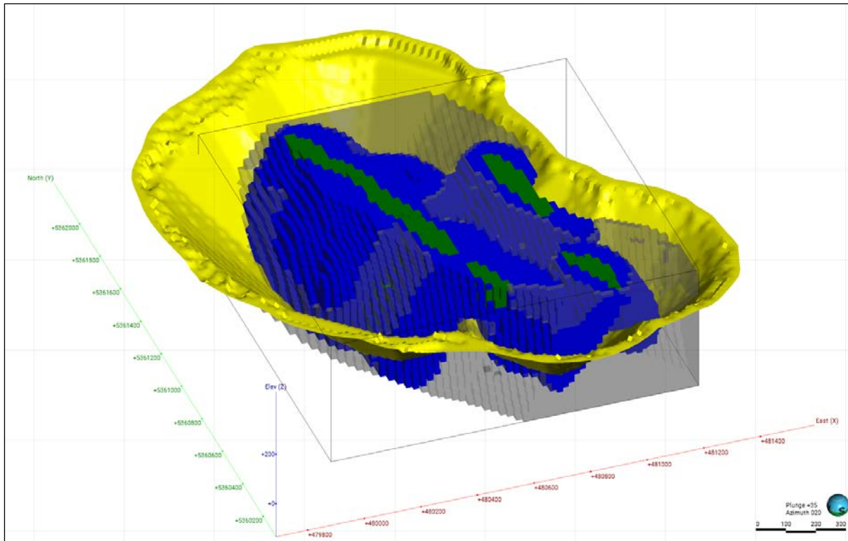
Figure 14-25. 3D Perspective (Looking NE) of the Pit Shell and Resource Classification Blocks. Conceptual pit shell (yellow) against indicated (green), inferred (blue) and potential (transparent grey) resource blocks. The box-shaped edges represent the current resource boundary and main modelling volume (Caracle Creek, 2024).
