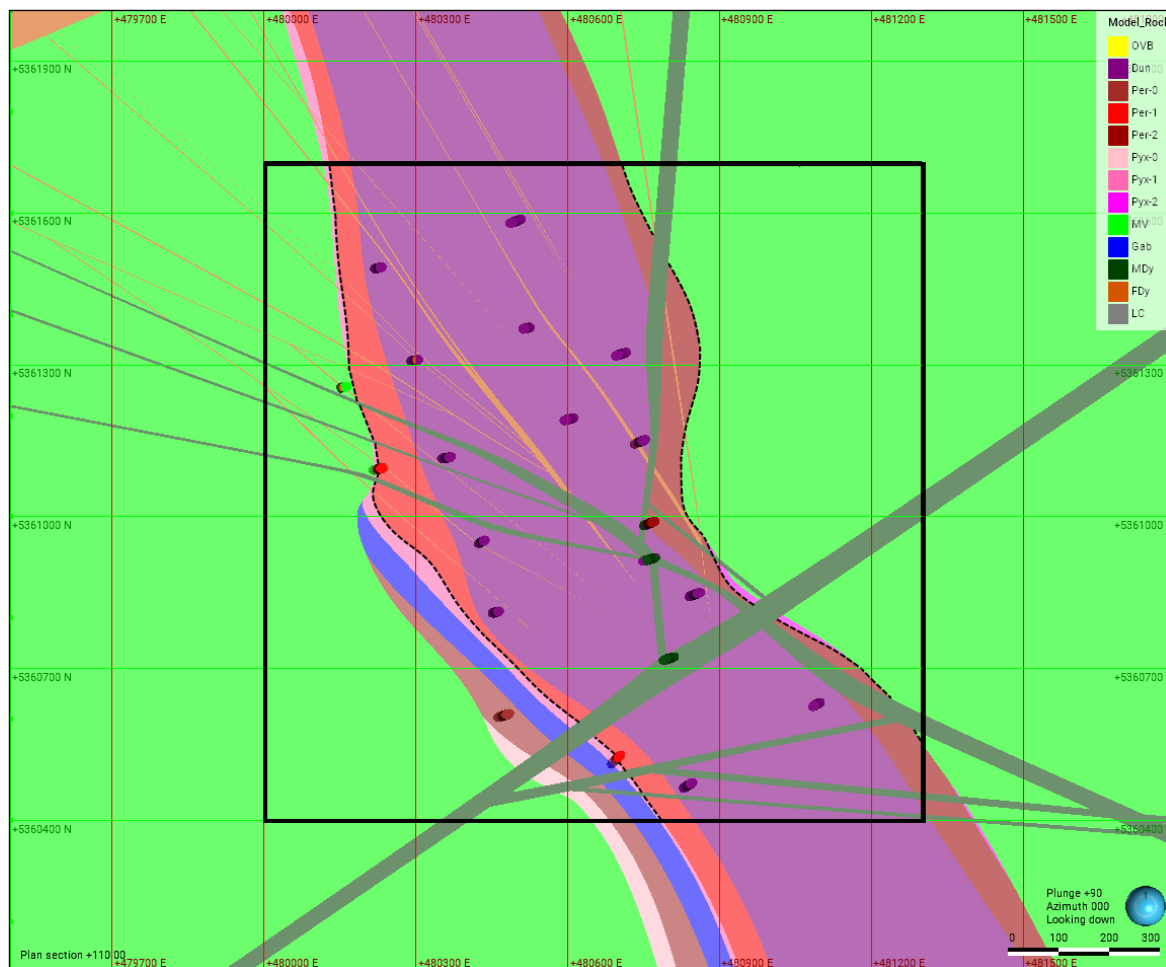
Figure 14-4. Plan section (110 m level) of the extended lithology model with CNC drill hole intercepts. The black square represents the current resource boundary and main modelling area. The mineralization envelope limit is marked with dashed lines (Caracle Creek, 2024).
