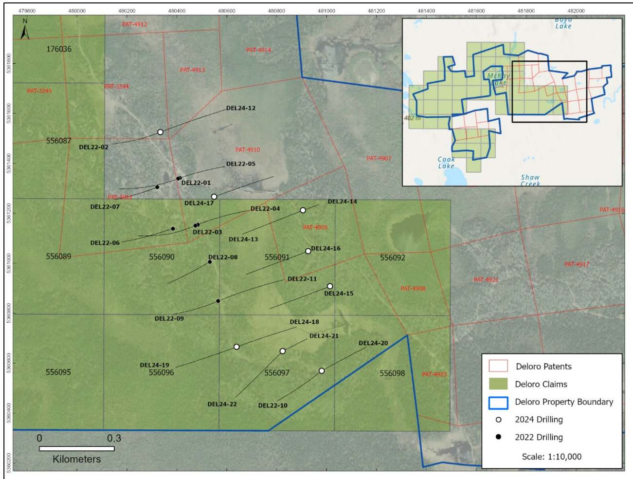
Figure 10-1. Plan view showing diamond drill hole traces from the DEL-series 2022 (11-hole) and 2024 (11-hole) diamond drilling programs, Deloro Nickel-Cobalt Sulphide Project (Canada Nickel, 2024).
