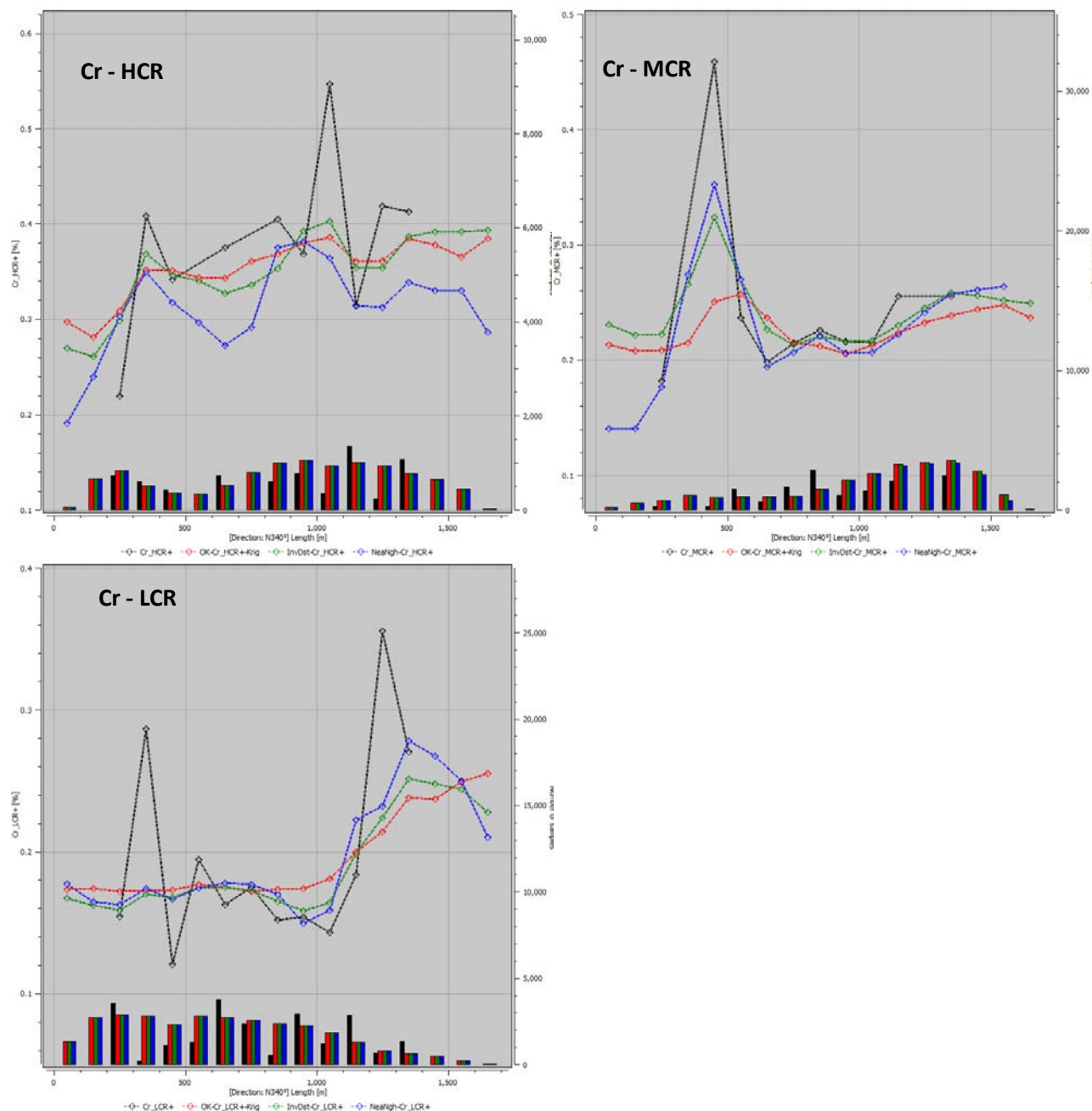
Figure 14-22. From top left to bottom: 100-m spaced Swath Plots of chromium grades within the HCR, MCR and LCR sub-domains (Caracle Creek, 2024).
