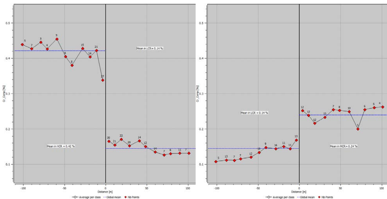
Figure 14-15. From left to right, Contact Analysis Plots of the HCR/LCR and LCR/MCR sub-domains for chromium grades (Caracle Creek, 2024).
