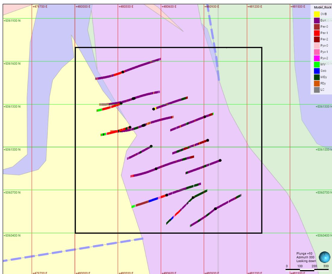
Figure 14-3. Plan view of CNC Drill holes with lithologies coded for modelling. Background geology from Ontario Geological Survey (MRD126). The black square represents the current resource boundary and main modelling area (Caracle Creek, 2024).
