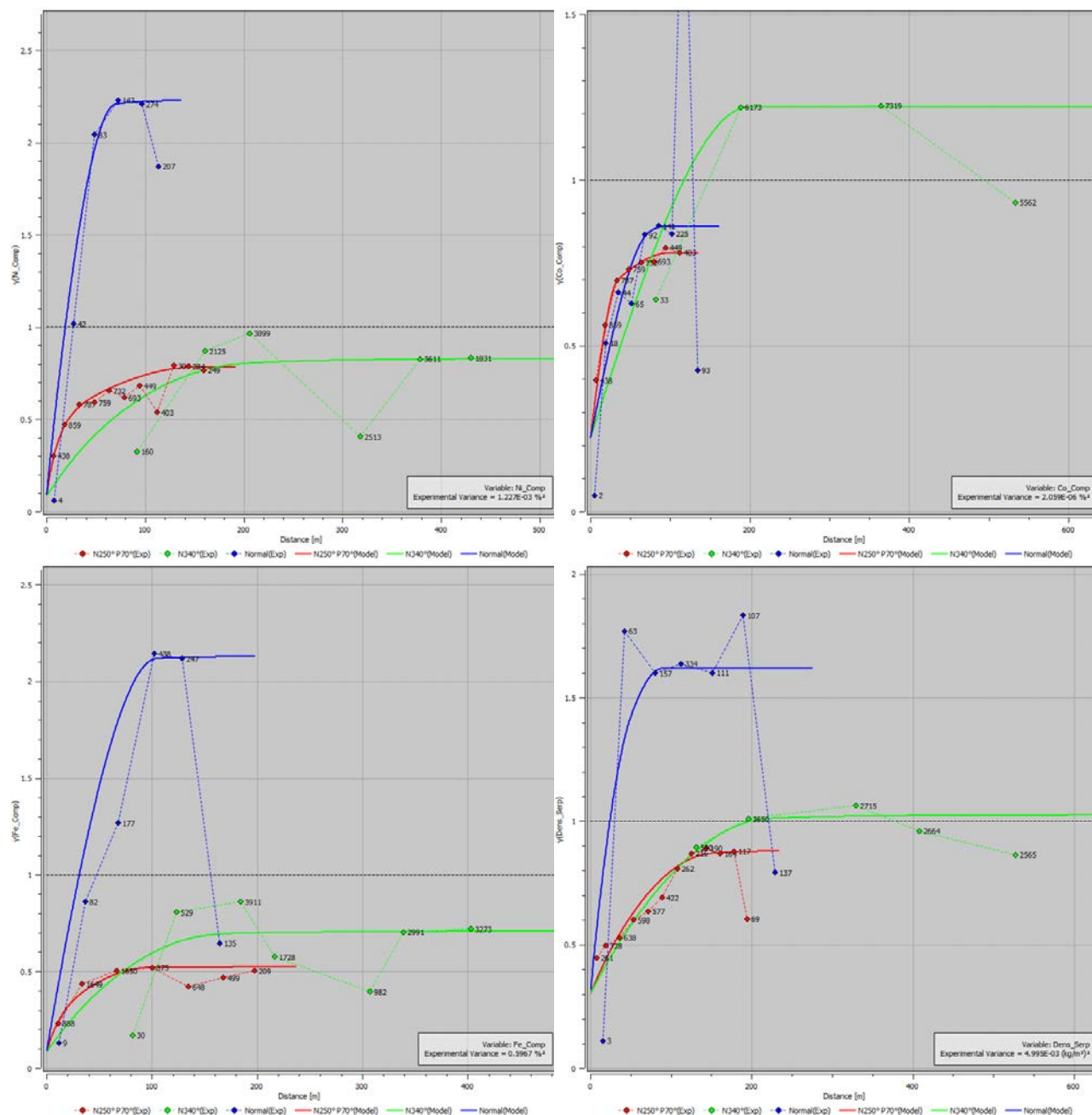
Figure 14-17. From top left to bottom right: variograms of nickel, cobalt, iron grades and density values (Caracle Creek, 2024).
