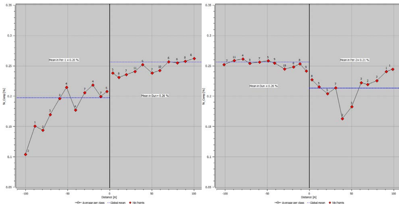
Figure 14-14. Contact Analysis Plots of the Per-1/Dun (left) and Dun/Per-2 (right) rock domains for nickel grades (Caracle Creek, 2024).
