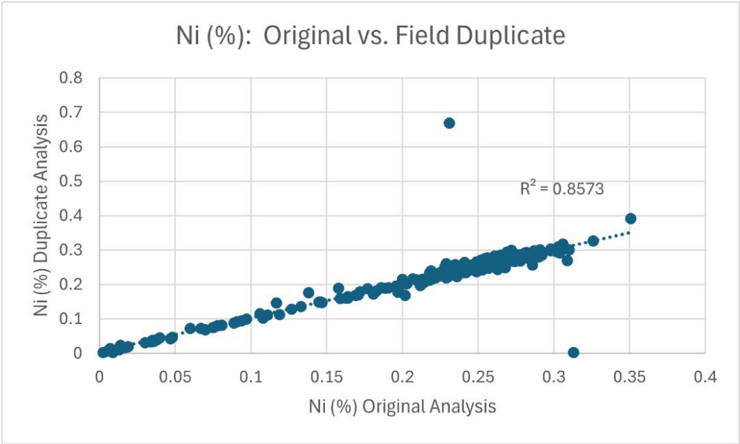
Figure 11-8. Plot of Absolute Concentrations of Pairs of Duplicate Samples Analyzed for Nickel (Ni) (Caracle Creek, 2024).
