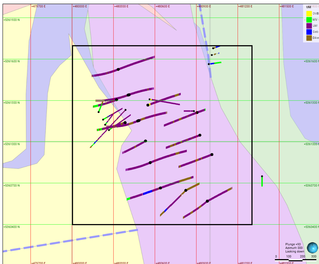
Figure 14-2. Plan view of the Deloro Project showing historical and CNC drill holes with grouped lithologies. Background geology from Ontario Geological Survey (MRD126). The ultramafic package (UM) is coloured purple both in the map and drill traces. Broader traces represent CNC holes while narrower ones are historical holes. The black square represents the current resource boundary and main modelling area (Caracle Creek, 2024).
