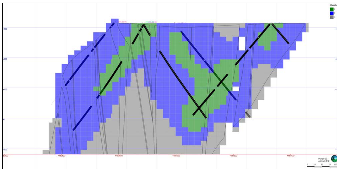
Figure 14-24. Oblique vertical section (Looking NW) of Smoothed Resource Classification against Composites within the EST Domain Envelope. Block colours represent indicated (green), inferred (blue) and potential (grey) resource classes. Some drill hole intercepts may not precisely match their corresponding feature due to section plane distance (up to 50 m). (Caracle Creek, 2024).
