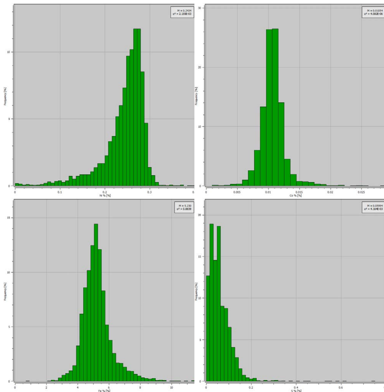
Figure 14-9. From top left to bottom right: unimodal histograms for EST Domain nickel, cobalt, iron, and sulphur grades (Caracle Creek, 2024).
