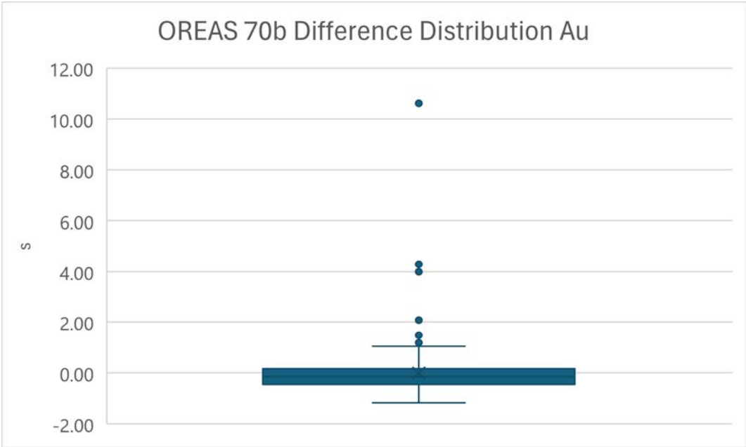
Figure 11-4. CRM OREAS 70b – Distribution of Standard Deviations Difference for Au Analysis from the Average Value (Caracle Creek, 2024).
