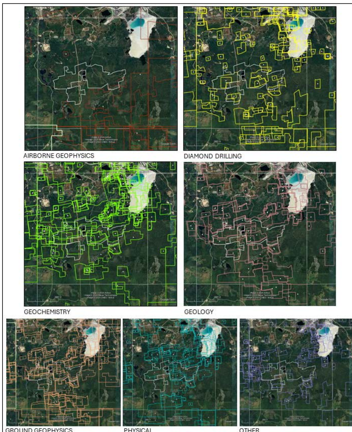
Figure 6-1. Distribution of historical assessment work types within Deloro Township, relative to the Property boundary shown in white and in central Deloro Township (Caracle Creek, 2024).
