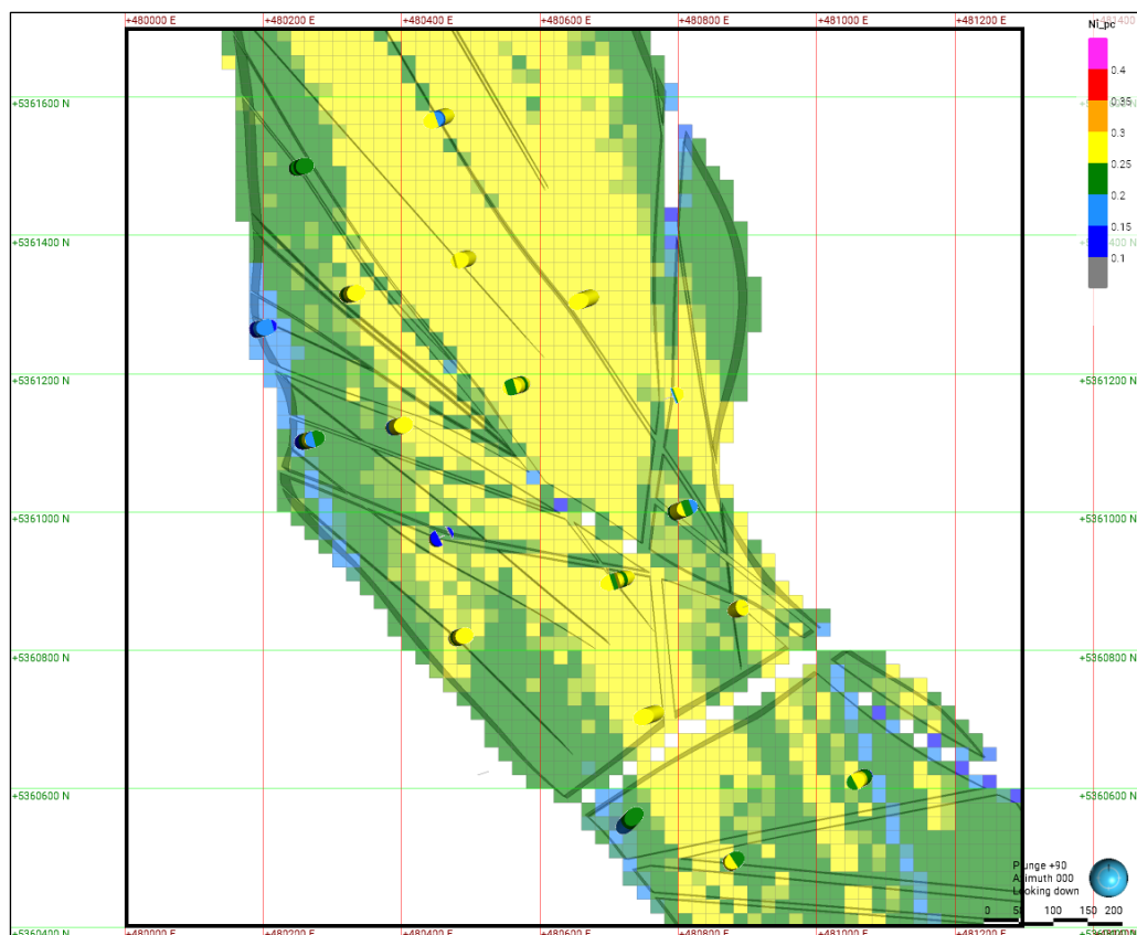
Figure 14-19. Plan Section (165 m) of Nickel Grade Blocks against Nickel Composites within the EST Domain Envelope. The black square represents the current resource boundary and main modelling area. (Caracle Creek, 2024).
