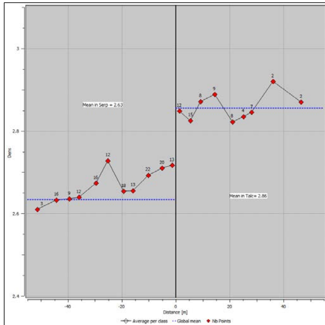
Figure 14-16. Contact Analysis Plot of the Serp/Talc alteration domains for density values (Caracle Creek, 2024).
