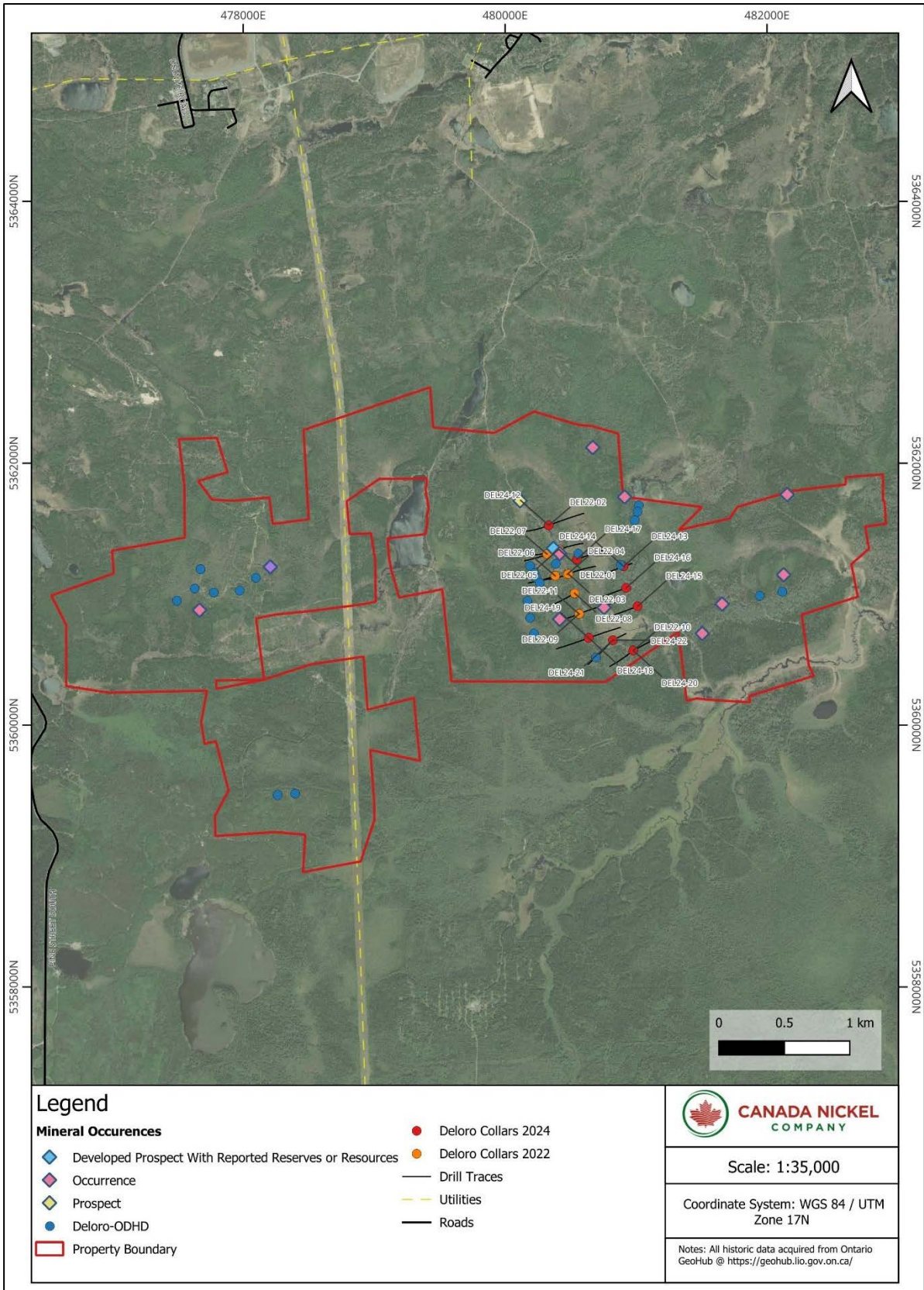
Figure 6-2. Location of historical drill holes, prospects and mineral occurrences, and collars and traces from the 2022 and 2024 drill holes completed by CNC, within the Deloro Property (see also Figure 6-3) (Canada Nickel, 2024).
