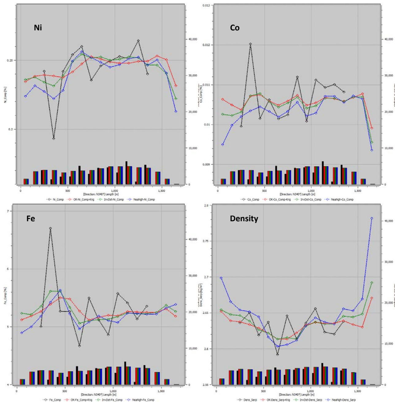
Figure 14-21. From top left to bottom right: 100-m spaced Swath Plots of nickel, cobalt, iron grades and density values (Caracle Creek, 2024).
