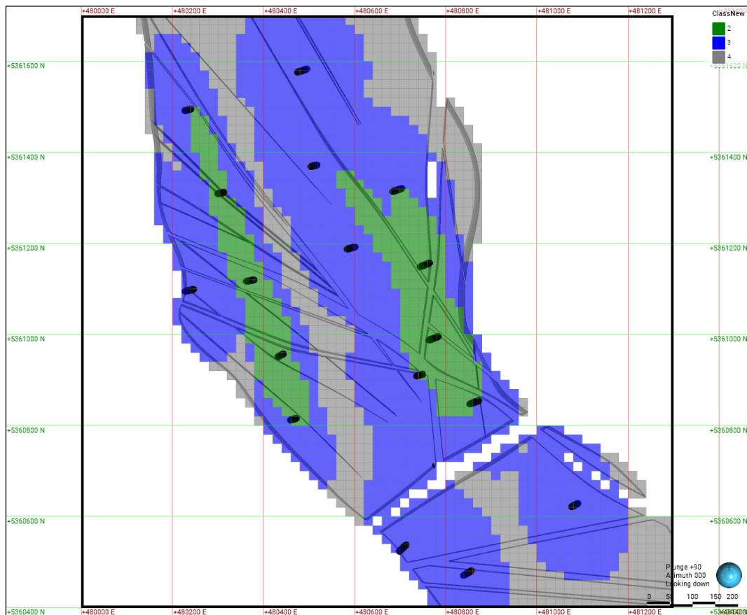
Figure 14-23. Plan section (125 m) of Smoothed Resource Classification against Composites within the EST Domain Envelope. Block colours represent indicated (green), inferred (blue) and potential (grey) resource classes. The black square represents the current resource boundary and main modelling area. (Caracle Creek, 2024).
