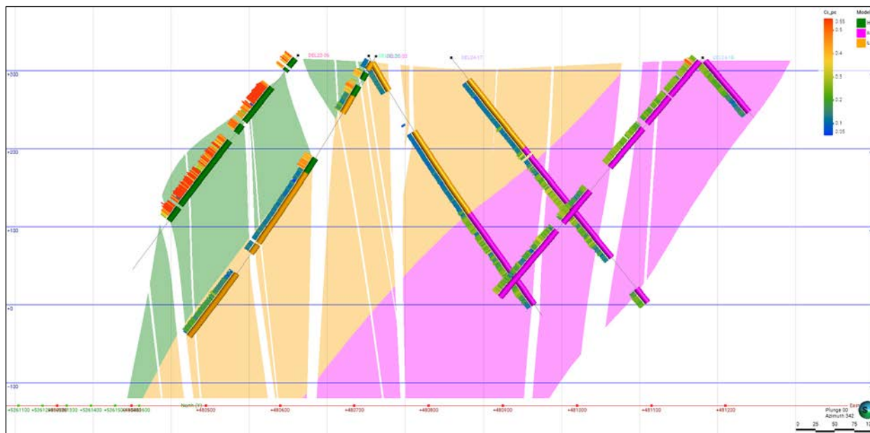
Figure 14-12. Oblique vertical section (Looking NW) of the HCR/LCR/MCR Estimation Sub-Domains with CNC drill hole Intercepts and chromium grades. Background outline and drill trace colours represent HCR (green), MCR (pink) and LCR (orange) estimation sub-domains. Some drill hole intercepts may not precisely match their corresponding feature due to section plane distance (up to 50 m) (Caracle Creek, 2024).
