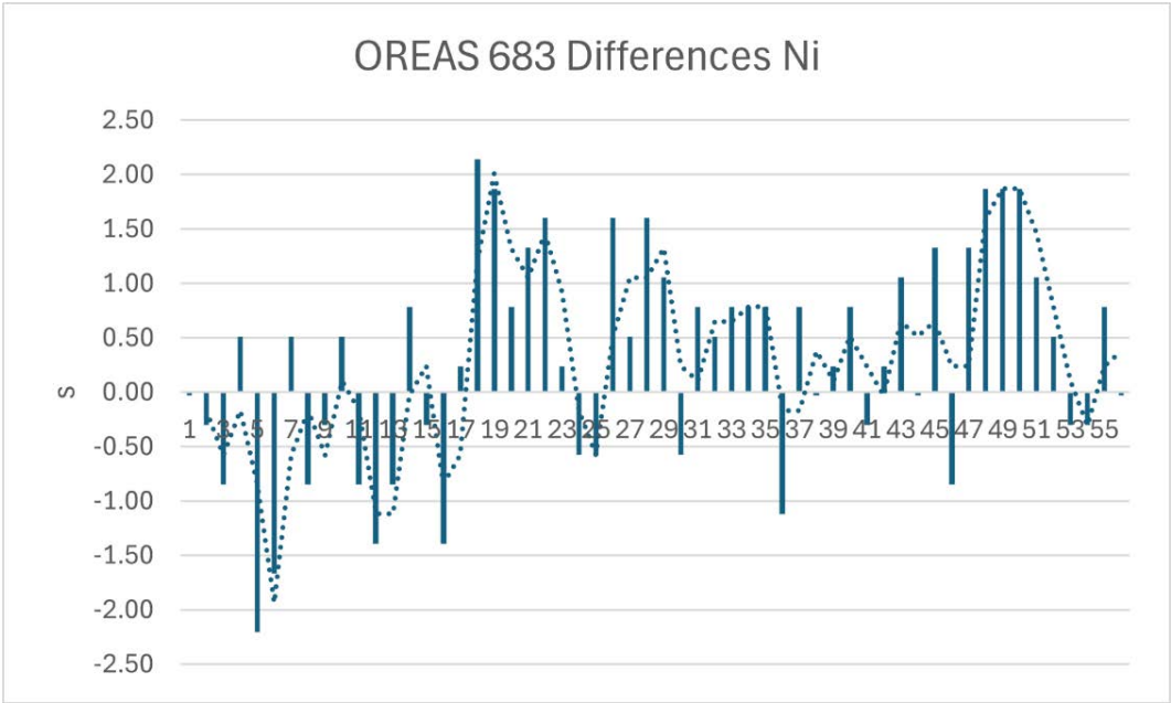
Figure 11-5. CRM OREAS 683 – Number of Standard Deviations Difference for Ni Analysis from the Average Value for Various Analytical Runs (Caracle Creek, 2024).
