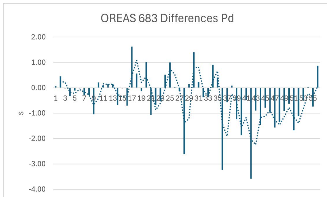
Figure 11-7. CRM OREAS 683 – Number of Standard Deviations Difference for Pd Analysis from the Certified Value for Various Analytical Runs (Caracle Creek, 2024).
