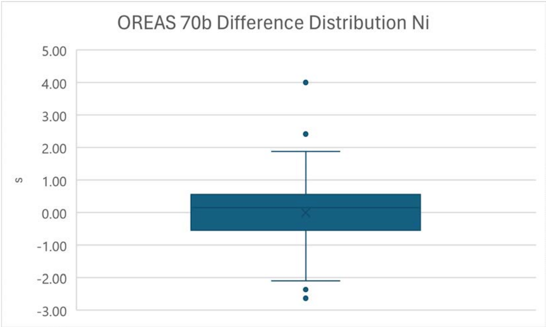
Figure 11-2. CRM OREAS 70b – Distribution of Standard Deviations Difference for Ni Analysis from the Average Value (Caracle Creek, 2024).
