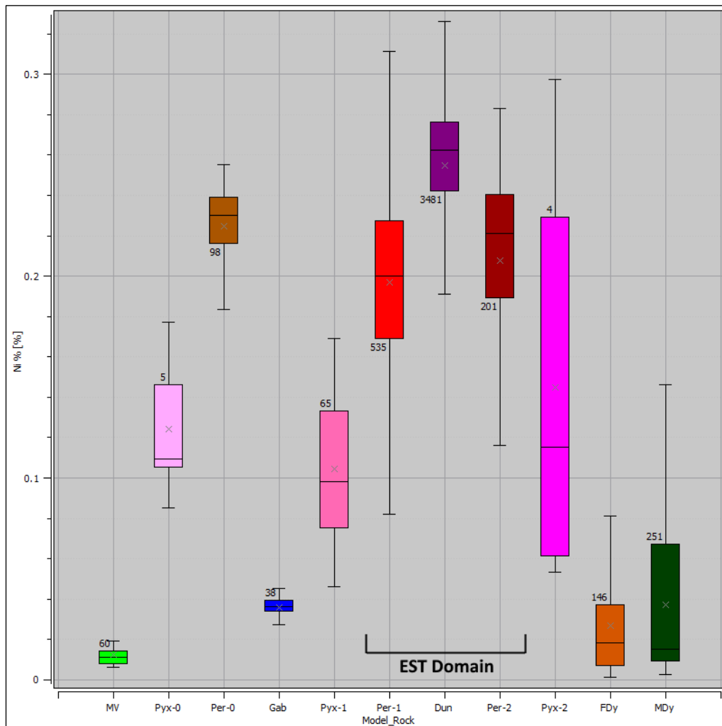
Figure 14-8. Nickel grade boxplot according to model lithologies (Caracle Creek, 2024).
