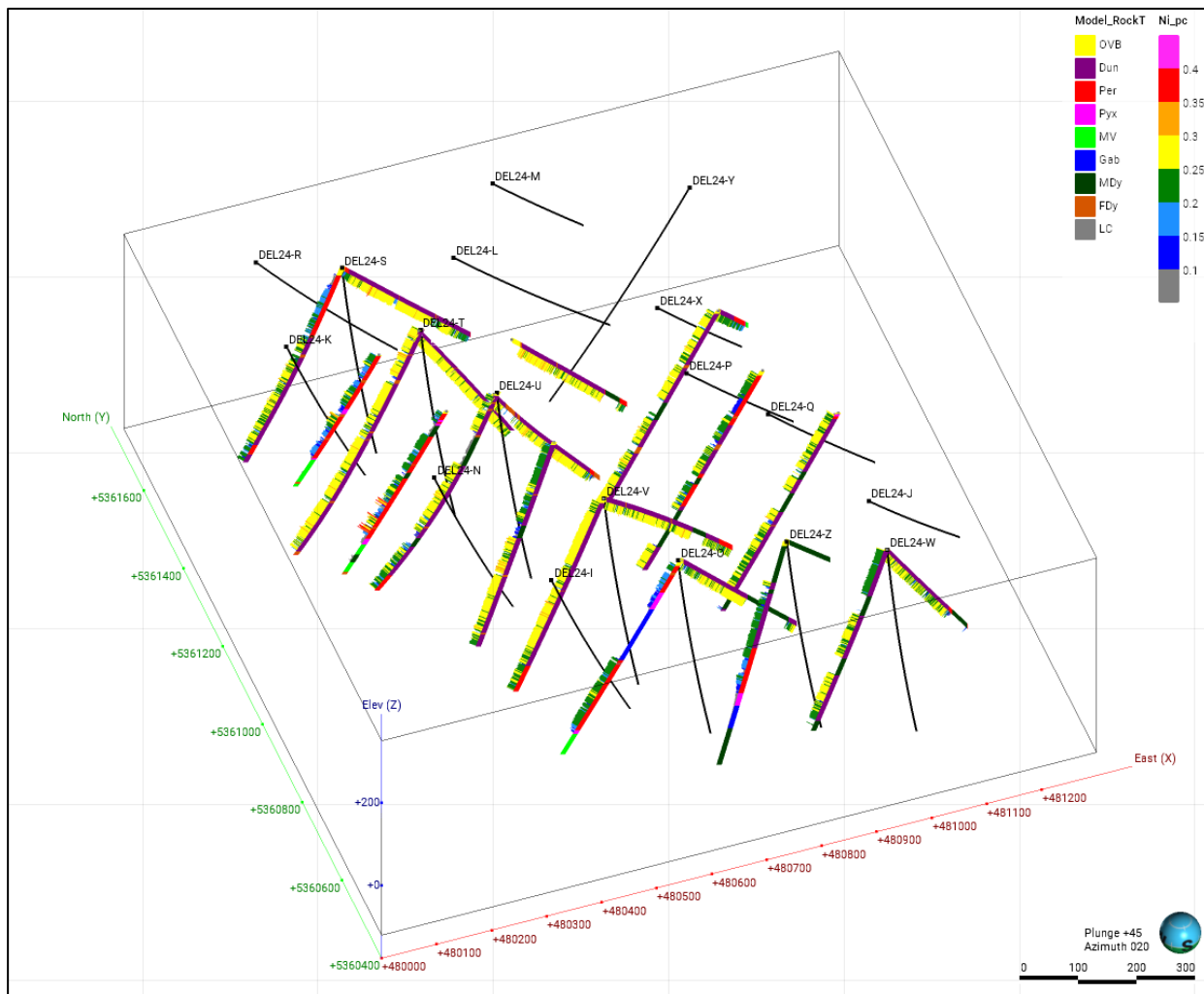
Figure 26-1. Isometric view of the 18 proposed diamond drill holes (black collars and traces) and unlabelled drill holes (with Ni% and lithologies plotted) used in the current MRE, Deloro Project (Caracle Creek, 2024).
