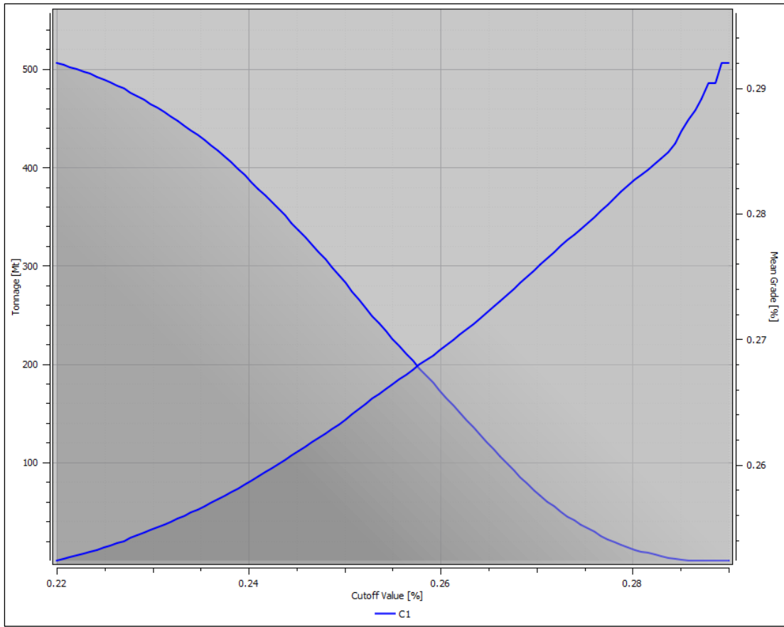
Figure 14-26. Grade-Tonnage Curve for nickel grades (Caracle Creek, 2024).
