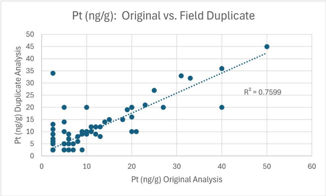
Figure 11-12. Plot of Absolute Concentrations of Pairs of Duplicate Samples Analyzed for Platinum (Pt) (Caracle Creek, 2024).
