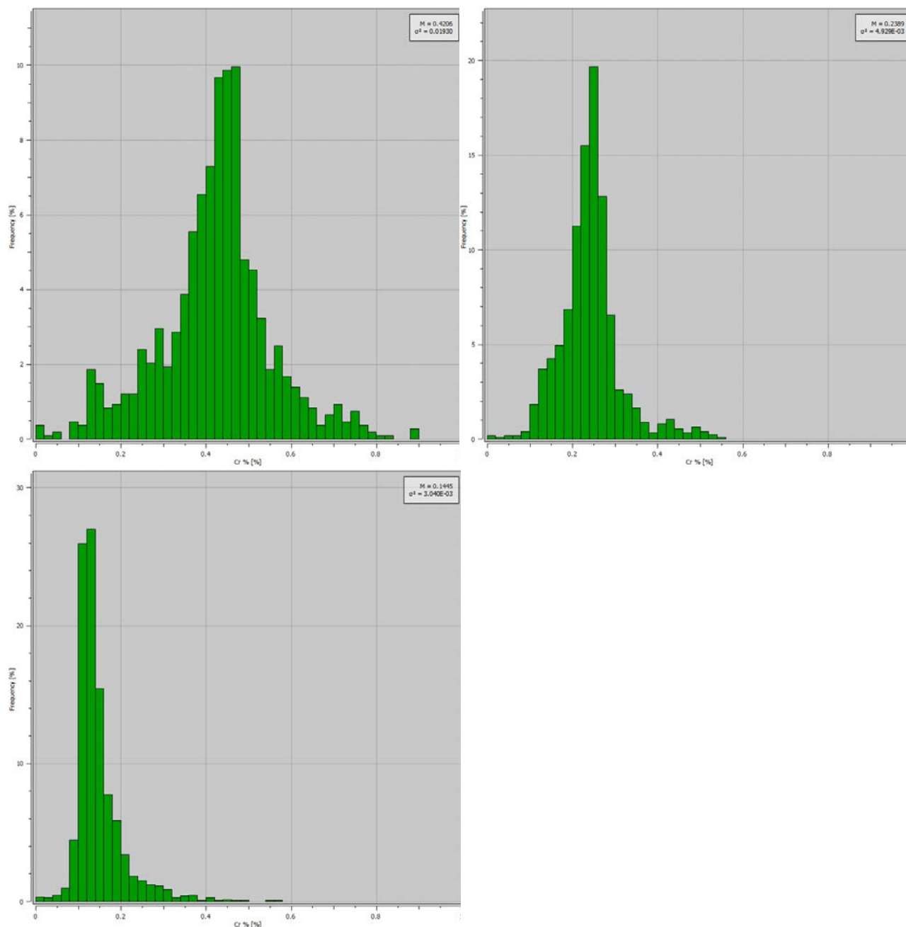
Figure 14-13. From top left to bottom: chromium grade histograms for the HCR, MCR, and LCR estimation sub-domains (Caracle Creek, 2024).
