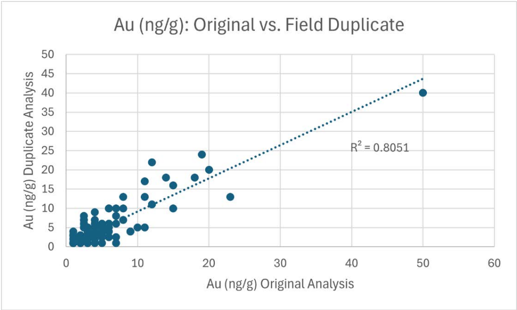
Figure 11-11. Plot of Absolute Concentrations of Pairs of Duplicate Samples Analyzed for Gold (Au) (Caracle Creek, 2024).
