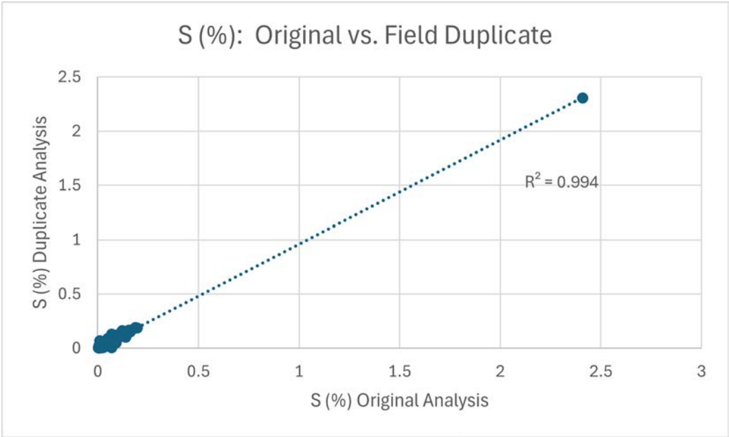
Figure 11-10. Plot of Absolute Concentrations of Pairs of Duplicate Samples Analyzed for Sulphur (S) (Caracle Creek, 2024).
