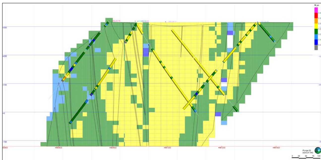
Figure 14-20. Oblique vertical section (Looking NW) of Nickel Grade Blocks against Nickel Composites within the EST Domain Envelope. Some drill hole intercepts may not precisely match their corresponding feature due to section plane distance (up to 50 m) (Caracle Creek, 2024).
