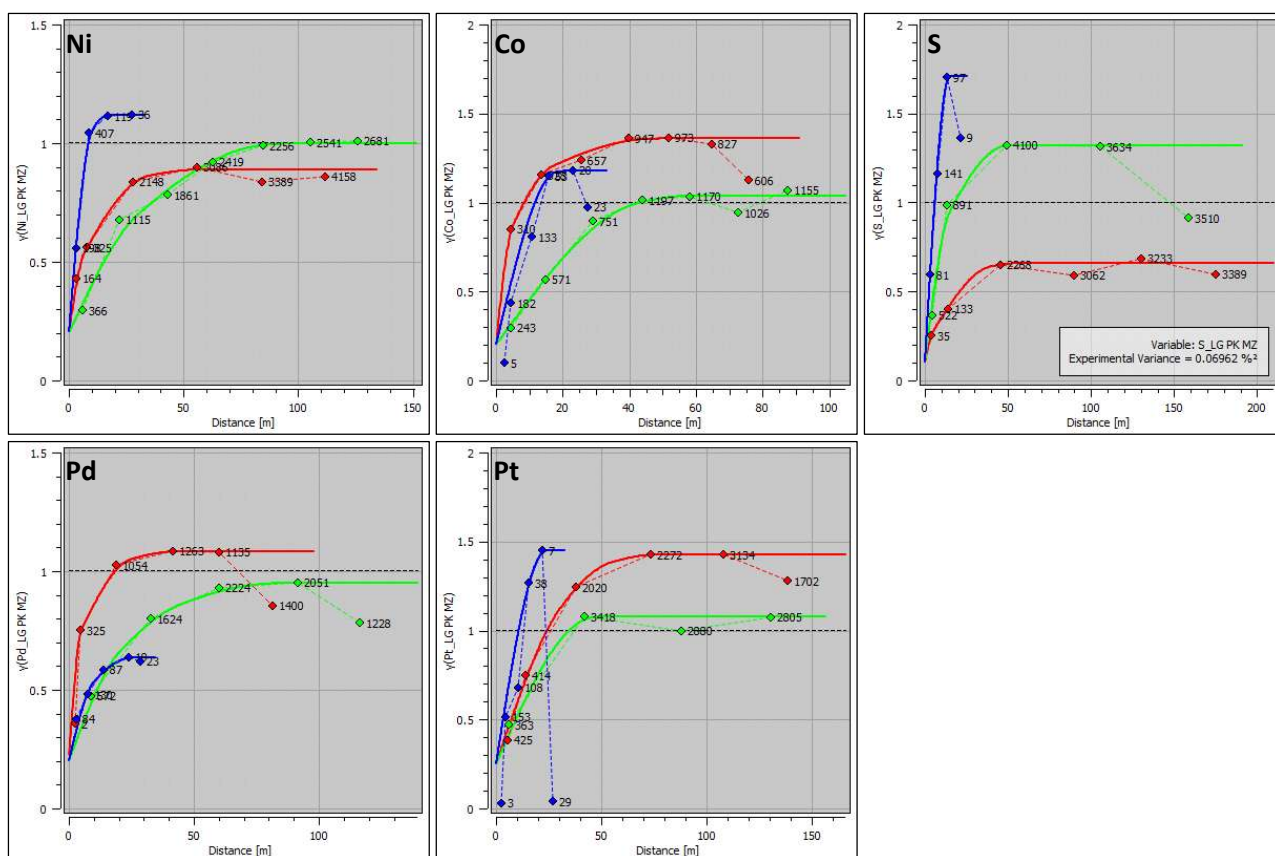
Figure 14-28. Variography for the LG domain in the Main Zone (Caracle Creek, 2025).
