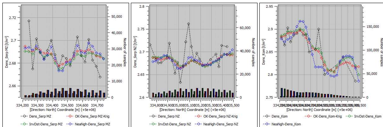
Figure 14-41. Density swath plots for the Serp domain in the Main (left) and North (centre) zones, and the Kom Domain (right) (Caracle Creek, 2025).
