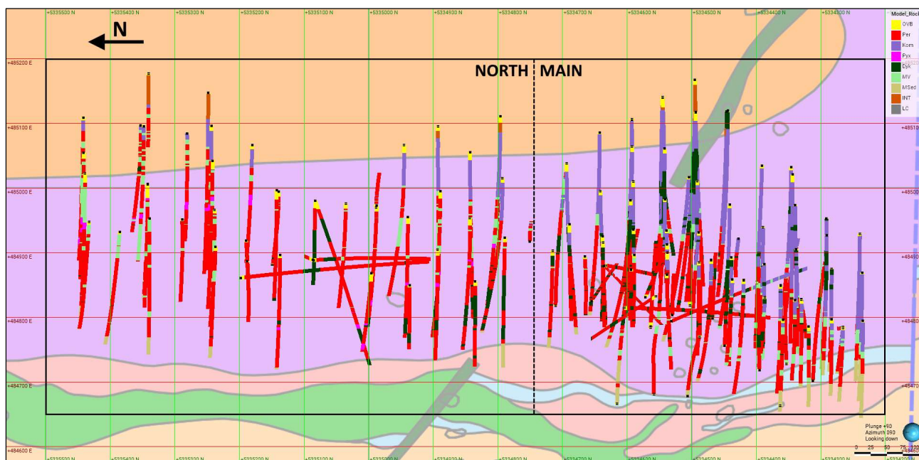
Figure 14-4. Plan view (North to the left) of the Texmont Project with drill hole intervals showing the final lithology codes for modelling. Background lithology from OGS (Houlé et al. , 2009). The black rectangle represents the current resource boundary and main modelling area (Caracle Creek, 2025).
