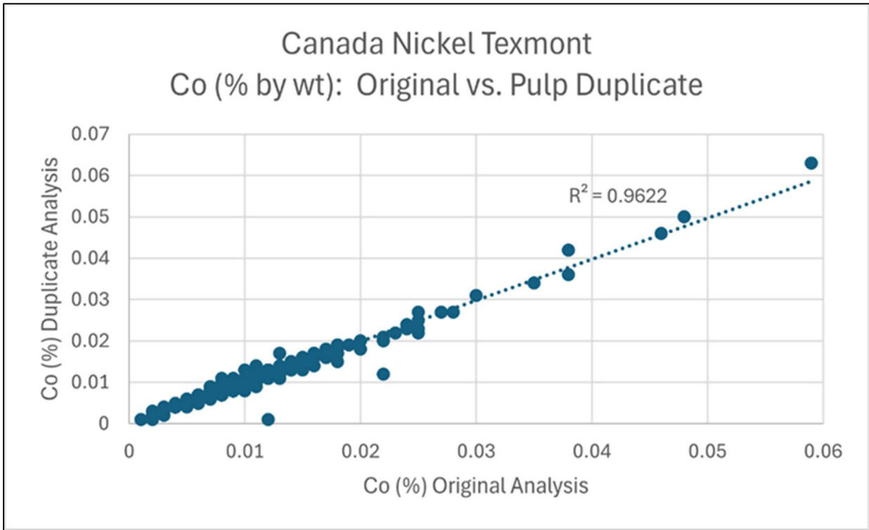
Figure 11-10: Plot of Absolute Concentrations of Pairs of Duplicate Samples Analyzed for Co (Siriunas, 2025).
