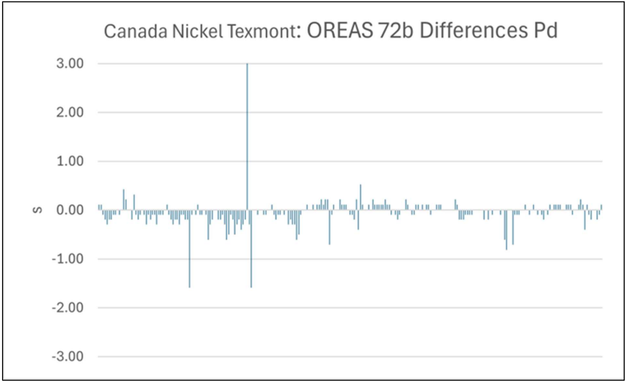
Figure 11-8. Canada Nickel Texmont CRM OREAS 72b – Number of Standard Deviations Difference for Pd Analysis from the Average Value for Various Analytical Runs (Siriunas, 2025).
