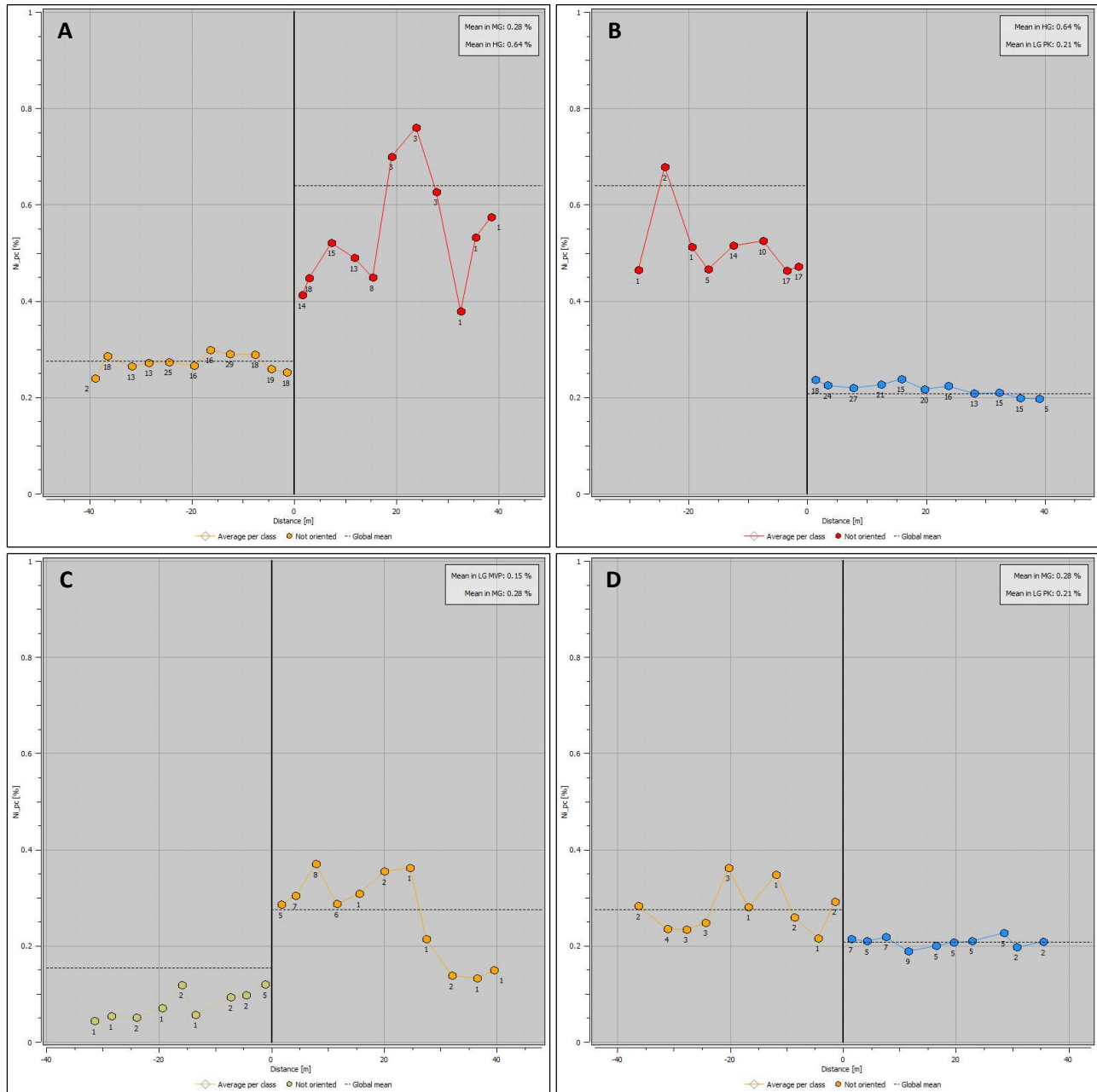
Figure 14-23. Contact analysis plots of nickel composites between North Zone domains: A) MG/HG, B) HG/LG PK, C) LG MVP/MG and D) MG/LG PK (Caracle Creek, 2025).
