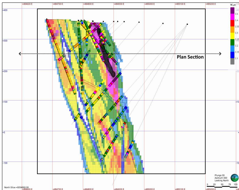
Figure 14-36. Vertical section 5334550 mN (Looking North) of the Texmont Deposit nickel grade blocks against composites within the PER domain in the Main Zone. Some intervals may not precisely match their corresponding feature due to the 50 m section width. The former Texmont Mine underground workings are represented by the dark envelope. The dashed line is the trace of the plan section presented in Figure 14-35 (Caracle Creek, 2025).
