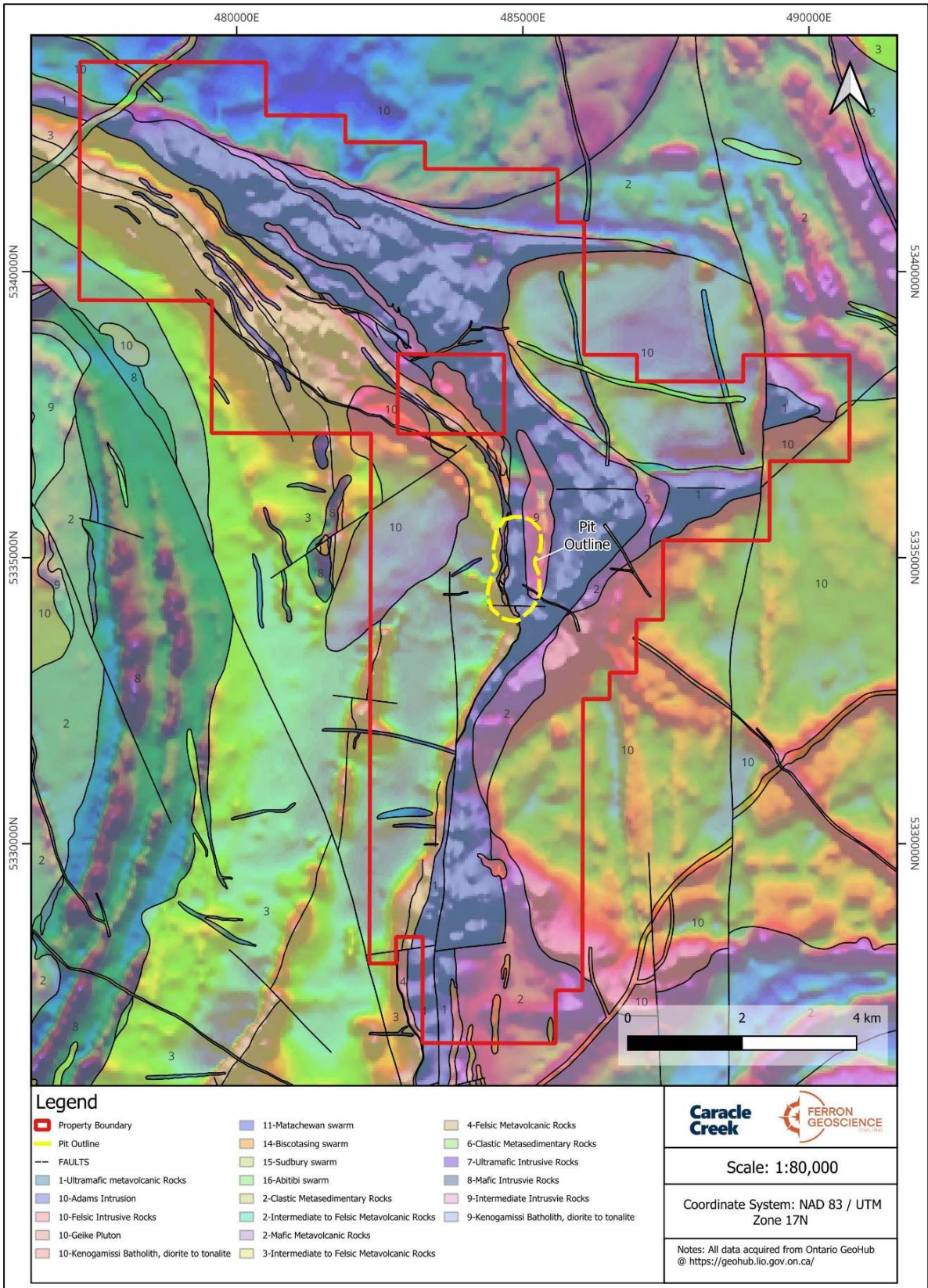
Figure 7-2. Total Magnetic Intensity (TMI) map of the TUC and the Texmont Project showing the location of the Texmont pit outline (yellow dashed outline) with overlain geological map from the 2019 Ontario Geological Survey field mapping of the Bartlett and Halliday Domes (Prefontaine et al. , 2019) (Caracle Creek, 2025).
