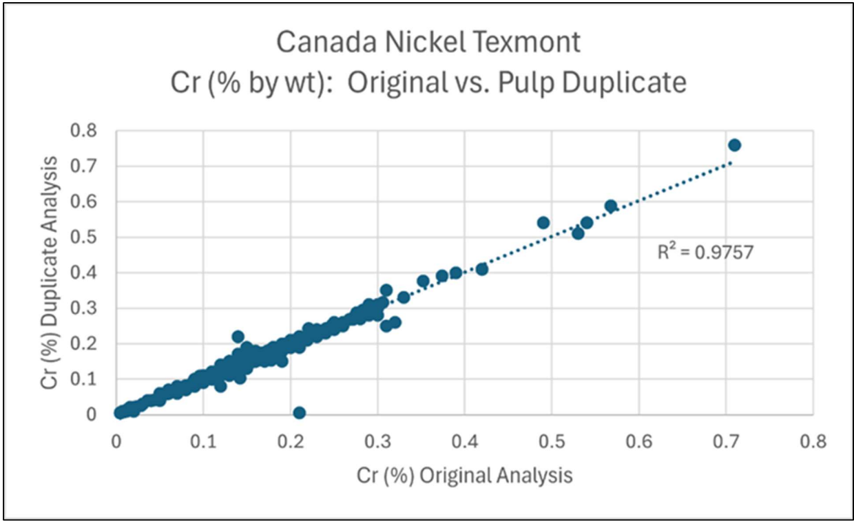
Figure 11-15. Plot of Absolute Concentrations (capped) of Pairs of Duplicate Samples Analyzed for Cr (Siriunas, 2025).
