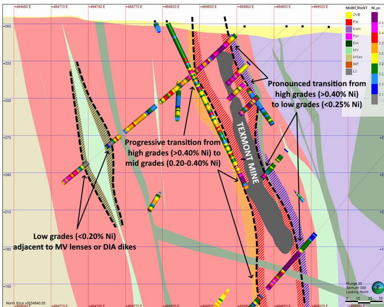
Figure 14-16. Vertical section 5334540 mN (close-up, Looking North) of the Texmont Deposit subdomaining criteria for grade estimation in the Main Zone (also applicable to the North Zone), with nickel grade intervals and the lithology model for context. Coloured hash marks delineate the inner side of the defined estimation domains: HG (red), MG (orange), LG PK (blue) and LG DYK (green), the remaining LG MVP domain not depicted. The former Texmont Mine underground workings are represented by the dark envelope, matching the high-grade (HG) domain (Caracle Creek, 2025).
