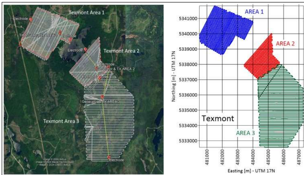
Figure 9-2. Semi-Airborne UAV EM-Mag flight lines (MGT, 2024).
