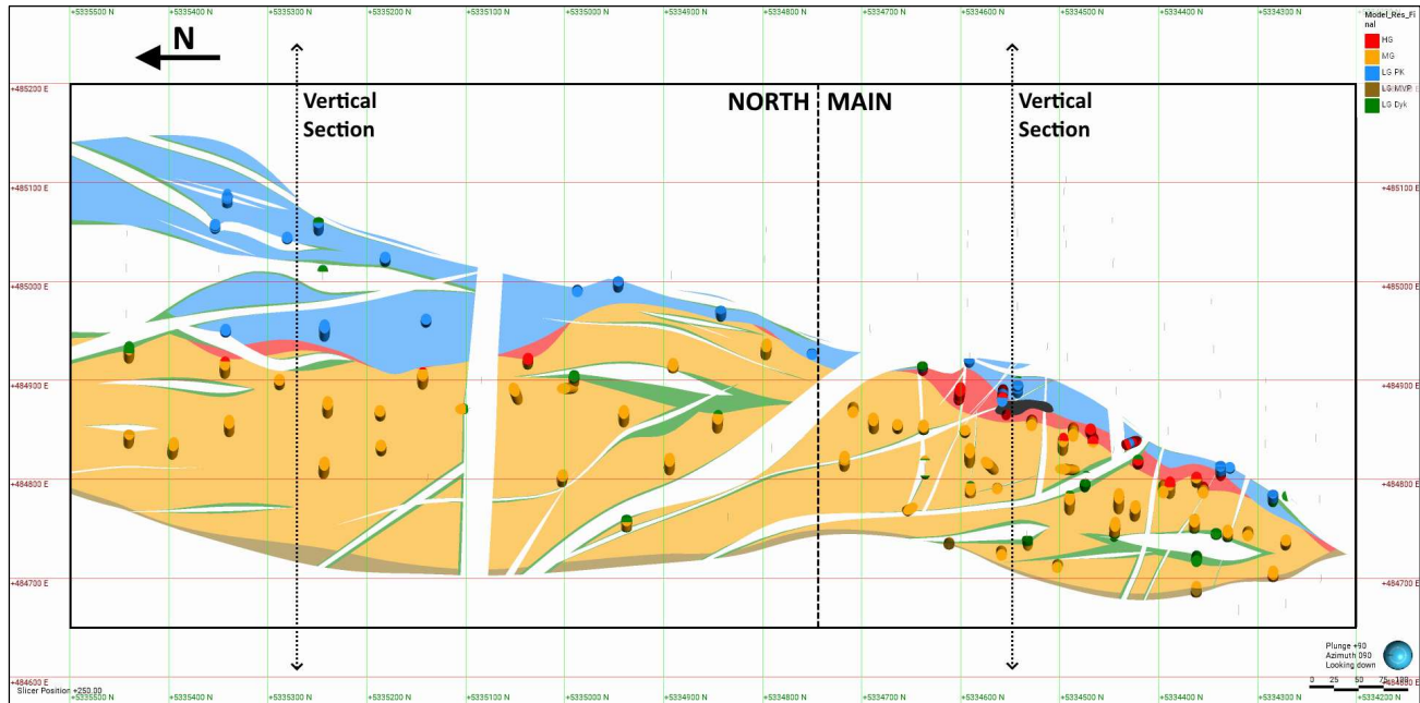
Figure 14-19. Plan section (250 RL) of the Texmont Deposit estimation domains and coded drill hole intervals: LG PK domain ( <0.25\% Ni) in blue, HG domain ( >0.40\% Ni) in red, MG domain ( 0.20\text{--}0.40\% Ni) in orange, LG DYK and LG MVP domains ( <0.20\% Ni) in green and brown respectively. The former Texmont Mine underground workings are represented by the dark spot in the Main Zone. The dashed lines are traces of the vertical sections presented in Figures 14-20 and 14-21 (Caracle Creek, 2025).
