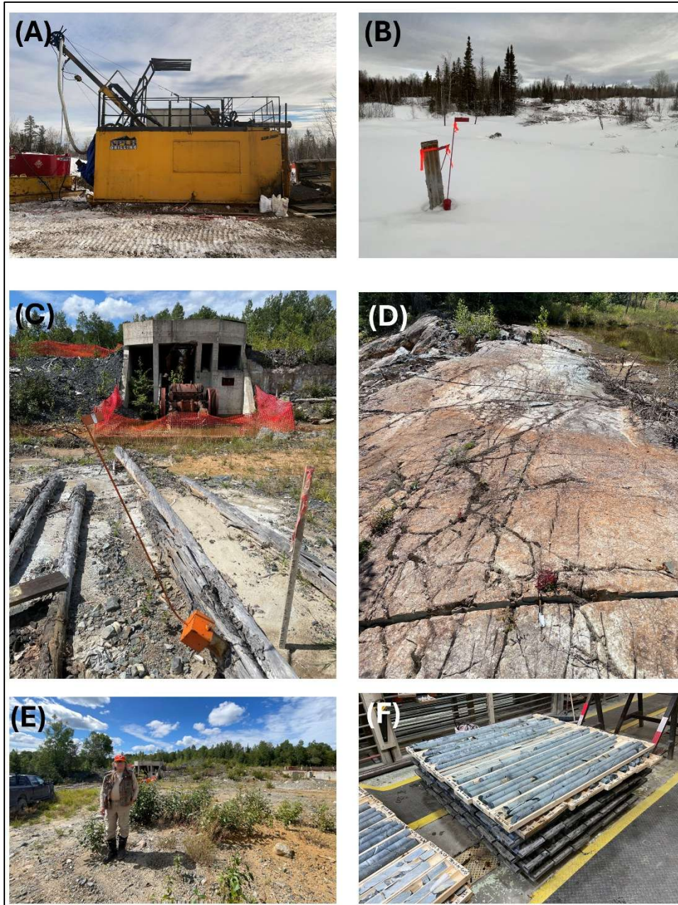
Figure 2-3. Selection of photos taking during the Personal Inspection of the Property by QP John Siriunas, 14 February 2023 and 18 August 2025. (A) Drilling rig of contract drilling company NPLH Drilling on-site at the Texmont Property (2023); (B) Historical drill casings flagged in the field (2023); (C) Drill casing for hole TXT24-64 flagged in the field near the historical mine workings (2025); (D) Area of 2023 channel sampling (picture taken in 2025); (E) Author in the vicinity of the historical mine workings (2025); (F) Historical core from Fletcher Nickel Inc. drilling ca. 2007 in the process of being transferred to new core boxes for re-logging and archival purposes (2023) (Siriunas, 2023 and 2025).
