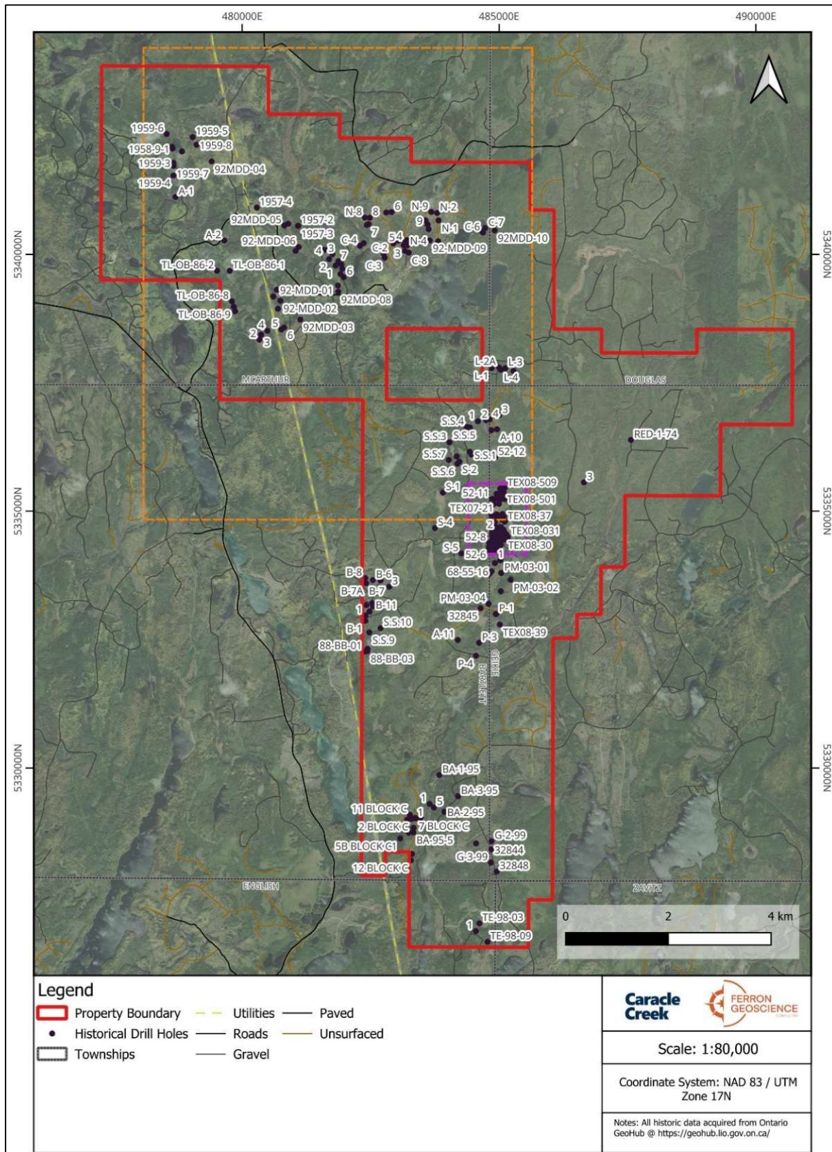
Figure 6-1. Historical diamond drillholes on the Property. Locations of inset maps for Figure 6-2 (purple) and Figure 6-3 (orange) are shown (Caracle Creek, 2025).
