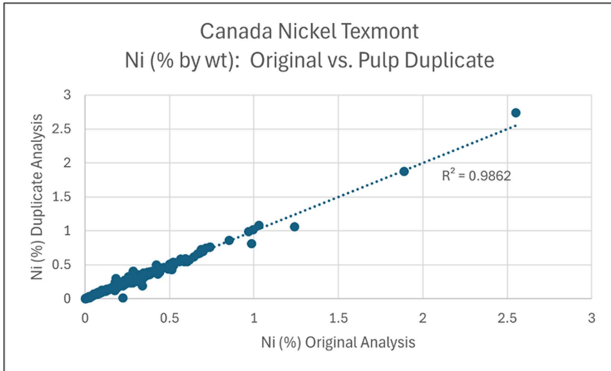
Figure 11-9. Plot of Absolute Concentrations of Pairs of Duplicate Samples Analyzed for Ni (Siriunas, 2025).
