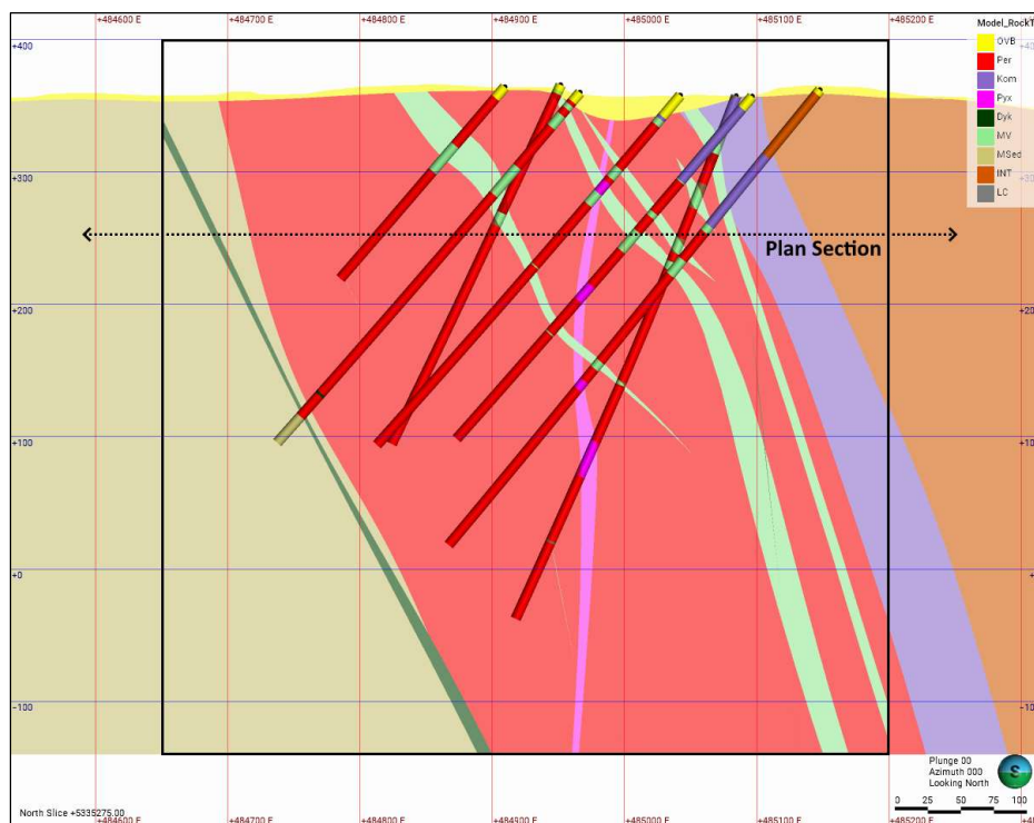
Figure 14-7. Vertical section 5335275 mN (Looking North) of the Texmont lithology model and coded drill hole intervals in the North Zone. Some intervals may not precisely match their corresponding feature due to the 80 m section width. The black outline represents the current resource boundary and main modelling area, and the dashed line is the trace of the plan section presented in Figure 14-5 (Caracle Creek, 2025).
