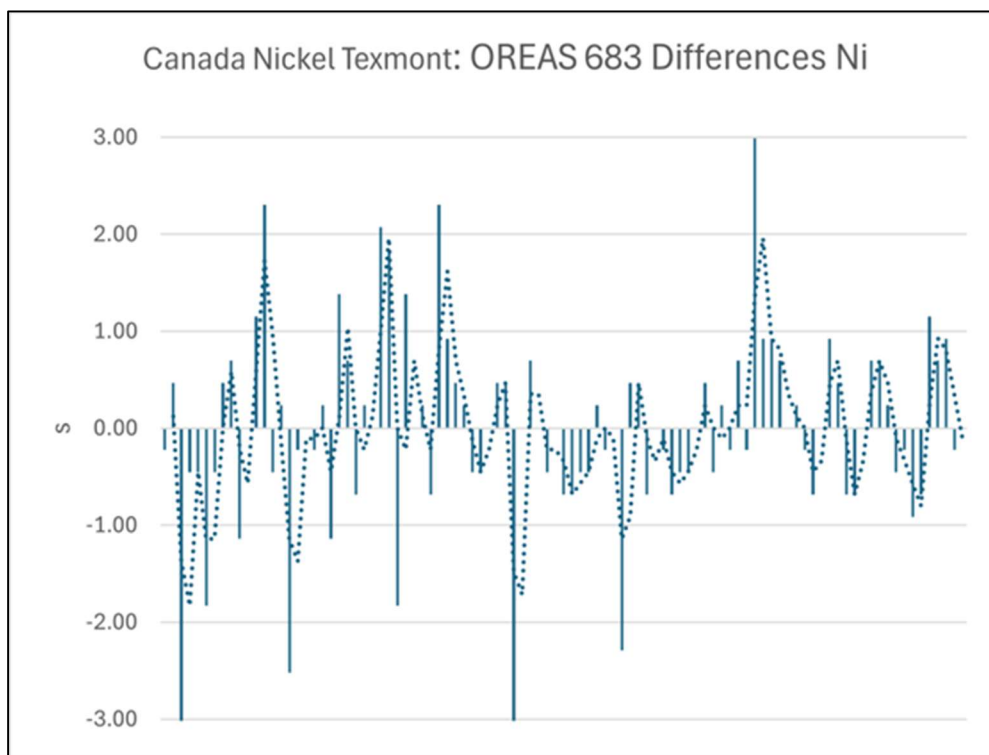
Figure 11-4. Canada Nickel Texmont CRM OREAS 683 – Distribution of Standard Deviations Difference for Ni Analysis from the Average Value for Various Analytical Runs (Siriunas, 2025).
