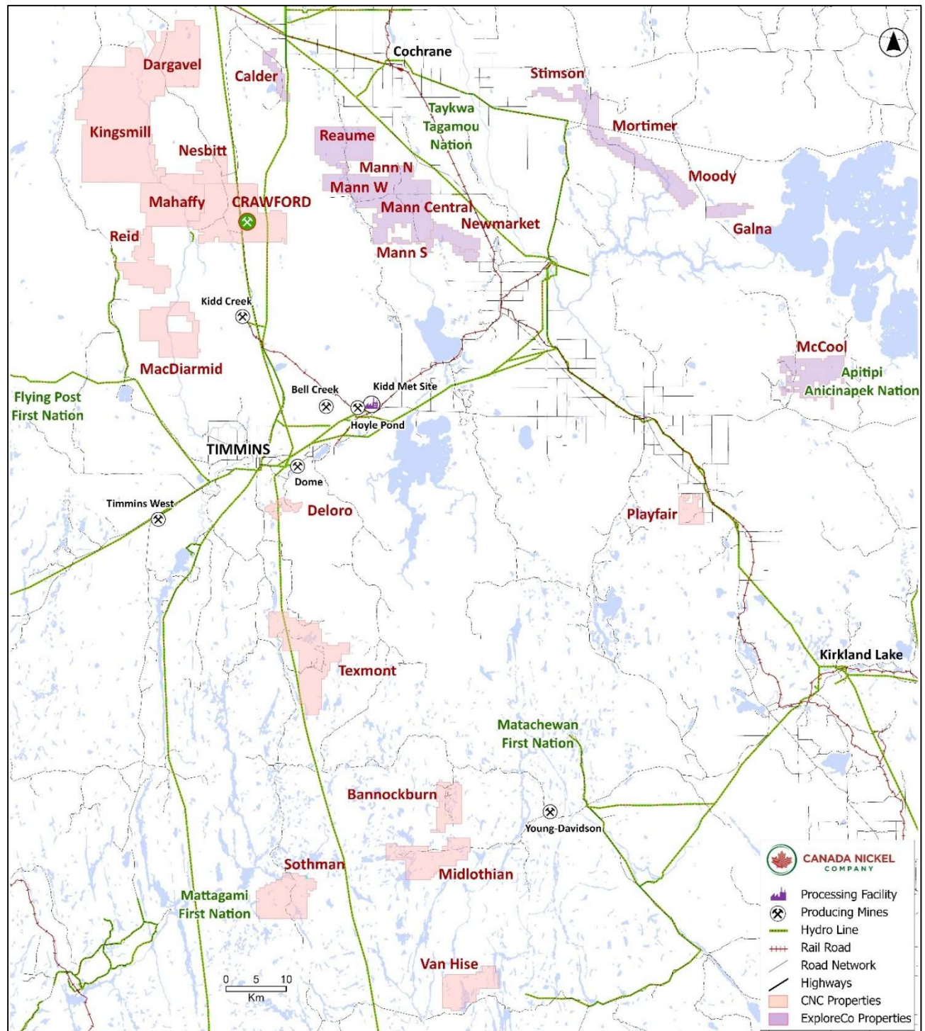
Figure 2-2. Location of the Texmont Project and other Canada Nickel projects and properties within the Timmins Nickel District (Canada Nickel, 2025).
