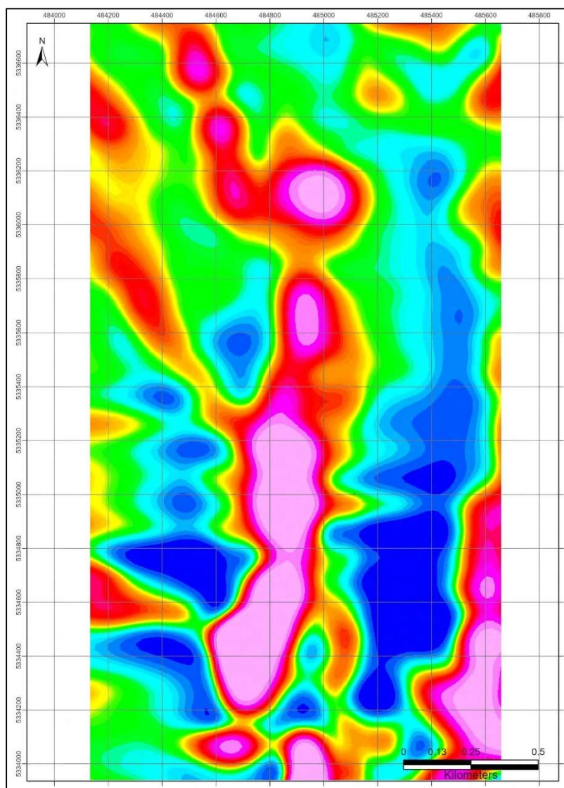
Figure 9-1. First vertical derivative of the Total Magnetic Intensity (BECI, 2022).
