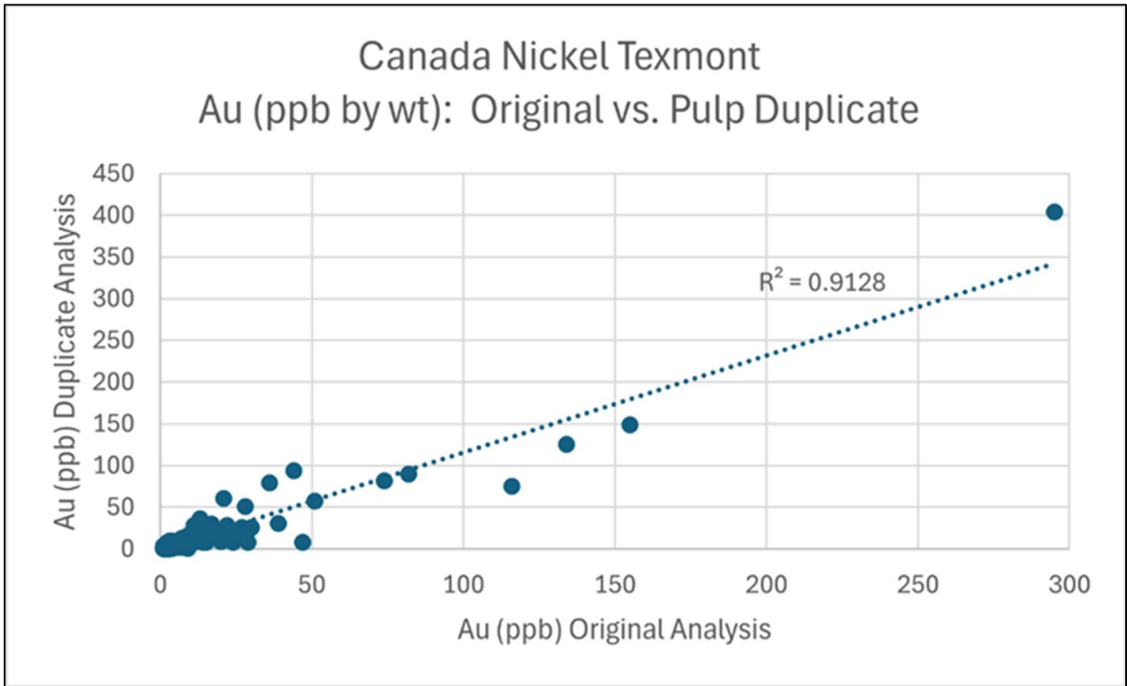
Figure 11-12: Plot of Absolute Concentrations (capped) of Pairs of Duplicate Samples Analyzed for Au (Siriunas, 2025).
