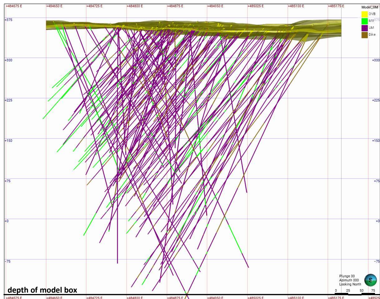
Figure 14-2. Longitudinal view (looking North) of the Texmont Project with the overburden volume (transparent yellow) and MRE drill holes showing the main rock types, including the UM package coloured purple (Caracle Creek, 2025).
