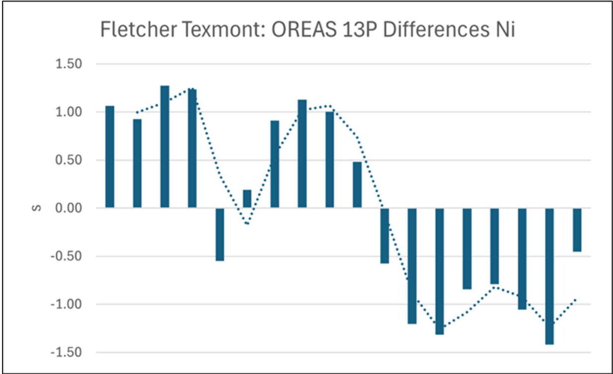
Figure 11-1. Fletcher Texmont CRM OREAS 13P – Number of Standard Deviations Difference for Ni Analysis from the Average Value for Various Analytical Runs (Siriunas, 2025).
