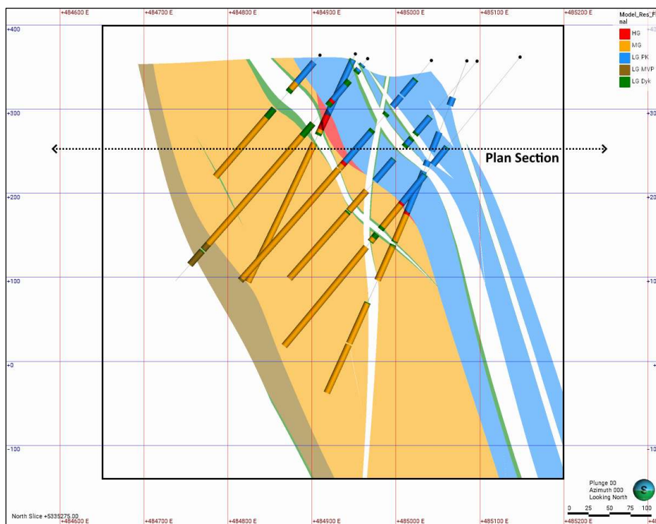
Figure 14-21. Vertical section 5335275 mN (Looking North) of the Texmont Deposit estimation domains and coded drill hole intervals in the North Zone. Some intervals may not precisely match their corresponding feature due to the 80 m section width. The dashed line is the trace of the plan section presented in Figure 14-19 (Caracle Creek, 2025).
