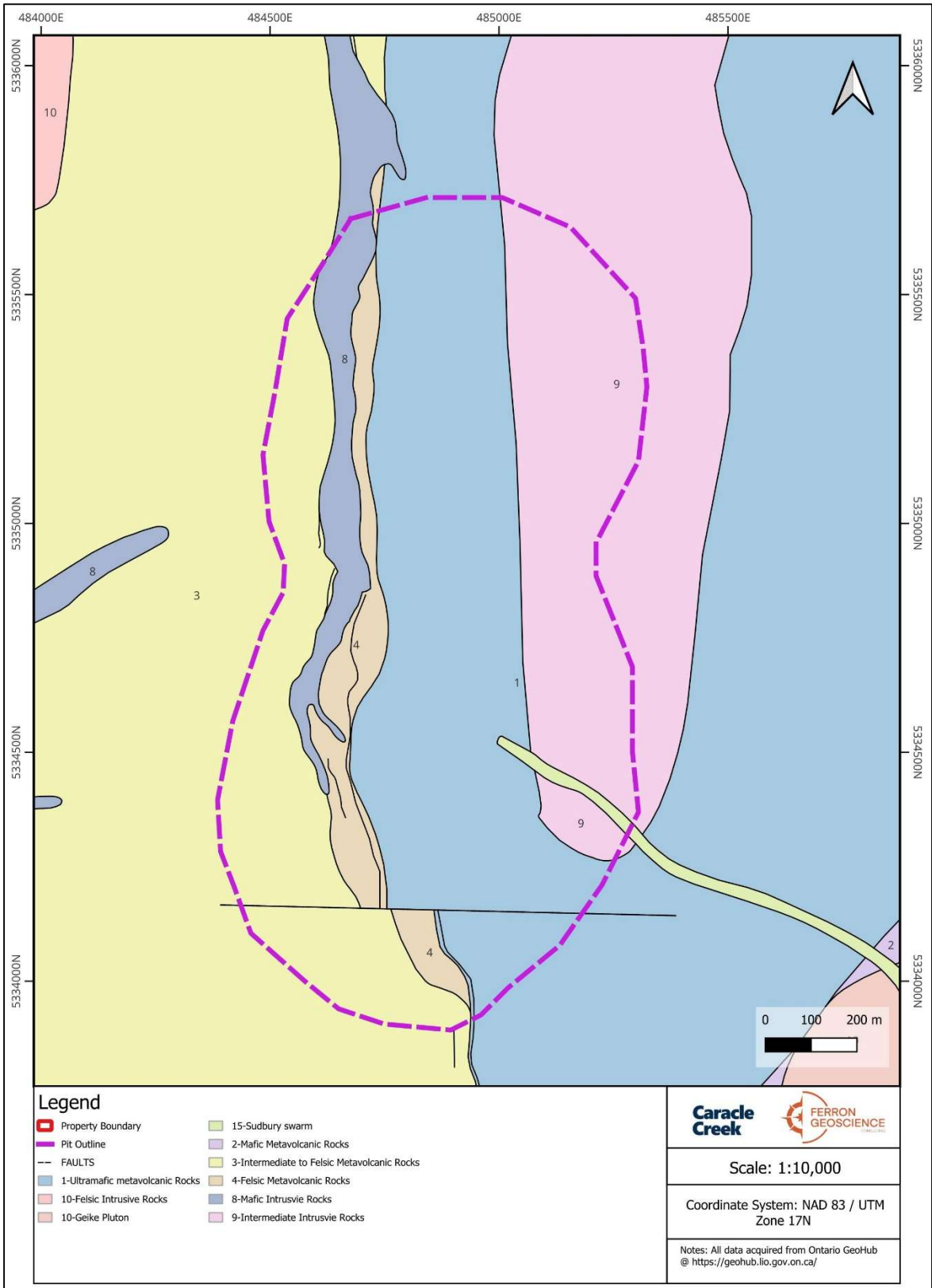
Figure 7-3. Geological map (OGS, 2019) of the Texmont Project showing the optimized pit outline (purple dashed line) (Caracle Creek, 2025).
