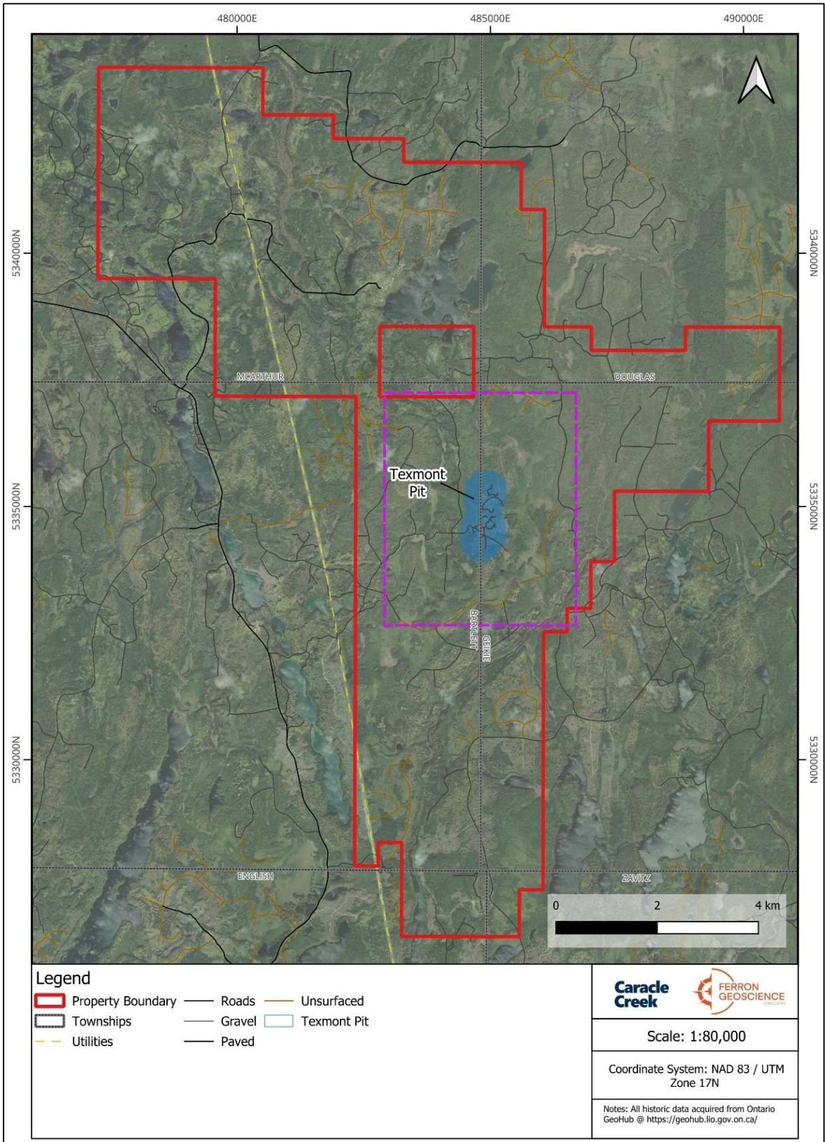
Figure 7-4. Texmont Project boundary showing the location of the optimized pit (shaded blue) along with the overview of Figure 7-5 (purple rectangle) (Caracle Creek, 2025).
