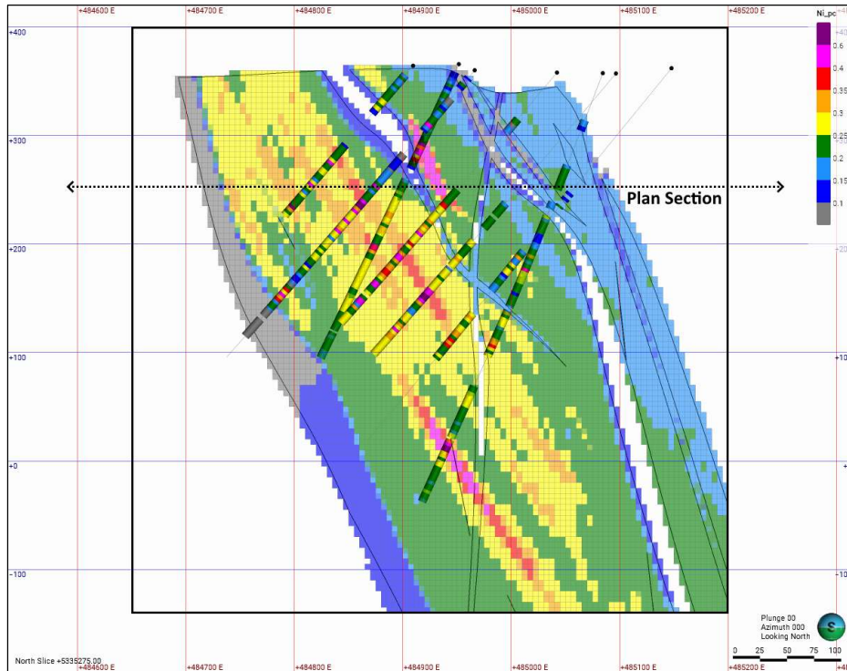
Figure 14-37. Vertical section 5335275 mN (Looking North) of the Texmont Deposit nickel grade blocks against composites within the PER domain in the North Zone. Some intervals may not precisely match their corresponding feature due to the 80 m section width. The dashed line is the trace of the plan section presented in Figure 14-35 (Caracle Creek, 2025).
