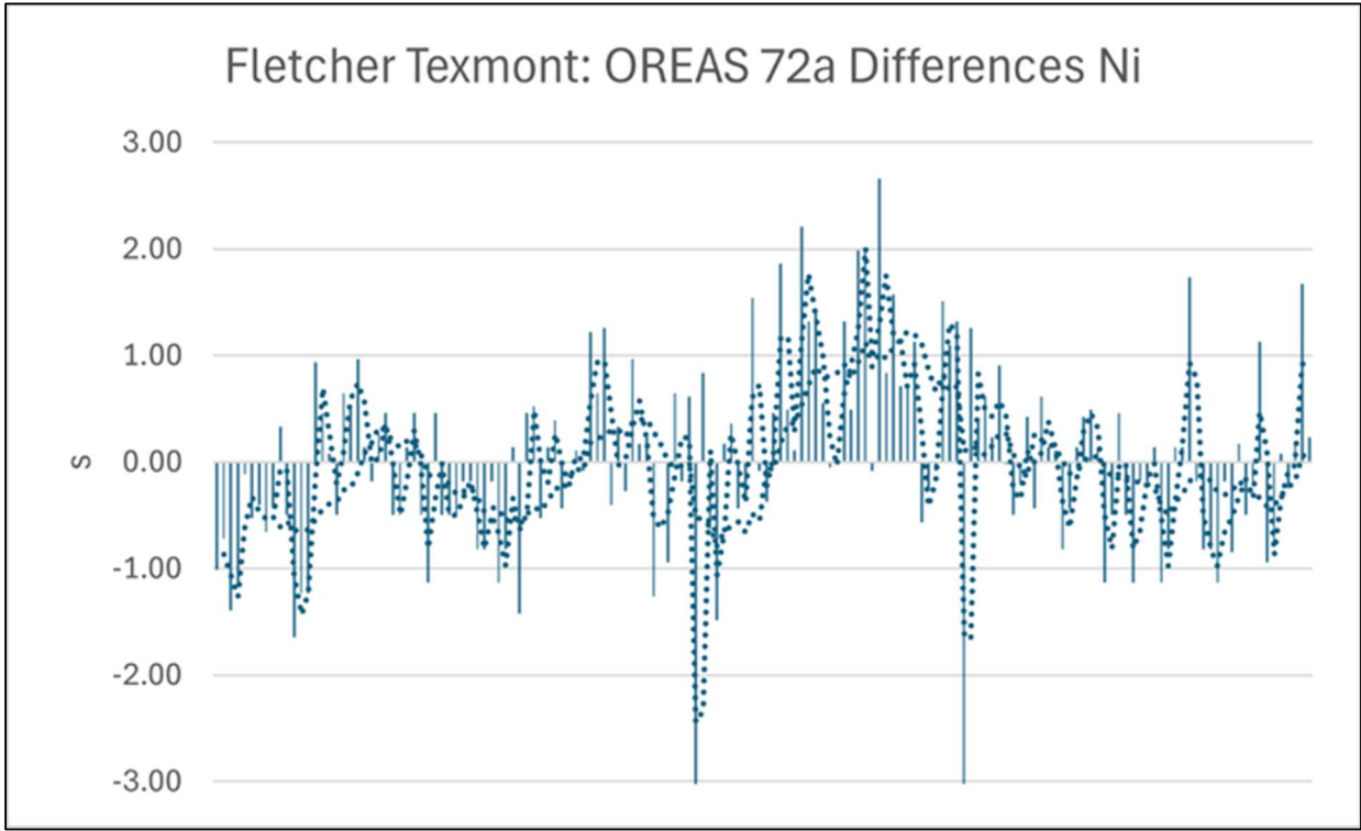
Figure 11-2. Fletcher Texmont CRM OREAS 72a – Number of Standard Deviations Difference for Ni Analysis from the Average Value for Various Analytical Runs (Siriunas, 2025).
