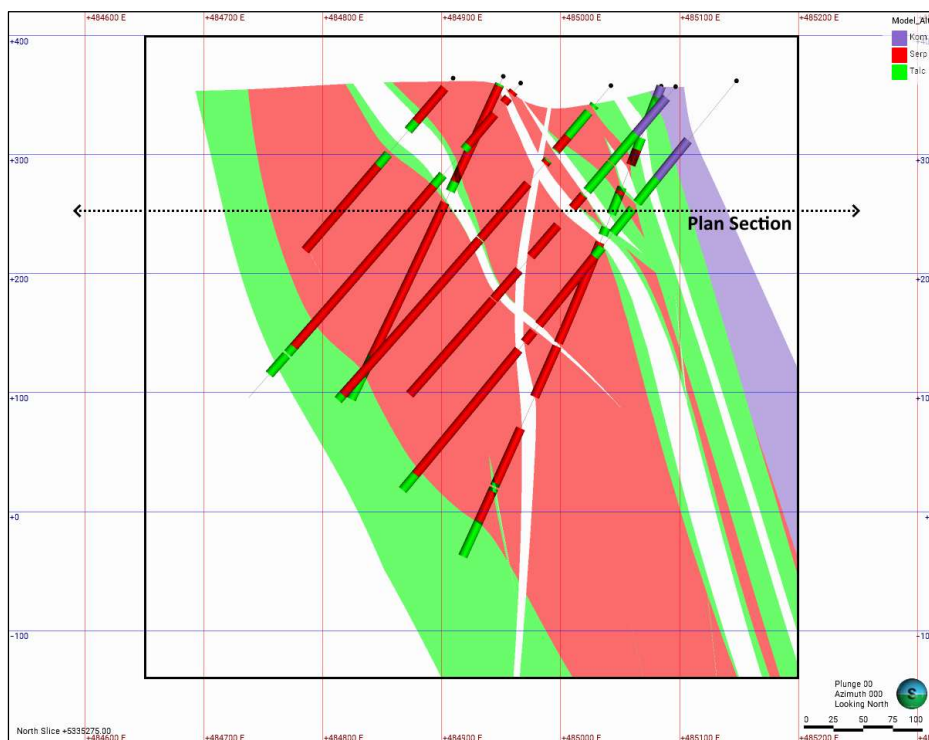
Figure 14-10. Vertical section 5335275 mN (Looking North) of the Texmont alteration model and coded drill hole intervals in the North Zone. Some intervals may not precisely match their corresponding feature due to the 80 m section width. The black outline represents the current resource boundary and main modelling area, and the dashed line is the trace of the plan section presented in Figure 14-8 (Caracle Creek, 2025).
