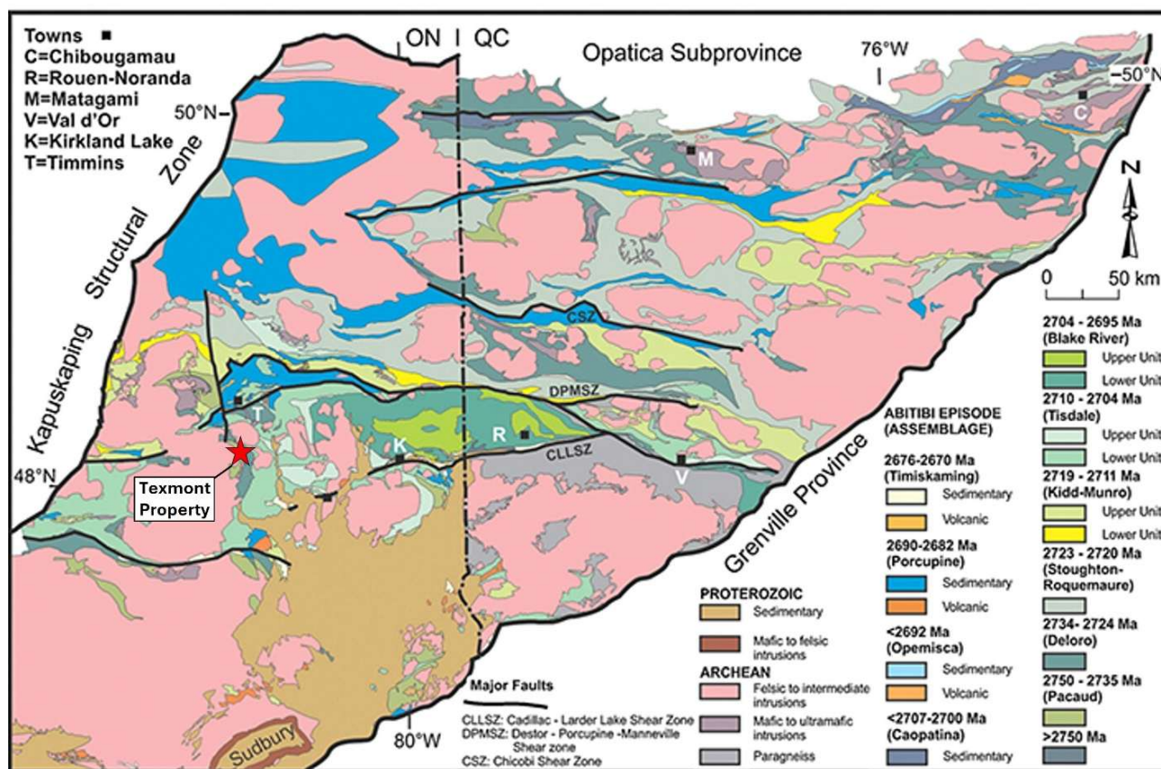
Figure 7-1. Generalized geology of the Abitibi Greenstone Belt showing the location of the Texmont Project (modified from Thurston et al. , 2008).
