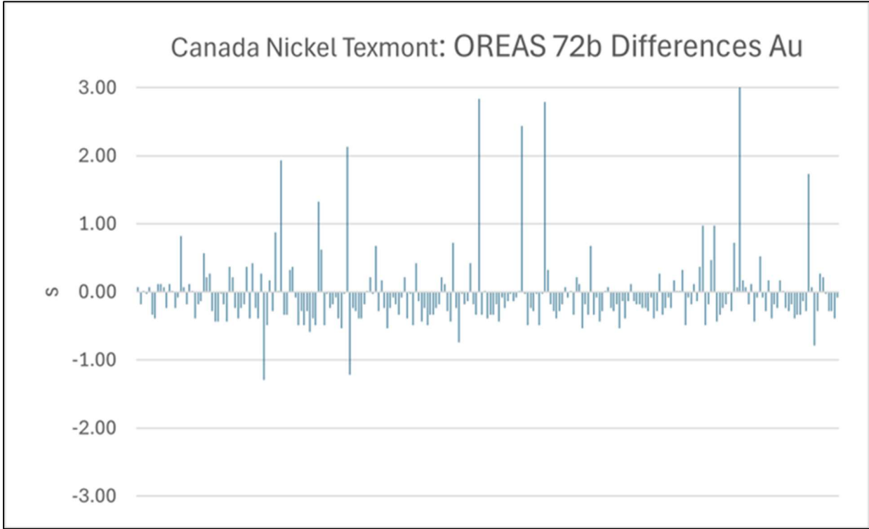
Figure 11-7. Canada Nickel Texmont CRM OREAS 72b – Number of Standard Deviations Difference for Au Analysis from the Average Value for Various Analytical Runs (Siriunas, 2025).
