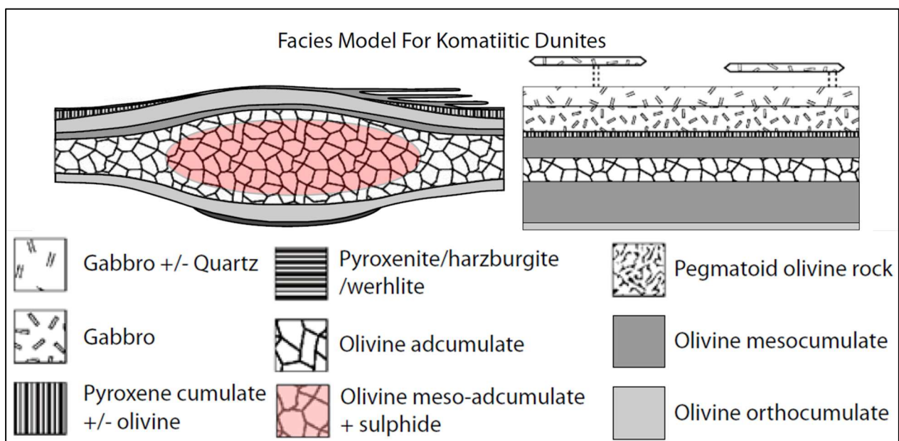
Figure 8-2. Facies model for intrusive komatiitic dunitic (adapted from Rosengren et al. , 2007).
