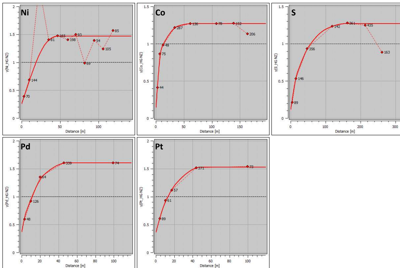
Figure 14-34. Variography for the HG domain in the North Zone (Caracle Creek, 2025).
