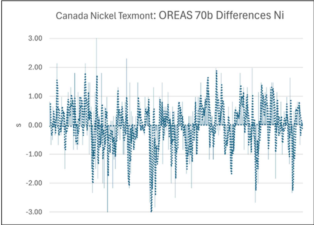
Figure 11-5. Canada Nickel Texmont CRM OREAS 70b – Number of Standard Deviations Difference for Ni Analysis from the Average Value for Various Analytical Runs (Siriunas, 2025).
