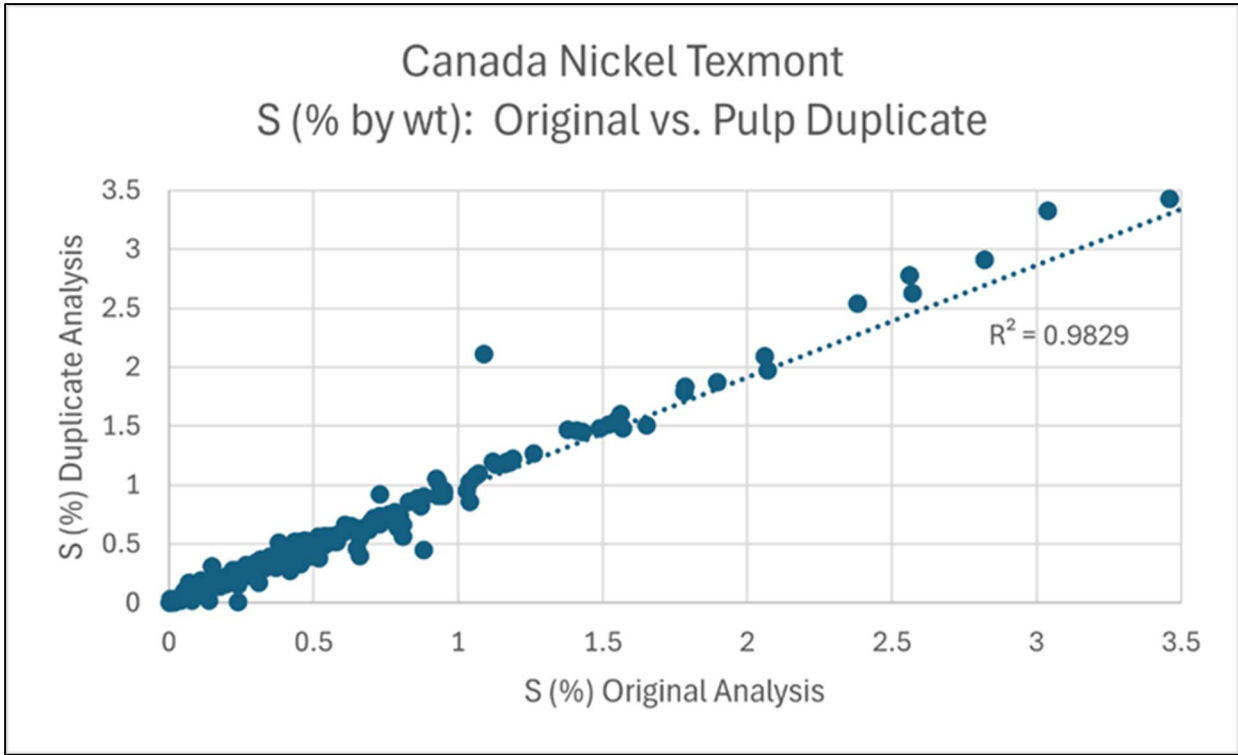
Figure 11-11: Plot of Absolute Concentrations of Pairs of Duplicate Samples Analyzed for S (Siriunas, 2025).
