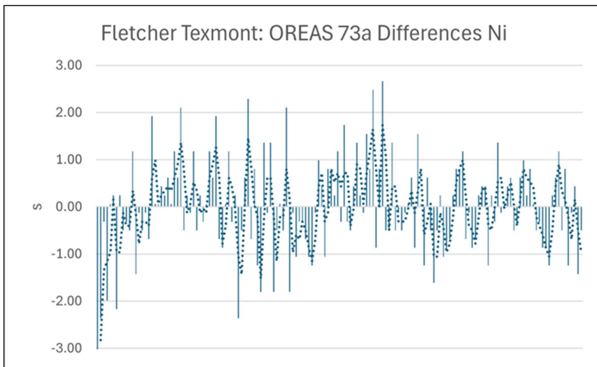
Figure 11-3. Fletcher Texmont CRM OREAS 73a – Number of Standard Deviations Difference for Ni Analysis from the Average Value for Various Analytical Runs (Siriunas, 2025).
