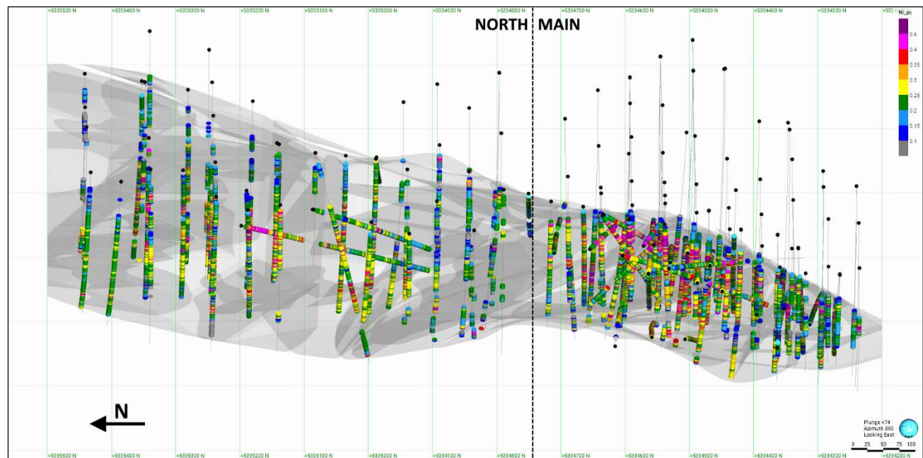
Figure 14-12. Oblique longitudinal view (Looking East and Downwards with 74° plunge), parallel to the mineralization trend, of the Texmont Deposit PER estimation domain (transparent grey) and nickel grade drill hole intervals (Caracle Creek, 2025).
