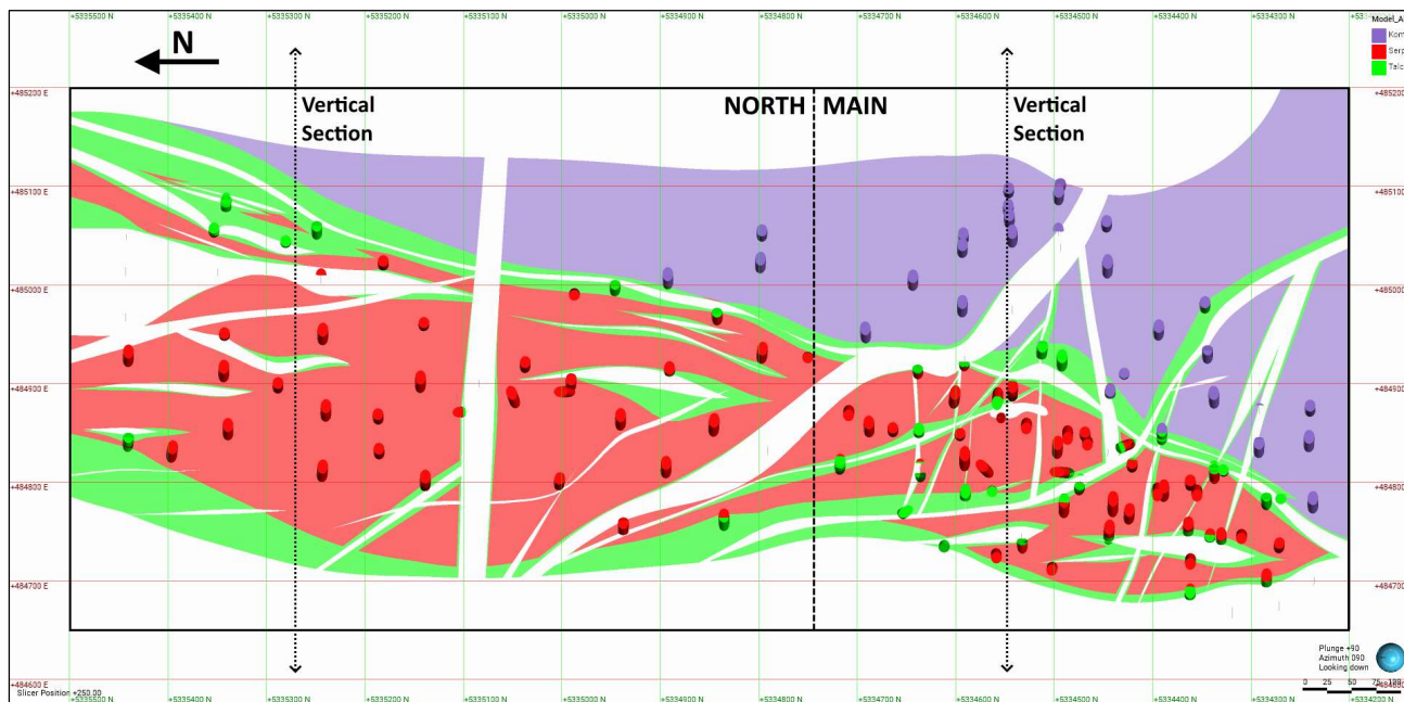
Figure 14-8. Plan section (250 RL) of the Texmont Deposit alteration model and coded drill hole intervals. The black rectangle represents the current resource boundary and main modelling area, and the dashed lines are traces of the vertical sections presented in Figures 14-9 and 14-10 (Caracle Creek, 2025).
