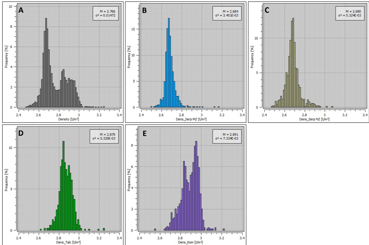
Figure 14-18. Histograms of density populations in: A) Ultramafic package (PER-KOM units), B) Serp domain in the Main Zone, C) Serp domain in the North Zone, D) Talc domain E) Kom Domain (Caracle Creek, 2025).
