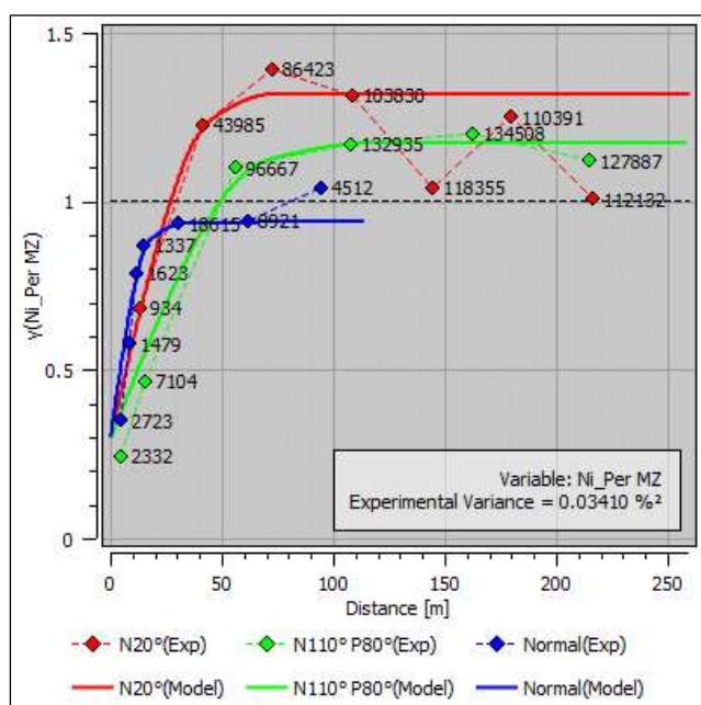
Figure 14-42. Nickel variogram of the Main Zone's PER domain, for resource classification (Caracle Creek, 2025).
