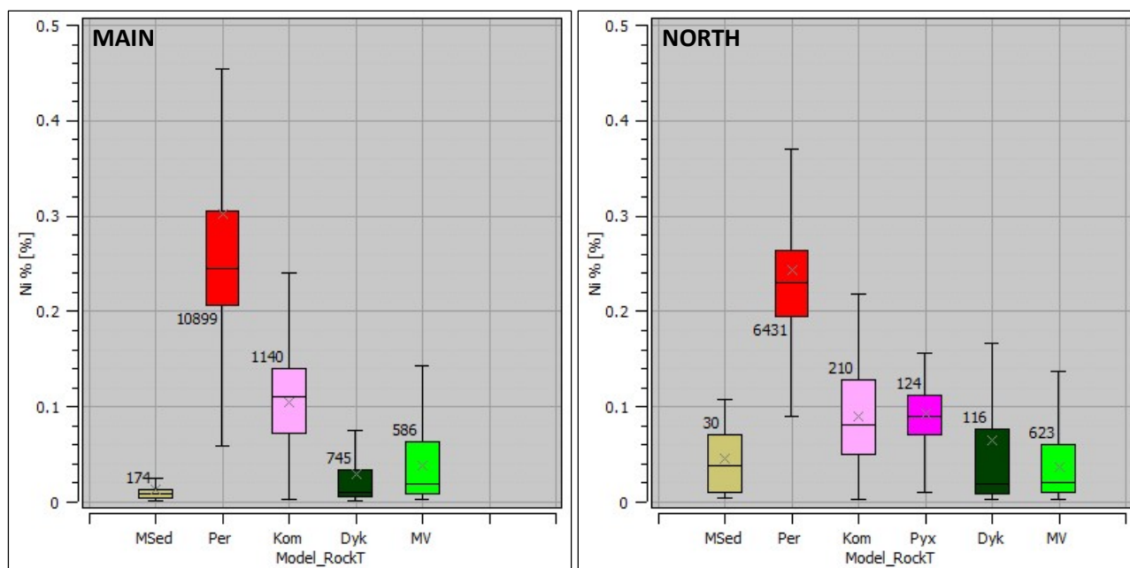
Figure 14-11. Boxplots of nickel grades according to the Texmont Deposit lithology model in the Main and North Zones, showing that the PER domain contains the bulk of the mineralization (Caracle Creek, 2025).
