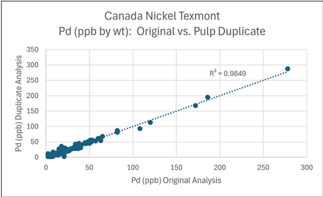
Figure 11-13: Plot of Absolute Concentrations of Pairs of Duplicate Samples Analyzed for Pd (Siriunas, 2025).
