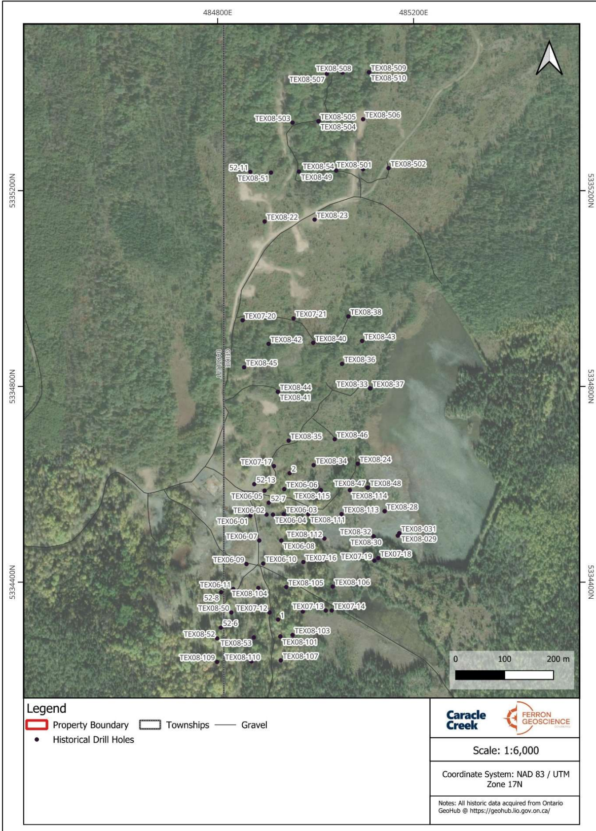
Figure 6-2. Locations of historical diamond drilling in the central historical mine site portion of the Property (Caracle Creek, 2025).
