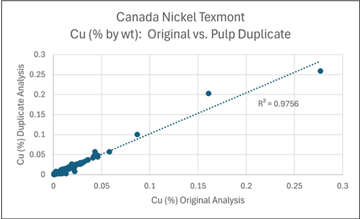
Figure 11-16. Plot of Absolute Concentrations (capped) of Pairs of Duplicate Samples Analyzed for Cu (Siriunas, 2025).
