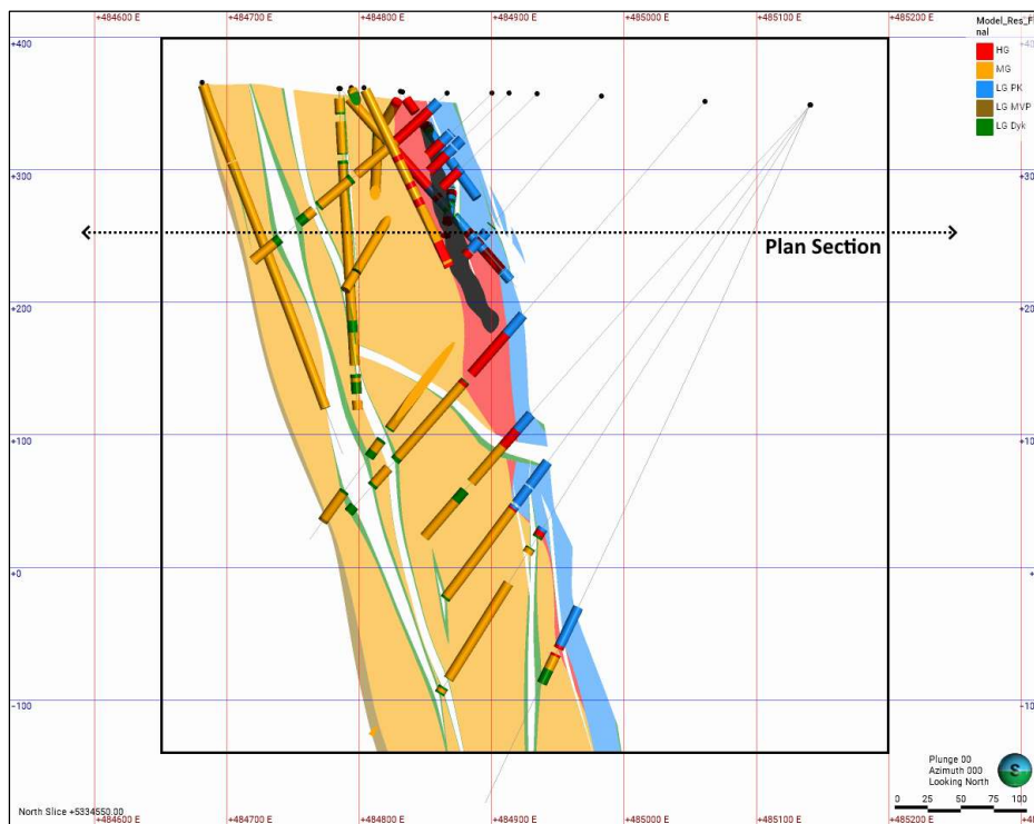
Figure 14-20. Vertical section 5334550 mN (Looking North) of the Texmont Deposit estimation domains and coded drill hole intervals in the Main Zone. Some intervals may not precisely match their corresponding feature due to the 50 m section width. The former Texmont Mine underground workings are represented by the dark envelope. The dashed line is the trace of the plan section presented in Figure 14-19 (Caracle Creek, 2025).
