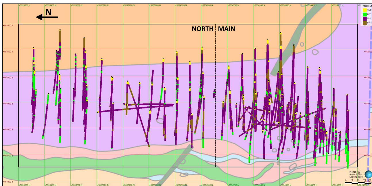
Figure 14-3. Plan view (North to the left) of the Texmont Project with drill hole intervals showing the main rock types. Background lithology from OGS (Houlé et al. , 2009). The ultramafic package (UM) is coloured purple in the map and drill traces. The black rectangle represents the current resource boundary and main modelling area (Caracle Creek, 2025).
