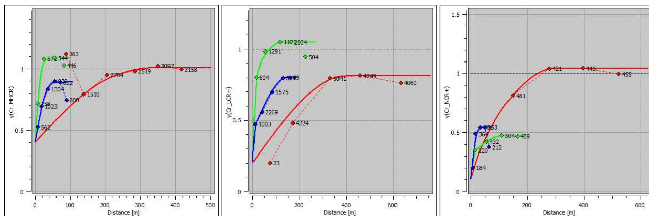
Figure 14-31. Density variography for the Serp domain in the Main (left) and North (centre) zones, and the Kom Domain (right) (Caracle Creek, 2025).
