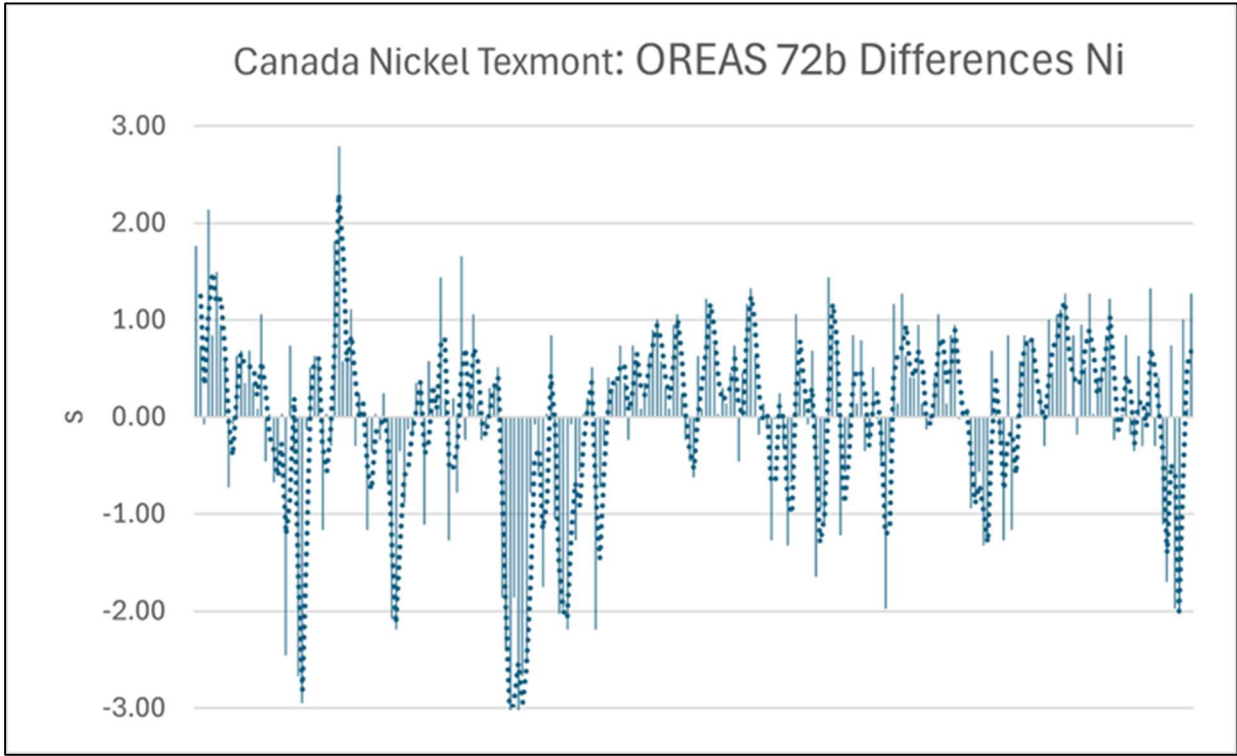
Figure 11-6. Canada Nickel Texmont CRM OREAS 72b – Distribution of Standard Deviations Difference for Ni Analysis from the Average Value for Various Analytical Runs at Actlabs (Siriunas, 2025).
