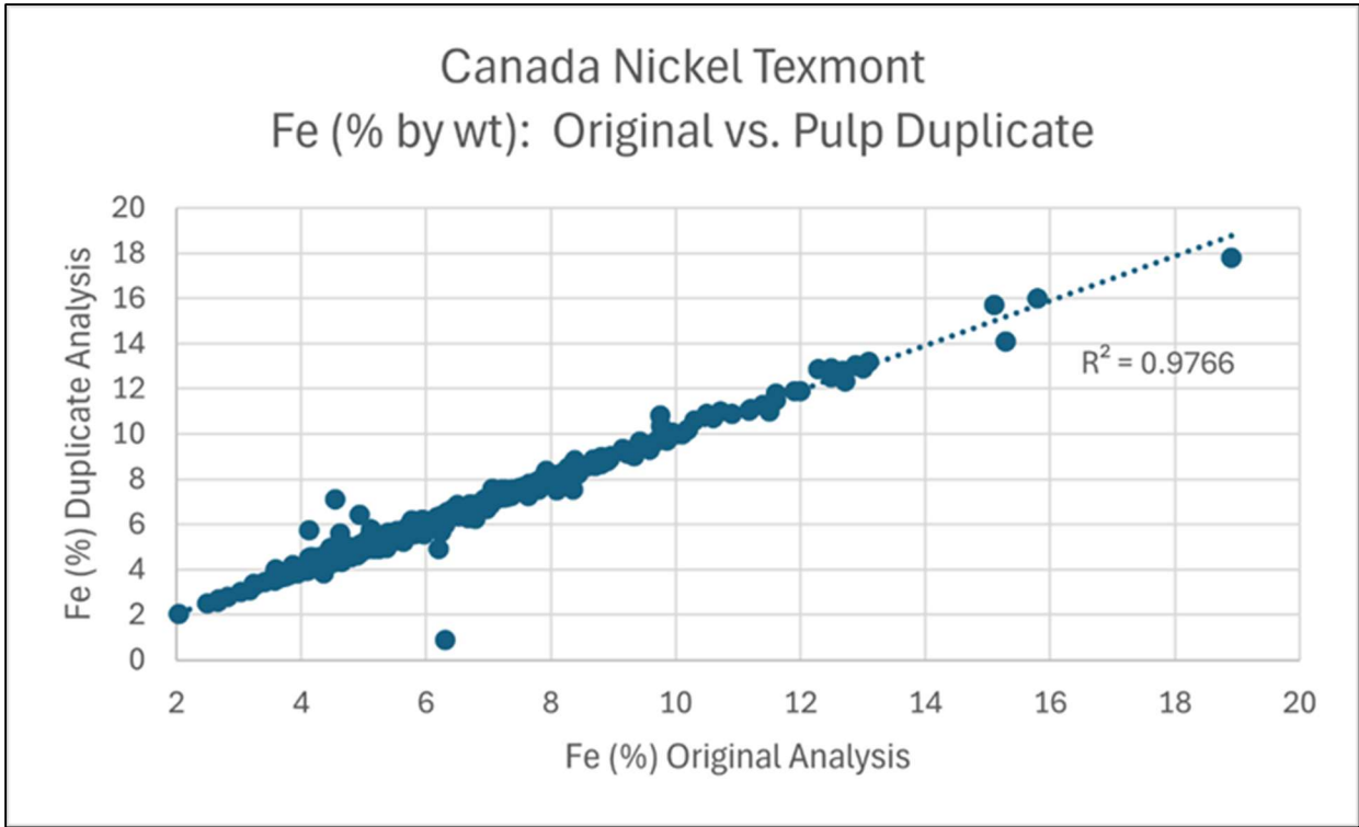
Figure 11-17. Plot of Absolute Concentrations of Pairs of Duplicate Samples Analyzed for Fe (Siriunas, 2025).
