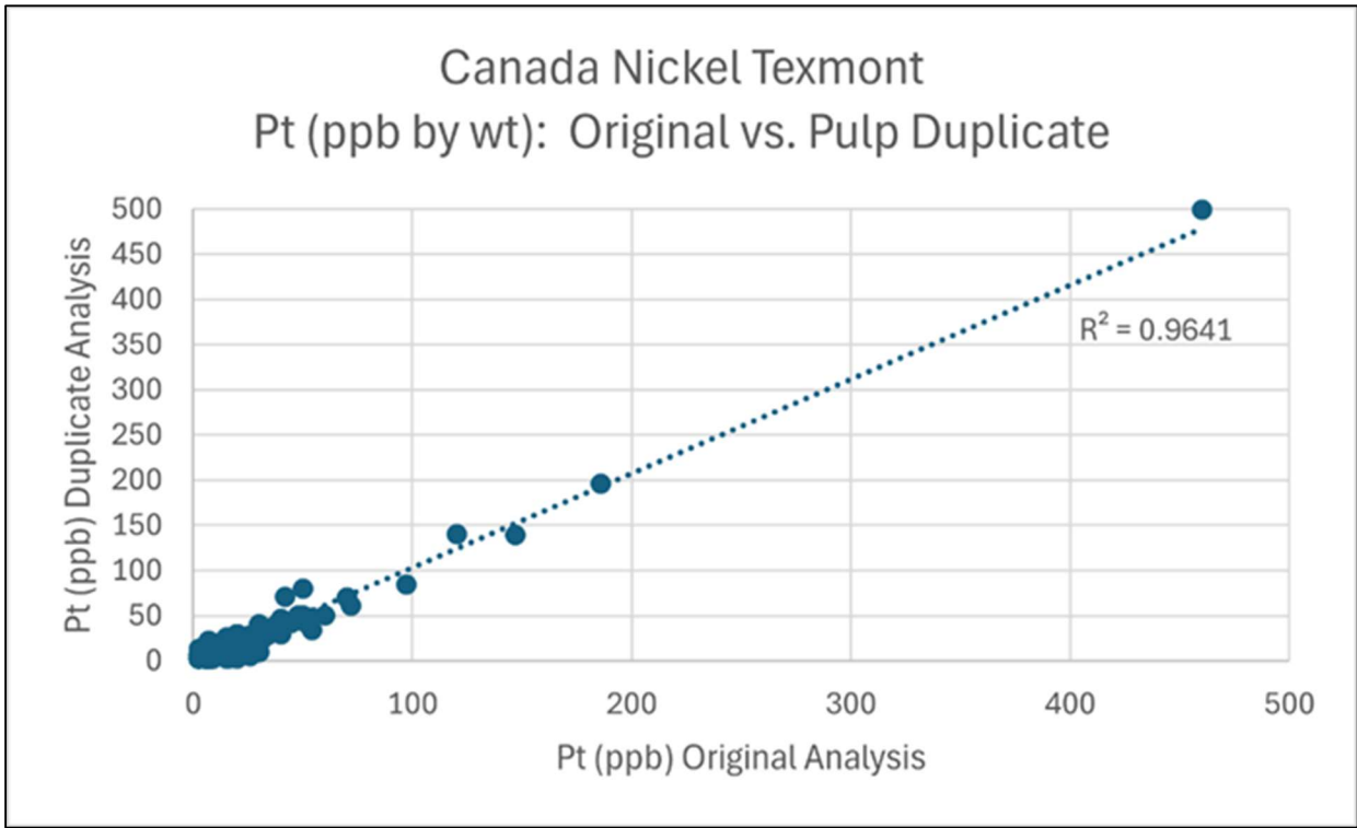
Figure 11-14. Plot of Absolute Concentrations of Pairs of Duplicate Samples Analyzed for Pt (Siriunas, 2025).
