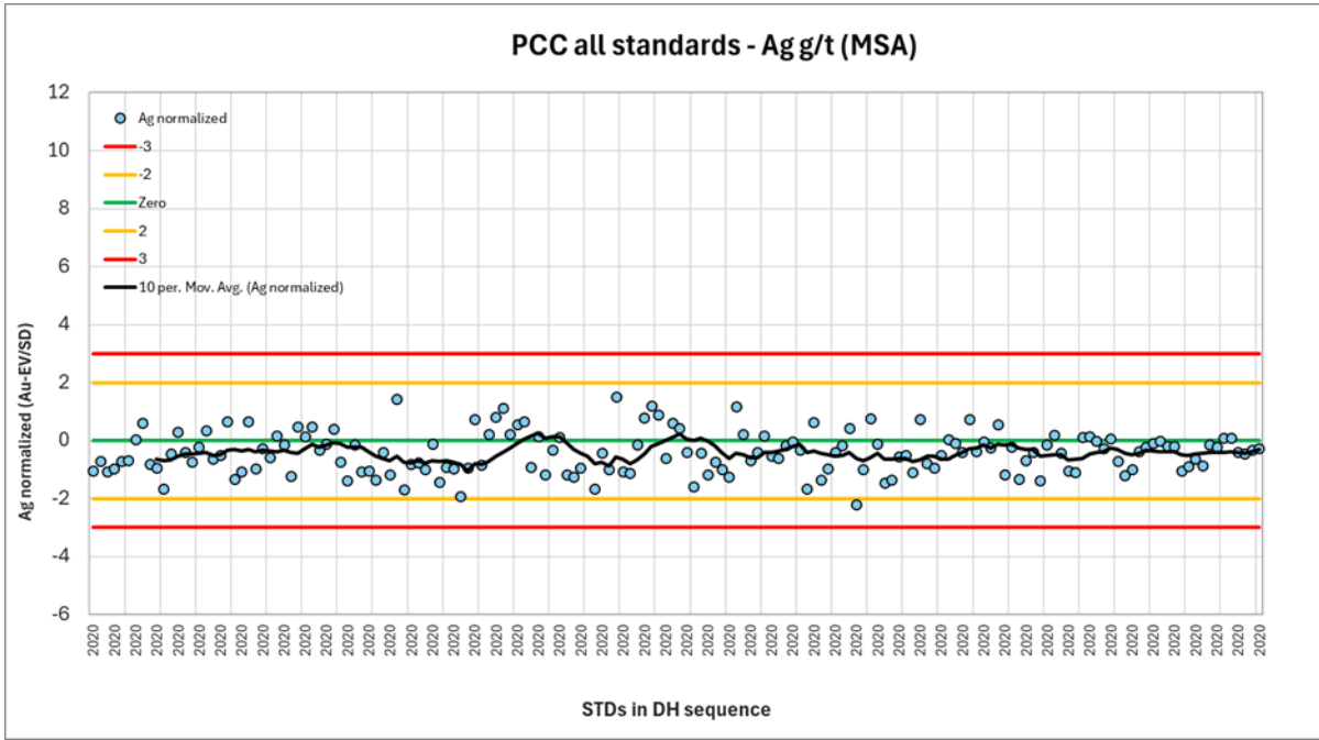
Figure 11-9: 2020 PCCCRM Performance MSA – Ag (Source: MMTS, 2025)
