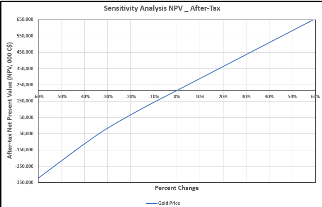
Figure 22-4: After-tax NPV Sensitivity (Gold Price Only, +/-60%)
