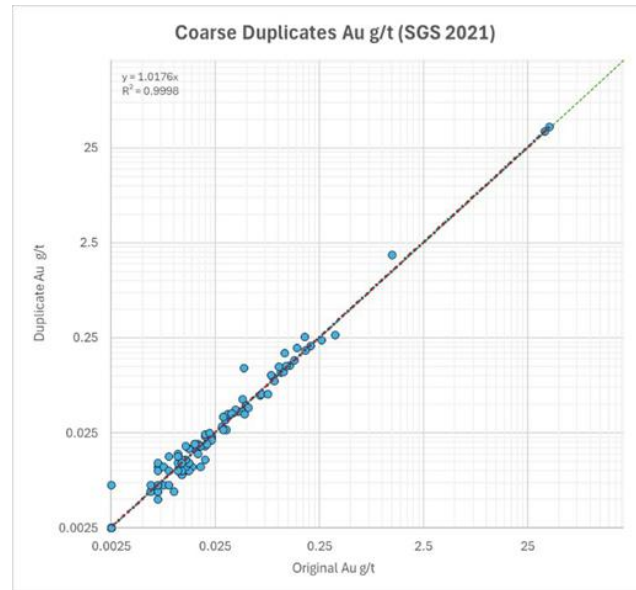
Figure 11-16: 2021 Coarse Duplicates Scatter Plot SGS – Au (Source: MMTS, 2025)
