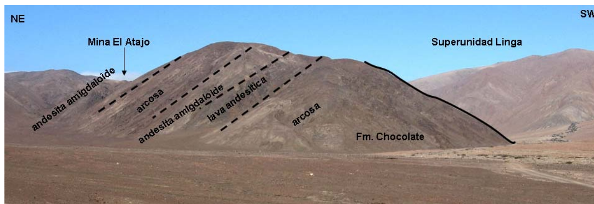
Figure 7.3 Gentle North-Northeast Regional Dip of the Chocolate Formation
