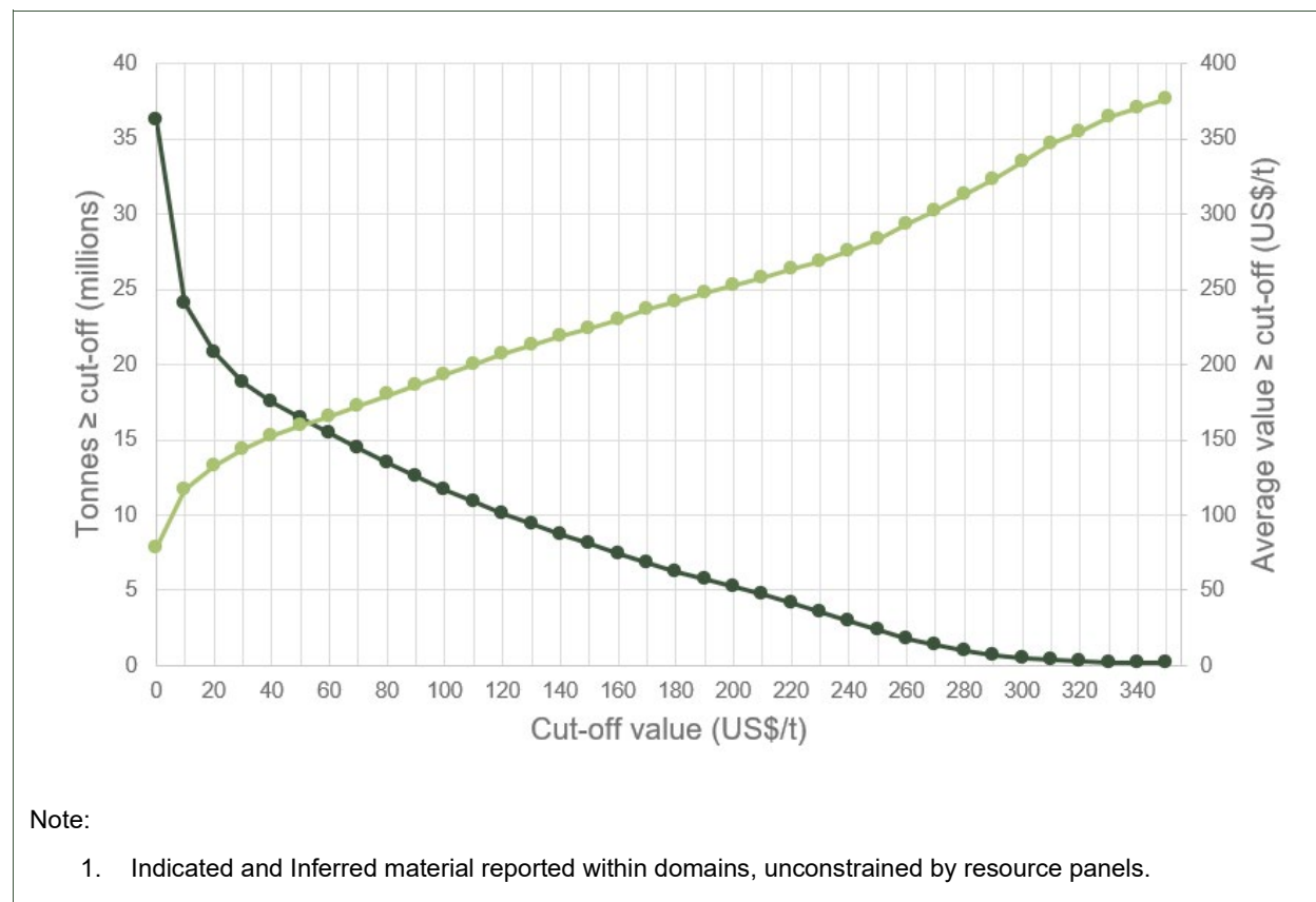
Figure 14-23: NSR Grade-Tonnage Curve – Selebi North
