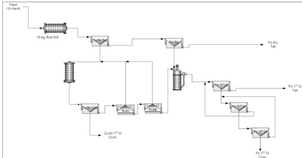
Figure 13-3: Flowsheet of LCT-9 and LCT-10
