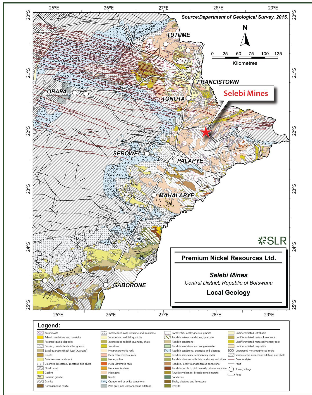
Figure 7-2: Local Geology
