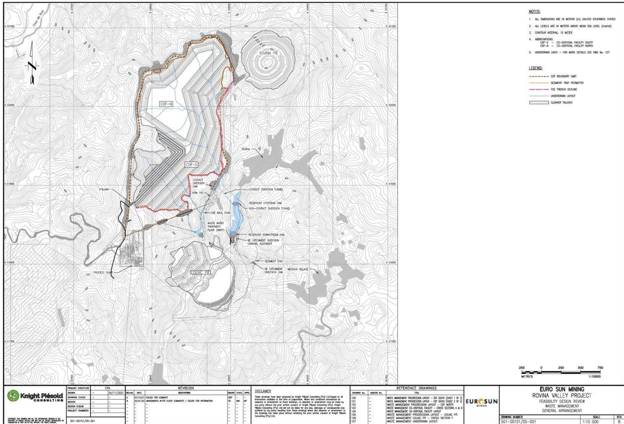
Figure 18.7: General Arrangement Plan of the CDF and Colnic Pit
