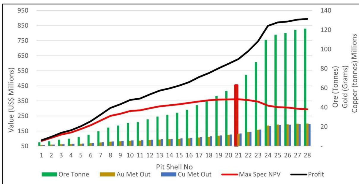
Figure 1.2: Rovina Whittle Analysis Results
