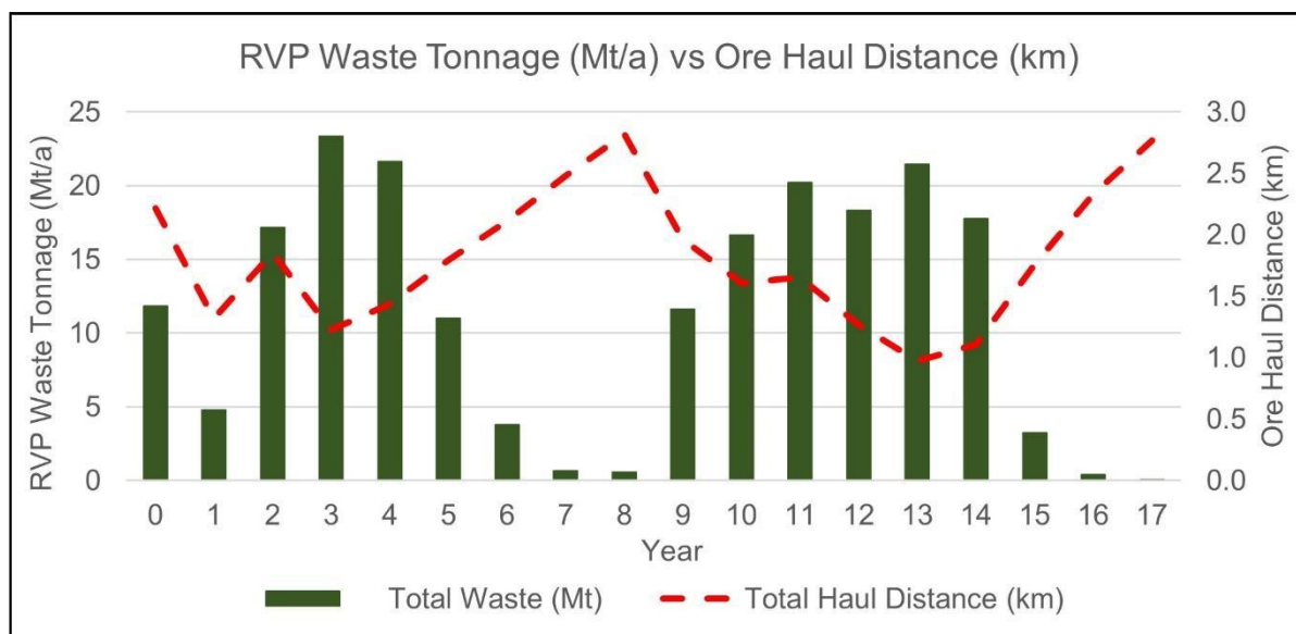
Figure 1.7: Weight Averaged Haul Distances – Total Mine Waste
