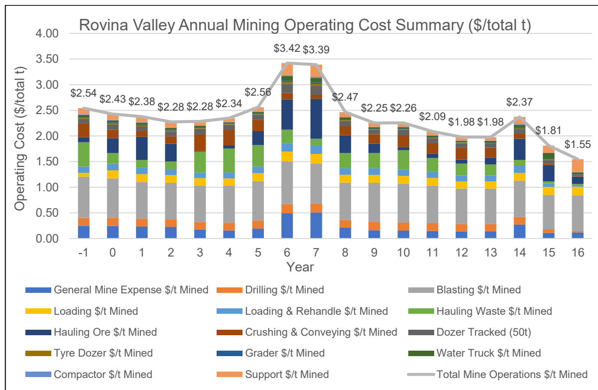
Figure 21.5: Mining Operating Cost (US$ per total tonne)
