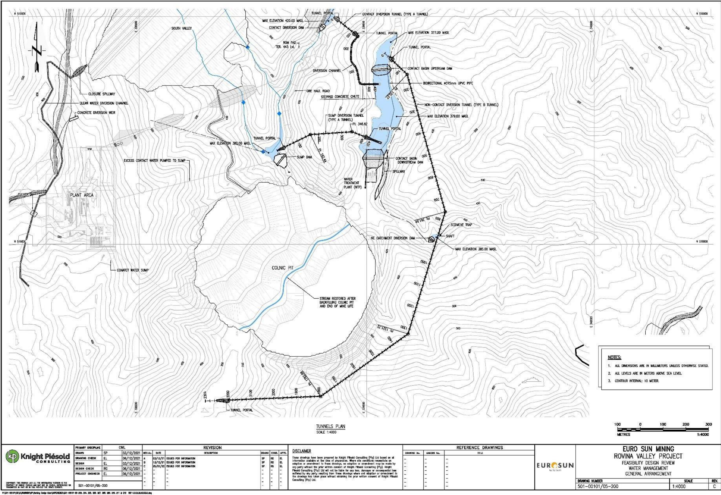
Figure 18.8: Water Management Facilities – Plan
