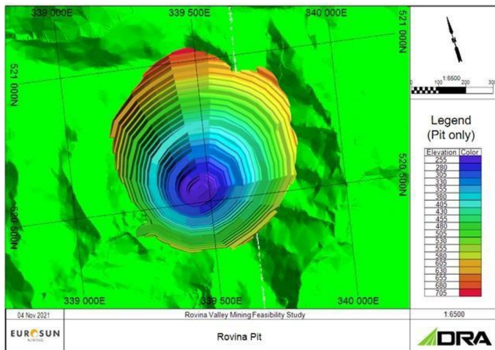
Figure 16.10: Rovina Pit Design
