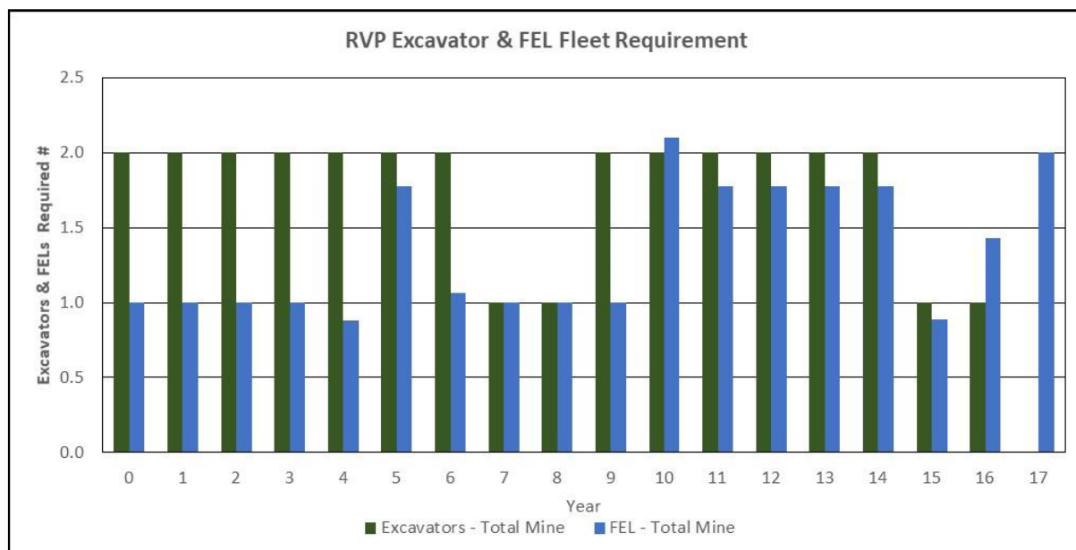
Figure 1.6: LOM Excavator and FEL Fleet
