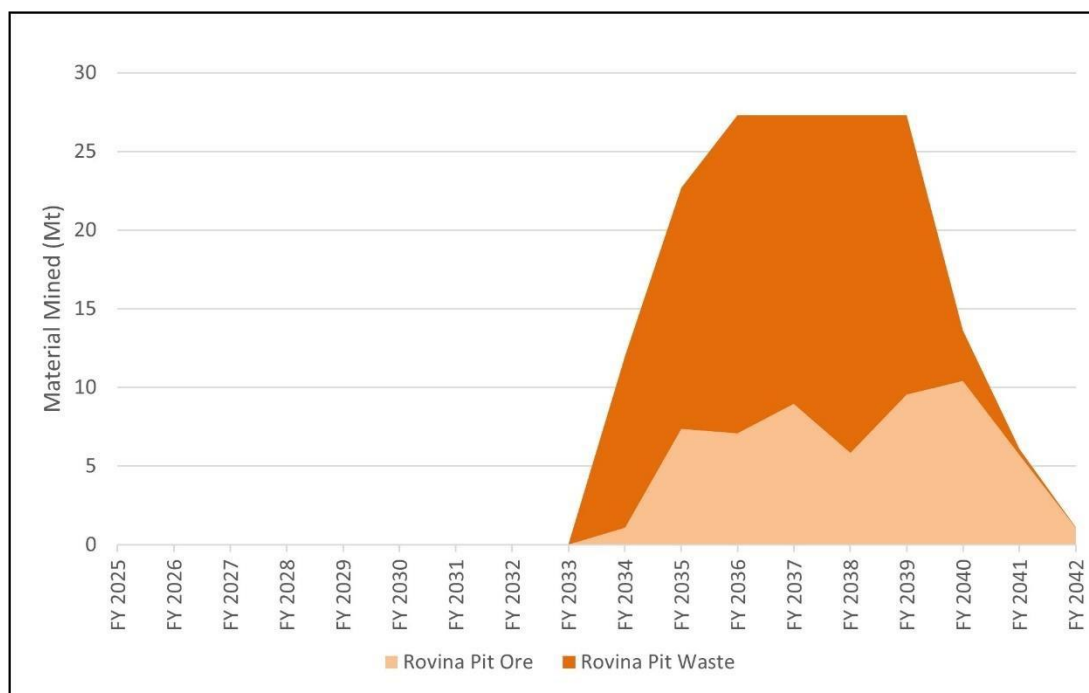
Figure 22.2: Mining at the Rovina Pit
