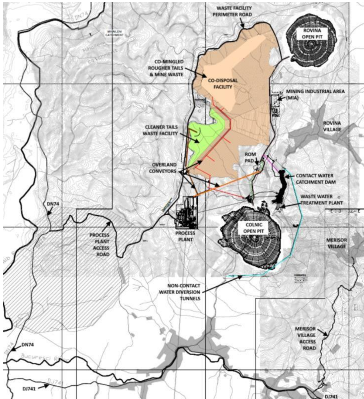
Figure 18.4: RVP Off-Site Infrastructure
