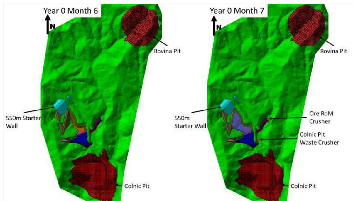
Figure 16.32: Co-Disposal Facilities (Year 0 – Months 6 and 7)
