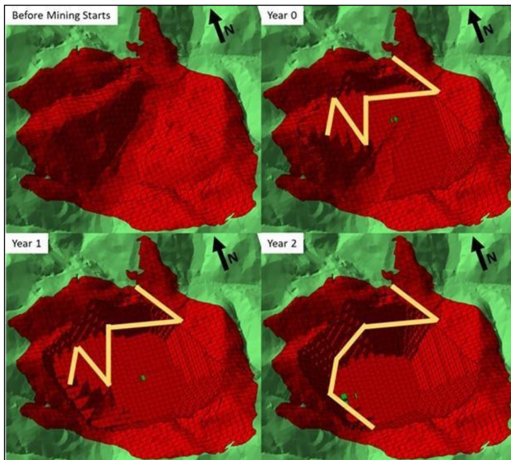
Figure 16.17: Colnic Pit (Pre-Mining to End of Year 2)
