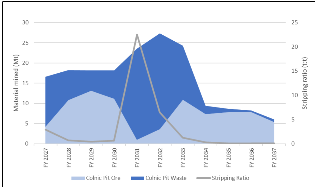
Figure 22.1: Mining at the Colnic Pit
