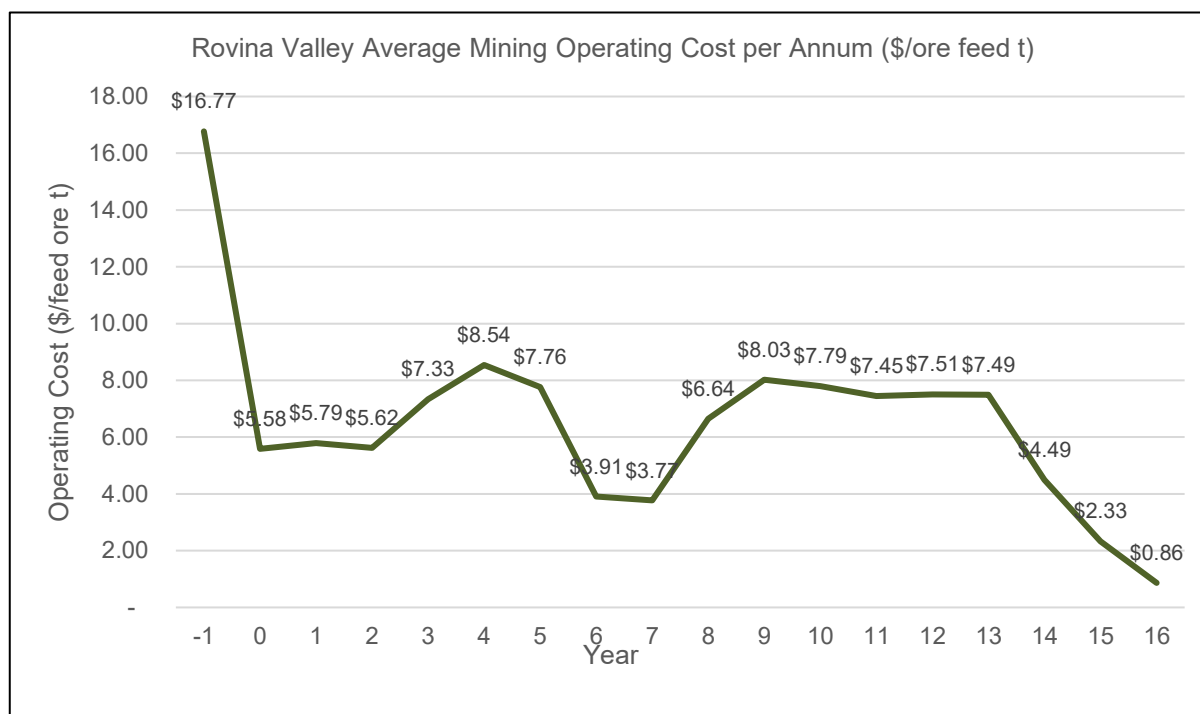
Figure 21.7: Mining Unit Cost per Tonne Milled per Annum
