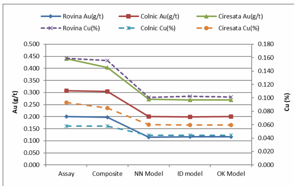
Figure 14.9: Global Statistical Comparison – All Lithologies at 0.00 Cut-Off
