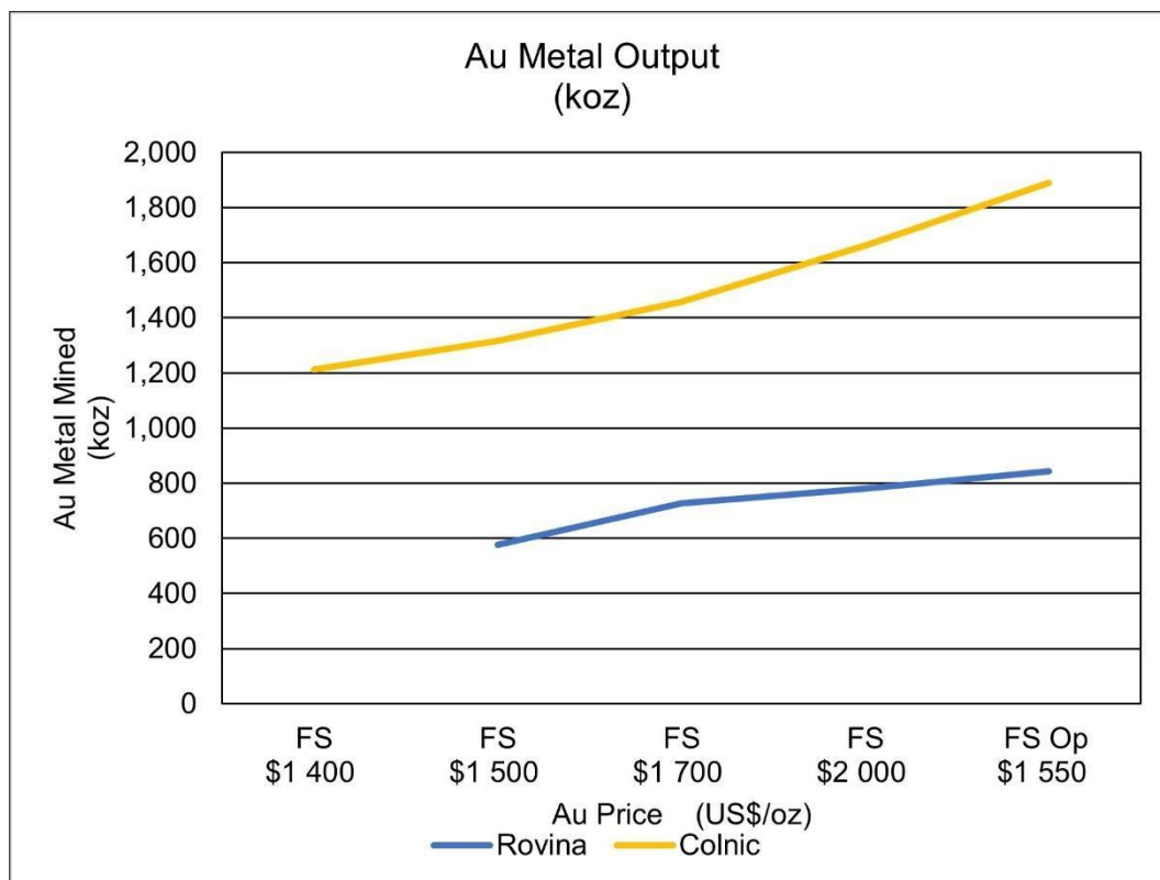
Figure 16.4: Mining Au Metal Output
