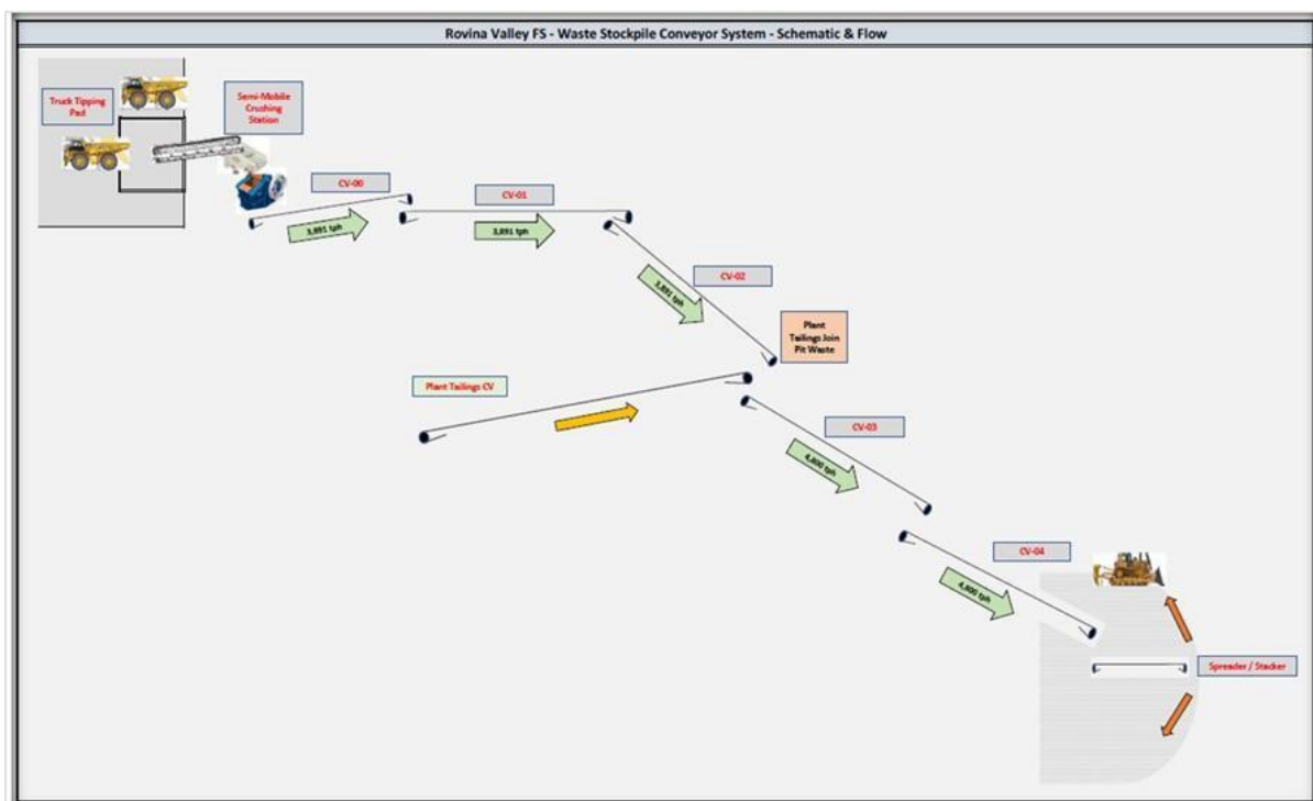
Figure 16.45: Waste Conveyor System Schematic
