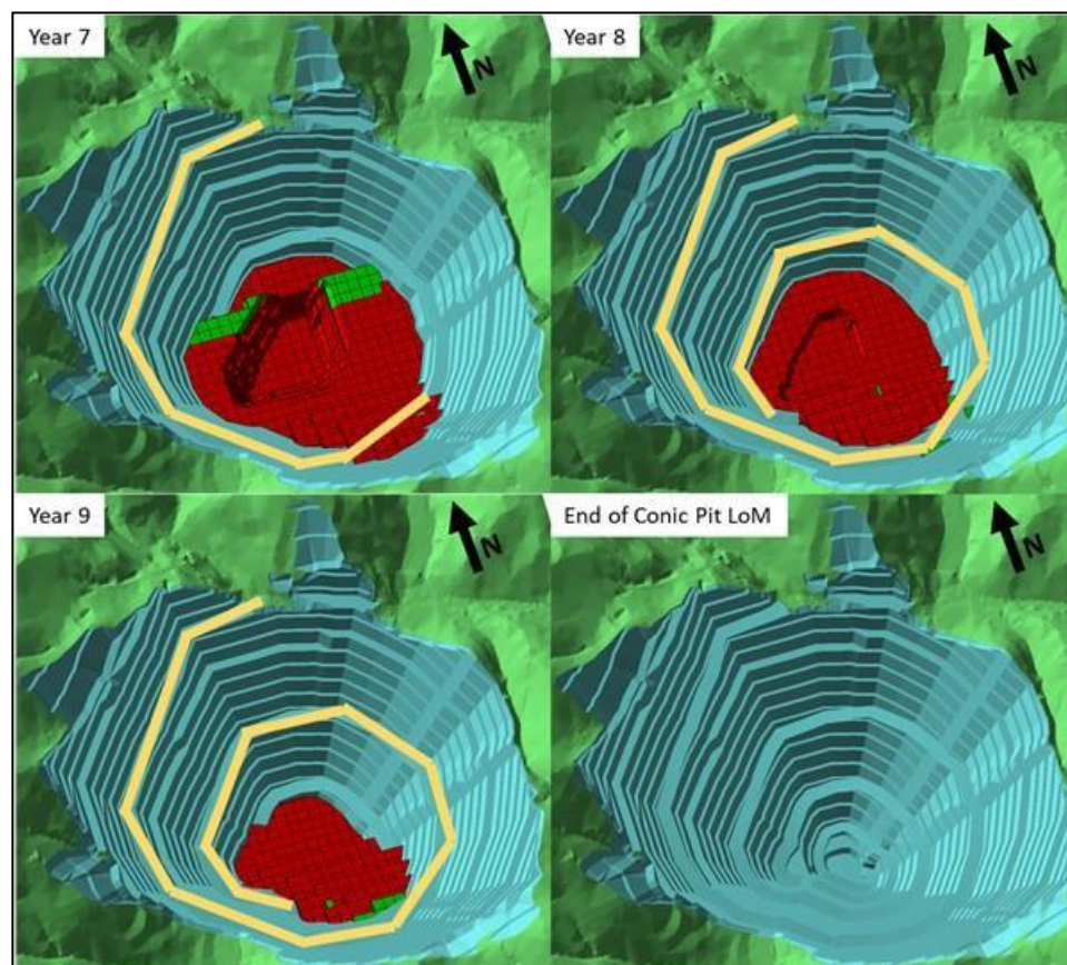
Figure 16.19: Colnic Pit (End of Year 7 to End of Life)
