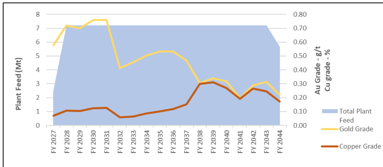
Figure 22.4: Plant Feed Tonnes and Grades
