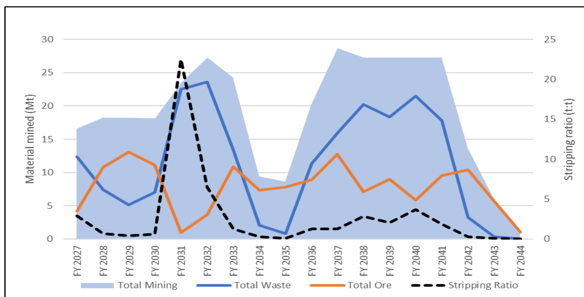
Figure 22.3: Combined Mining Schedule
