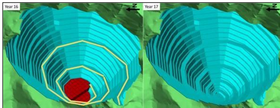
Figure 16.22: Rovina Pit (End of Mining Year 16 to LOM)
