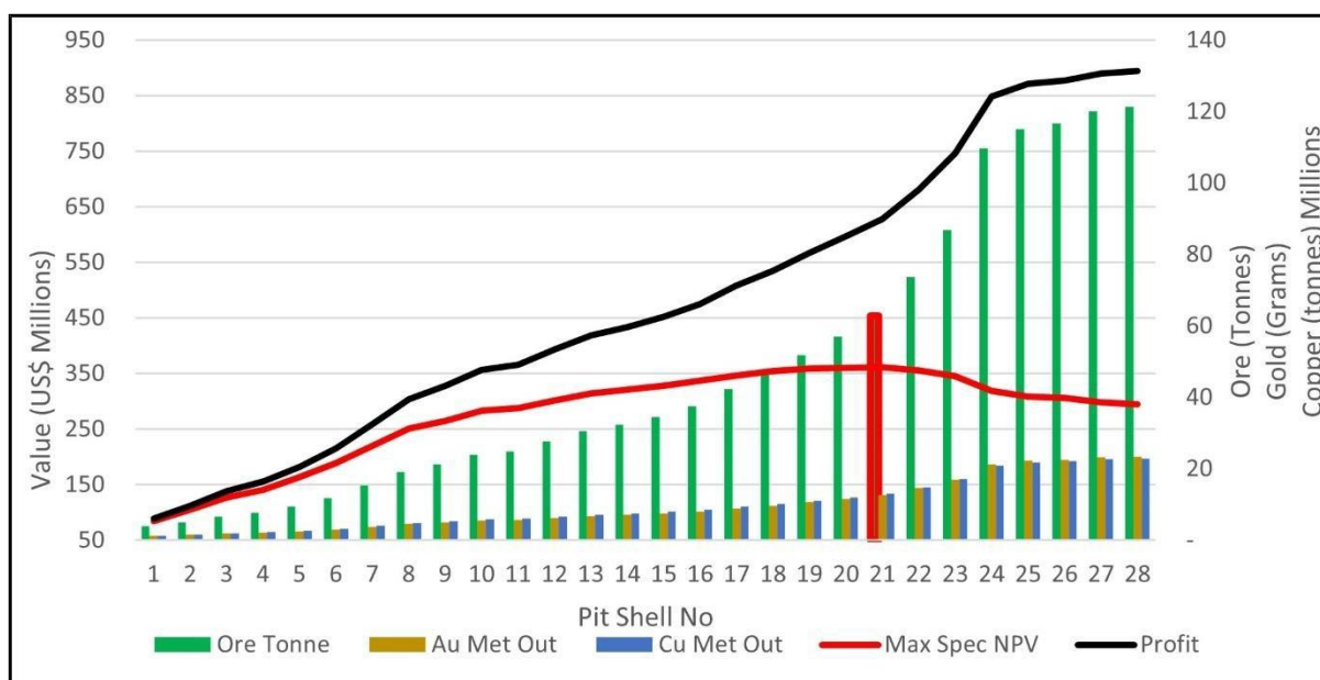
Figure 16.8: Rovina Whittle Analysis Results
