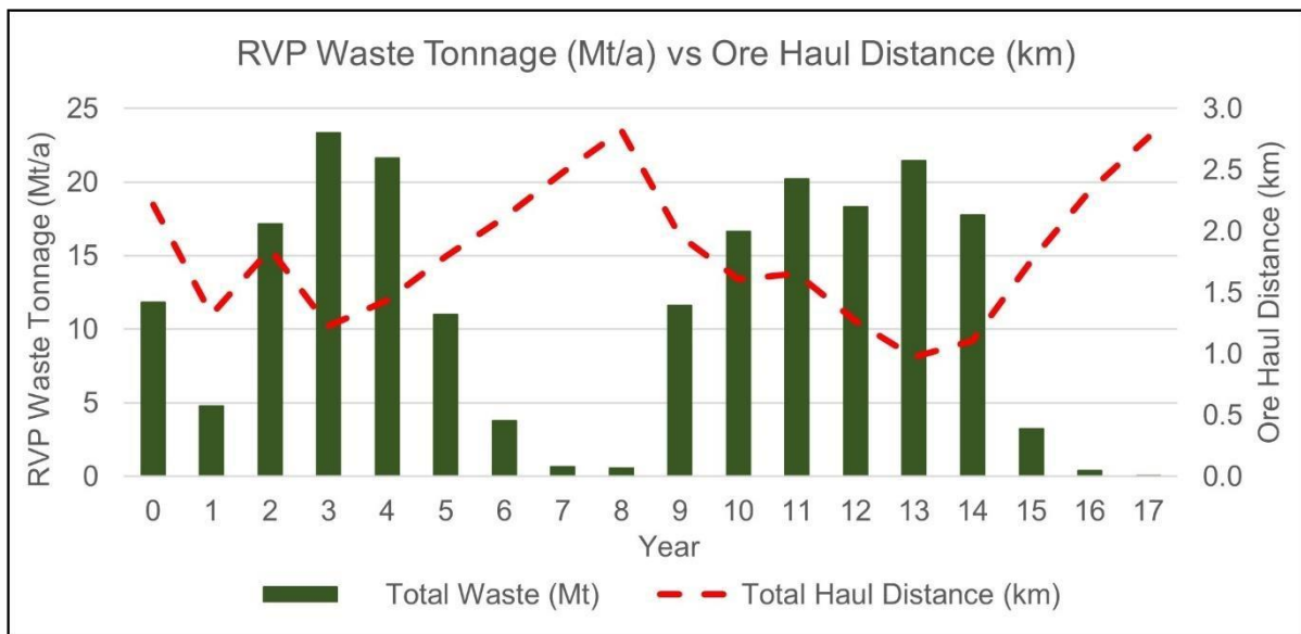
Figure 16.27: Weight Averaged Haul Distances – Total Mine Waste
