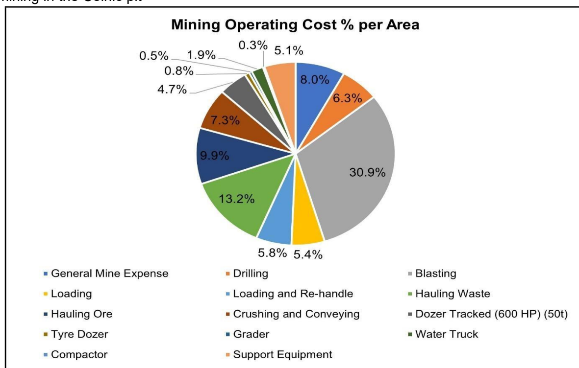
Figure 21.6: Mining LOM Operating Cost Distribution
