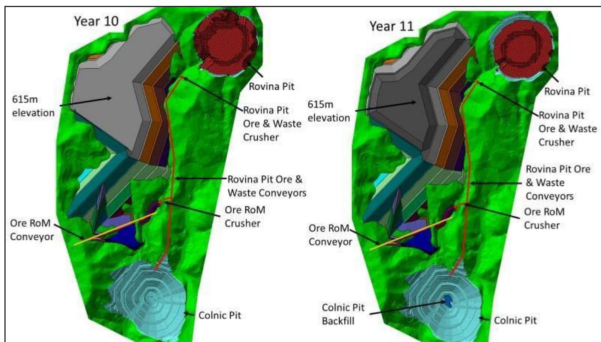
Figure 16.40: Co-Disposal Facilities (Years 10 and 11)
