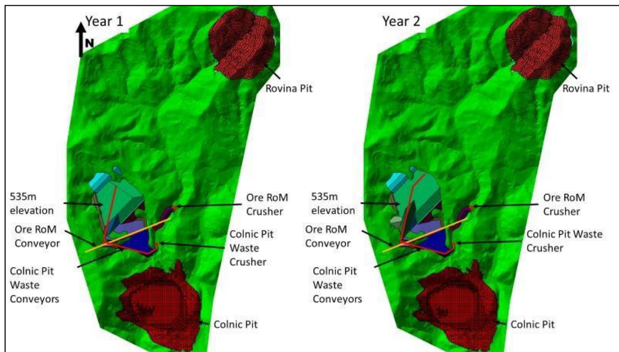
Figure 16.35: Co-Disposal Facilities (Years 1 and 2)
