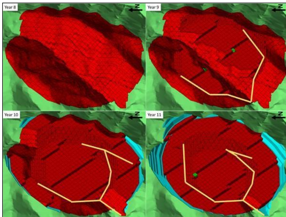
Figure 16.20: Rovina Pit (End of Mining Years 8 to 11)
