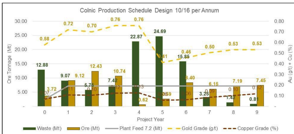
Figure 16.13: Colnic Production Schedule Design per Annum
