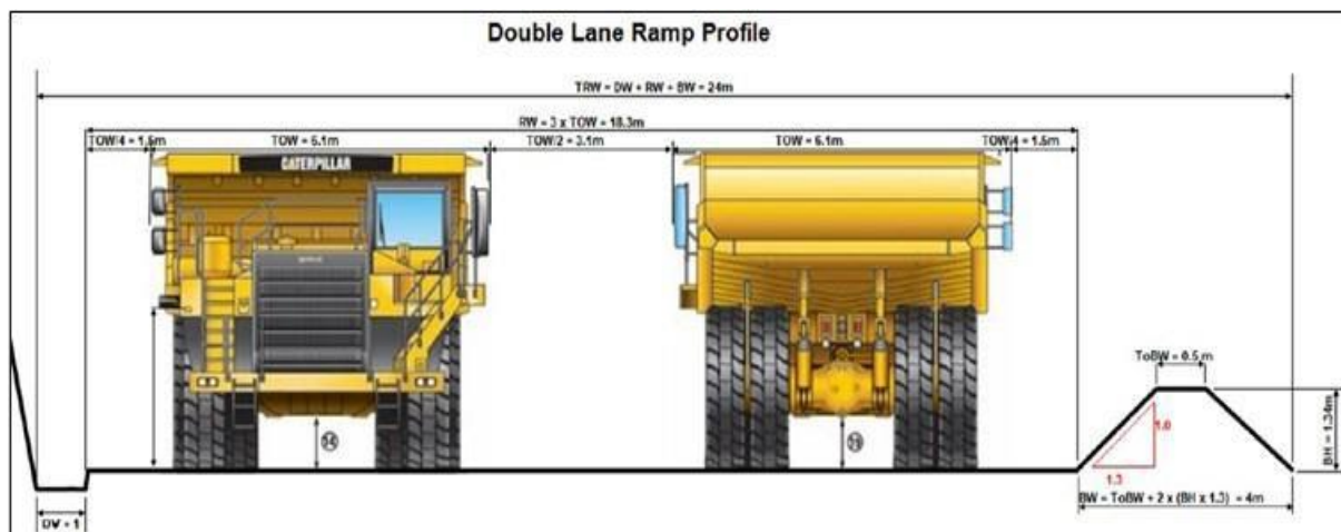
Figure 16.24: Double-Lane Ramp Profile
