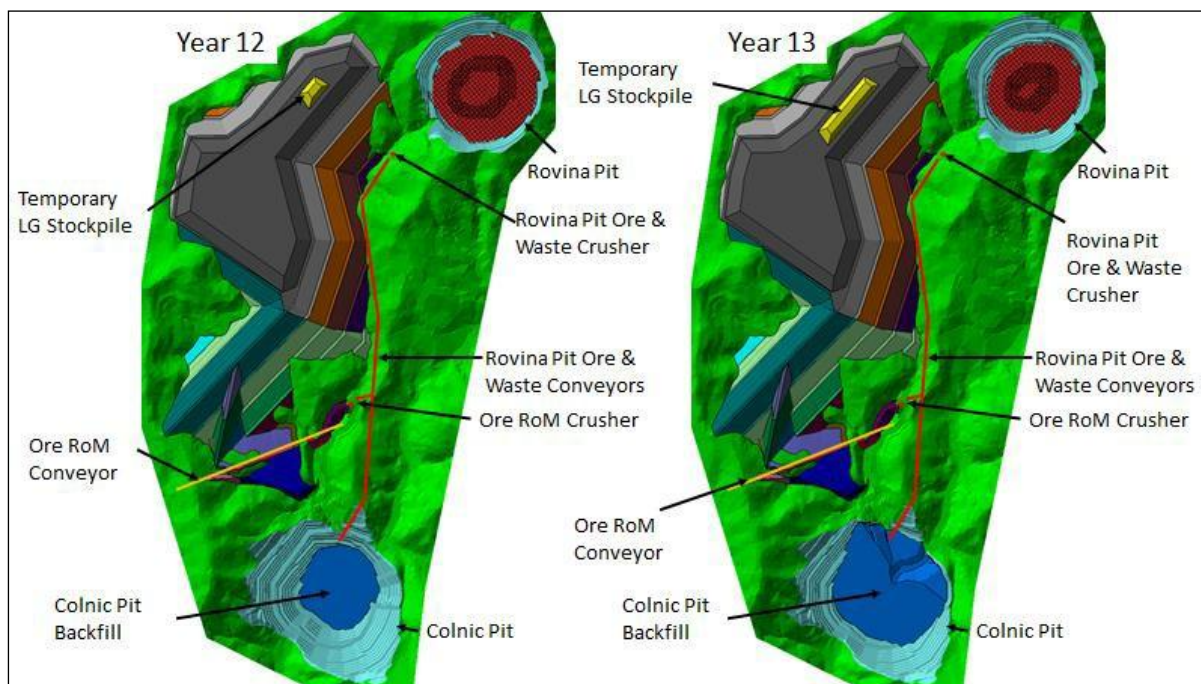
Figure 16.41: Co-Disposal Facilities (Years 12 and 13)
