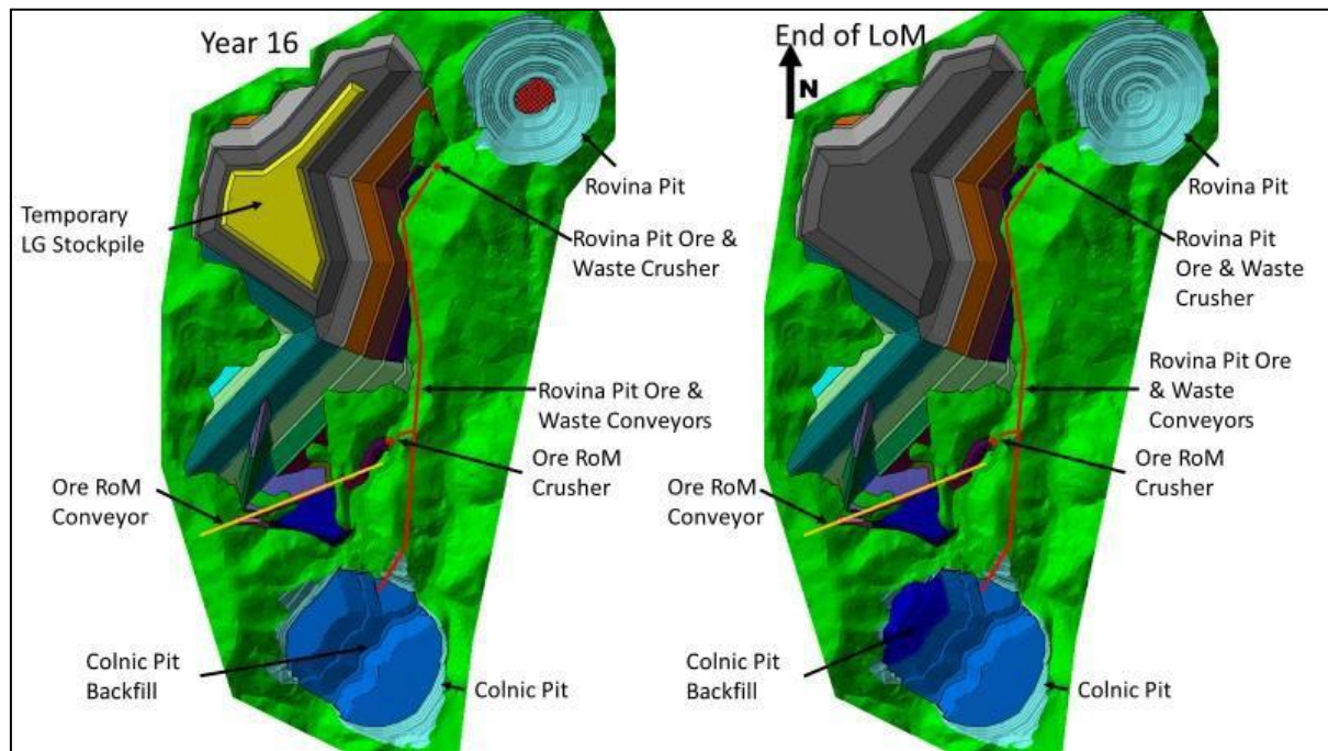
Figure 16.43: Co-Disposal Facilities (Year 16 and End of LOM)
