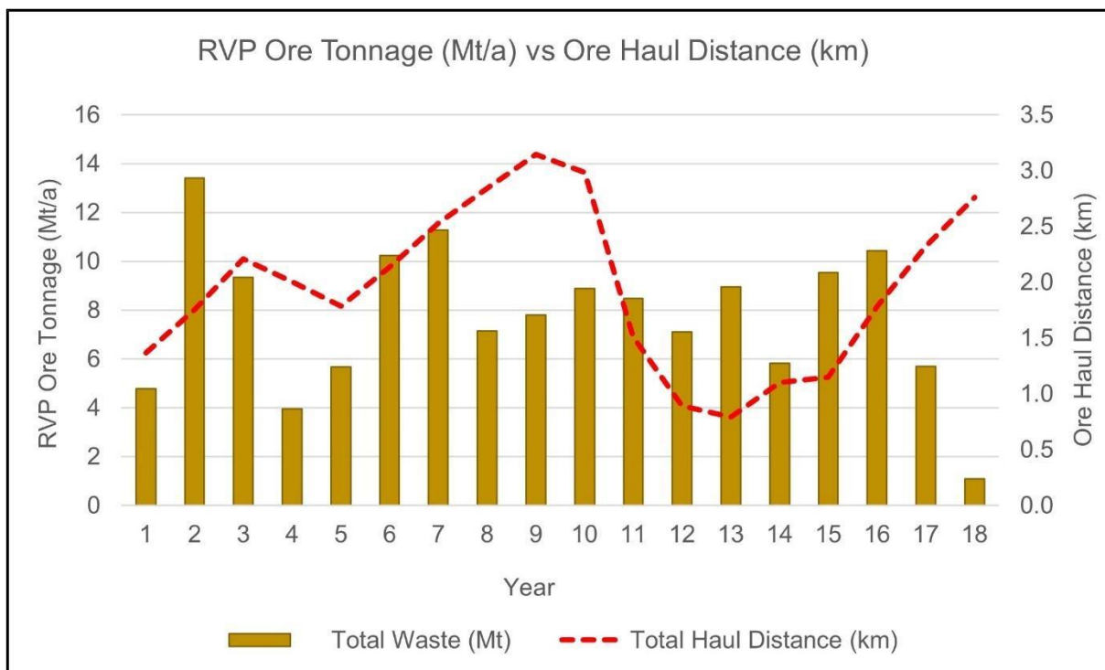
Figure 16.28: Weight Averaged One-Way Haul Distances – Total Mine Ore
