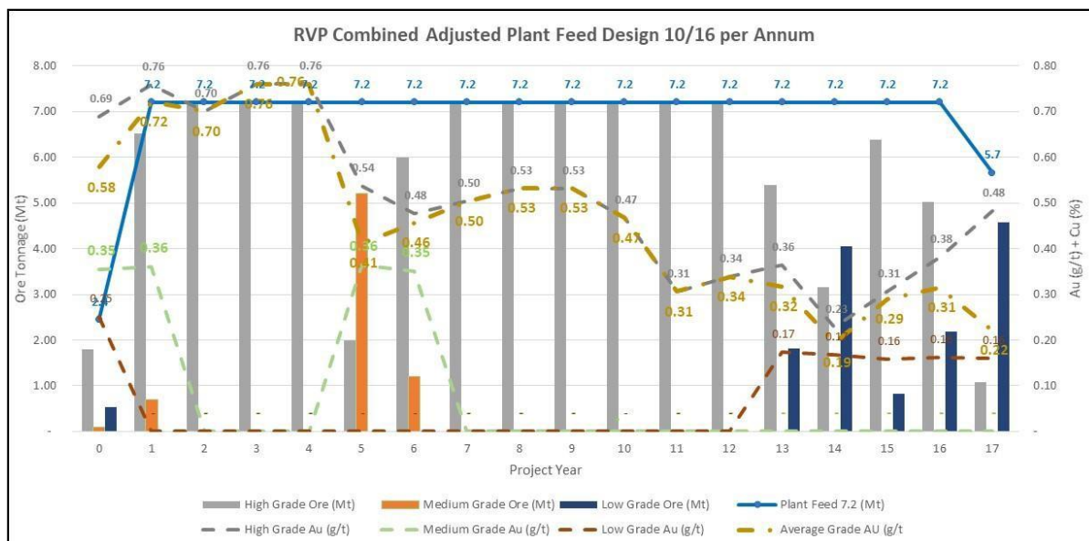
Figure 16.12: RVP Combined Plant Feed per Annum
