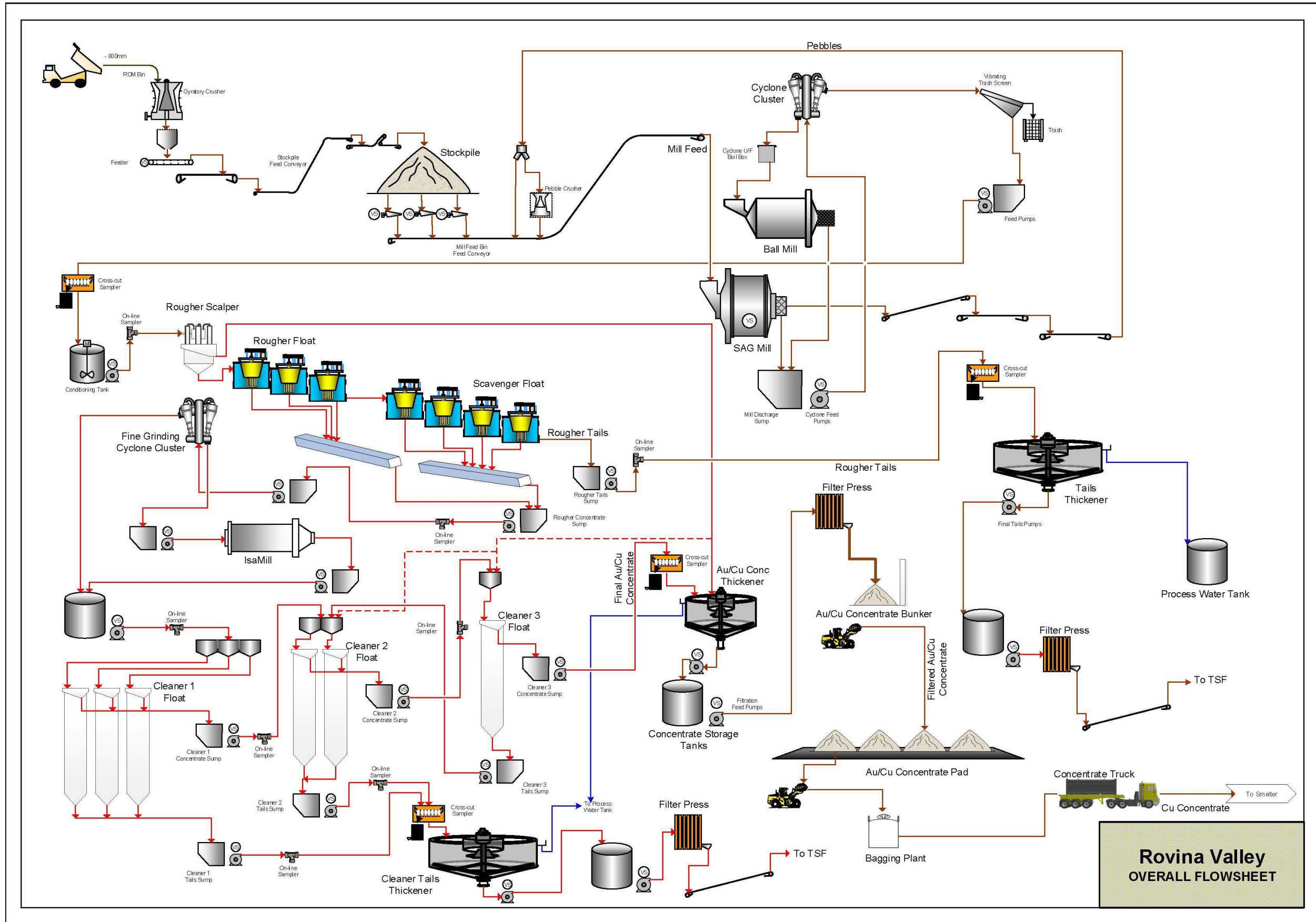
Figure 17.1: Process Flowsheet
