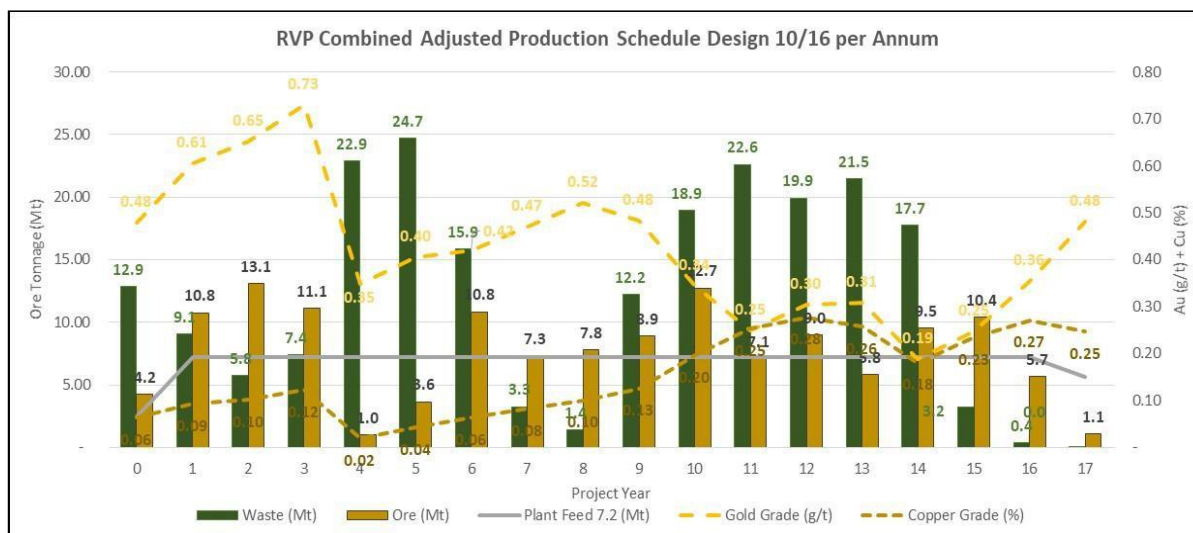
Figure 16.11: RVP Combined Production Schedule per Annum
