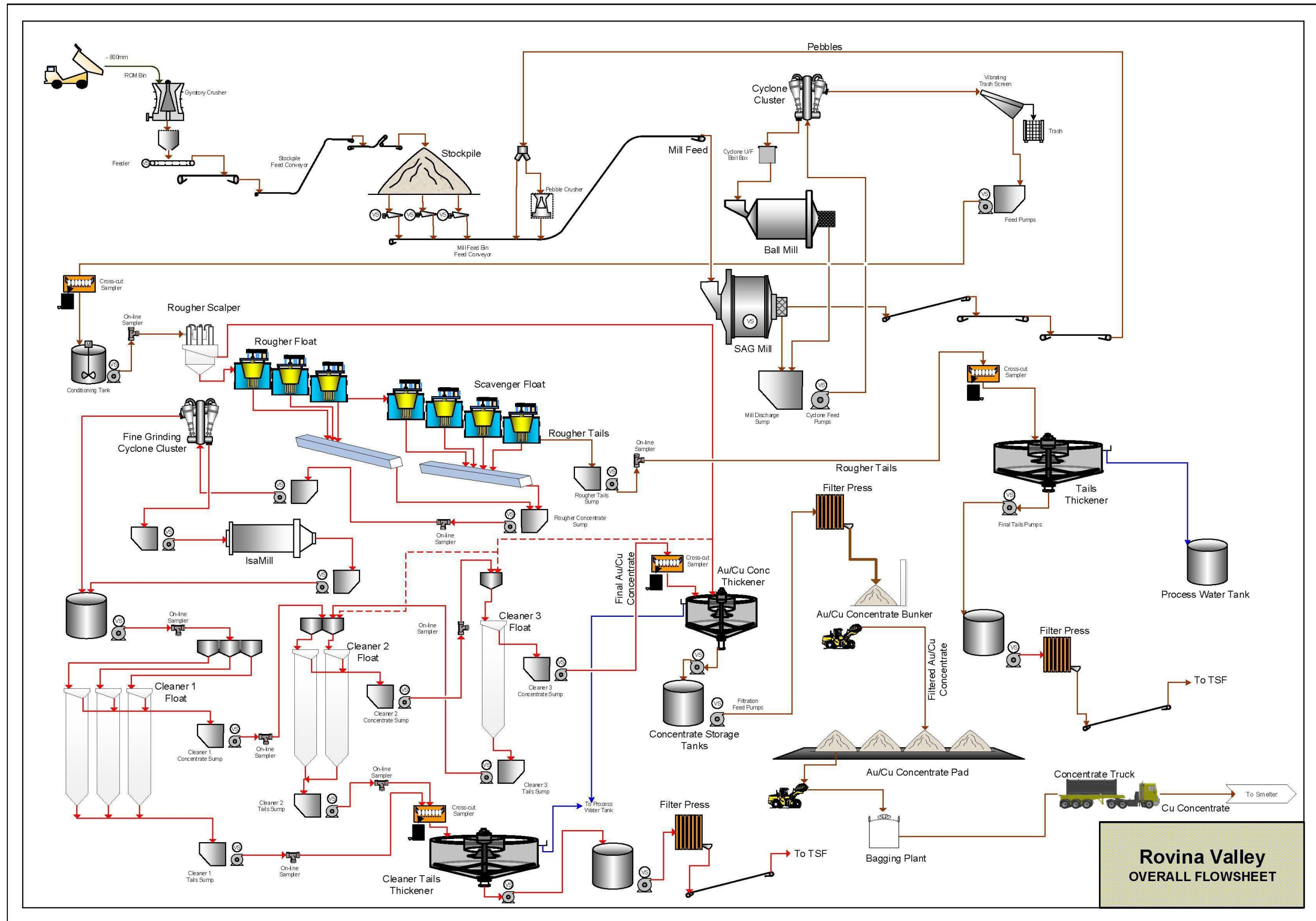
Figure 1.11: Process Flowsheet
