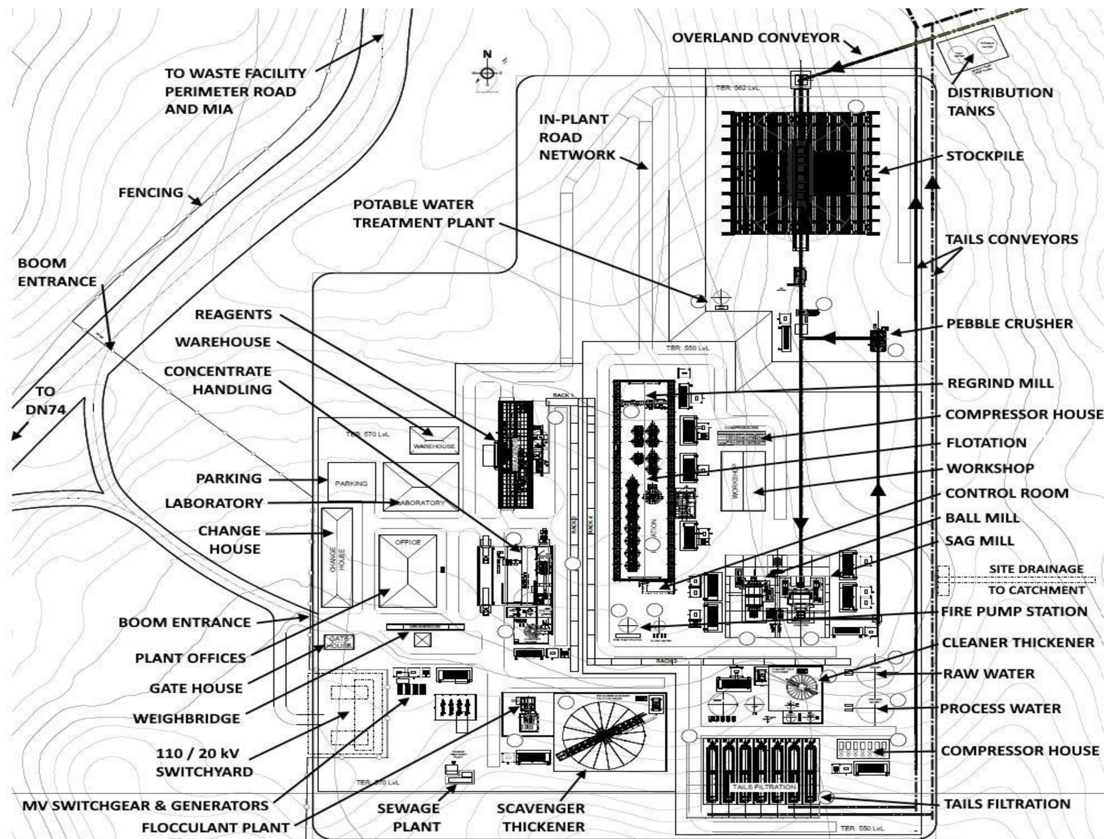
Figure 17.2: Process Plant General Arrangement
