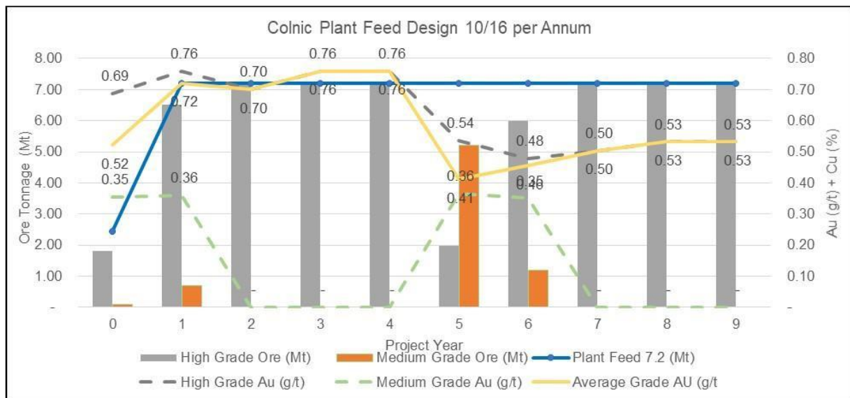
Figure 16.14: Colnic Plant Feed Design per Annum
