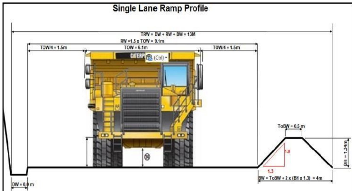
Figure 16.25: Single-Lane Ramp Profile
