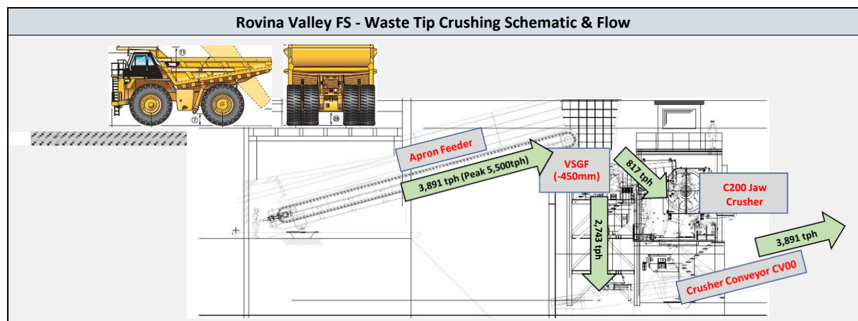
Figure 1.9: Waste Crusher GA and Flow
