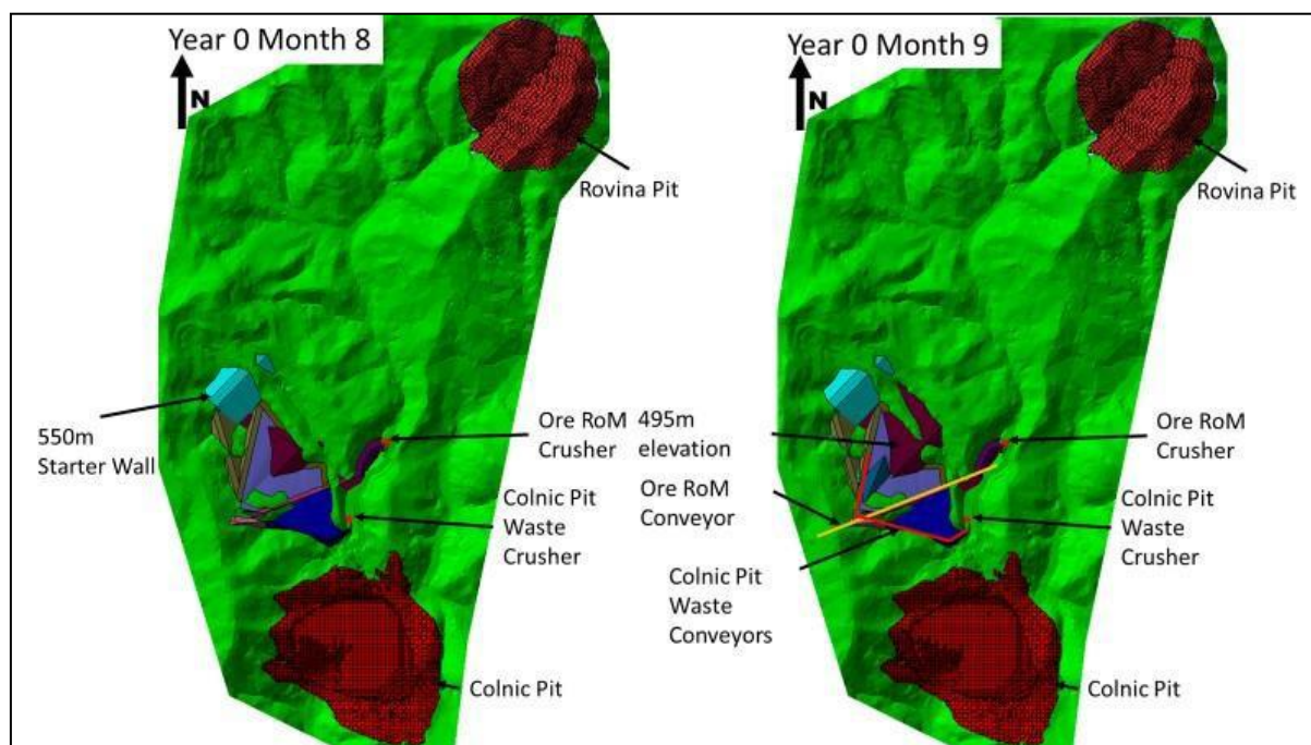
Figure 16.33: Co-Disposal Facilities (Year 0 – Months 8 and 9)
