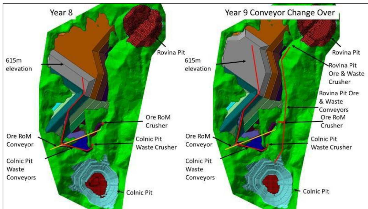
Figure 16.39: Co-Disposal Facilities (Years 8 and 9)
