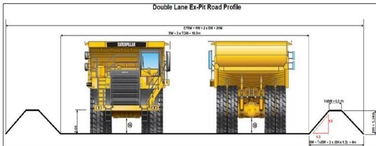
Figure 16.26: Double-Lane Ex-Pit Road Profile
