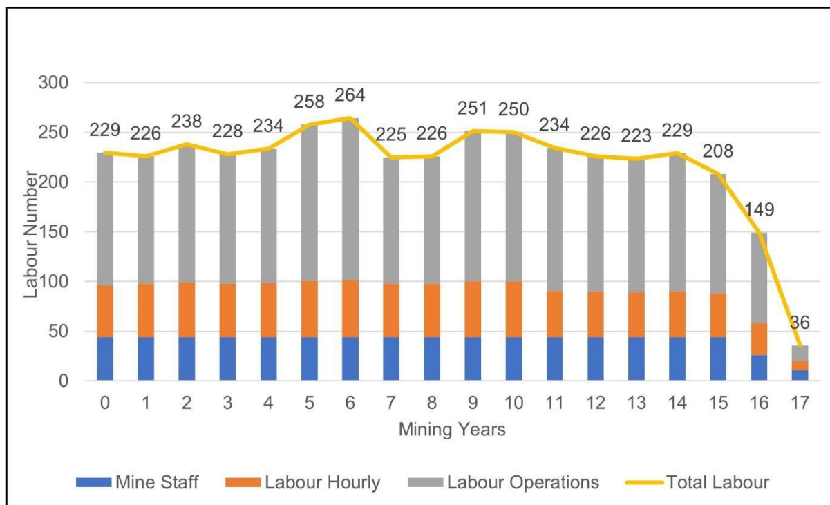
Figure 21.3: Mining Labour Complement per Annum
