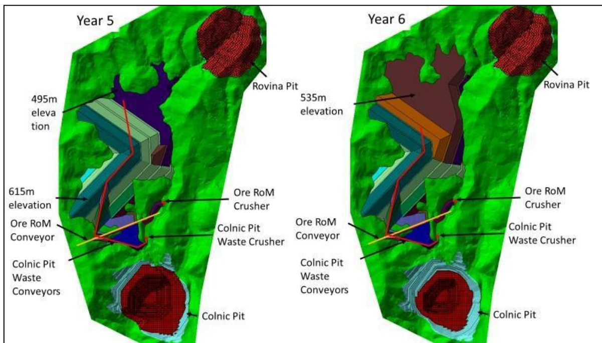
Figure 16.37: Co-Disposal Facilities (Years 5 and 6)
