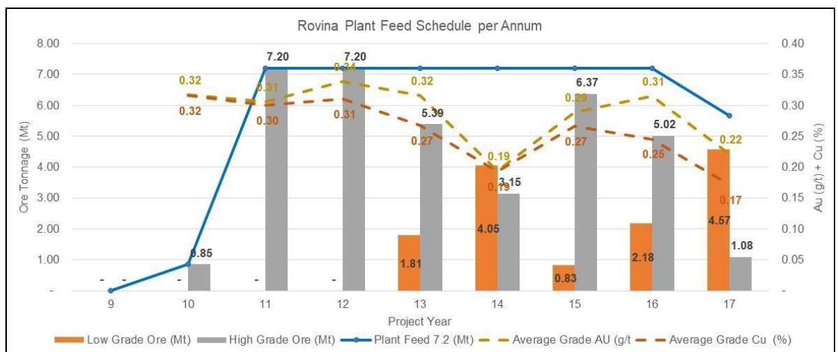
Figure 16.16: Rovina Plant Feed per Annum
