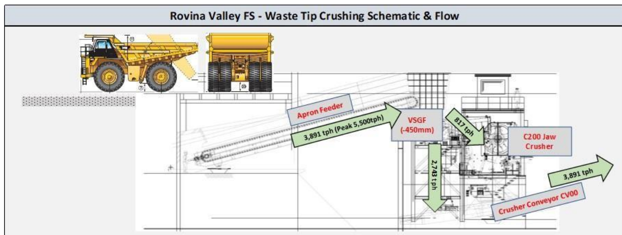
Figure 16.44: Waste Crusher GA and Flow
