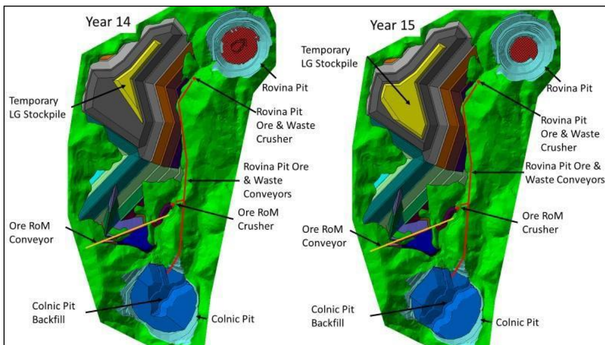
Figure 16.42: Co-Disposal Facilities (Years 14 and 15)
