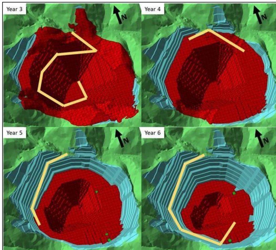
Figure 16.18: Colnic Pit (End of Year 3 to End of Year 6)
