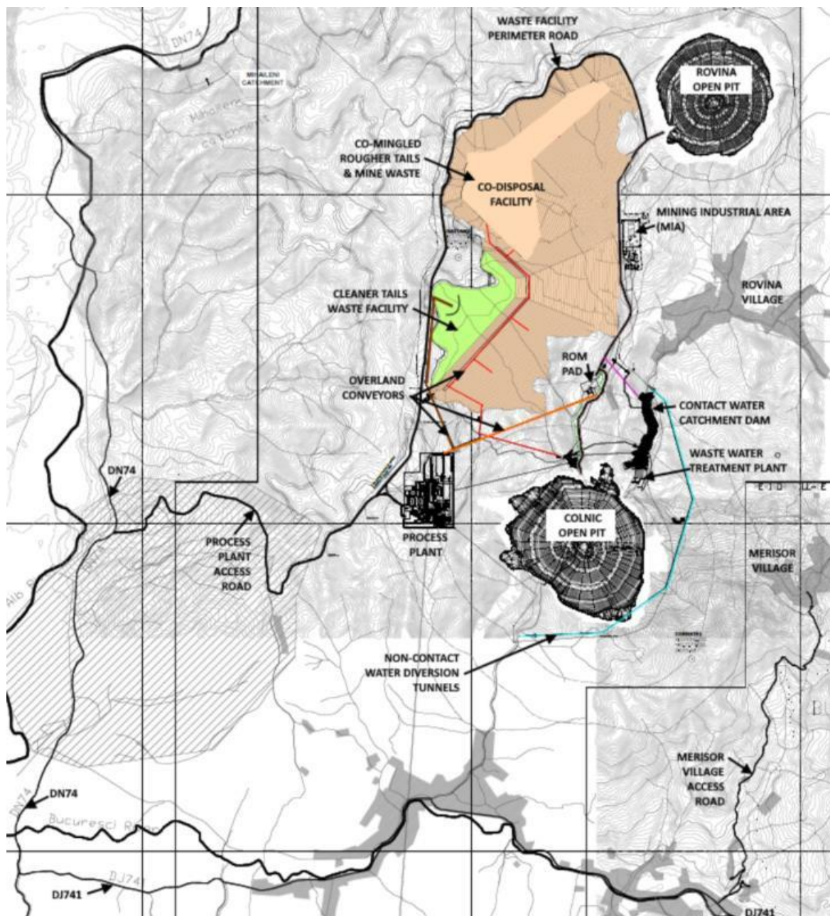
Figure 20.1: RVP Area of Influence and Infrastructure
