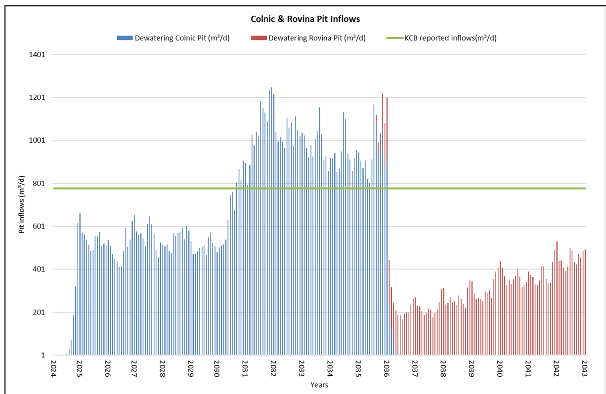
Figure 16.46: Colnic and Rovina Pit Inflows
