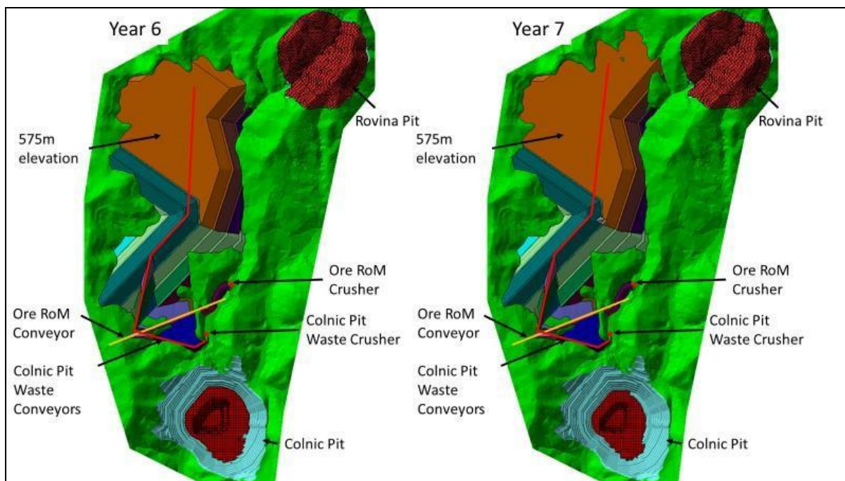
Figure 16.38: Co-Disposal Facilities (Years 6 and 7)
