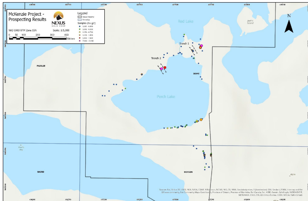
Figure 34: Plan map of 2019 and 2021 prospecting sample locations and Au values
