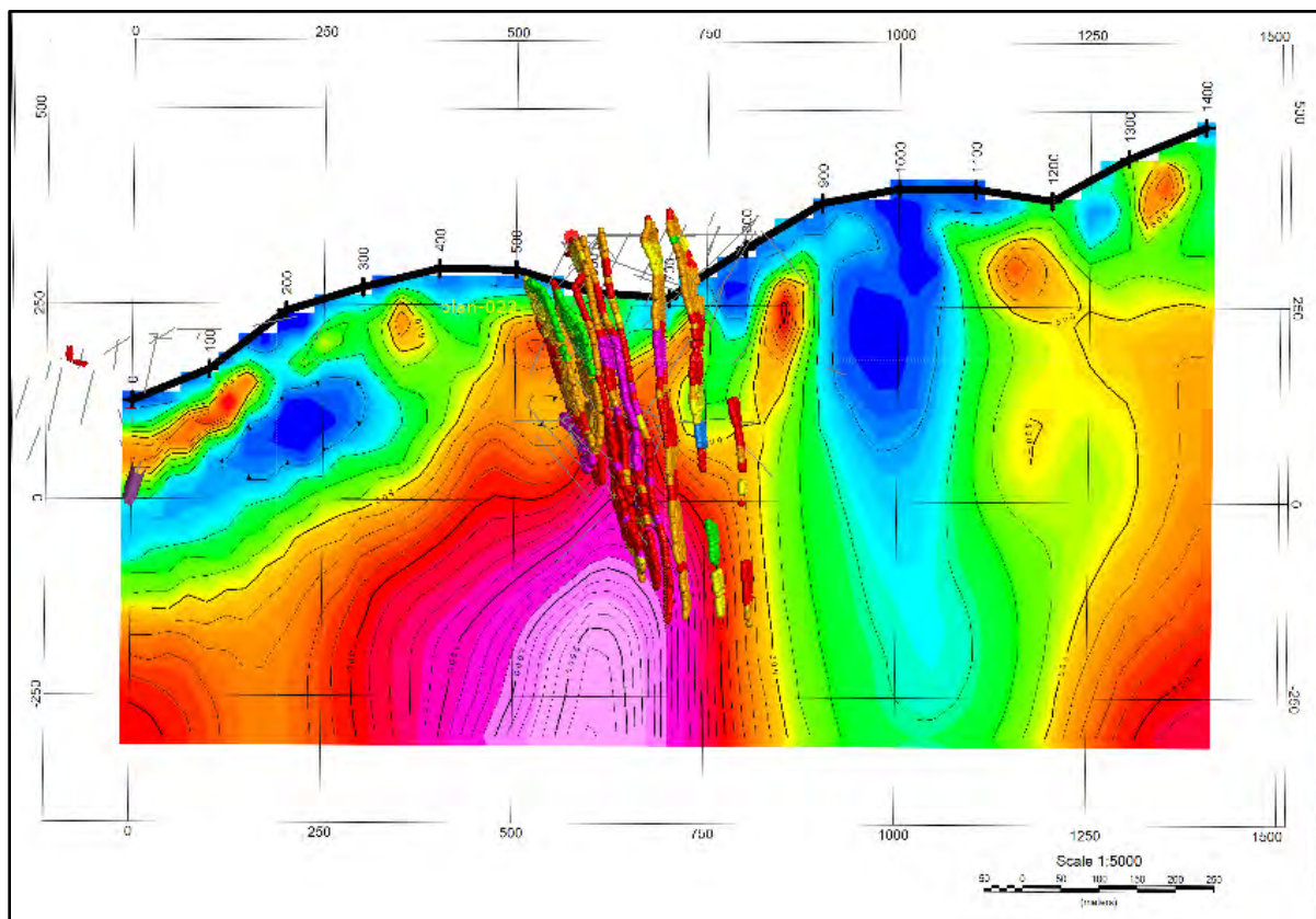
Figure 9-42: CSAMT section through the southern part of the Tuvatu mineralization-system (view north). The block model of veins is shown in the foreground, and the resistivity high is footwall to the main Tuvatu Lodes.
