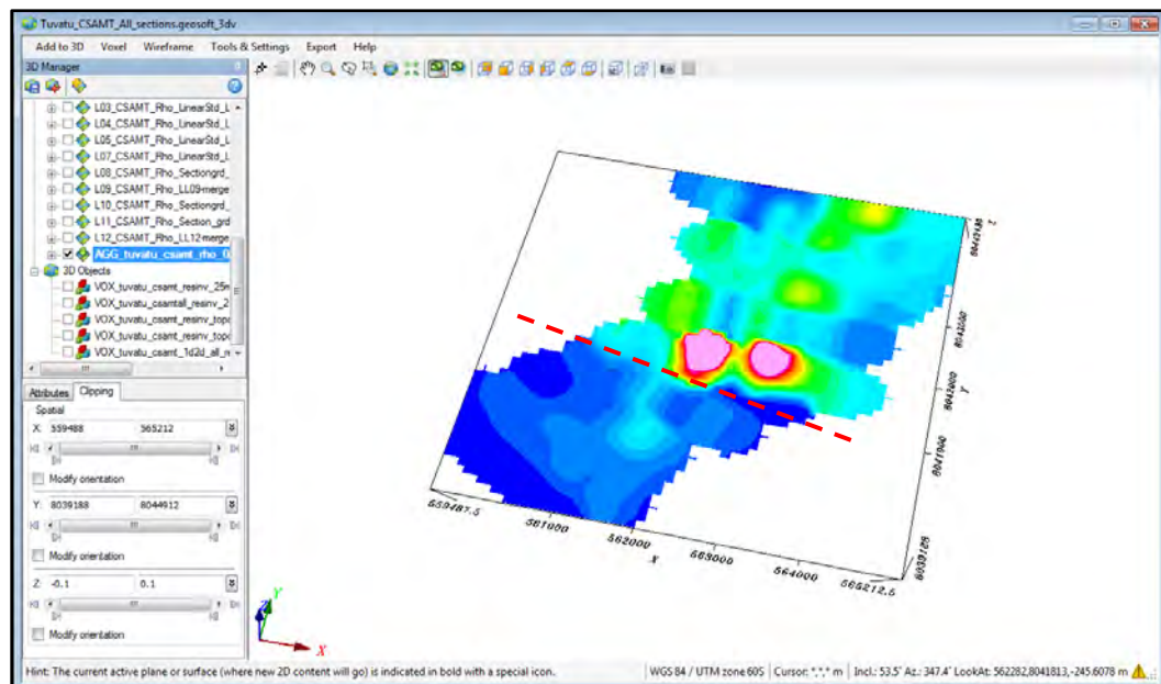
Figure 9-46: The 0 m resistivity elevation slice with clipped voxel removed
