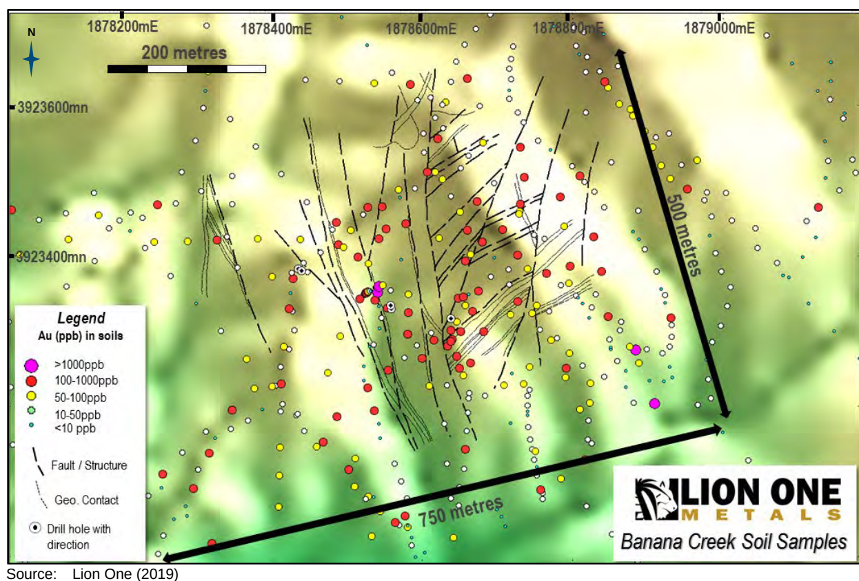
Figure 9-59: Historic soil sampling results from Banana Creek
