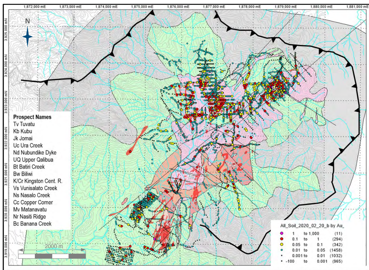
Figure 9-8: Soil samples at the Tuvatu Gold Project
