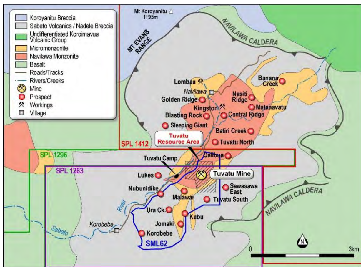
Figure 7-2: Project geology
