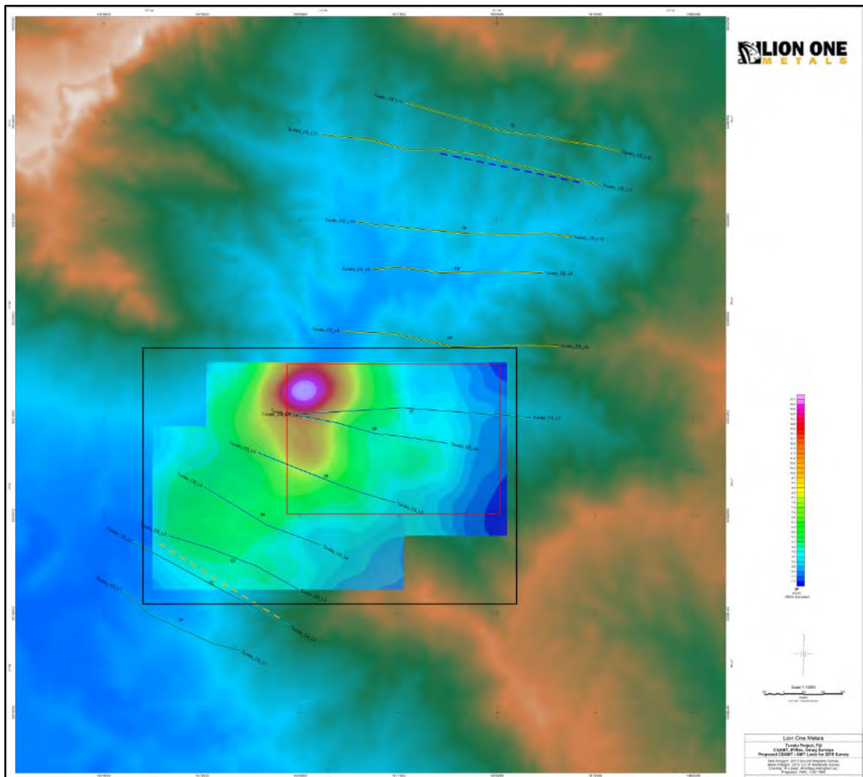
Figure 9-28: An index map showing the planned 2019 CSAMT line locations, the 2012 3-D IP/resistivity polygon (black), and the 2012 ground magnetic survey polygon (red). Data is plotted on digital topographic grid.
