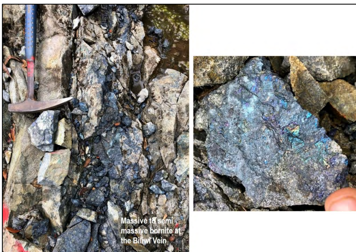
Figure 9-57: Massive to semi-massive bornite at the Biliwi Vein
