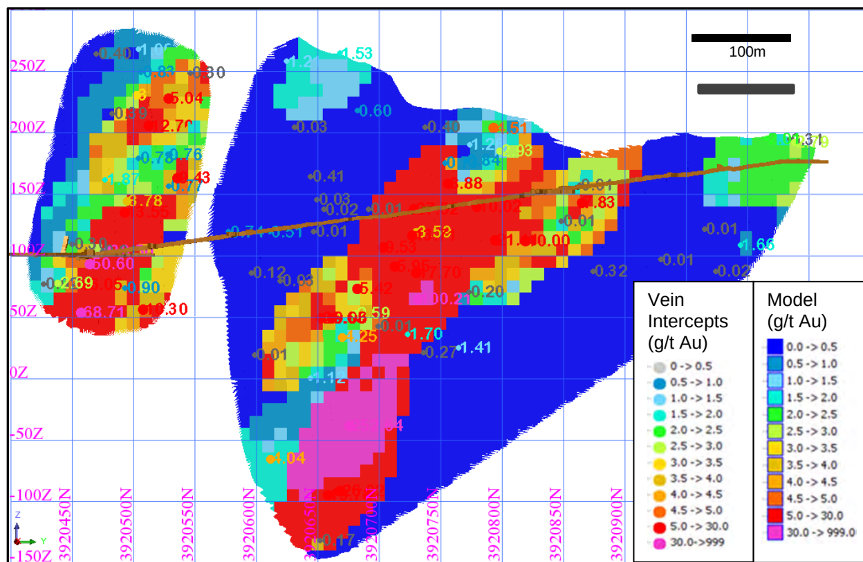
Figure 14-3: URW1 and URW1a estimated gold (long section view)
