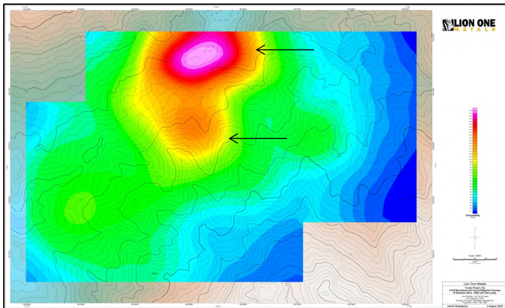
Figure 9-40: The Tuvatu IP -300 m elevation slice. The high IP responses of interest are indicated by the black arrows.
