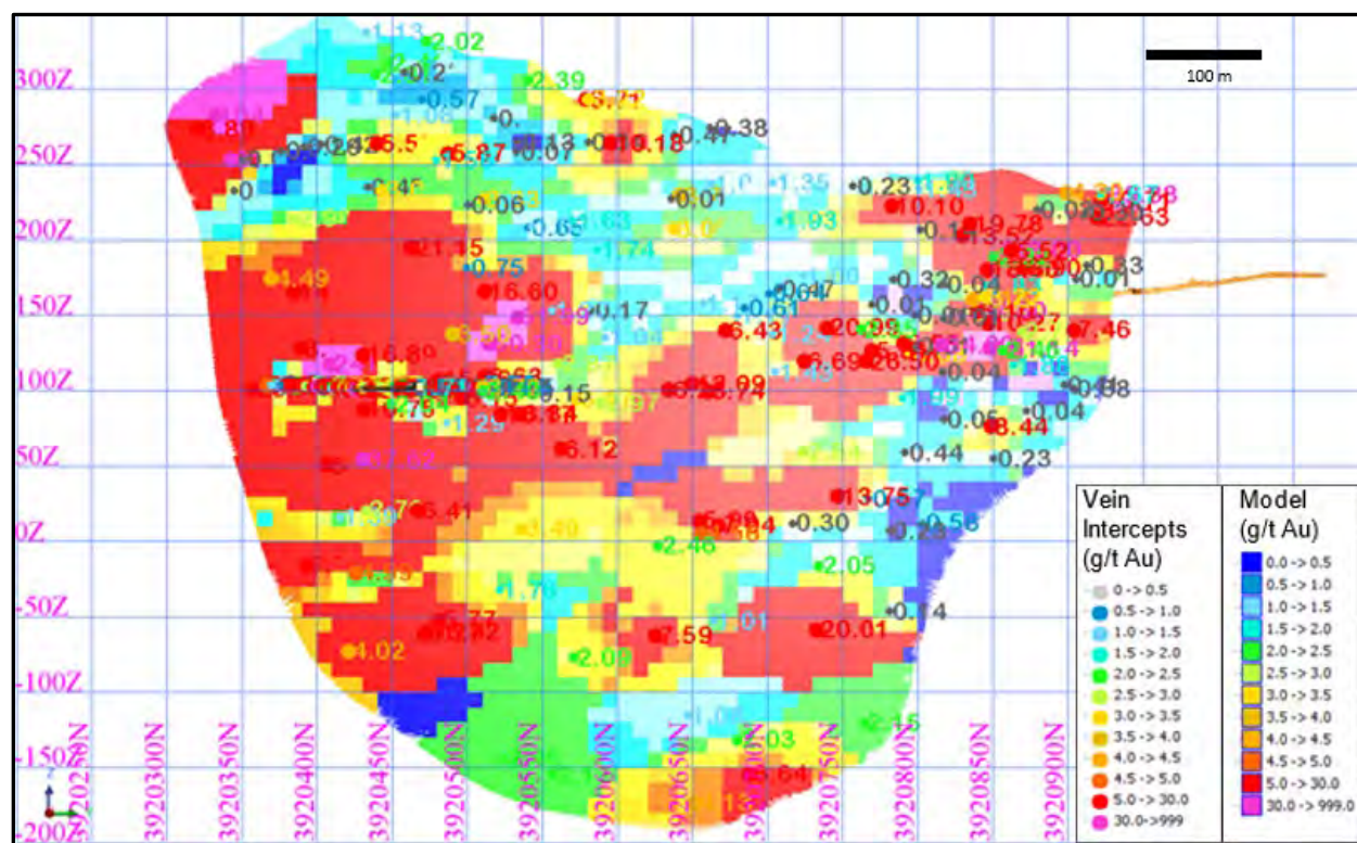
Figure 14-2: UR2 estimated gold (long section view)
