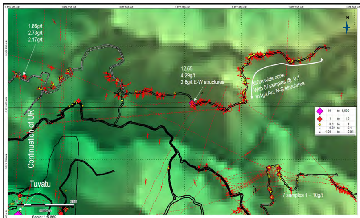
Figure 9-70: Upper Qalibua benching by gold with structures
