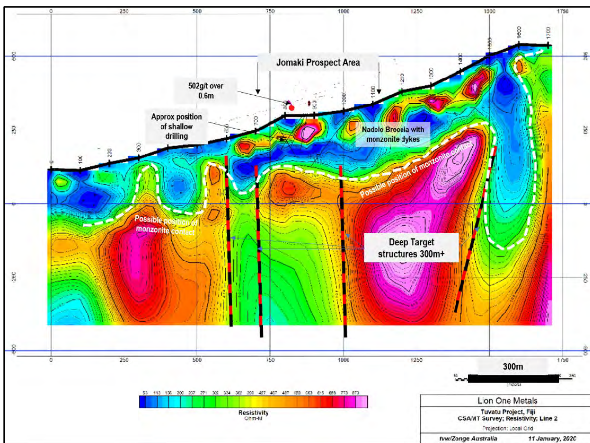
Figure 9-69: Jomaki CSAMT showing targets at depth
