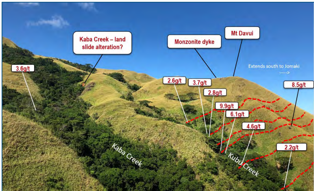
Figure 9-67: Illustration of terrain at the Kubu Prospect area with rock sampling
