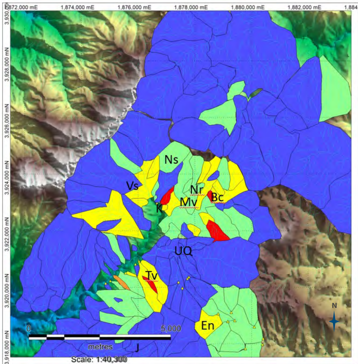
Figure 9-24: Lead in cBLEG stream survey samples
