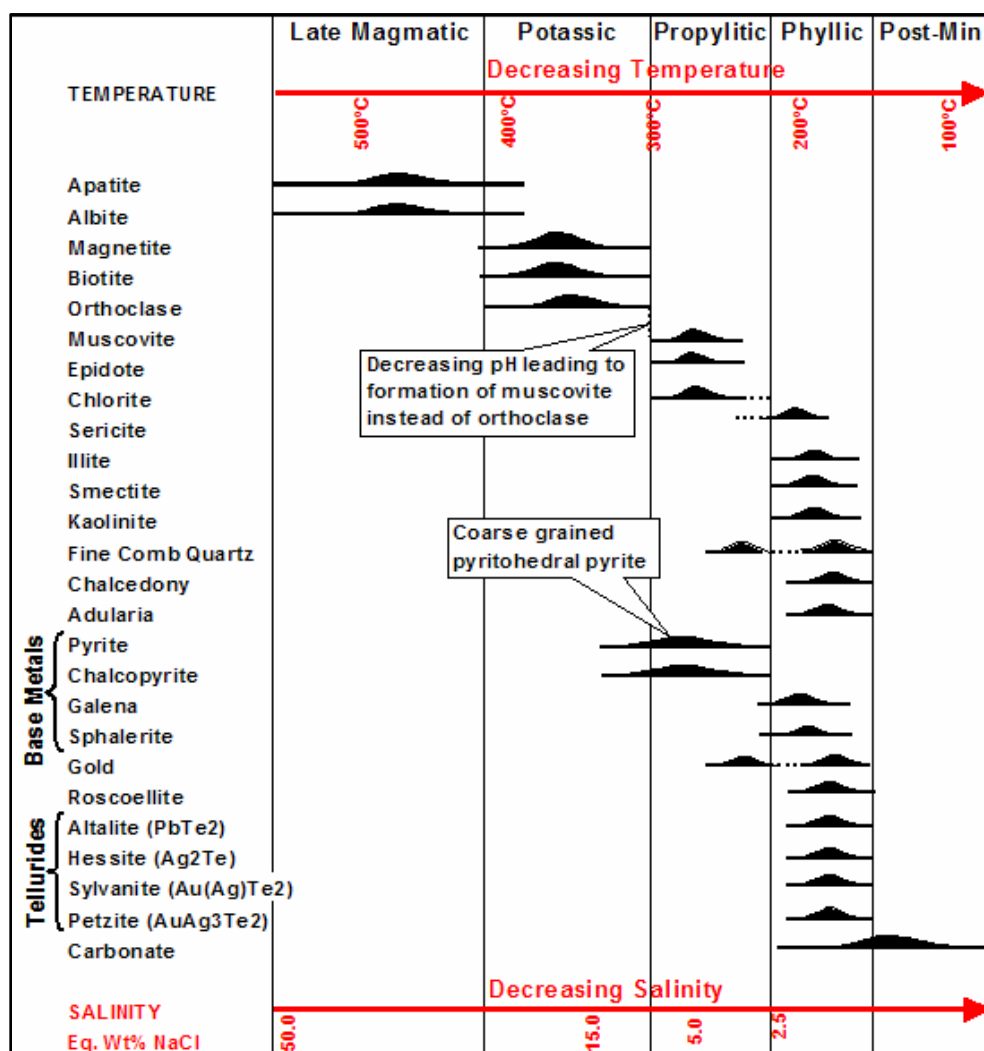
Figure 7-9 Paragenesis of mineralization
