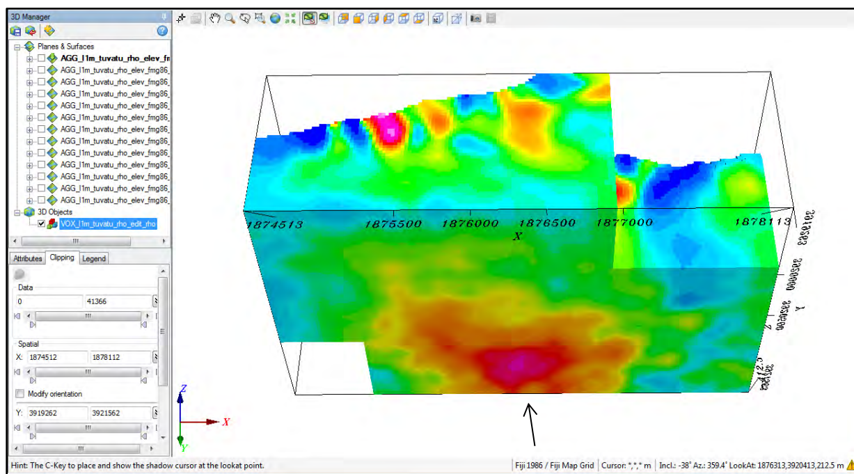
Figure 9-31: The 3-D resistivity voxel viewed up and to the north. Note the deep high resistivity zone located at the north end of the survey block (colored red). The source of this resistivity high is interpreted to be an intrusive body.
