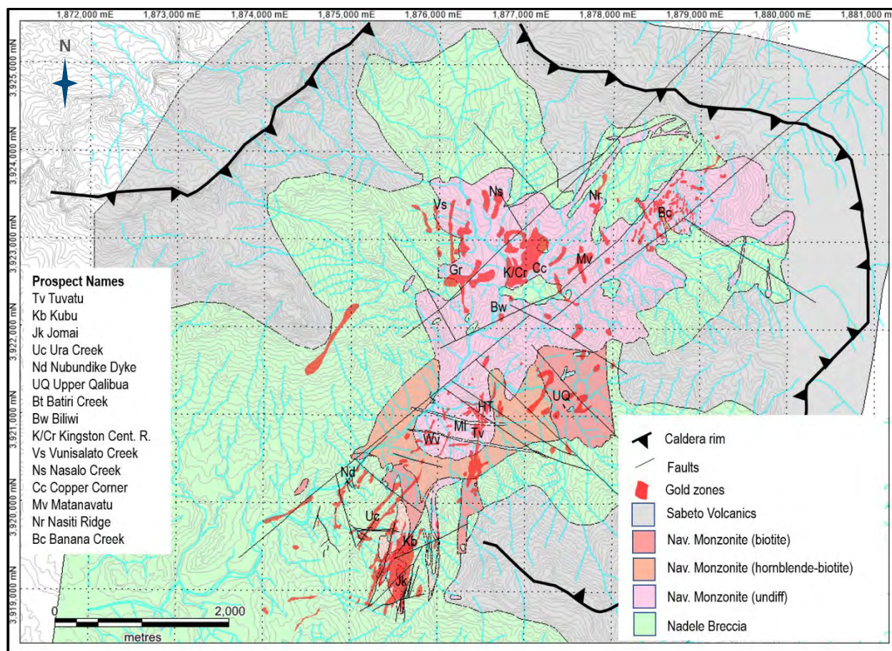
Figure 9-6: District geology map of the Navilawa Caldera
