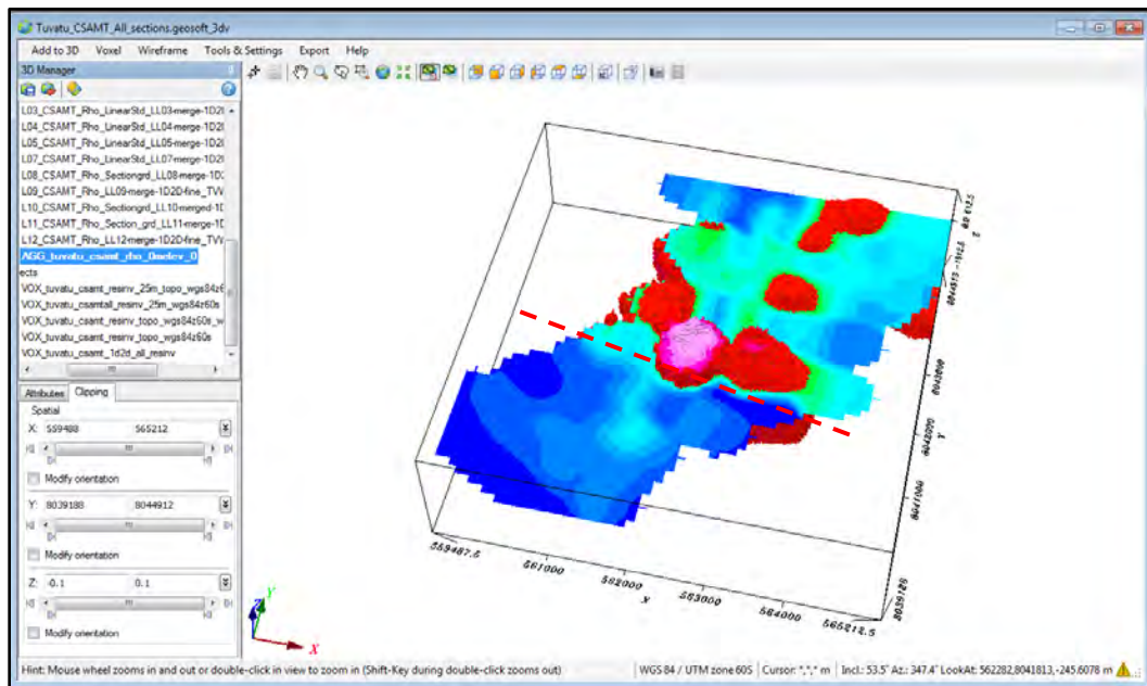
Figure 9-45: The 0 m resistivity elevation slice with the clipped ( \rho > 2500 ohm-m) voxel superimposed on top
