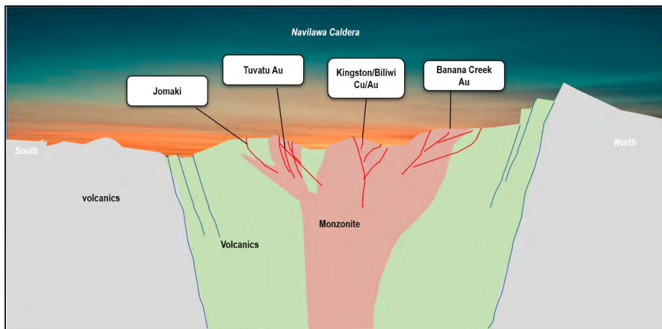
Figure 9-7: Schematic cross-section view west
