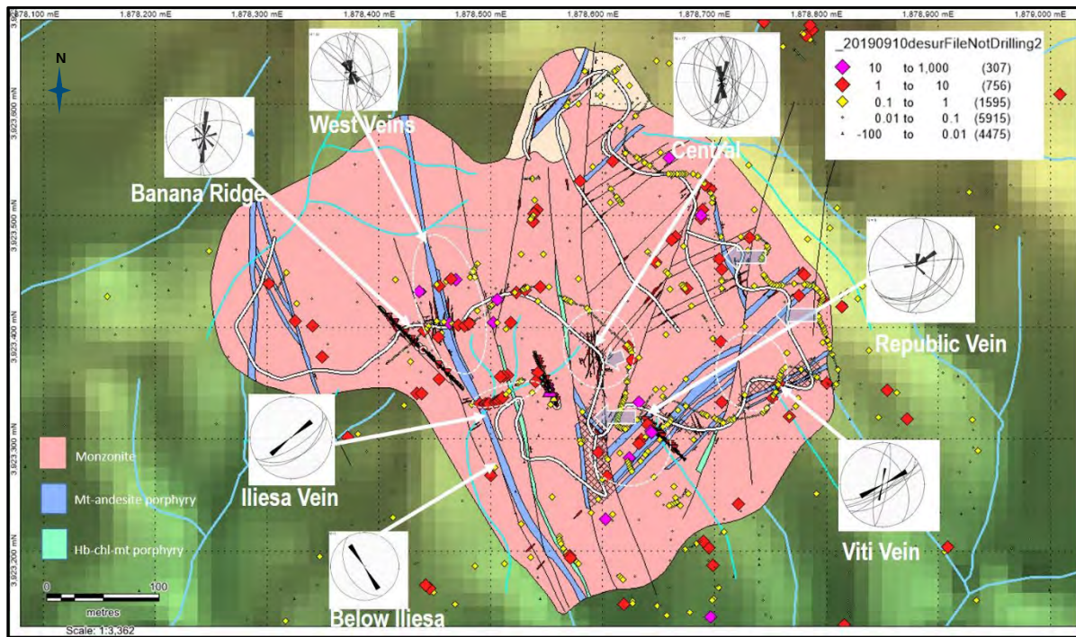
Figure 9-62: The Banana Creek Prospect with local scale geology map and major structures labeled. Historic rock and channel sampling grades show with diamond symbol insets are stereonets of Lion One mapping in the area.
