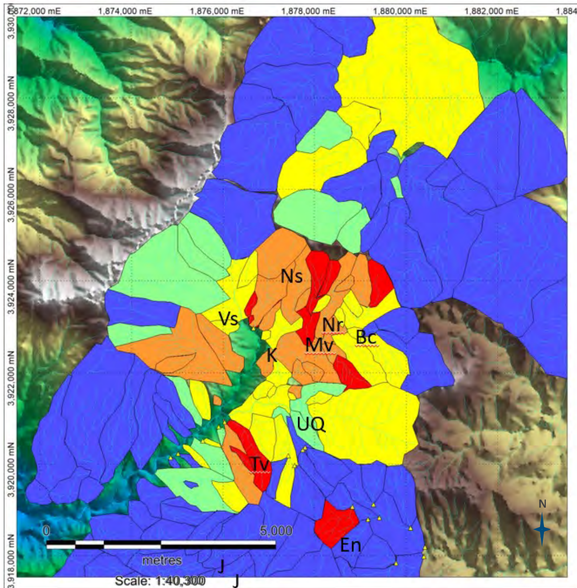
Figure 9-25: Tellurium in cBLEG stream survey samples
