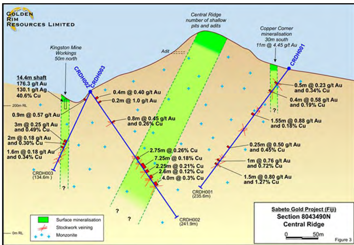
Figure 6-1: Drill hole cross-section showing significant intersection for holes drilled at Central Ridge
