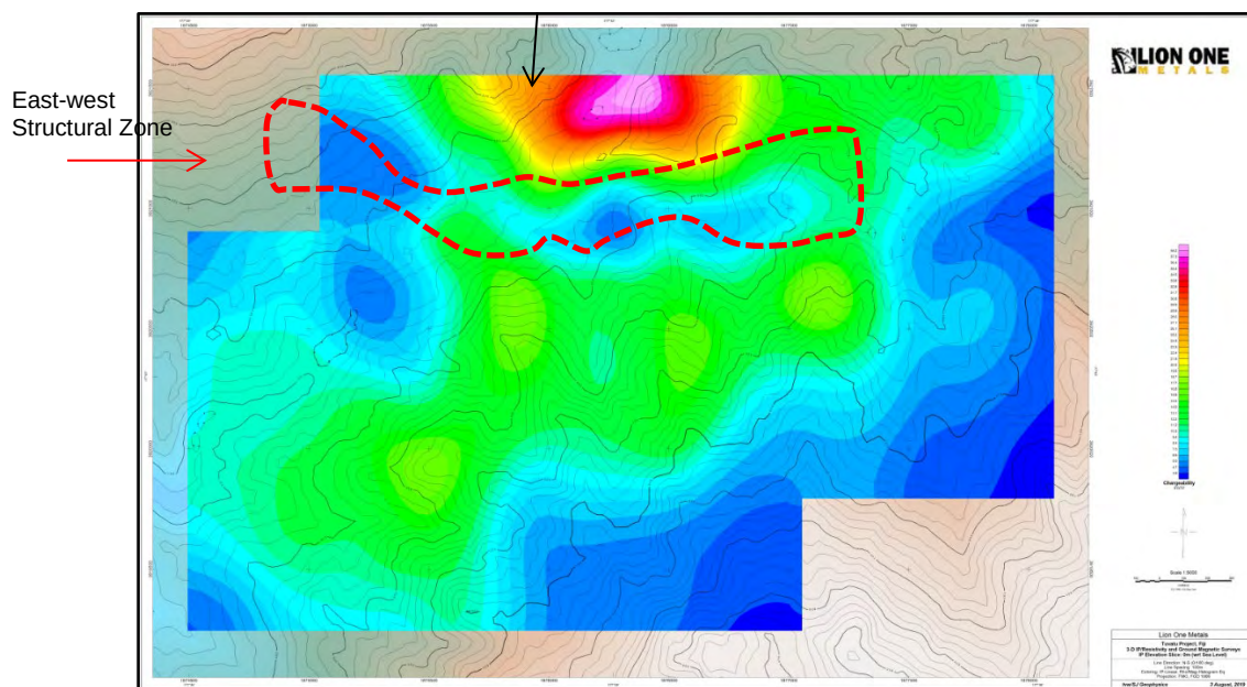
Figure 9-38: The Tuvatu IP 0 m elevation slice. The high IP response of interest is indicated by the black arrow. The east-west trending IP low (red dashed shape) is coincident with the east-west trending structural zone shown in Figure 9-39 (below).
