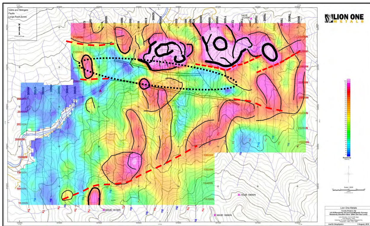
Figure 9-35: The MHG overlay plotted on top of the +200 m resistivity elevation slice and interpretation with the survey line / drill hole and topography as a base
