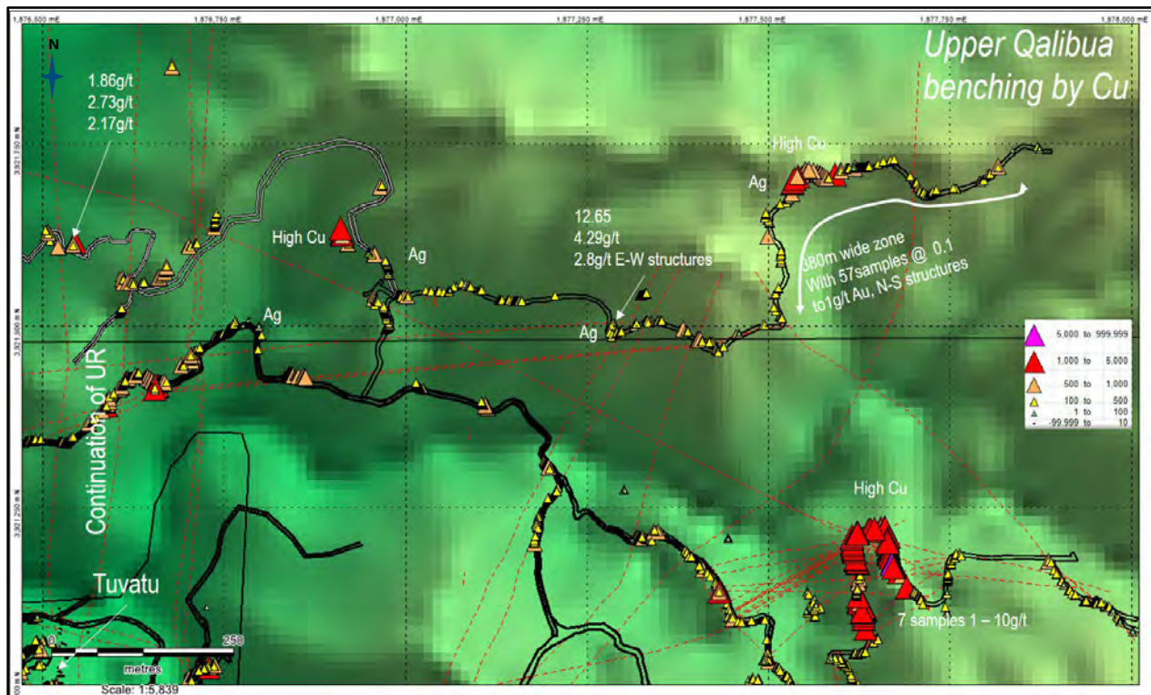
Figure 9-71: Upper Qalibua benching by copper (with gold grades labelled)
