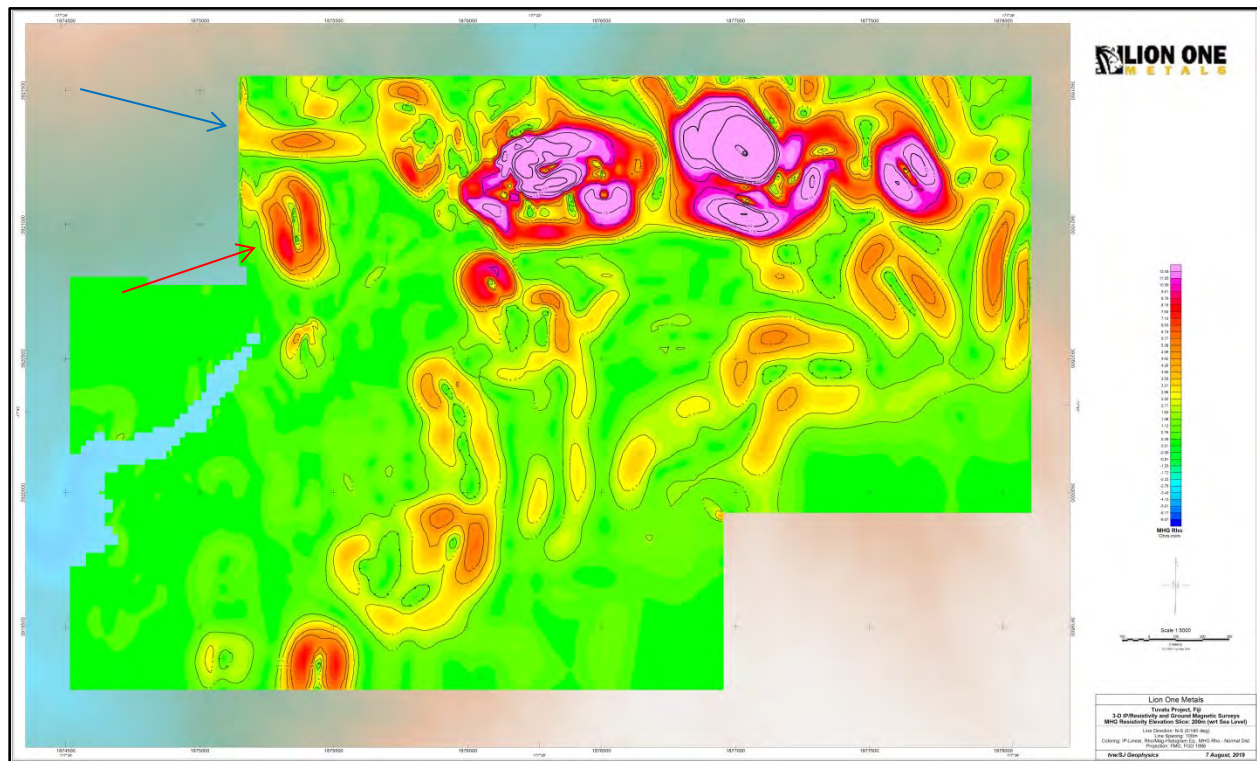
Figure 9-33: The MHG for the 200 m elevation slice. This systematically identifies the edges of bodies. Single MHG high features are contacts or structures (example blue arrow). Circular, closed, donut-like features are the edges of individual intrusive-like bodies (example red arrow). There are numerous features that are somewhere in between.
