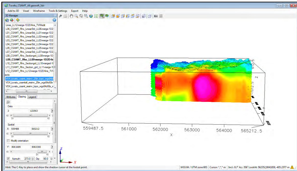
Figure 9-53: The Line 9, 2-D inversion section is not shown. The detailed high resistivity features are not present in the 3-D voxel display.
