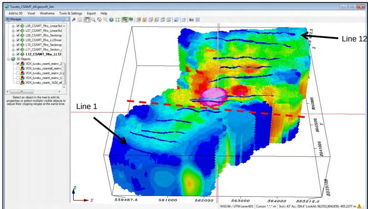
Figure 9-44: The Tuvatu 3-D resistivity voxel display of the combined 2-D inversion models. Line 1 is located on the south end of the survey block. Line 12 is located on the north end of the survey block with the remaining lines numbered sequentially from south to north. The red dashed line separates a zone of higher resistivity to the north and lower resistivity to the south.
