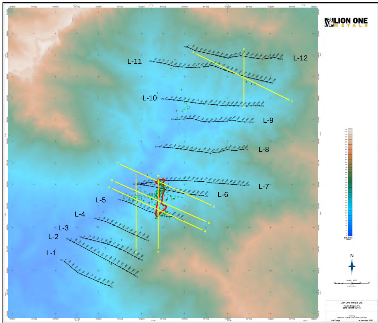
Figure 9-43: The Tuvatu CSAMT/AMT survey lines plotted on topography (Fiji Map Grid, FGD1986). The black lines with stations posted are the CSAMT lines in local coordinates. The red polygon is the approximate location of the deposit projected to the surface. The green circles are drill hole collar positions. The yellow lines are interpreted section lines from a company advisor (Quinton Hennigh).
