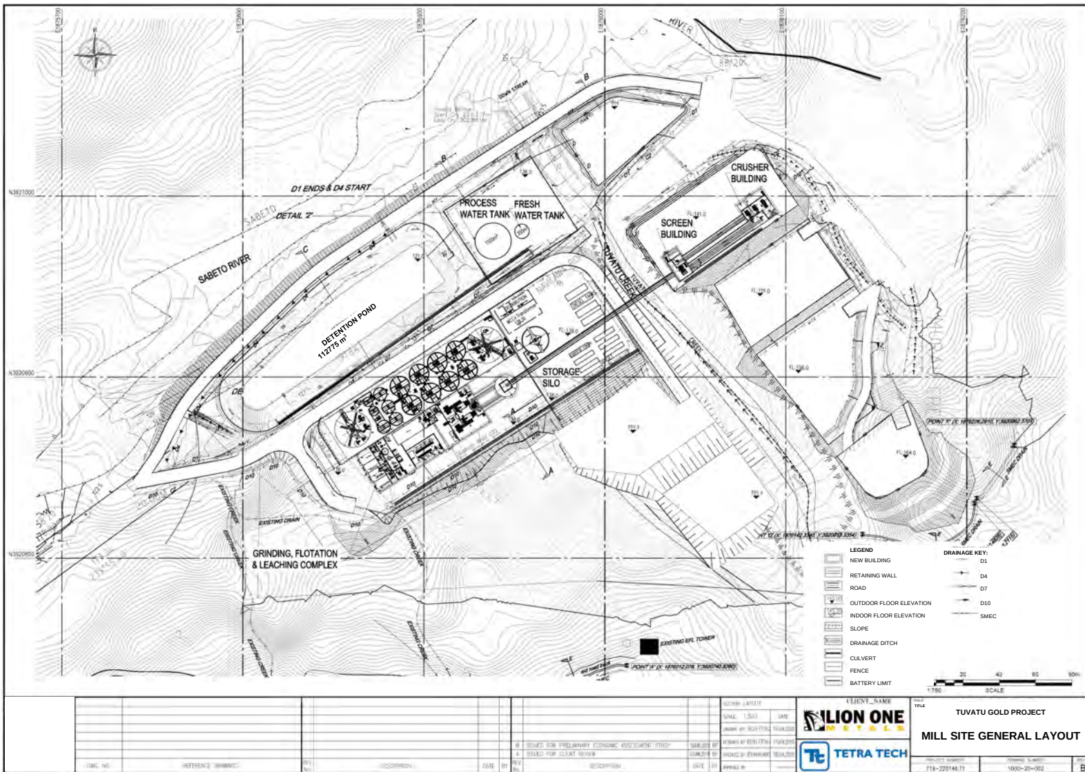
Figure 17-2: Mill layout
