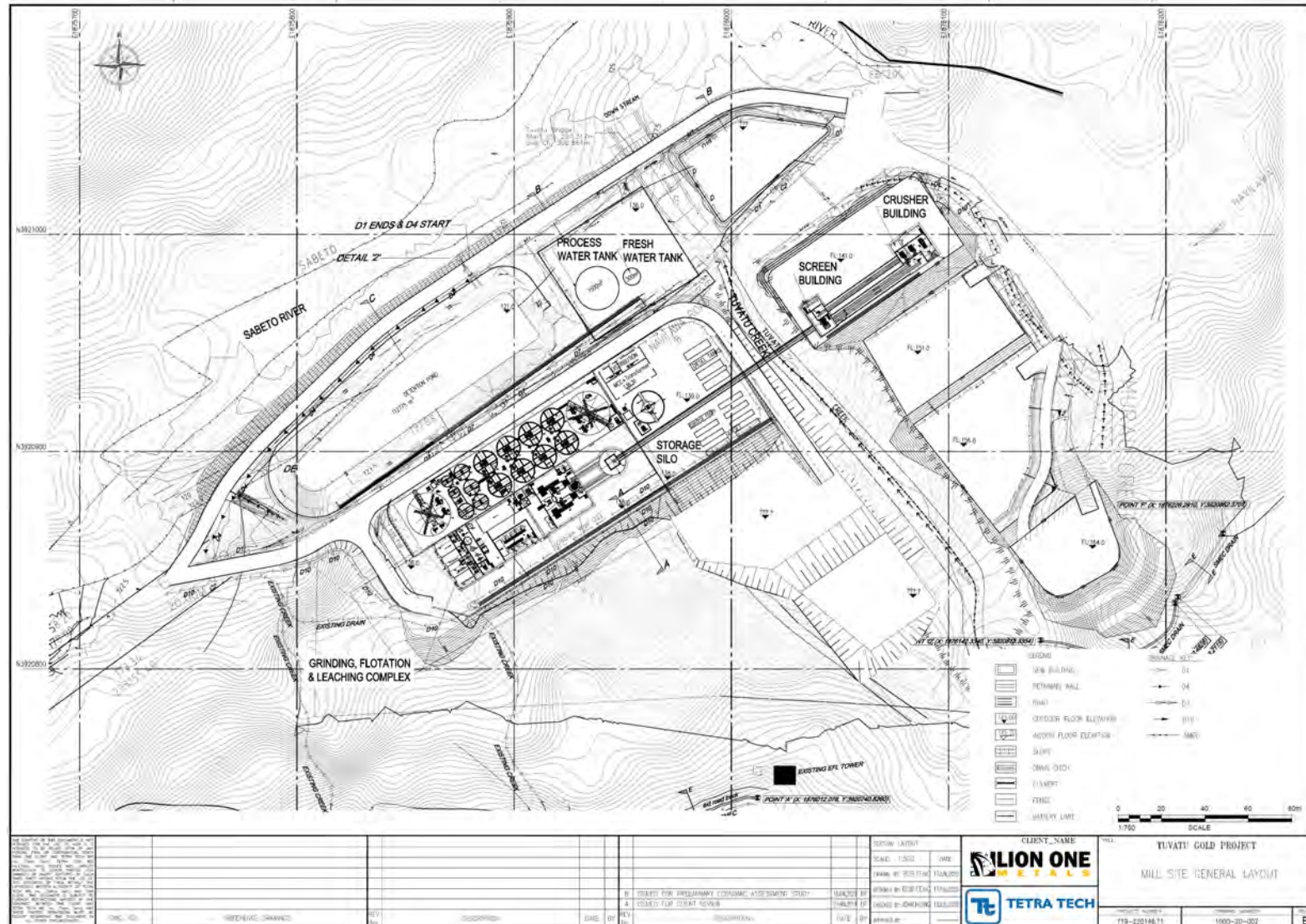
Figure 18-3: General plant site layout – plan view
