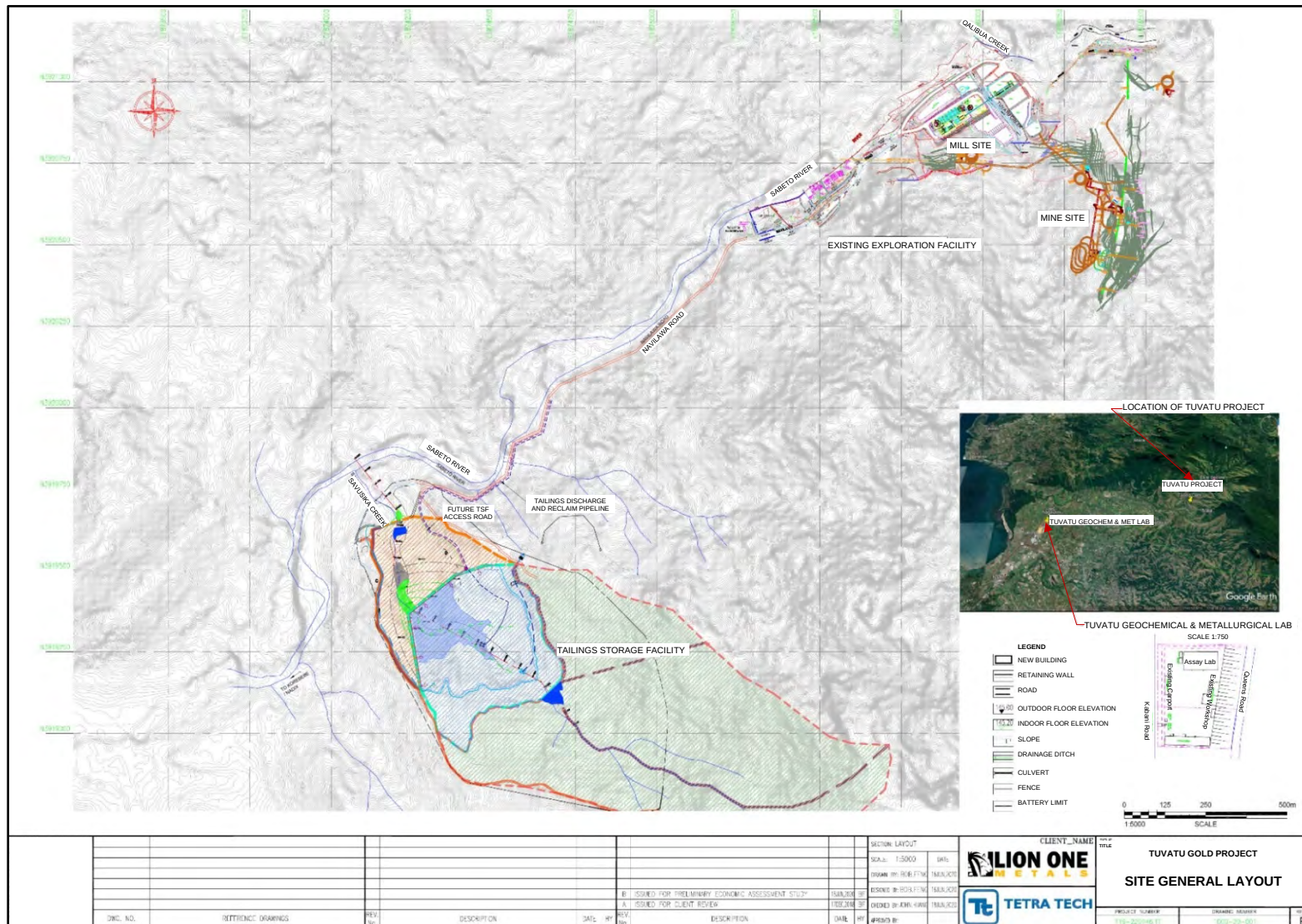
Figure 18-1: Overall Project site – plan view
