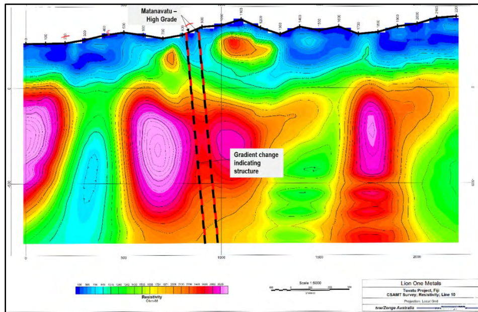
Figure 9-58: CSAMT section (view north) close to the Matanavatu high-grade structures exposed in benching
