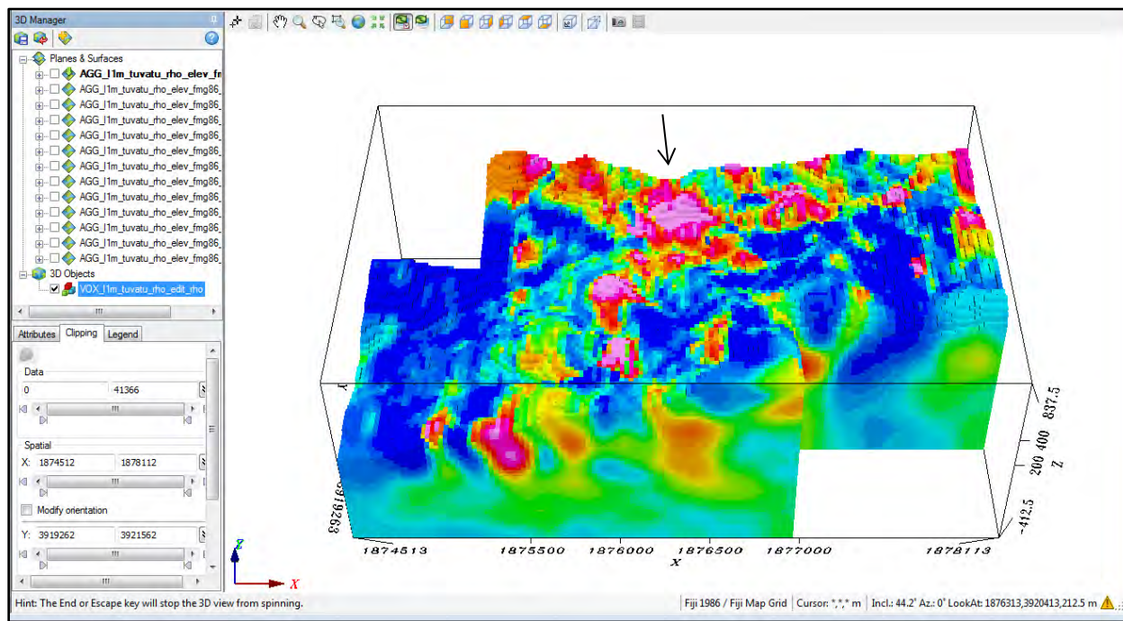
Figure 9-30: The 3-D resistivity voxel viewed down and to the north. Note the near surface resistivity highs located at the north end of the survey block (colored red). This 3D model is attached to this report as an ASCII file and can be entered into a 3D viewing package such as Vulcan or Leapfrog.
