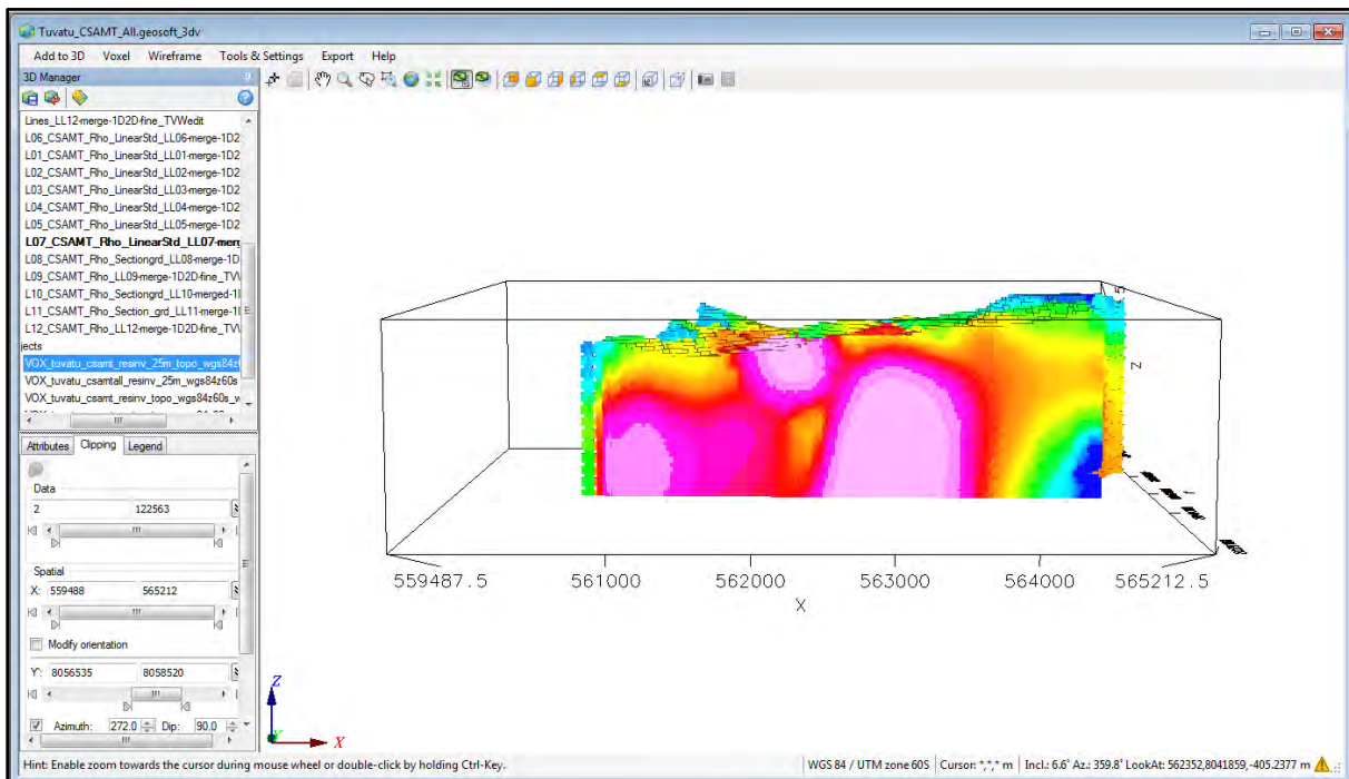
Figure 9-51: The Line 7, 2-D section is not shown. Compared with Figure 9-60, the added detail observed in the 2-D line is replicated in the 3-D model. It should also be noted that on Line 7, a major power line goes through the area resulting in noisy data that is highly edited. Two distinctly different models have been generated, which are shown below.
