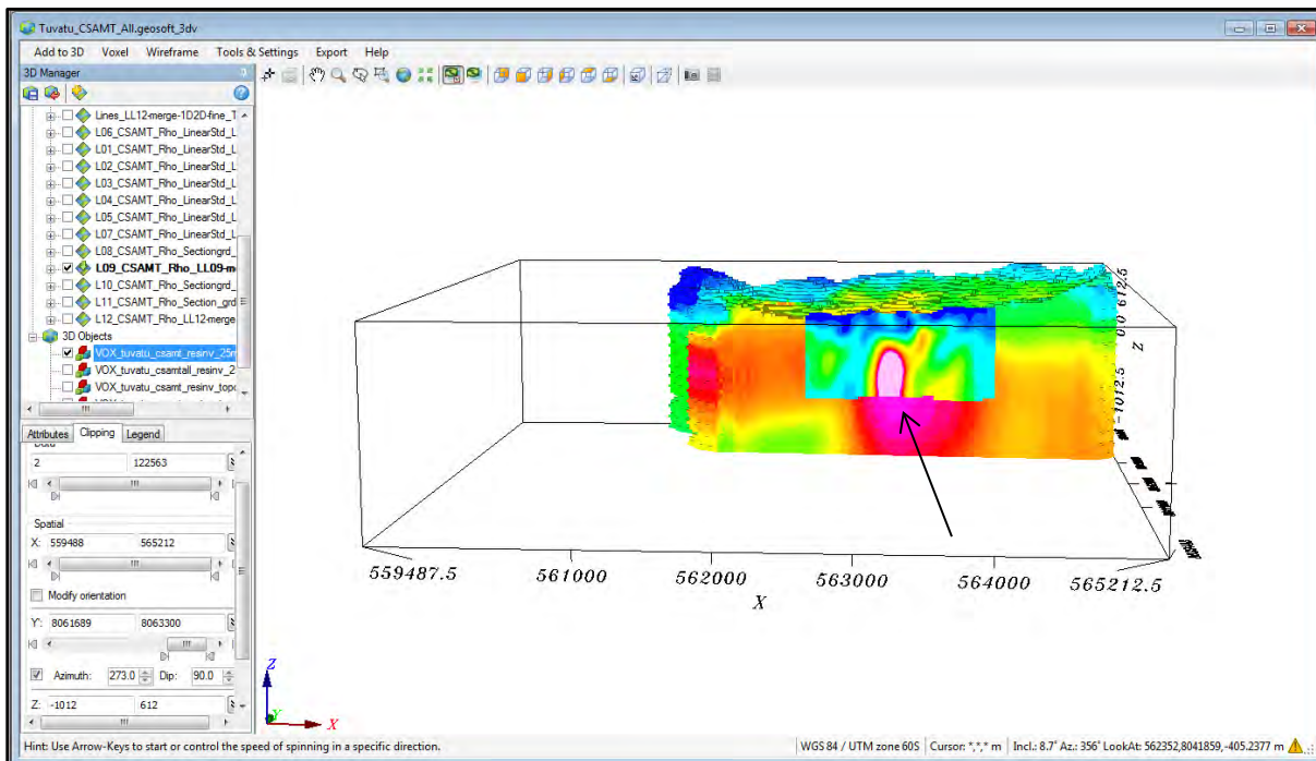
Figure 9-52: The Line 9, 2-D section is shown. Note the high resolution detail in the 2-D inversion section (see black arrow).
