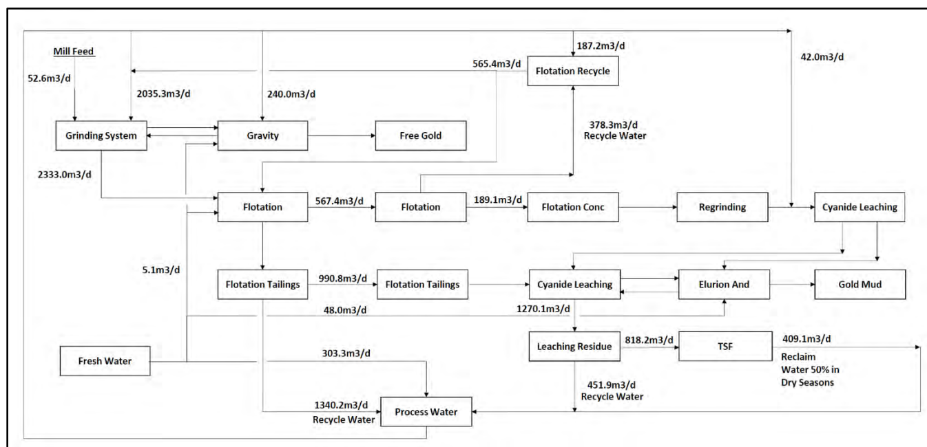
Figure 18-9: Process water balance block model
