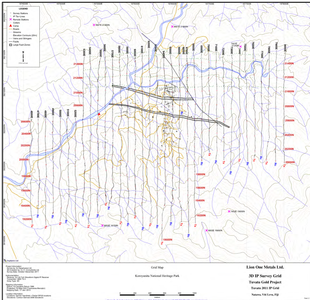
Figure 9-29: The IP/resistivity grid plotted on the topography with drill pattern and main structures indicated. The line spacing is approximately 100 m and stations are marked out every 25 m on the ground with potential electric measurements every 50 m.
