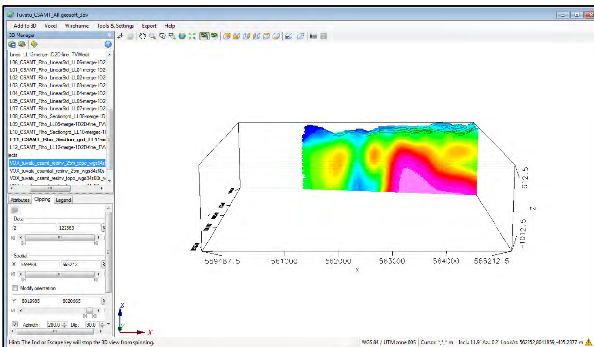
Figure 9-55: The Line 11, 2-D resistivity inversion section is not shown. The general shape of the 3-D voxel slice is similar to the 2-D inversion section, but the detail is missing.
