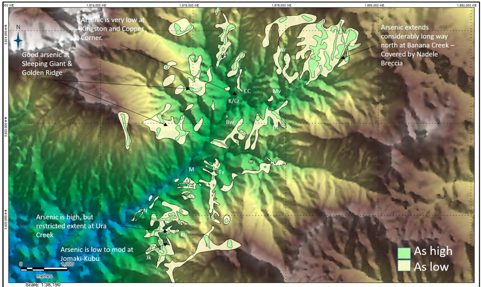
Figure 9-16: Regional analysis of arsenic mineralizing cells from a combination of surface sampling techniques
