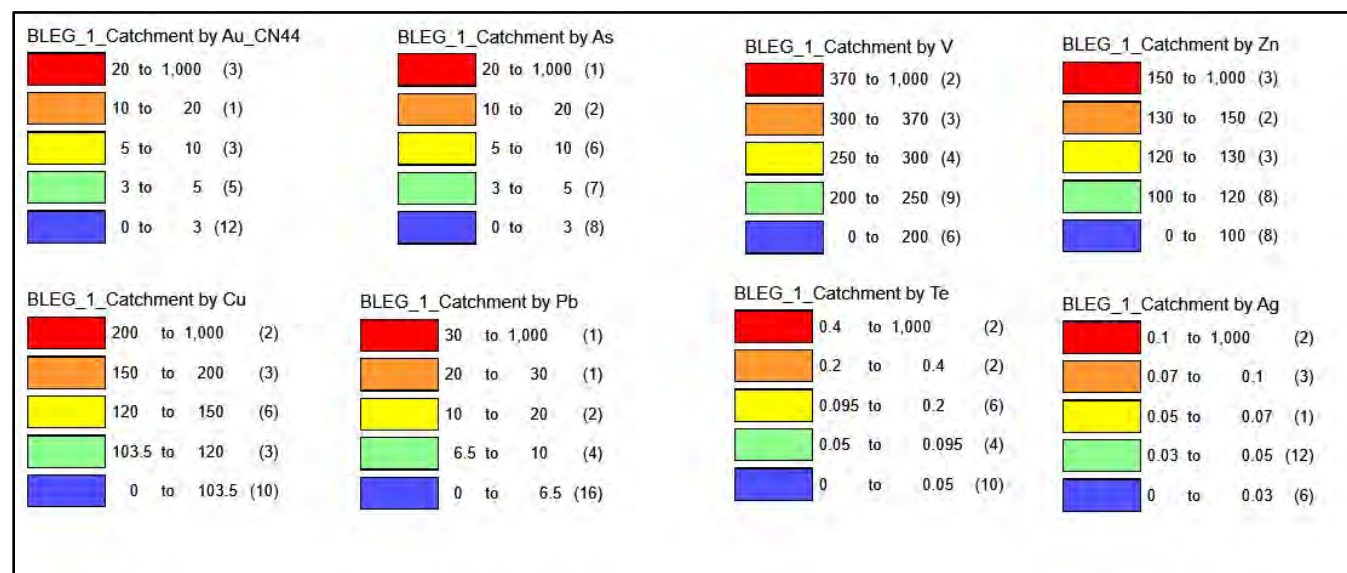
Figure 9-19: Legends for cBLEG multi-element images. Au = PPB, remaining elements in PPM.
