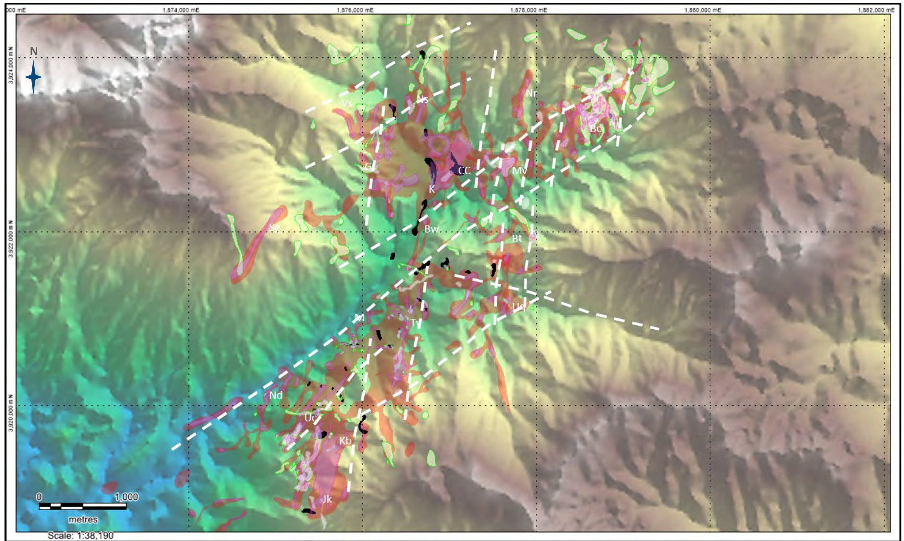
Figure 9-17: Regional analysis of Au-Ag-As-Te mineralizing cells from a combination of surface sampling techniques
