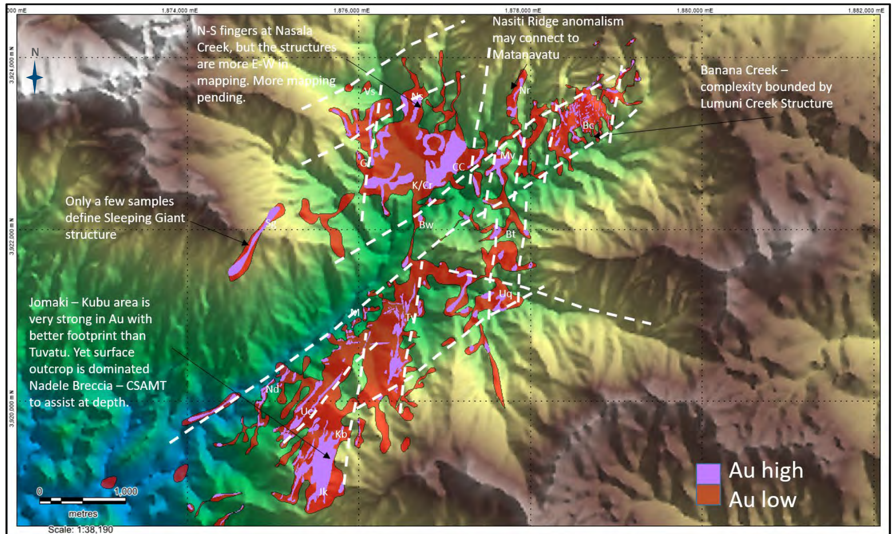
Figure 9-13: Regional analysis of gold mineralizing cells from a combination of surface sampling techniques
