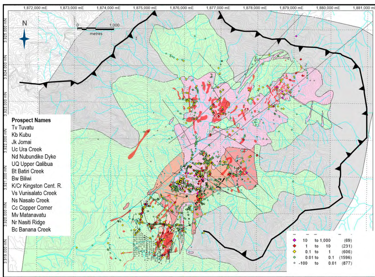
Figure 9-9: Rock sampling locations by gold on background geology
