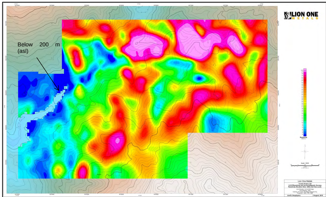
Figure 9-32: The Tuvatu 3-D resistivity elevation slice at 200 m (asl). This is the shallowest elevation slice that covers the complete survey area. Note the gap in the data (black arrow) where the topographic surface is lower than 200 m (asl) in the river drainage. Numerous structurally controlled resistivity highs are shown here (red). These features are relatively near surface. Edges of these bodies are difficult to pick visually from this data set.
