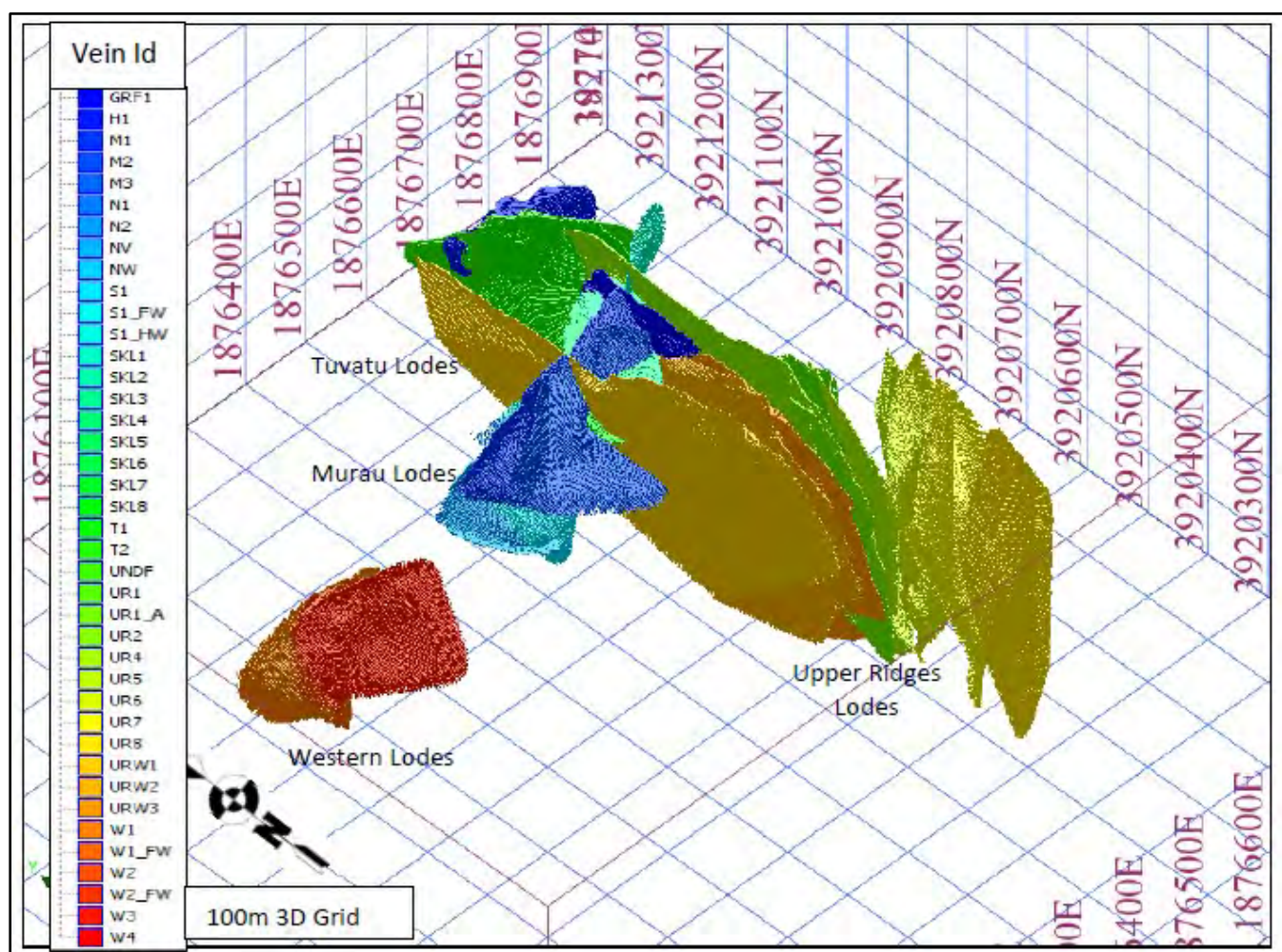
Figure 14-1: Tuvatu Lodes (oblique view [45°E -45°])
