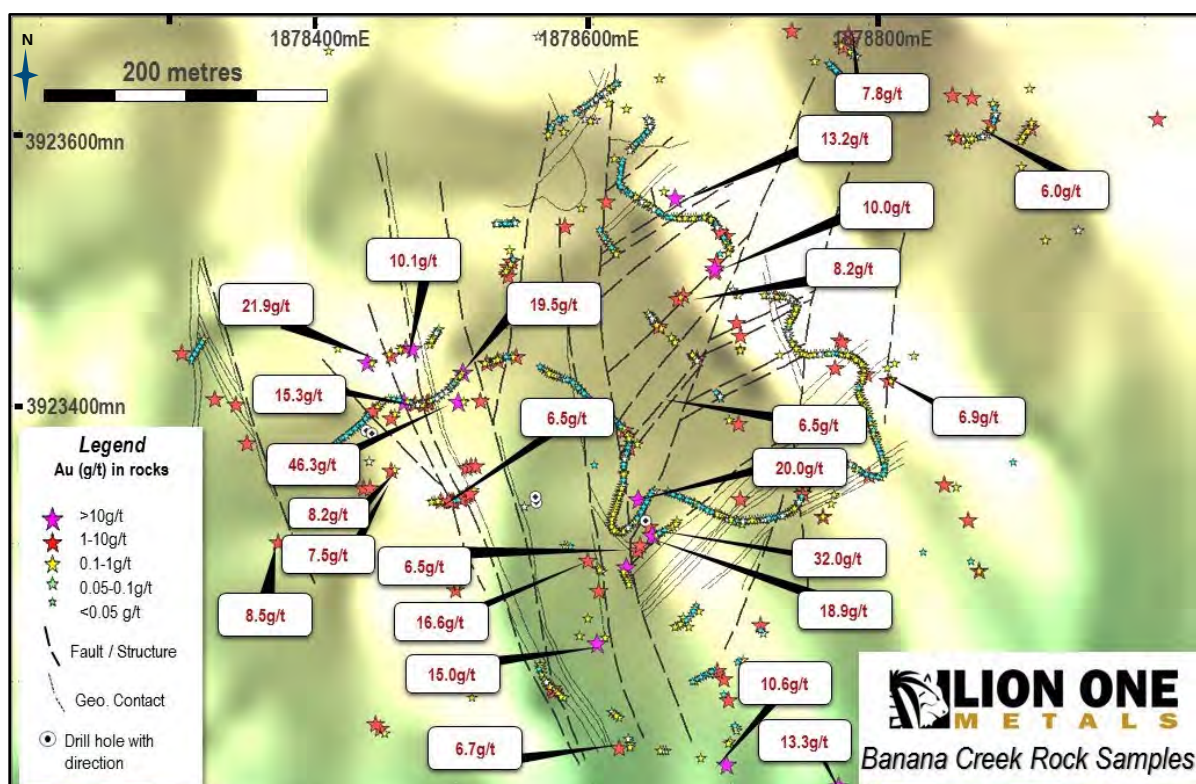
Figure 9-60: Historic rock sampling results from Banana Creek
