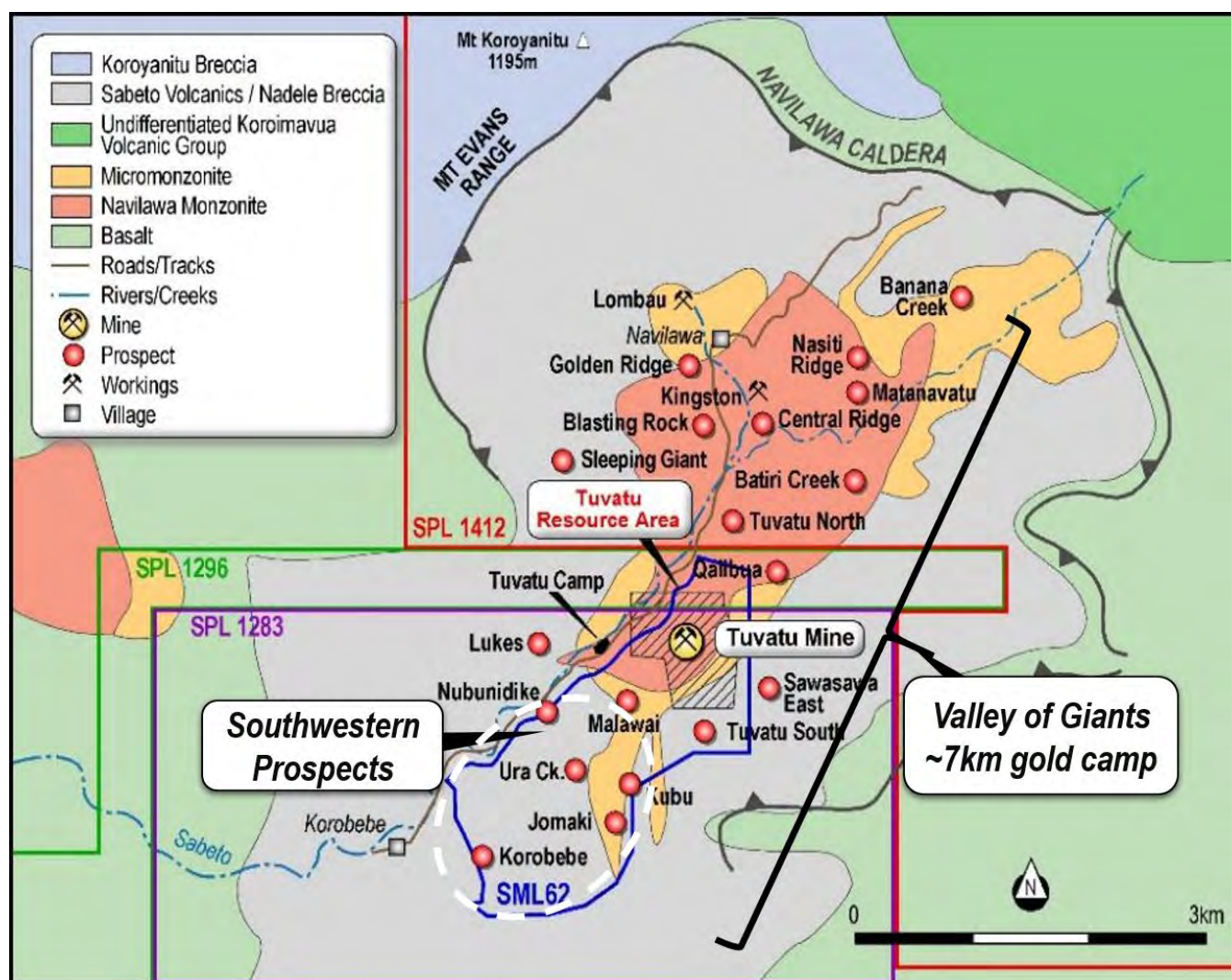
Figure 9-1: 2008 prospect locations
