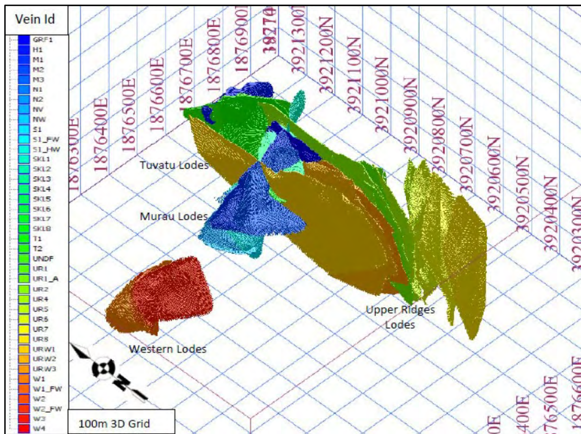
Figure 1-2: Tuvatu Lodes (oblique view [45°E -45°])
