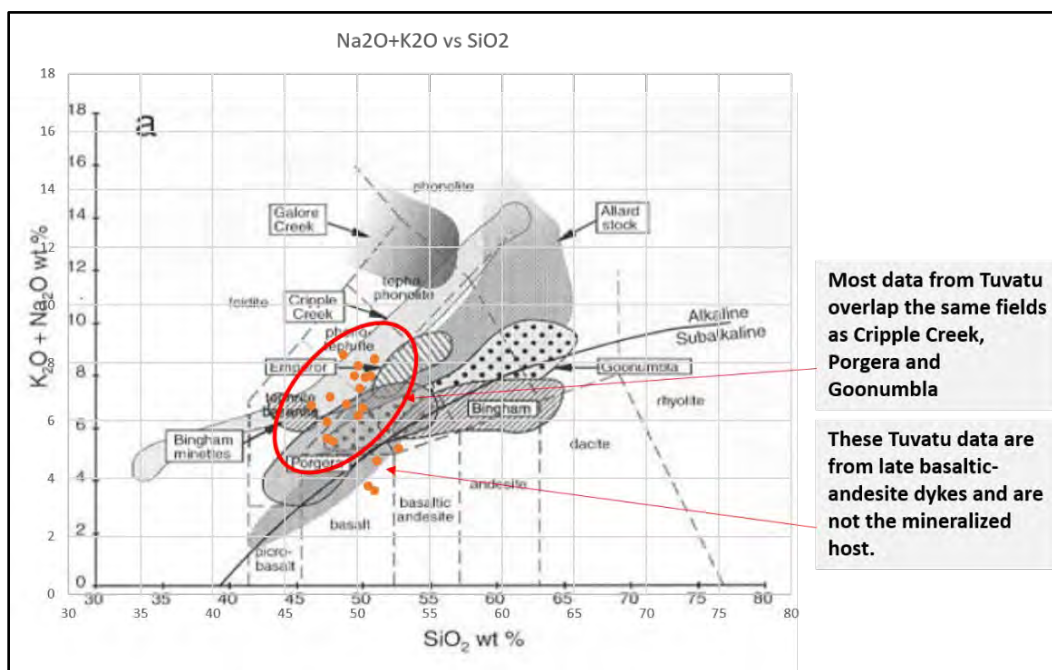
Figure 8-1: Data from Tuvatu (orange dots) derived from Scherbarth and Spry (2006) compared to K_2O+Na_2O vs. SiO_2 plot of alkali gold systems from Jensen and Barton (2000)
