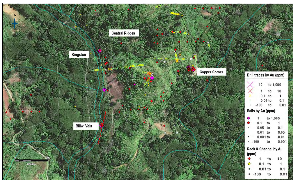
Figure 9-56: Kingston/Biliwi soil samples and target area location
