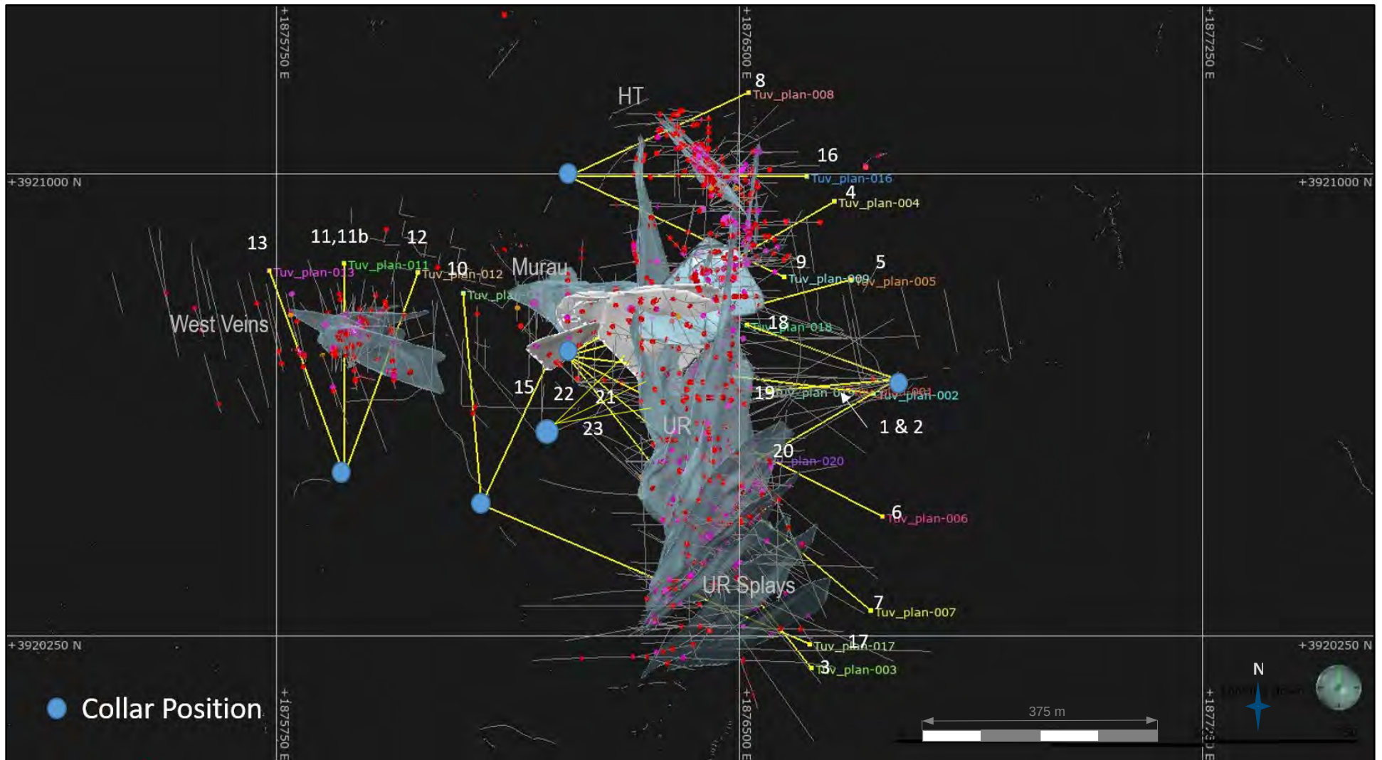
Figure 9-5: 2019/2020 deep drill plan (map view) with planned hole IDs
