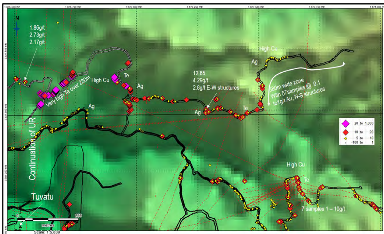
Figure 9-72: Upper Qalibua benching by tellurium (with gold grades labelled)
