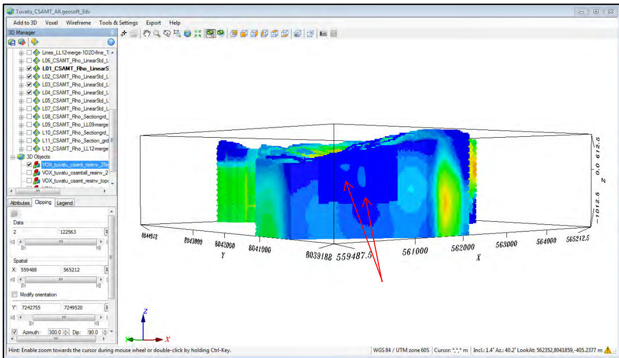
Figure 9-48: The Line 1, 2-D section is turned on. Note the weak, detailed resistivity highs (red arrows).
