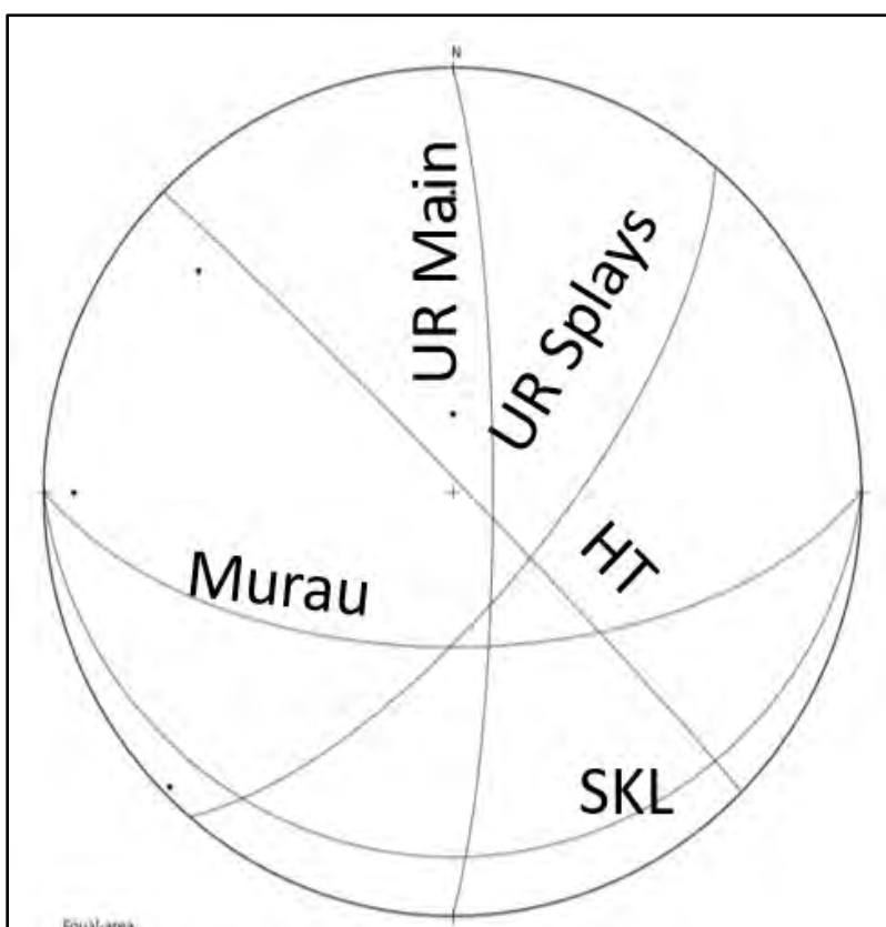
Figure 9-4: Stereonet showing general orientation of lodes at Tuvatu
