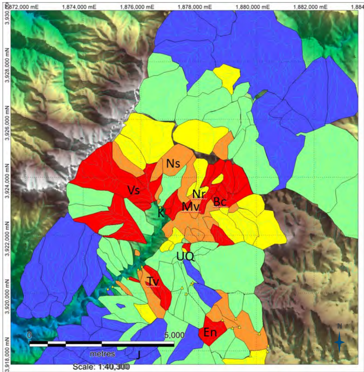
Figure 9-21: Silver in cBLEG stream survey samples
