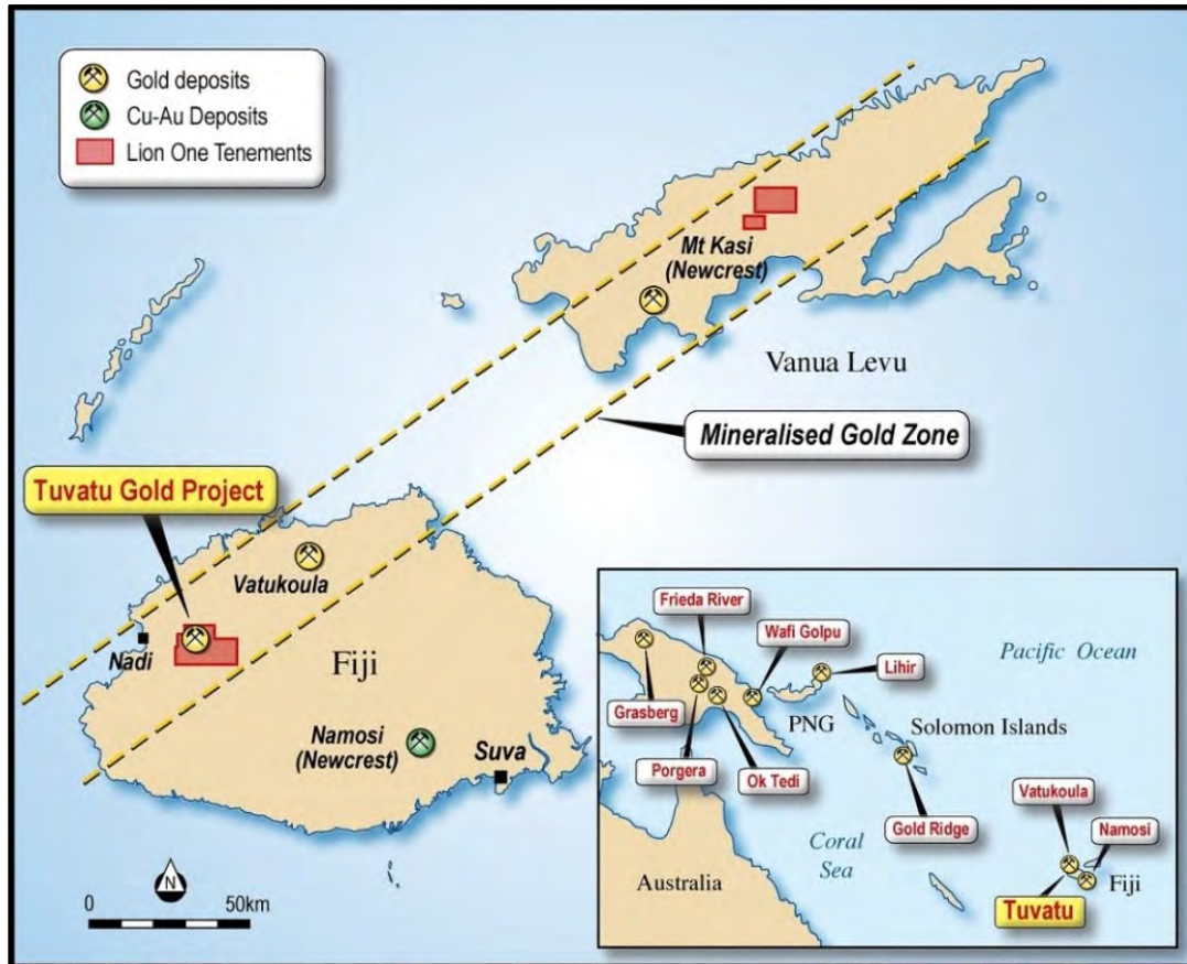
Figure 1-1: Project location
