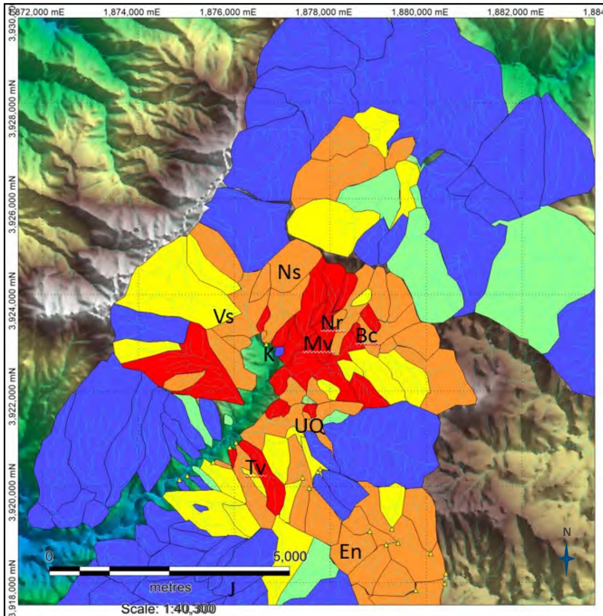
Figure 9-23: Copper in cBLEG stream survey samples
