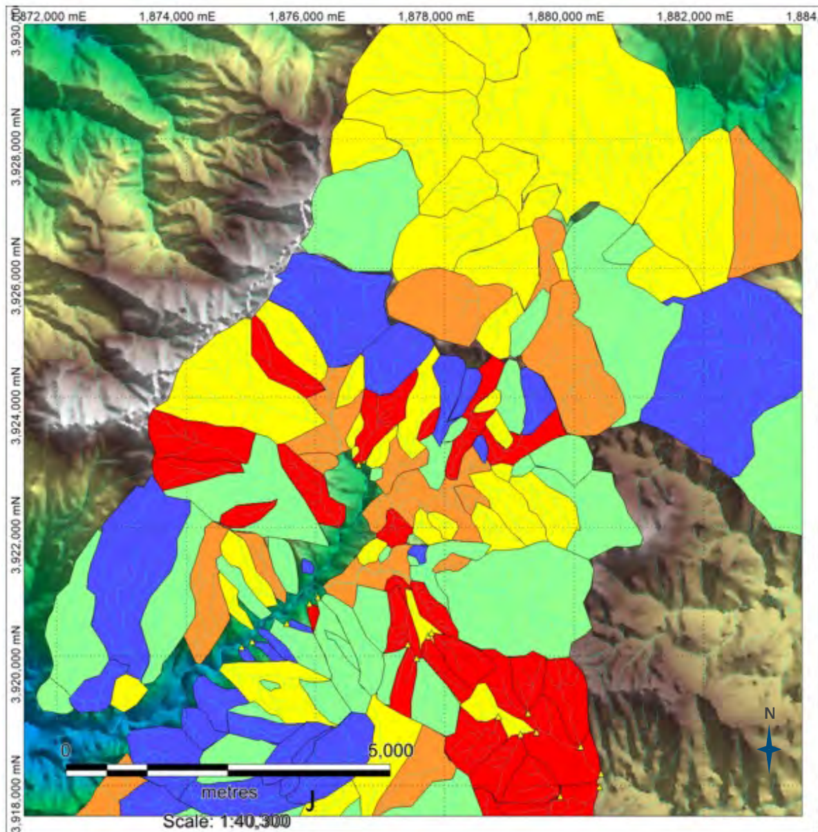
Figure 9-26: Vanadium in cBLEG stream survey samples
