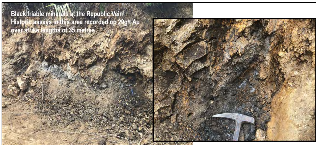
Figure 9-64: Manganese alteration at the Republic Vein
