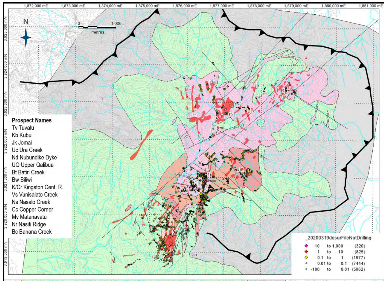
Figure 9-10: Chip channel sampling from benching and creek sampling on background geology
