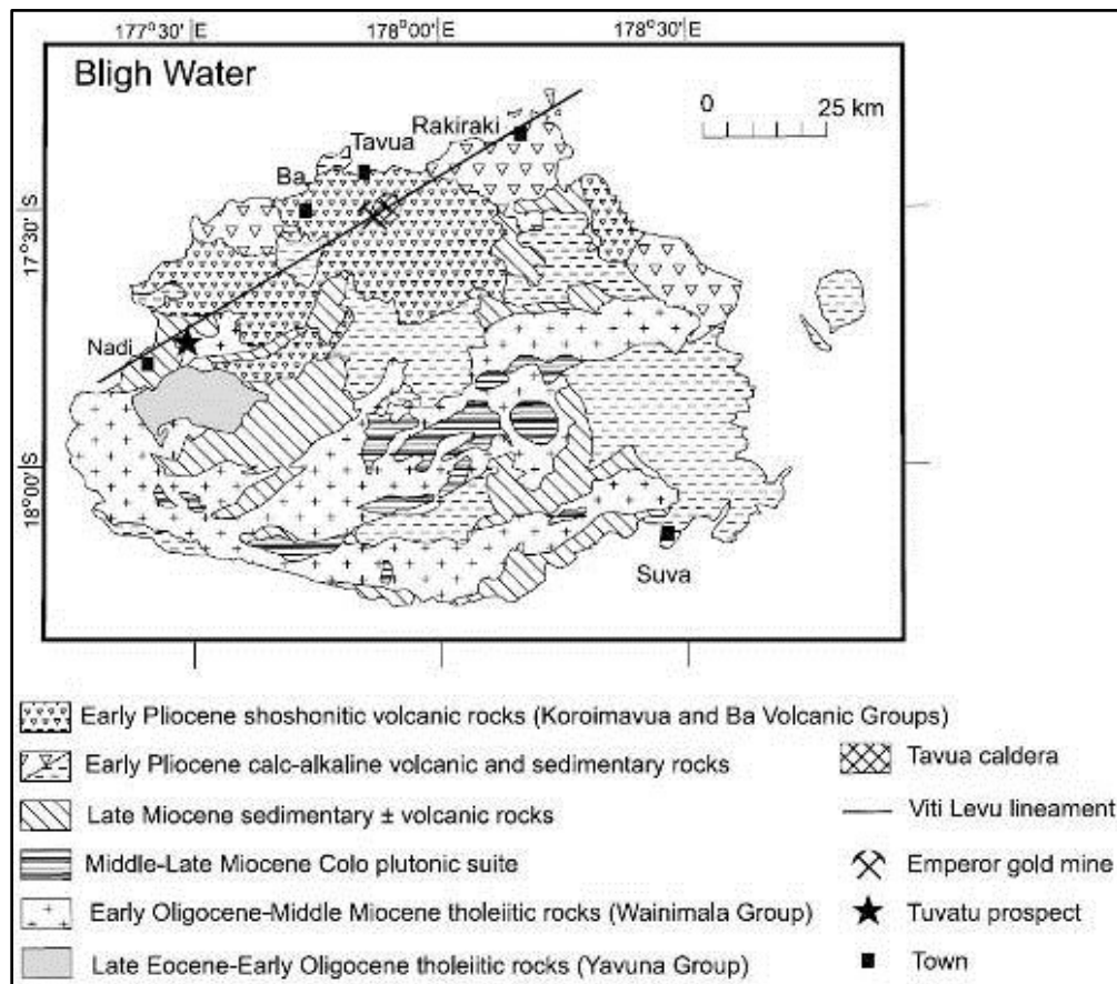
Figure 7-1: Regional geology. Location of Tuvatu Project with respect to Viti Levu lineament is indicated.
