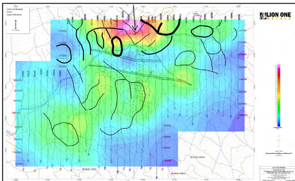
Figure 9-39: The 0 m MHG resistivity overlay plotted on the 0 meter IP elevation slice. Note that once again the IP anomaly is shifted to the side of the resistivity high zones (see black arrow). In fact the high IP response is surrounded by the higher resistivity features in this elevation slice. Once again interpreted contacts and structures adjacent to the IP high are exploration targets.
