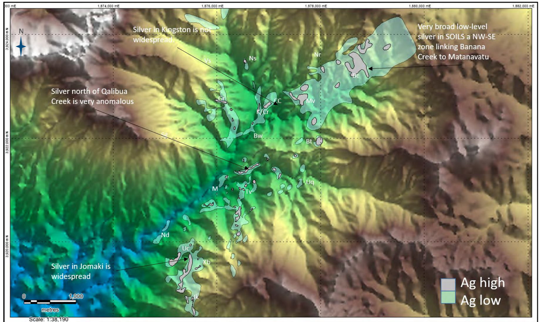
Figure 9-14: Regional analysis of silver mineralizing cells from a combination of surface sampling techniques
