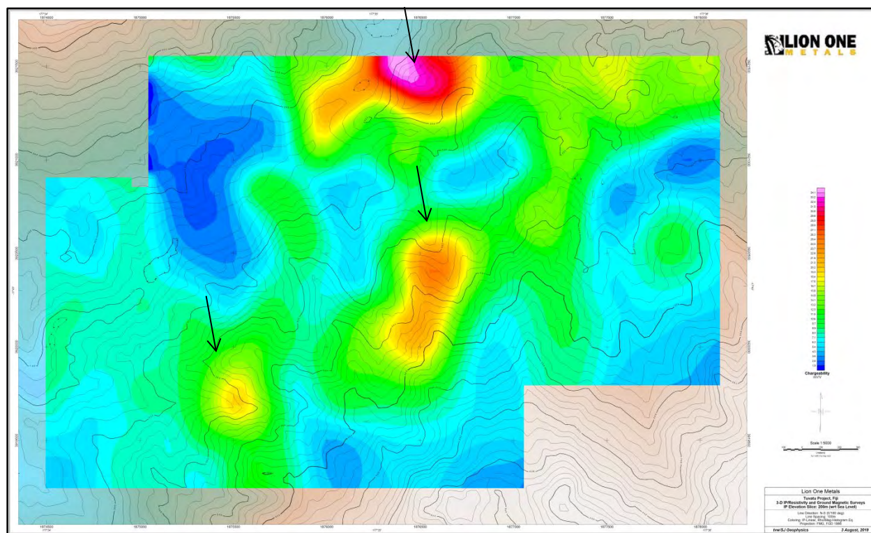
Figure 9-36: The Tuvatu IP +200 m elevation slice. The near surface high IP responses are indicated by the black arrows. The relationship of these anomalous IP responses to gold mineralization is unknown at this time. They could be related to a porphyry system. The important point is that the IP highs are shifted to the side of the resistivity highs and are interpreted to occur at the edges of high resistivity intrusions (see Figure 9-37).
