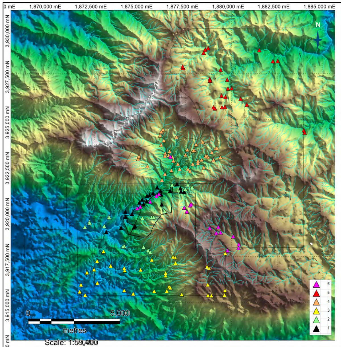
Figure 9-18: 2019 cBLEG sample locations coloured by batch number
