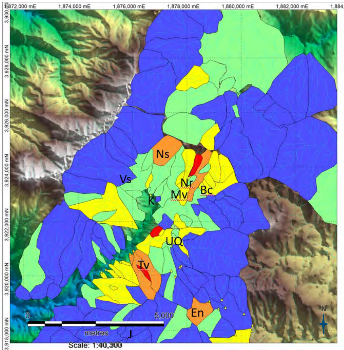
Figure 9-22: Arsenic in cBLEG stream survey samples
