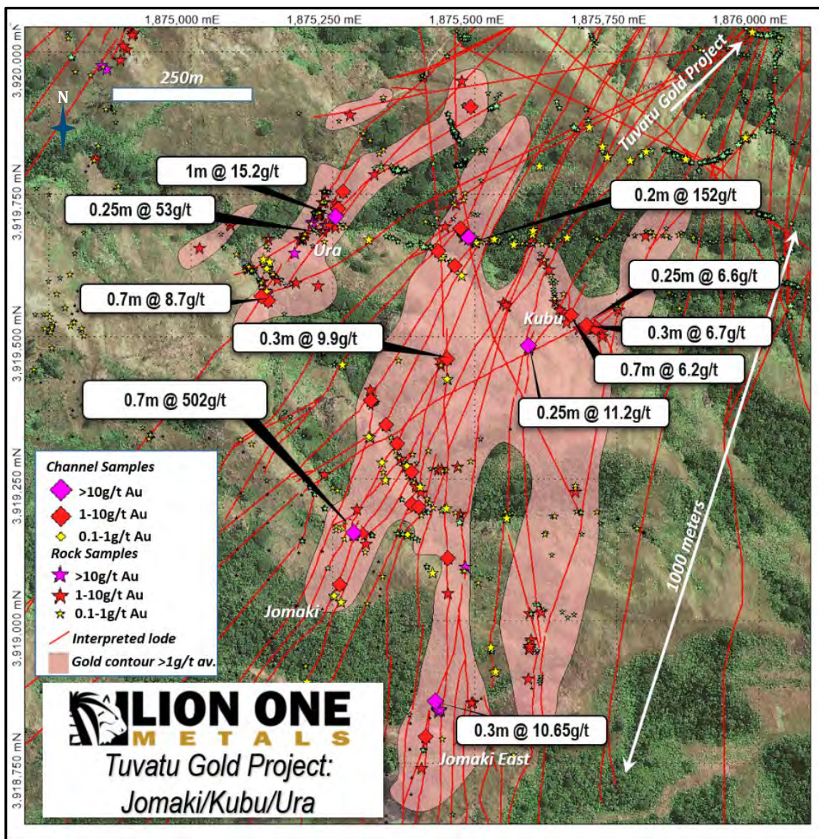
Figure 9-3: 2017 to 2018 benching program for the southern prospects
