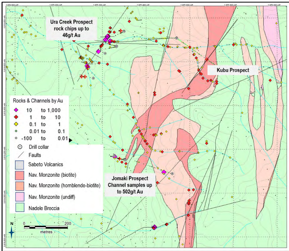
Figure 9-68: Jomaki-Ura-Kubu geology, with drill collars
