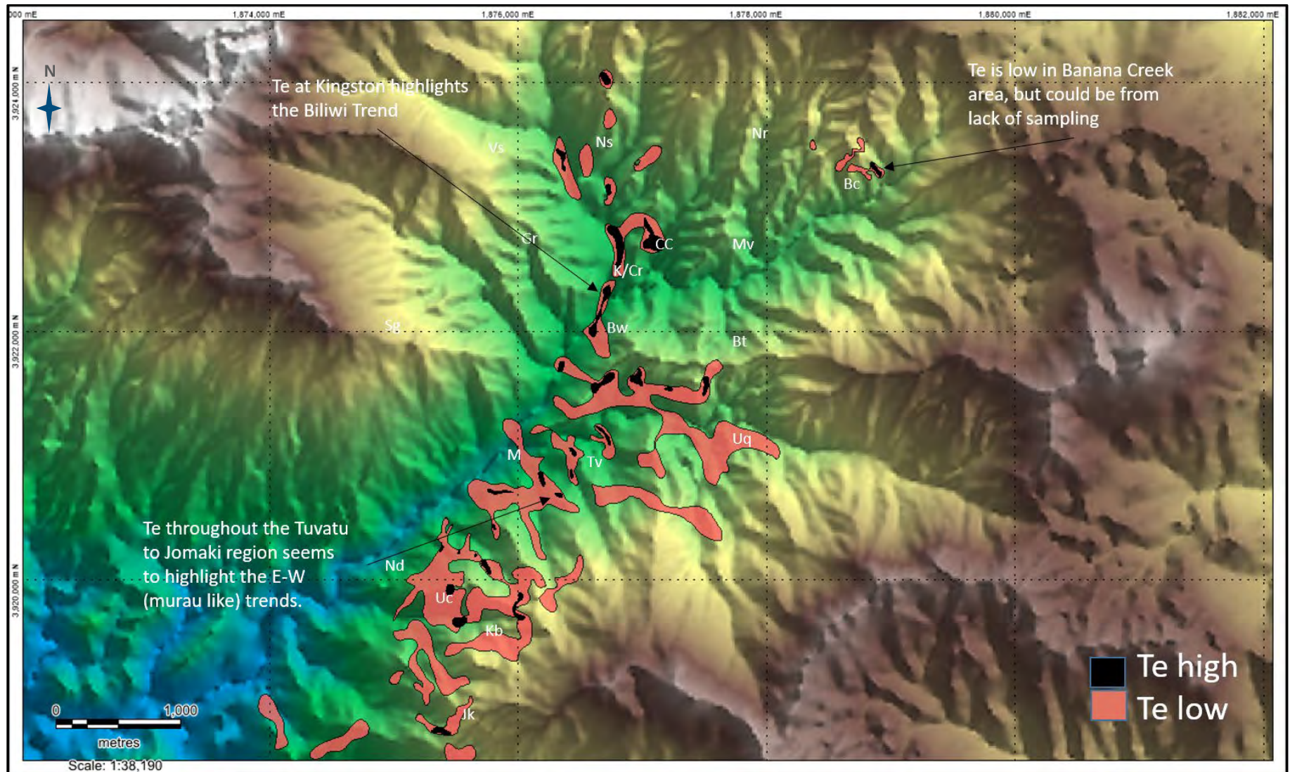
Figure 9-15: Regional analysis of tellurium mineralizing cells from a combination of surface sampling techniques
