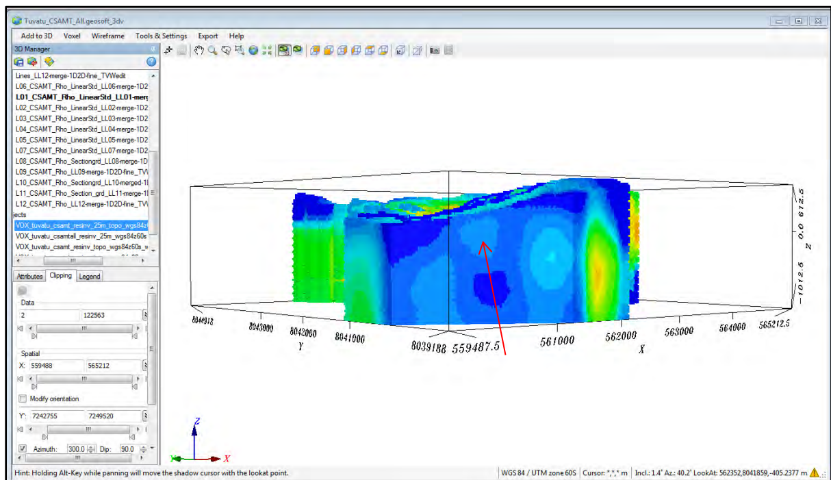
Figure 9-49: The Line 1, 2-D section is turned off. Note the lack of weak, detailed resistivity highs as indicated by the red arrow. A broad resistivity high exists, but no detail is resolved.
