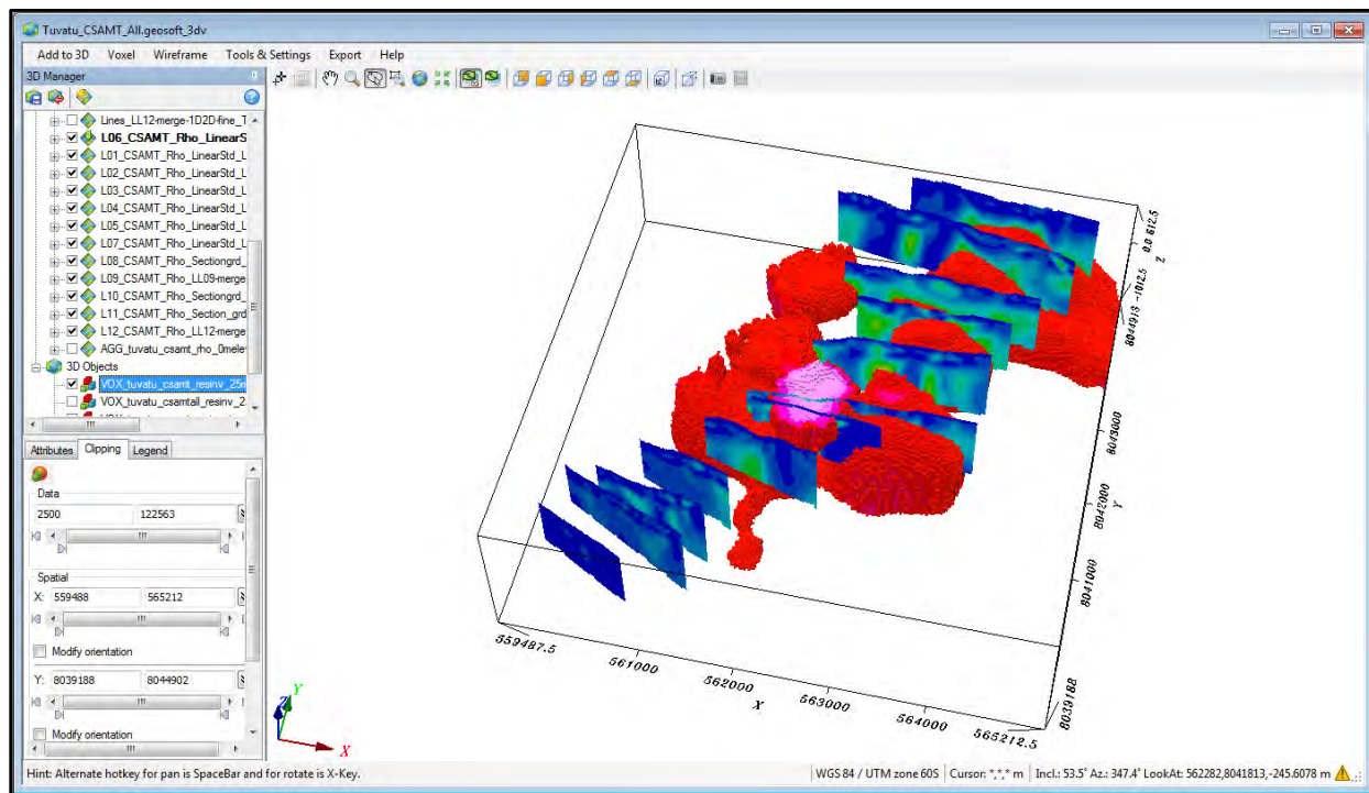
Figure 9-47: The section slices for Lines 1 through 12 superimposed on the clipped ( \rho > 2500 ohm-m) voxel display of the combined 2-D inversion models
