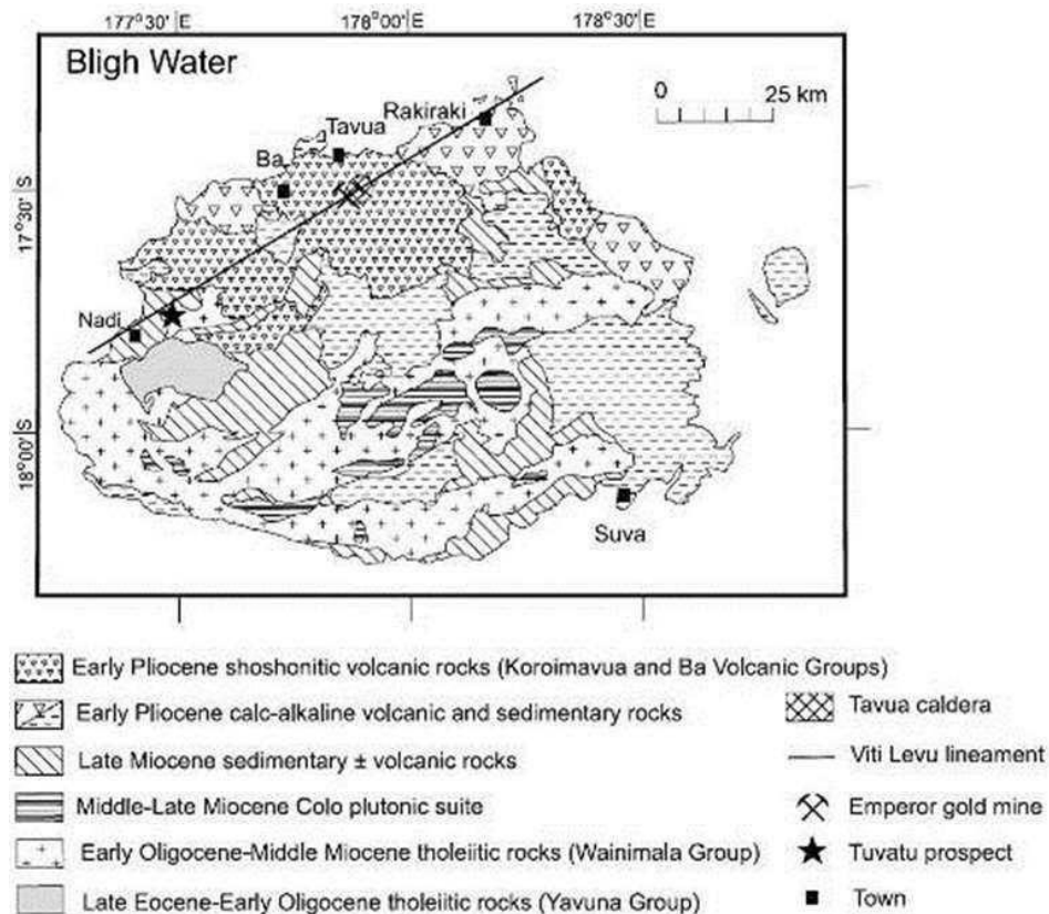
Figure 2- Regional Geology. Location of Tuvatu Project with Respect to Viti Levu Lineament is
