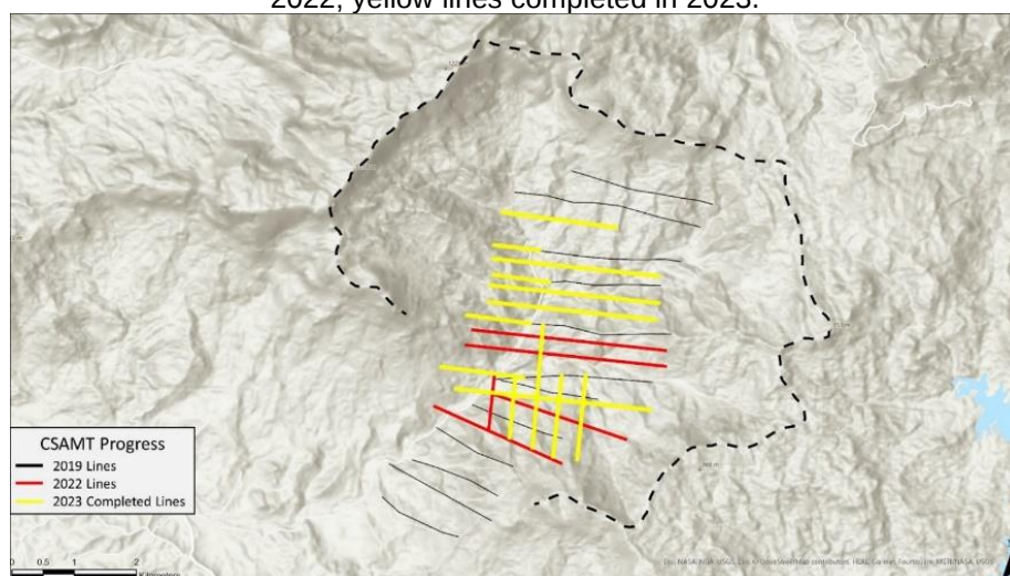
Figure 3: Location of 2019-2023 CSAMT Survey Lines; black lines completed in 2019; red lines completed in 2022; yellow lines completed in 2023.
