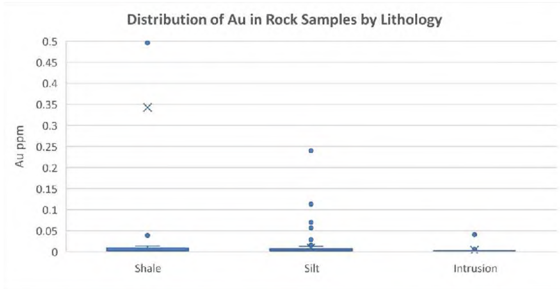
Figure 9-6: Box Plot - Rock Samples and Au Assay (Note: not all shale analysis visible).
