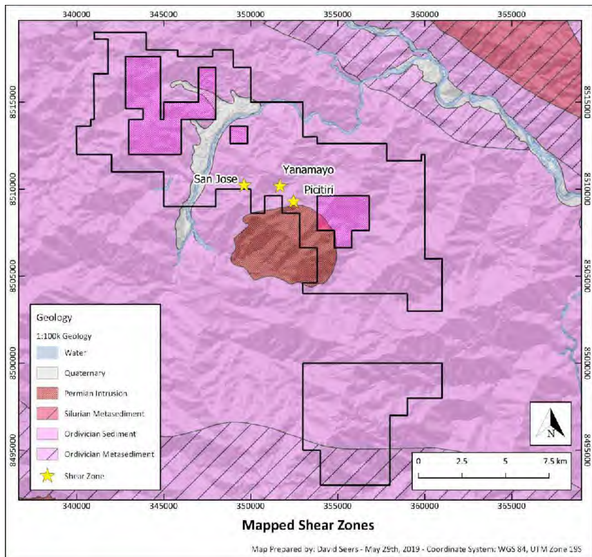
Figure 9-3: Mapped Shear Zones
