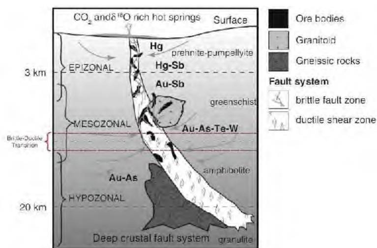
Figure 8-1: Typical cross-section of an orogenic system
