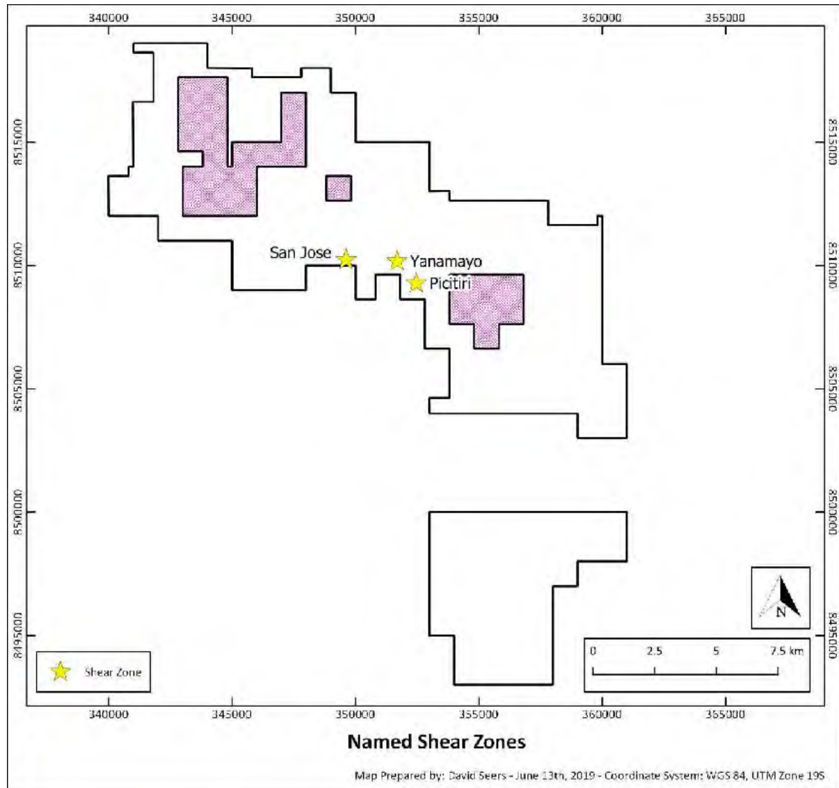
Figure 7-3: Named Auriferous Shear Zones
