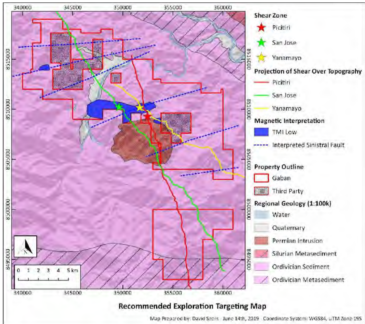
Figure 26-1: Recommended Exploration Targeting Map
