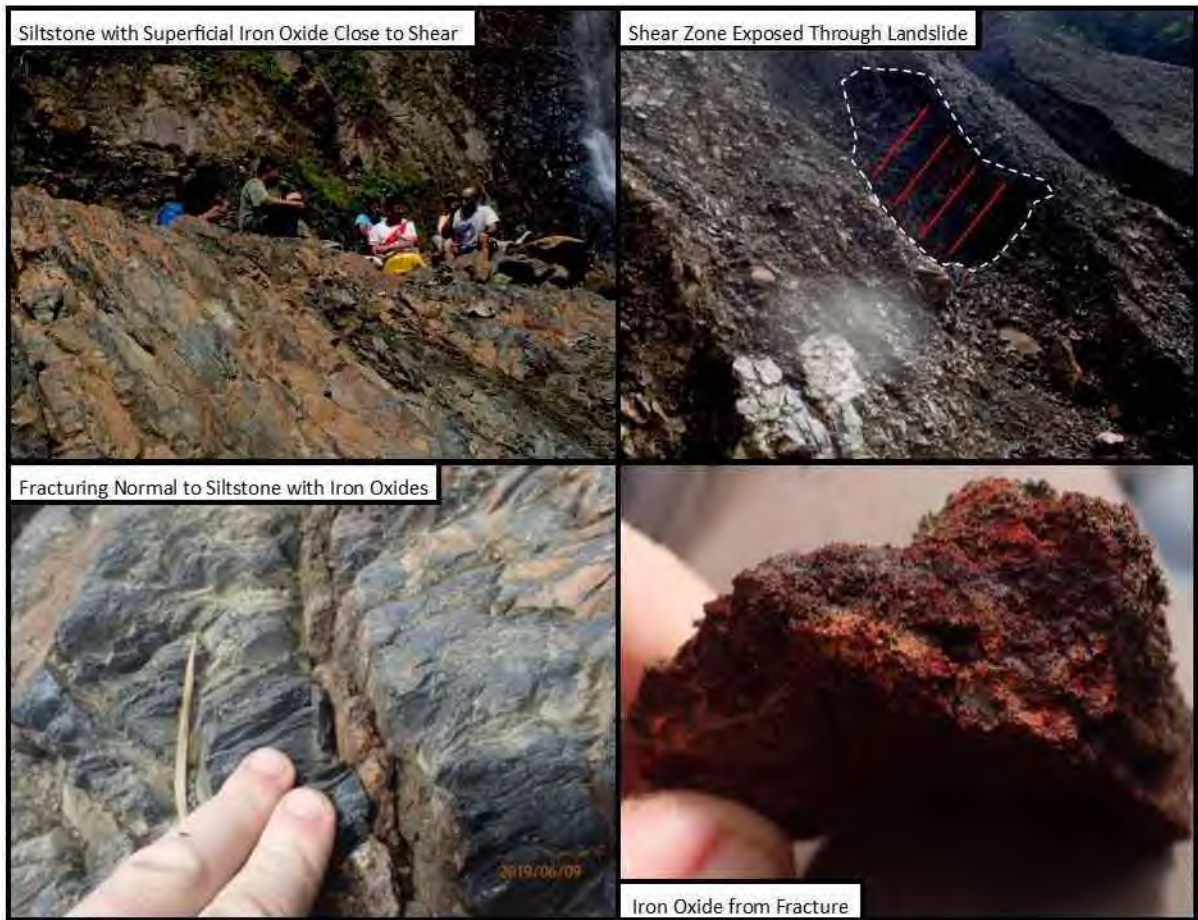
Figure 7-10: Photographs from the San Jose Shear
