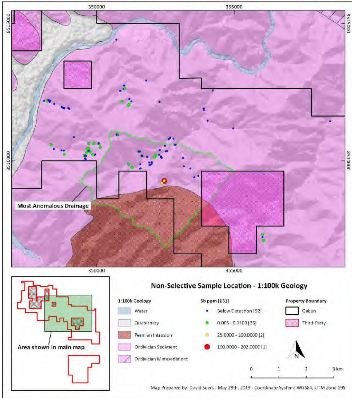
Figure 9-10: Non-Selective Samples - Distribution and Sb Assay
