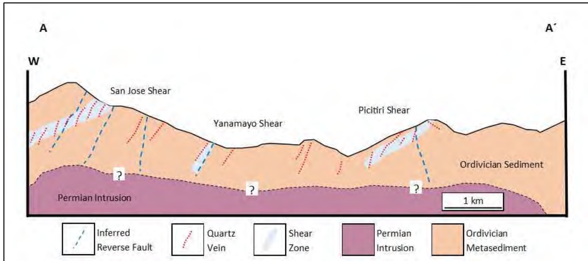
Figure 7-4: Local Geology - Conceptual Cross Section
