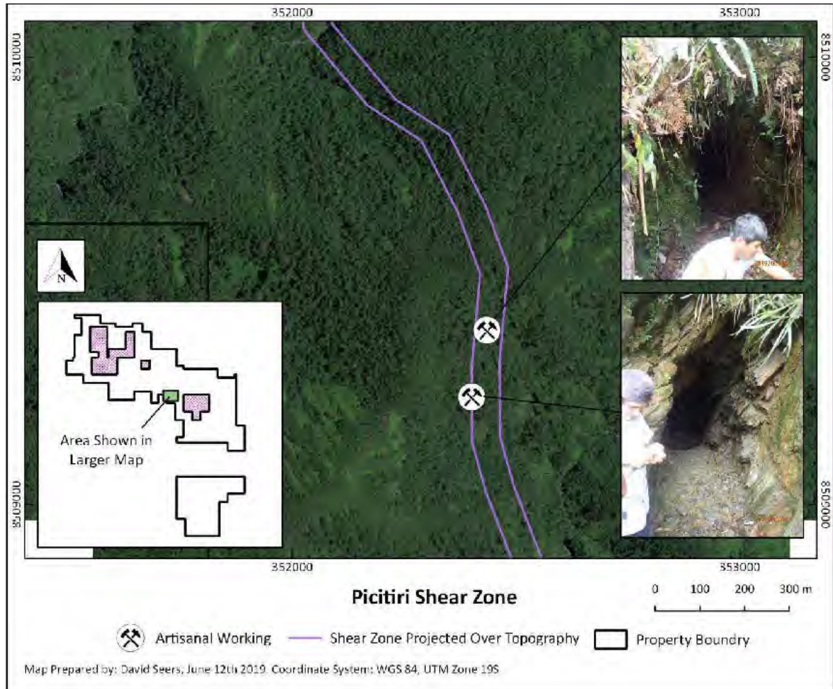
Figure 7-5: Picitiri Shear Zone
