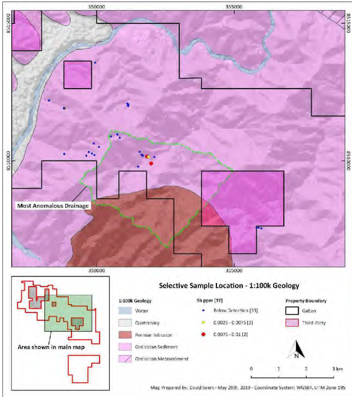
Figure 9-8: Selective Rock Sampling - Distribution and Sb Assays
