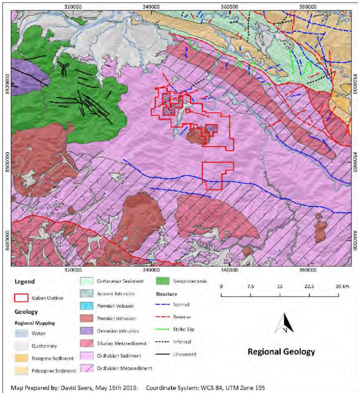
Figure 7-1: Regional Geology
