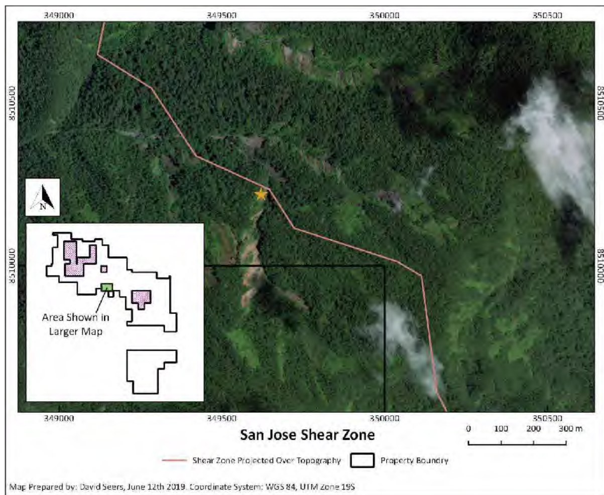
Figure 7-9: San Jose Shear
