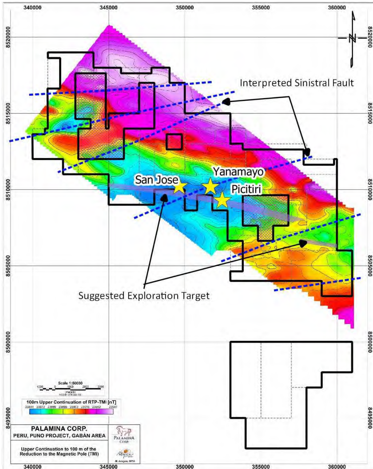
Figure 9-11: RTP TMI - Interpretation Shown with Shear Zones
