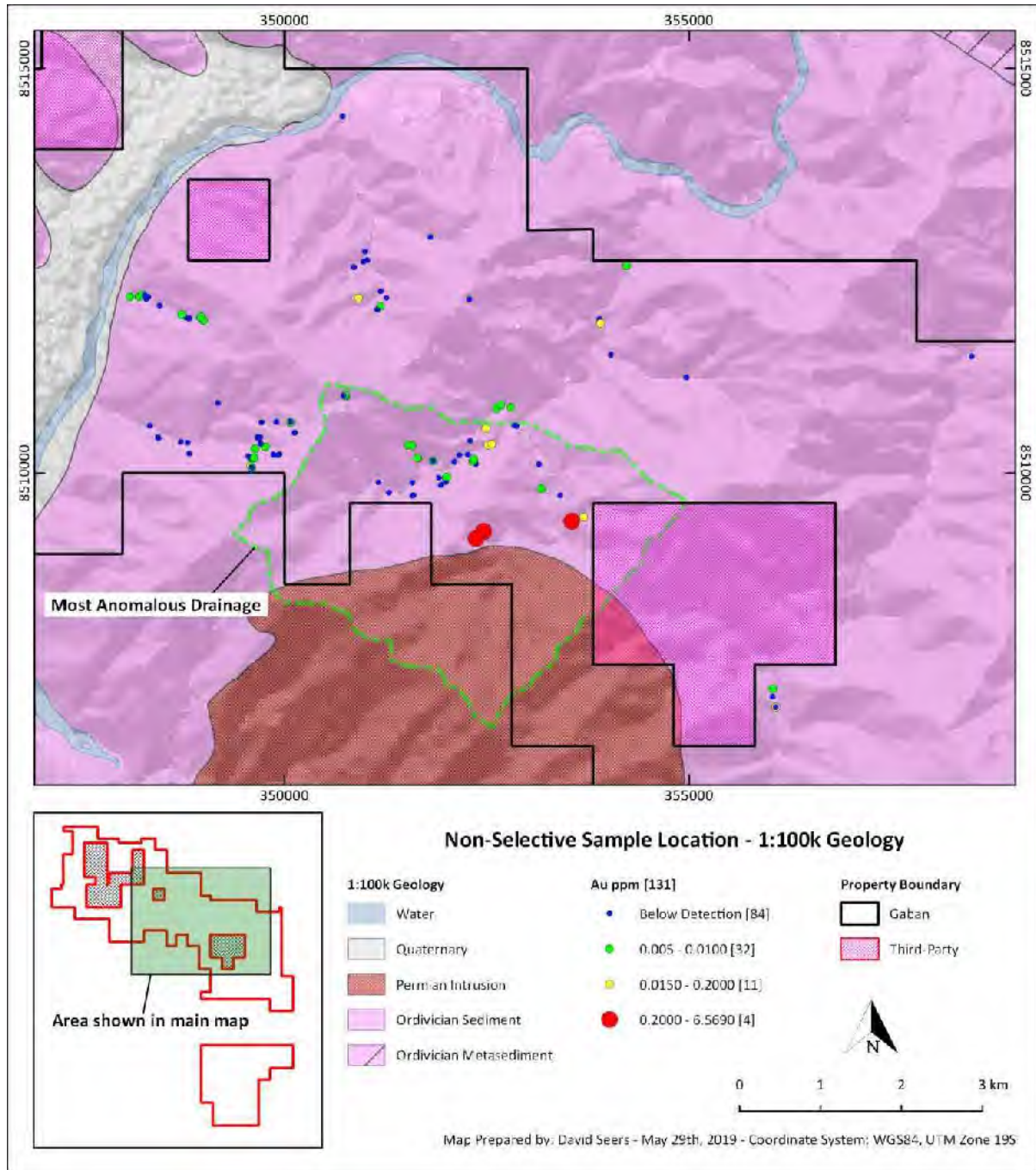
Figure 9-9: Non-Selective Samples - Distribution and Au Assay
