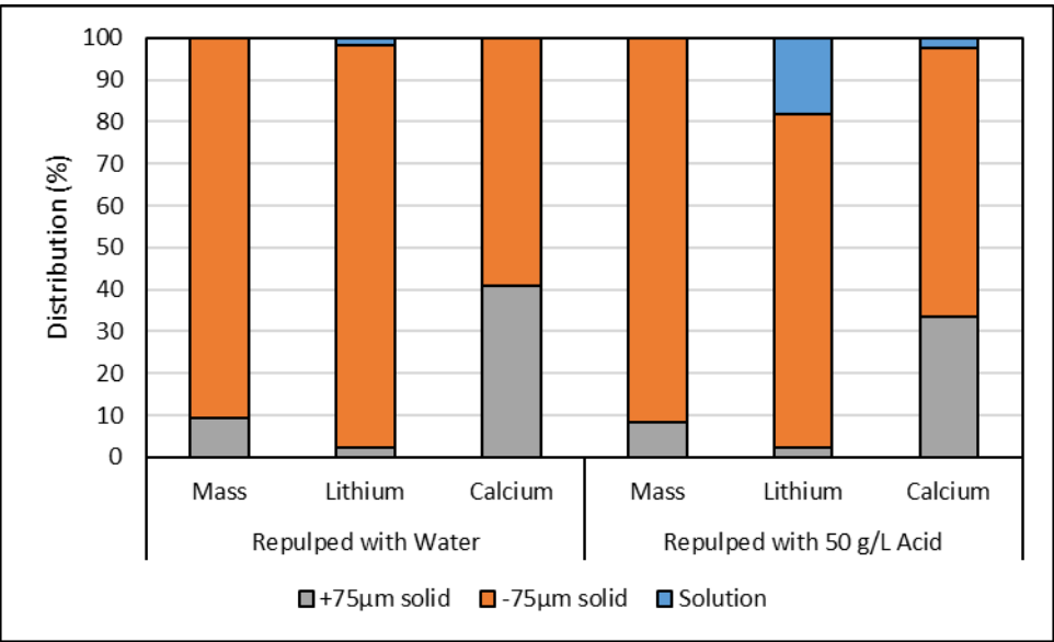
Figure 13-1: Beneficiation Summary
