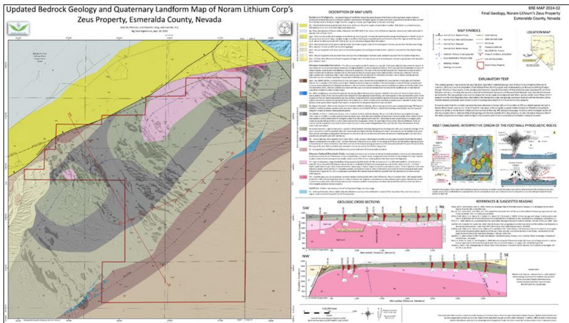
Figure 7-4: Property Geology Map
