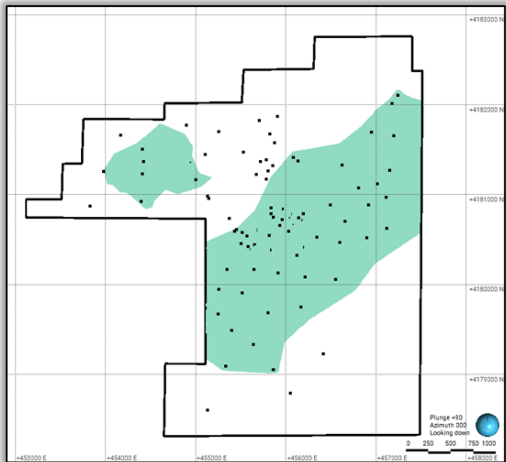
Figure 14-5 Plan View of the Indicated Resources
