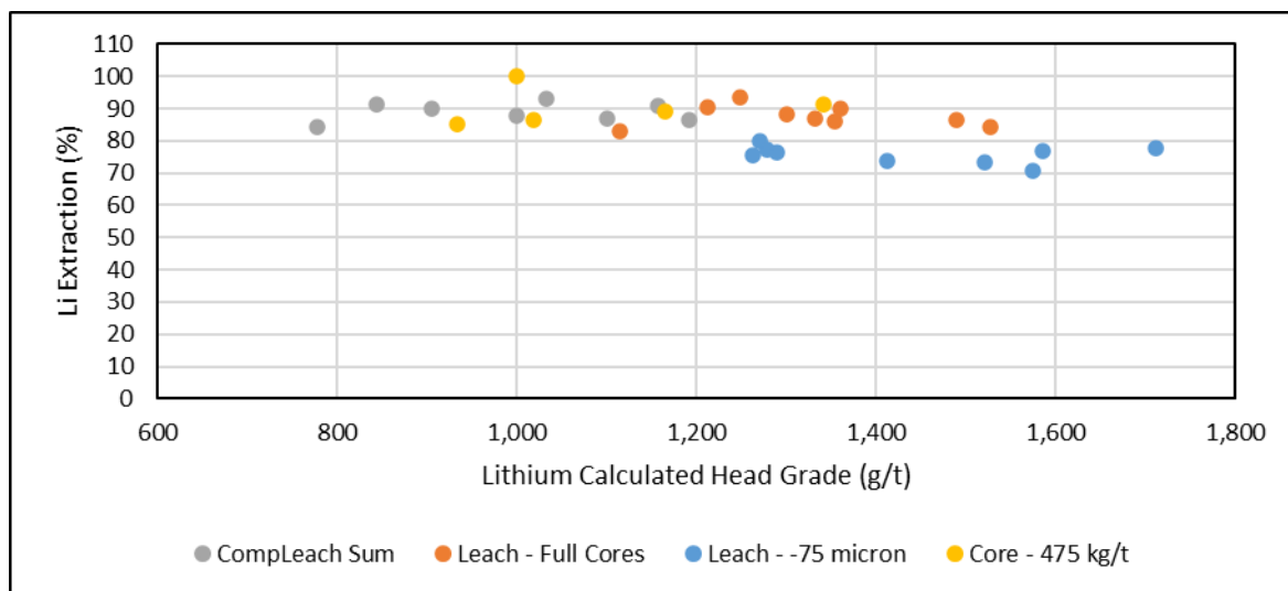
Figure 13-3: Leaching Summary – Recovery vs Lithium Head Grade
