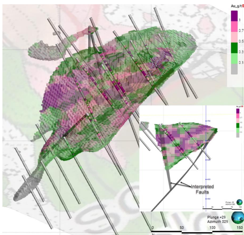
Figure 2: 3D and Sectional (Inset) Views of the Southern Gold Zone Block Model
