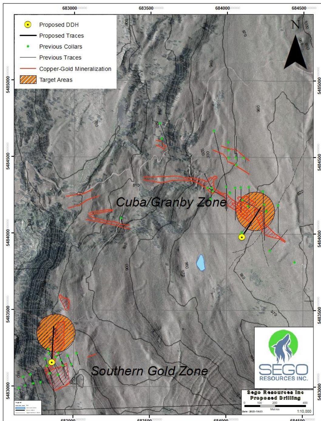
Figure 4. Overview of existing copper-gold mineralization, previous drill holes, new targets and proposed drill holes.
