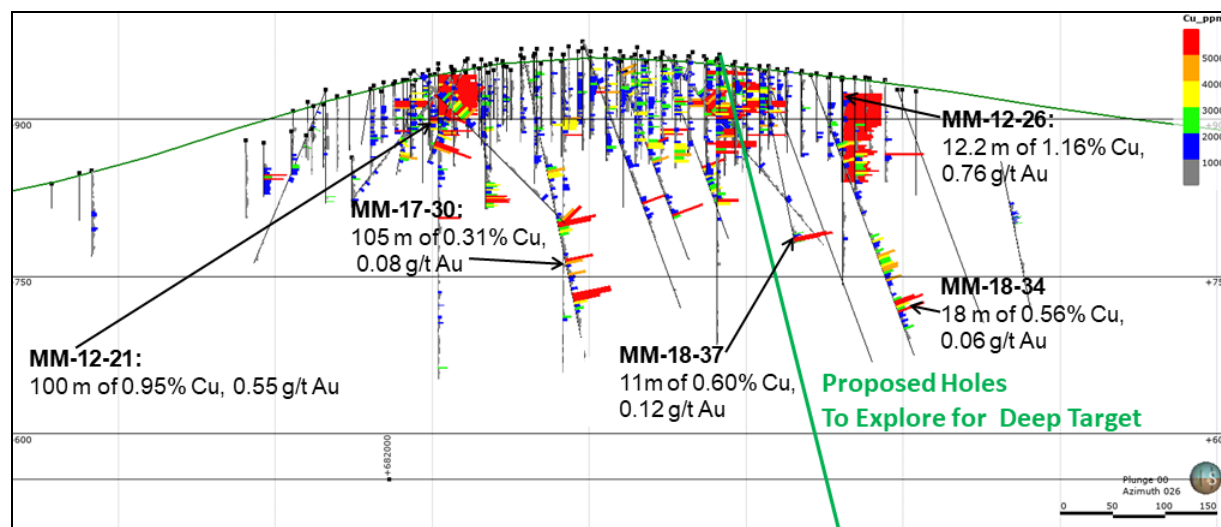
Figure 1. Long section looking northeast, showing the proposed deep drill holes below the Cuba Zone porphyry copper-gold mineralization.
