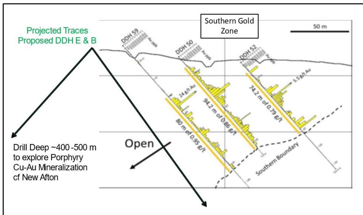
Figure 3. A section looking east that locates a proposed hole to drill north to explore for deep porphyry copper-gold mineralization north from the Southern Gold Zone and a second hole to drill south to extend the north dipping Southern Gold Zone and check for porphyry copper-gold mineralization in that area.
