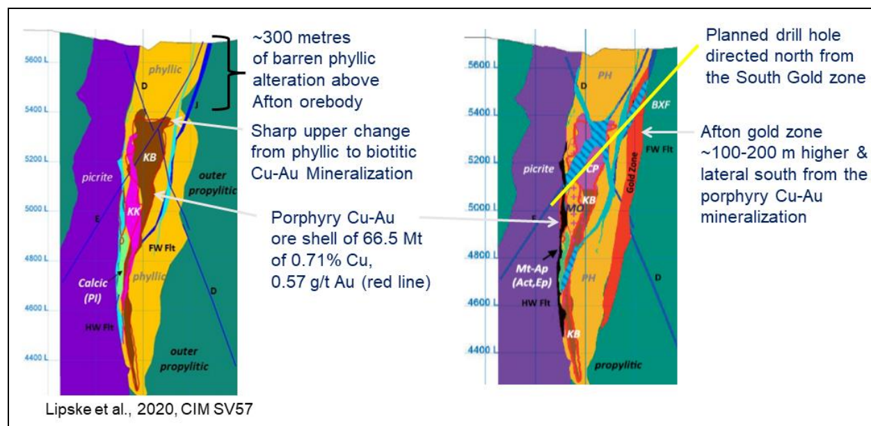
Figure 2. New Afton – porphyry copper-gold and gold zone analogue for the Southern Gold Zone and the deep drill test porphyry copper-gold mineralization (trace of yellow drill hole).
