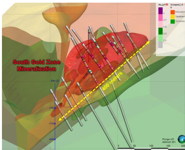
Figure 1: 3-D View of the Litho-structural and Mineralization Models of the Southern Gold Zone
