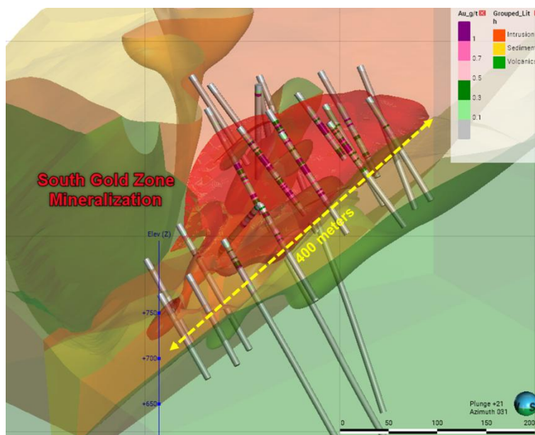
Figure 1: 3-D View of the Litho-structural and Mineralization Models of the Southern Gold Zone Source: SRK, 2024
