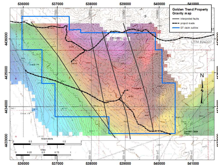
Figure 10 Gravity map with interpreted faults
