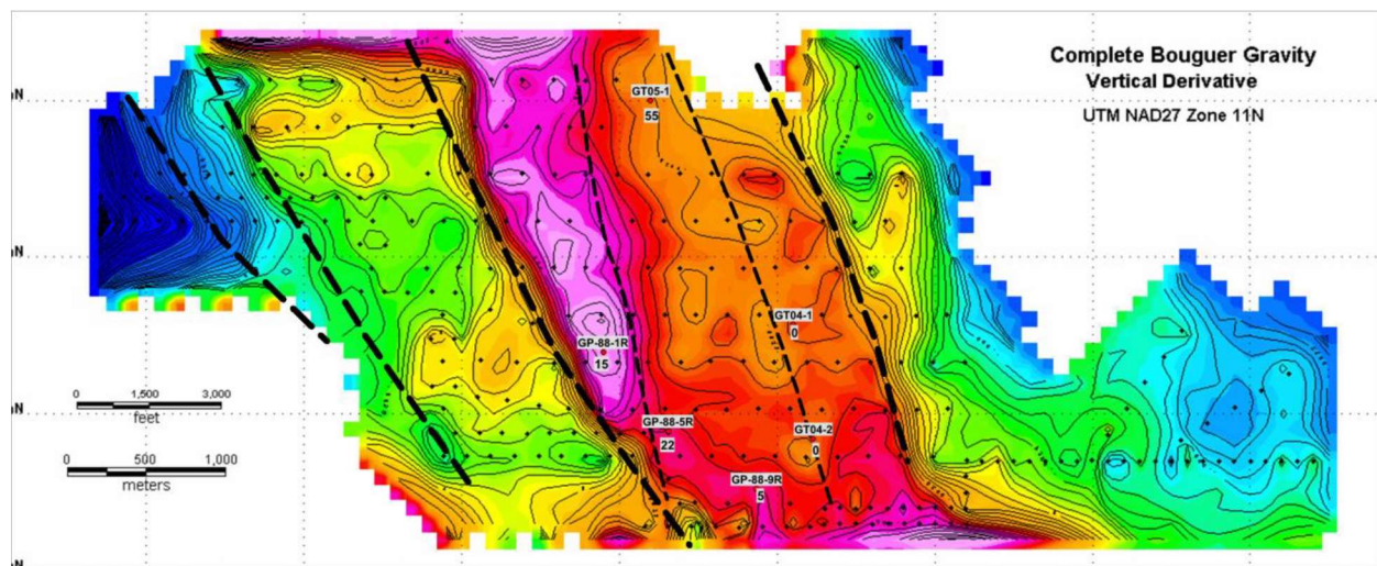
Figure 11 Vertical derivative of gravity data
