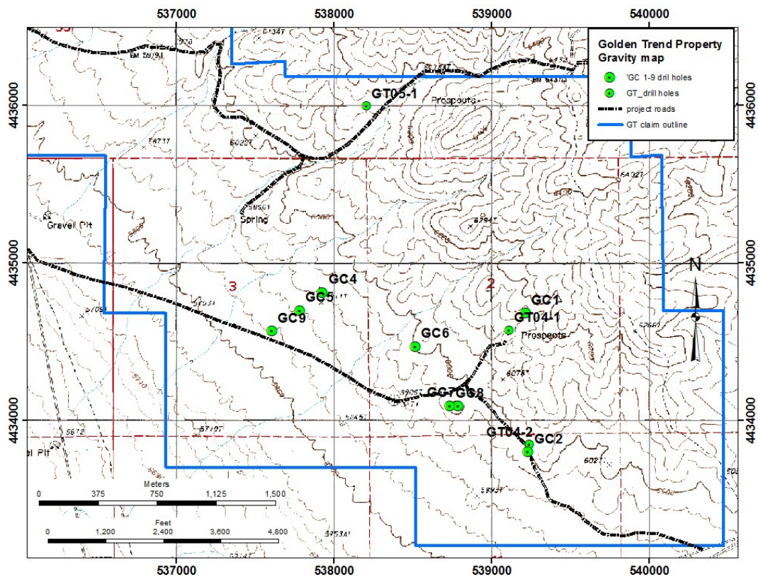
Figure 8 J-Pacific drill hole location map
