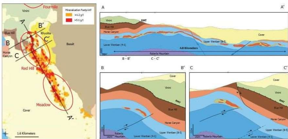
Figure 18 Structural and stratigraphic control of the Goldrush orebody
