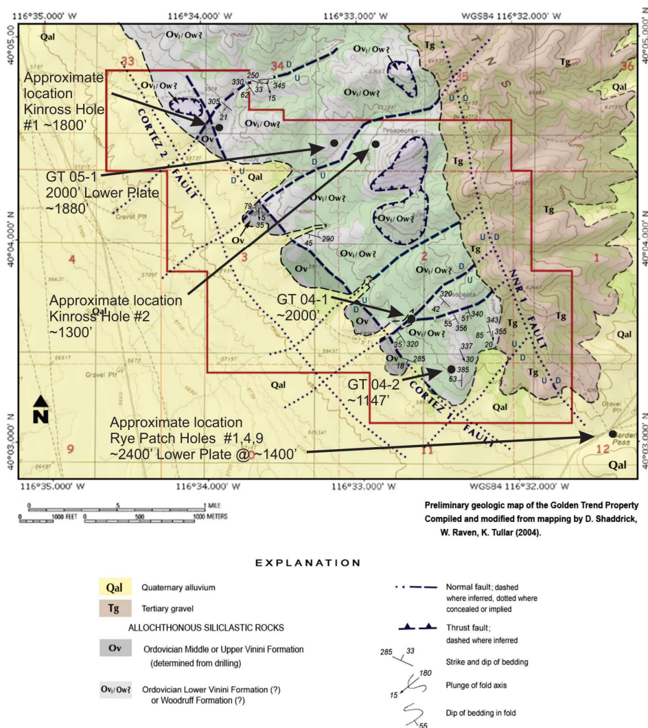
Figure 12 Kinross drill hole map
