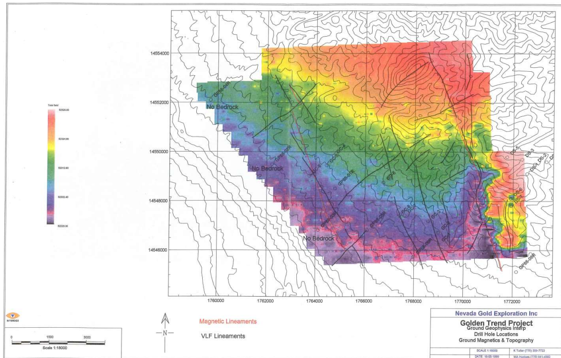
Figure 9. Ground magnetic map
