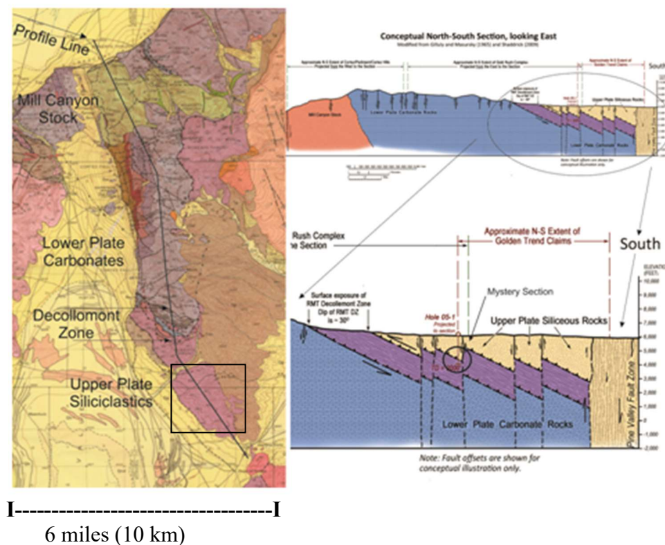
Figure 13 Regional geology and structure
