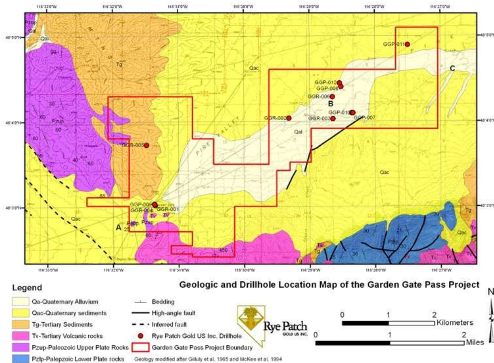
Figure 21 Ryepatch Gold drill hole map
