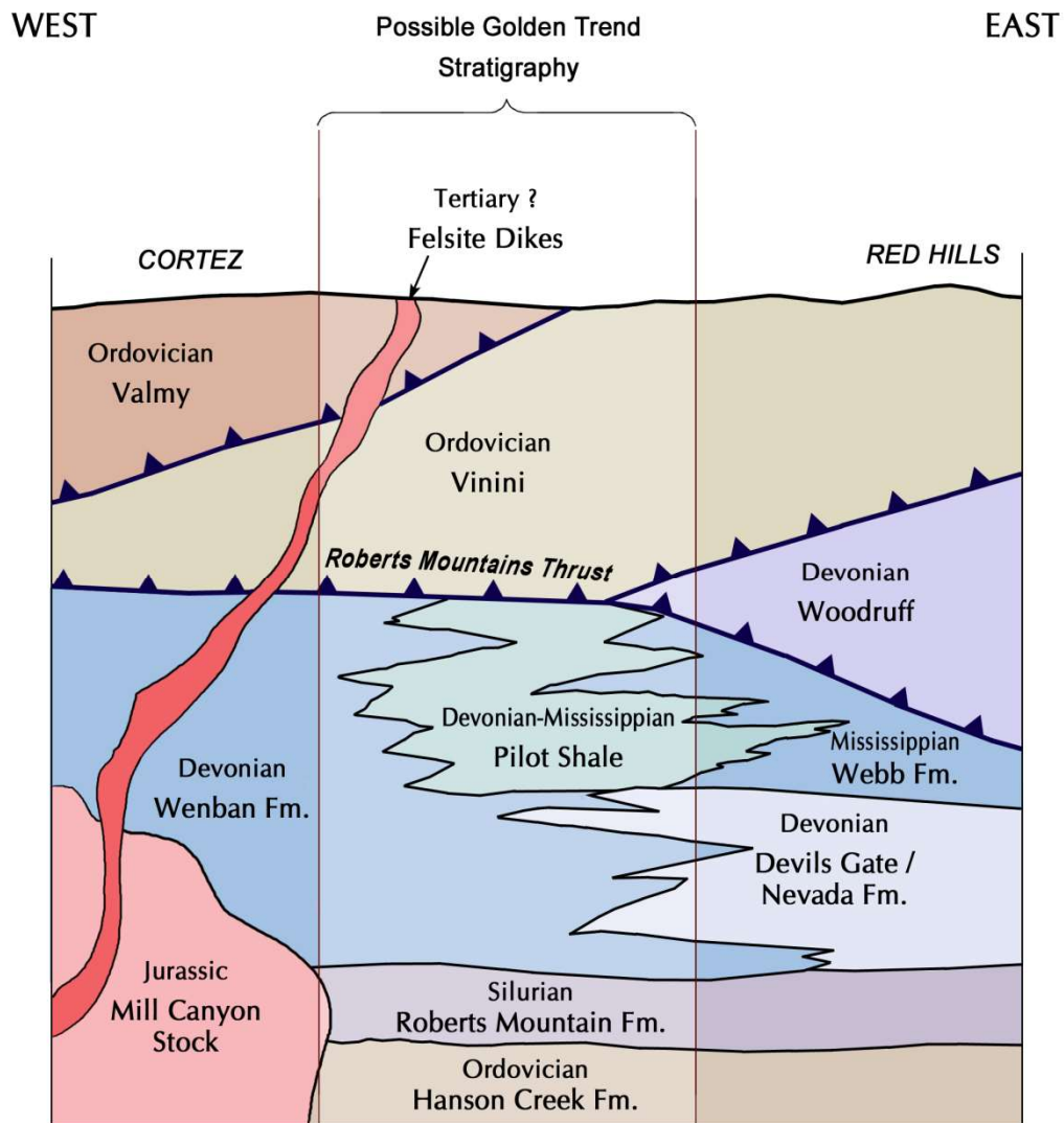
Figure 15 District stratigraphy (not to scale)
