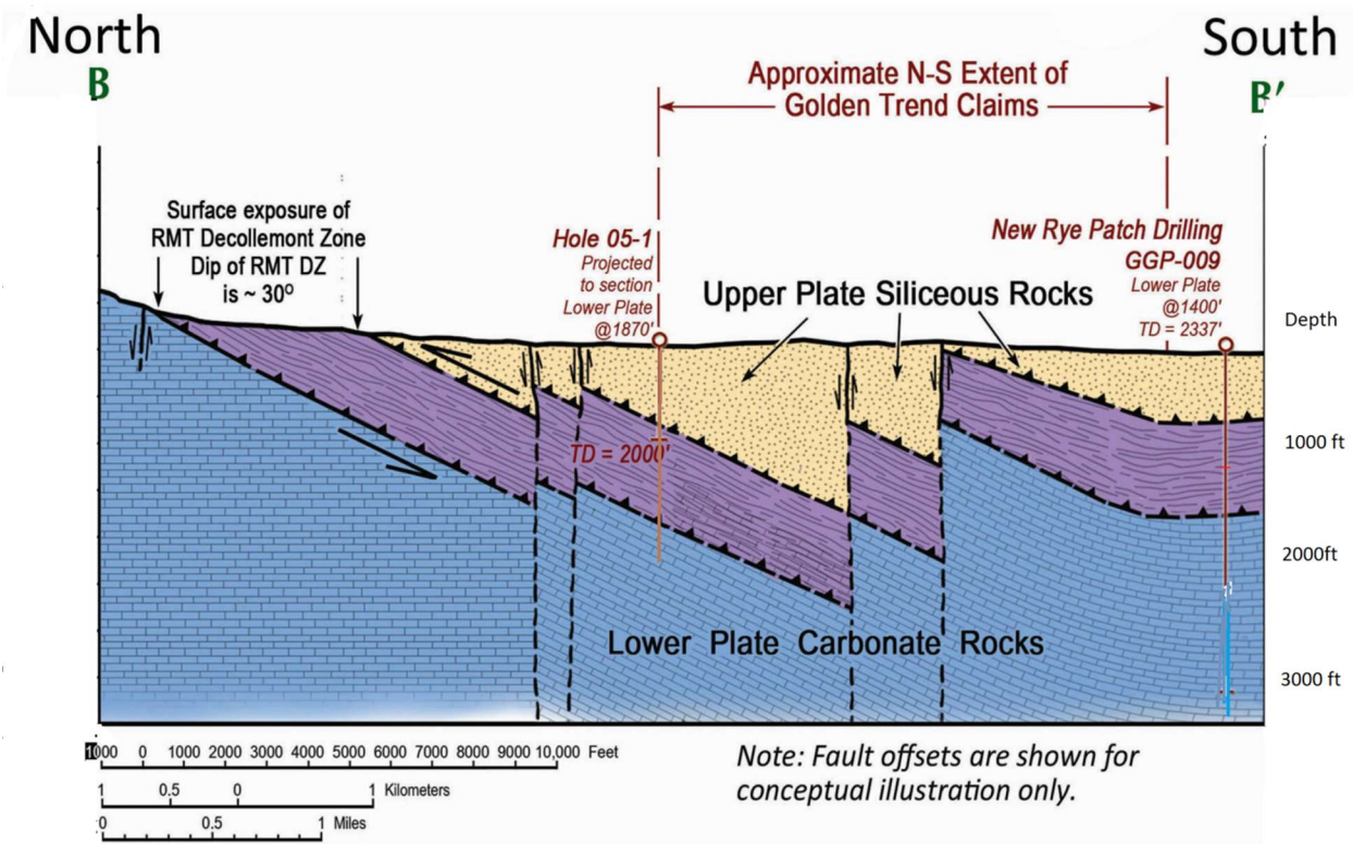
Figure 22 Idealized cross section of property
