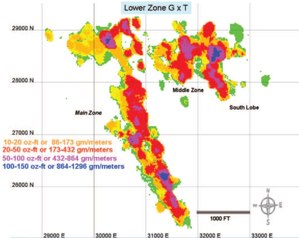
Figure 17 Cortez Hills Lower zone ore body
