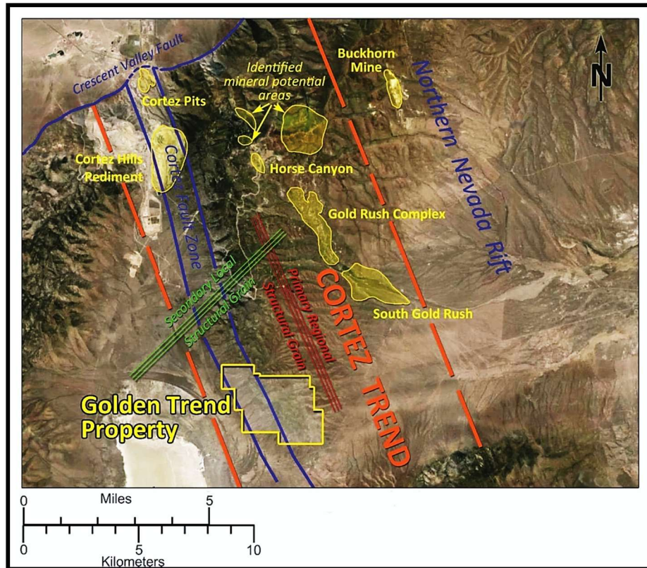
Figure 4 Deposits and mines in the district
