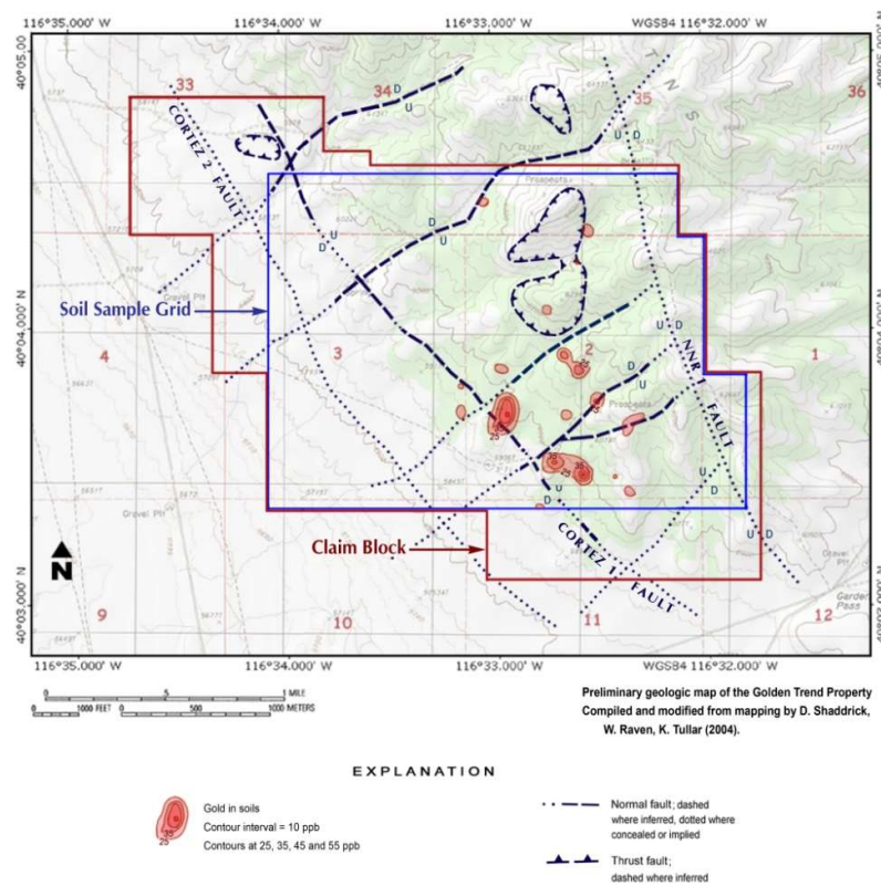
Gold in soils
