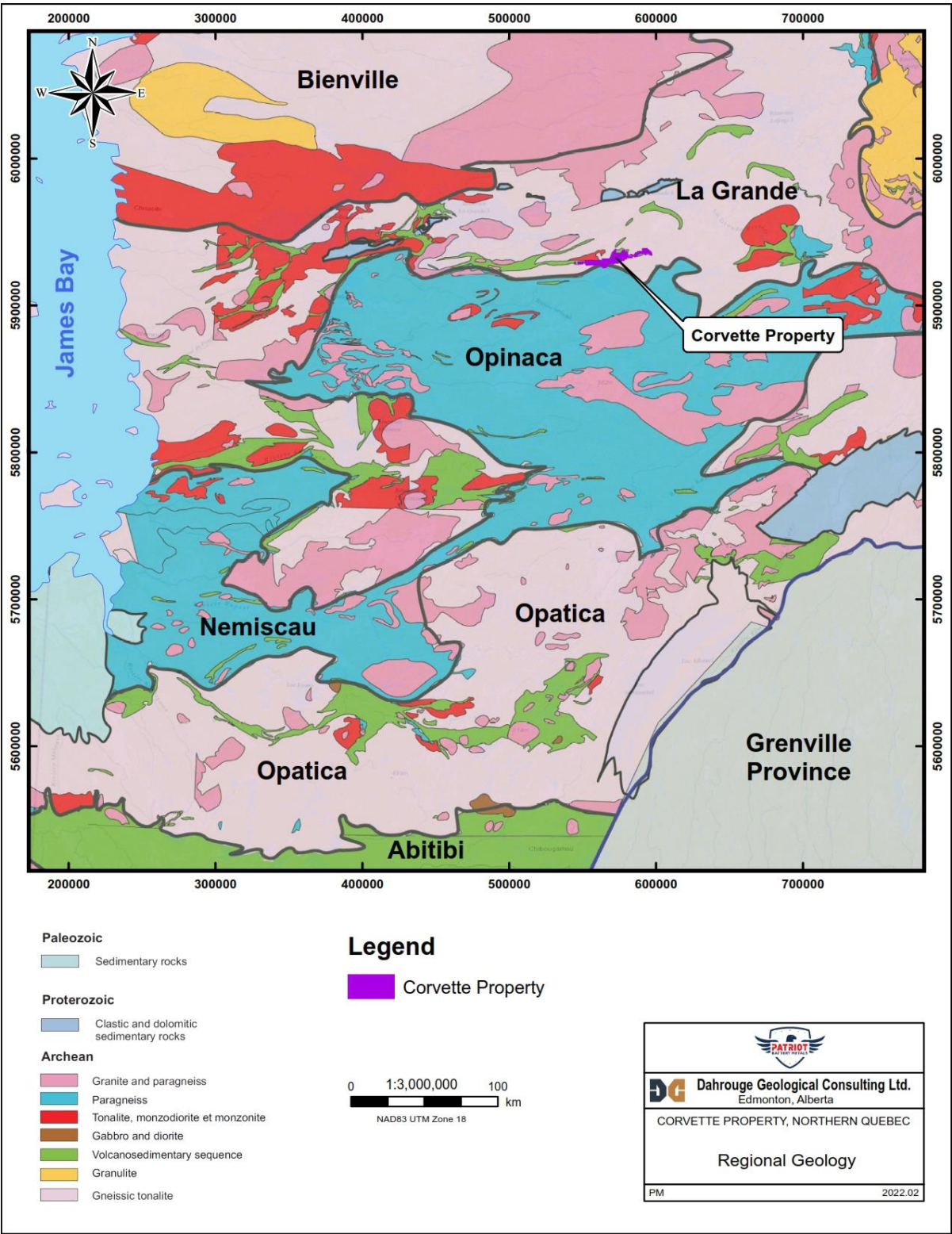
Figure 13: Regional geology
