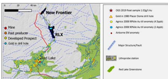
Figure 3: RLX property location map
