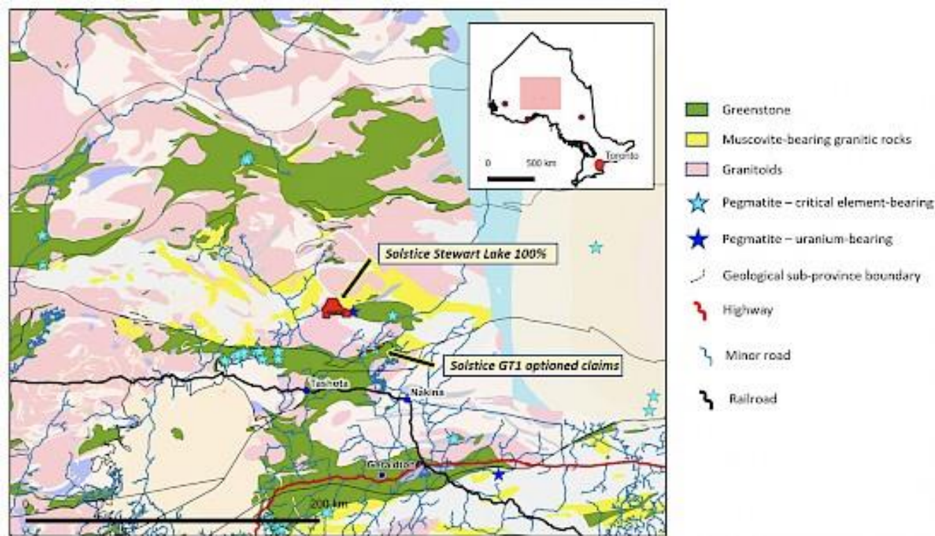
Figure 2. Location of the SLP project claims. Geological units from Ontario Geological Survey 2011. 1:250 000 scale bedrock geology of Ontario; Ontario Geological Survey, Miscellaneous Release—Data 126—Revision 1. Mineral occurrences from MNDM MDI mineral occurrence data
