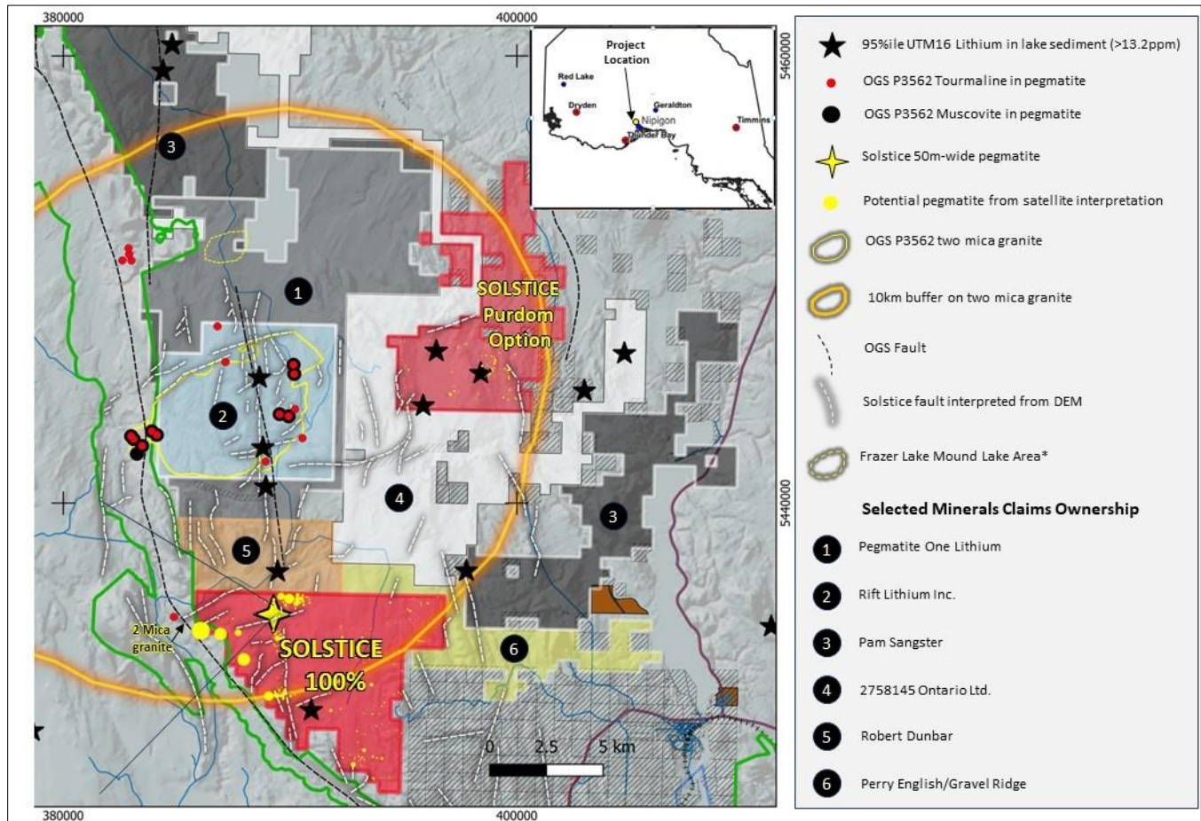
Figure 4. Map of the Project within the Frazer Mound Area.
