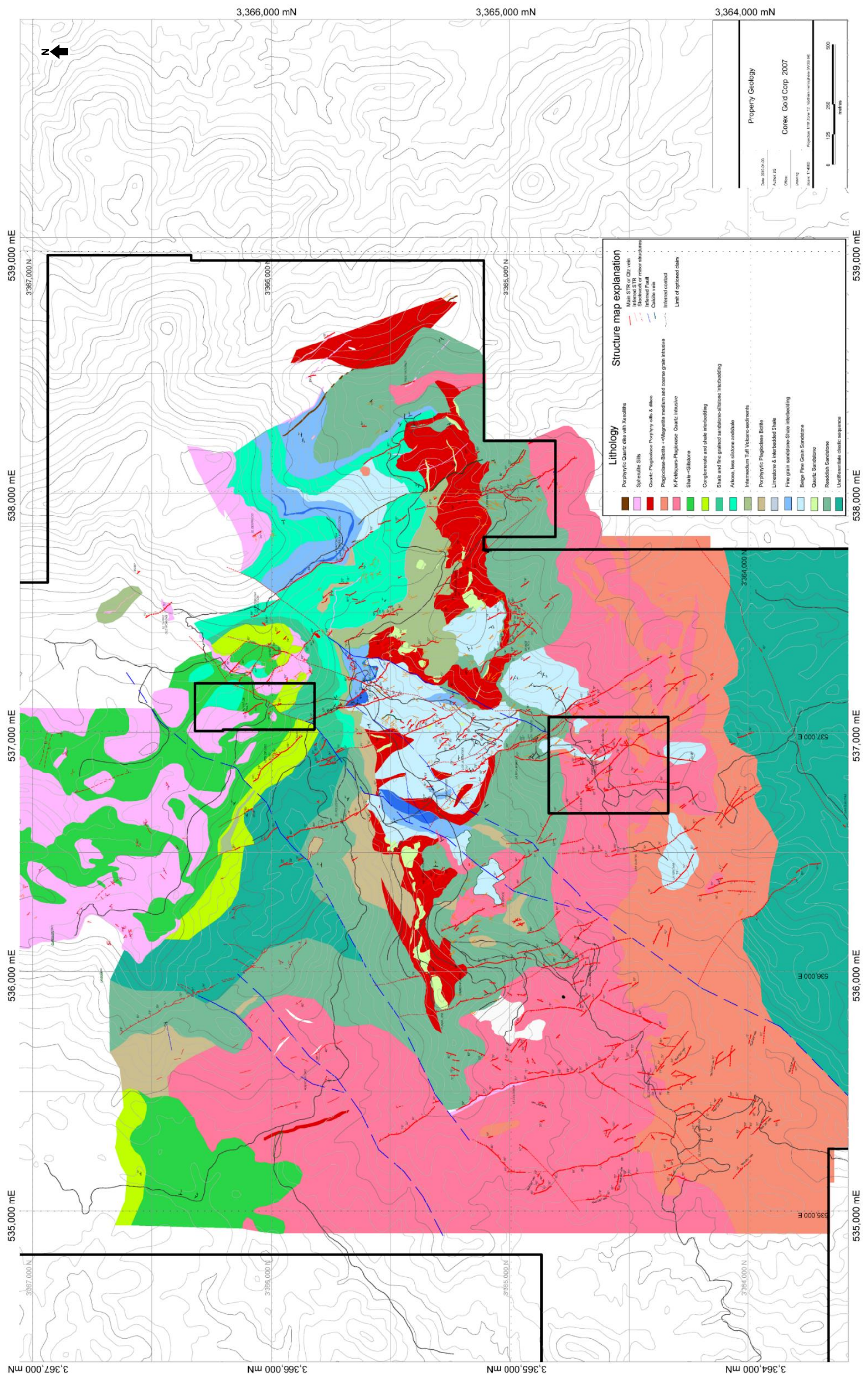
Figure 7-2: Property Geology
