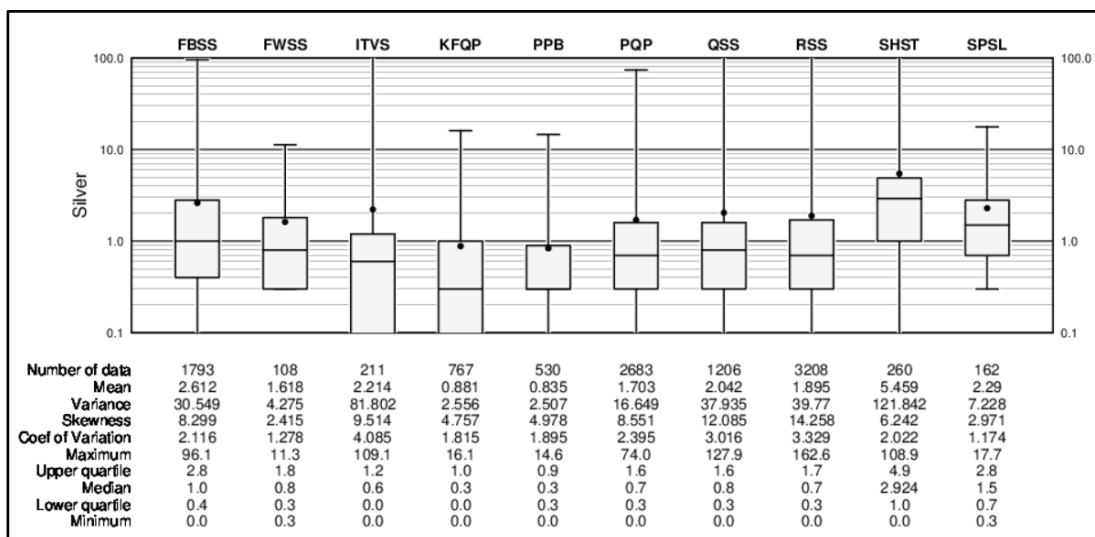
Figure 14-7: Boxplot of Silver by Lithology Type
