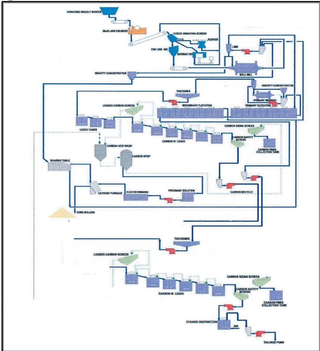
Figure 24-11 True Gold Mine Process Plant Flowsheet
