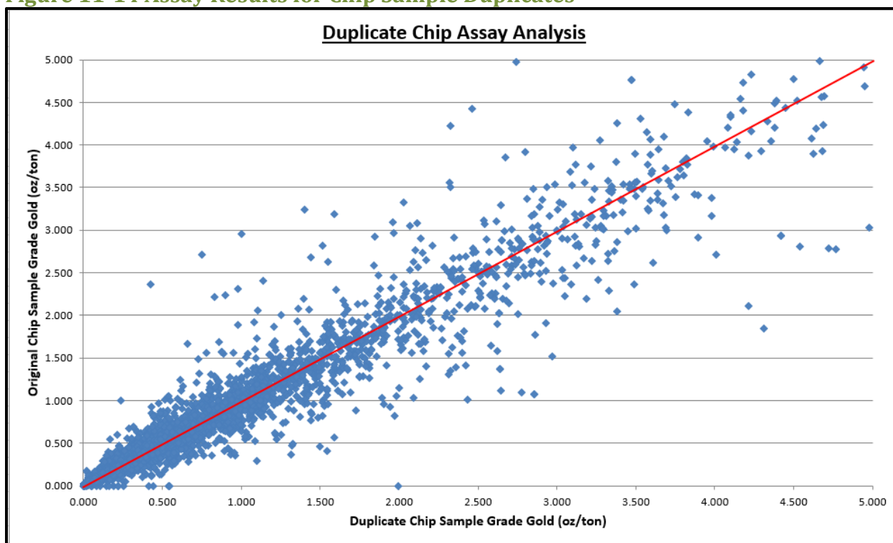
Figure 11-14 Assay Results for Chip Sample Duplicates
