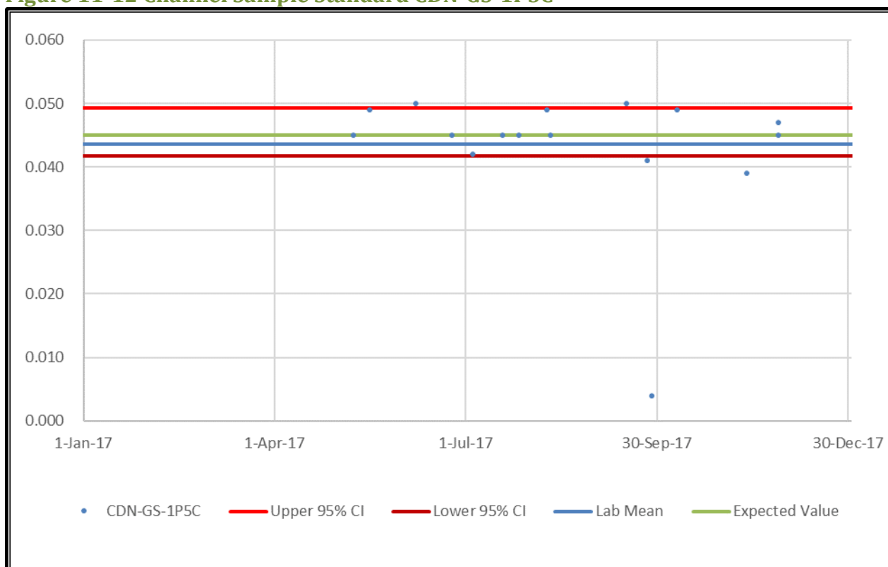
Figure 11-12 Channel Sample Standard CDN-GS-1P5C
