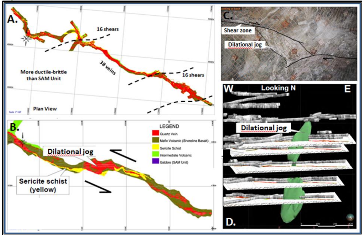
Figure 7-7 Controls on Gold Mineralization in the 007 Zone
