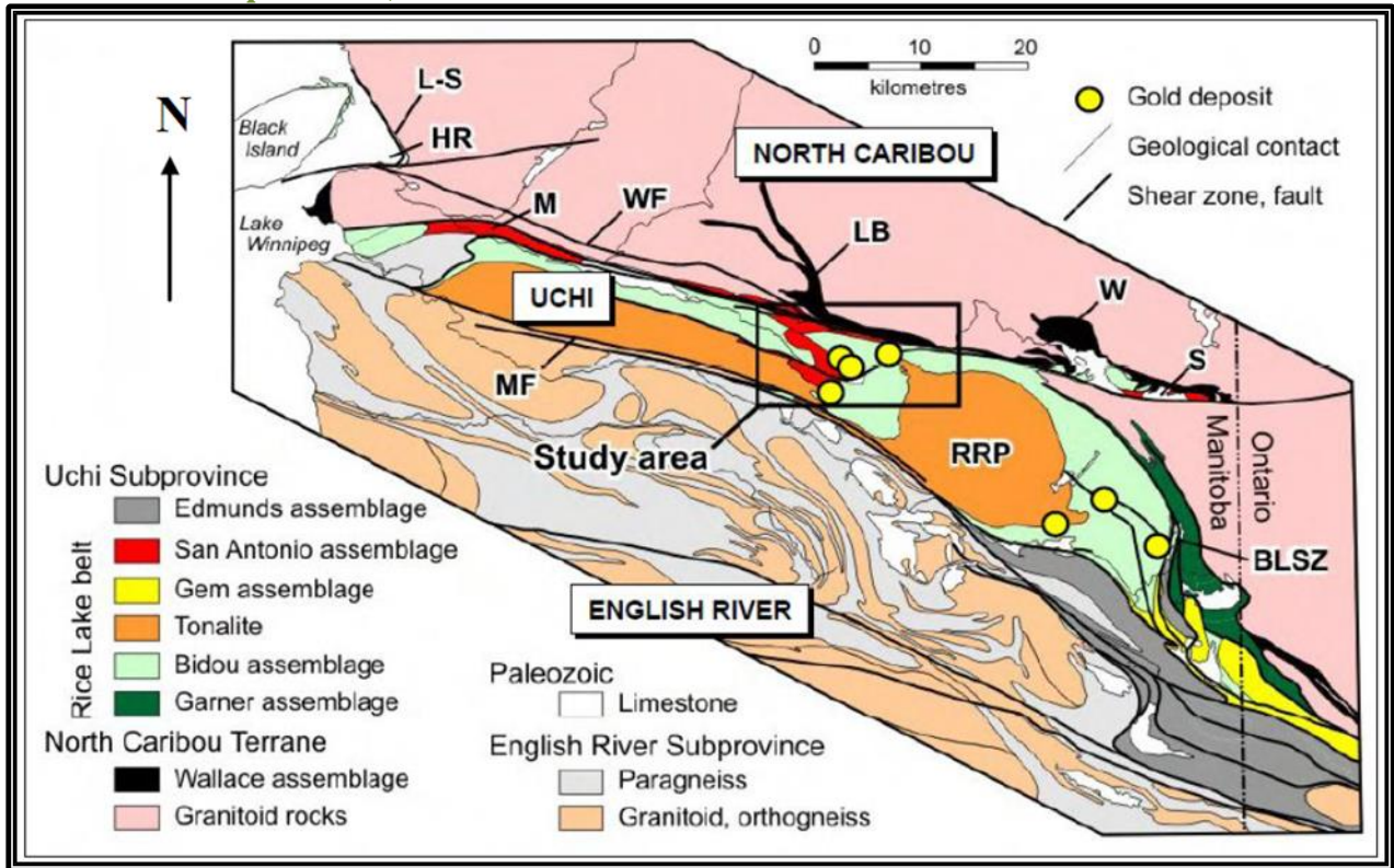
Figure 7-1 Regional Geologic Map showing the Location of True North Gold Mine in the Archean Uchi Subprovince, Manitoba
