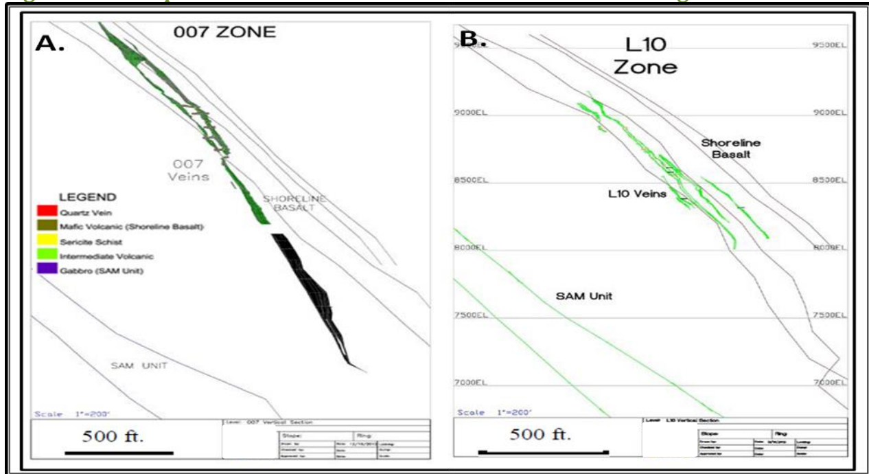
Figure 7-8 Interpreted Cross-Sections of 007 and L10 Zones Looking West
