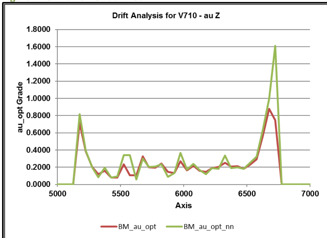
Figure 14-5 710 Vein Swath Plot Z
