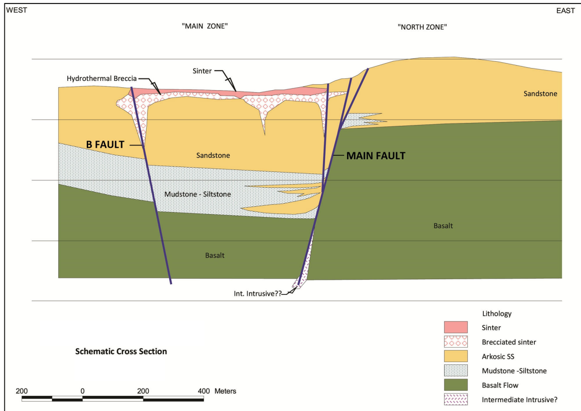
Figure 7.3 Almaden Schematic Cross-Section
