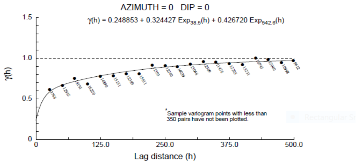
Figure 14.3 Almaden Variogram
