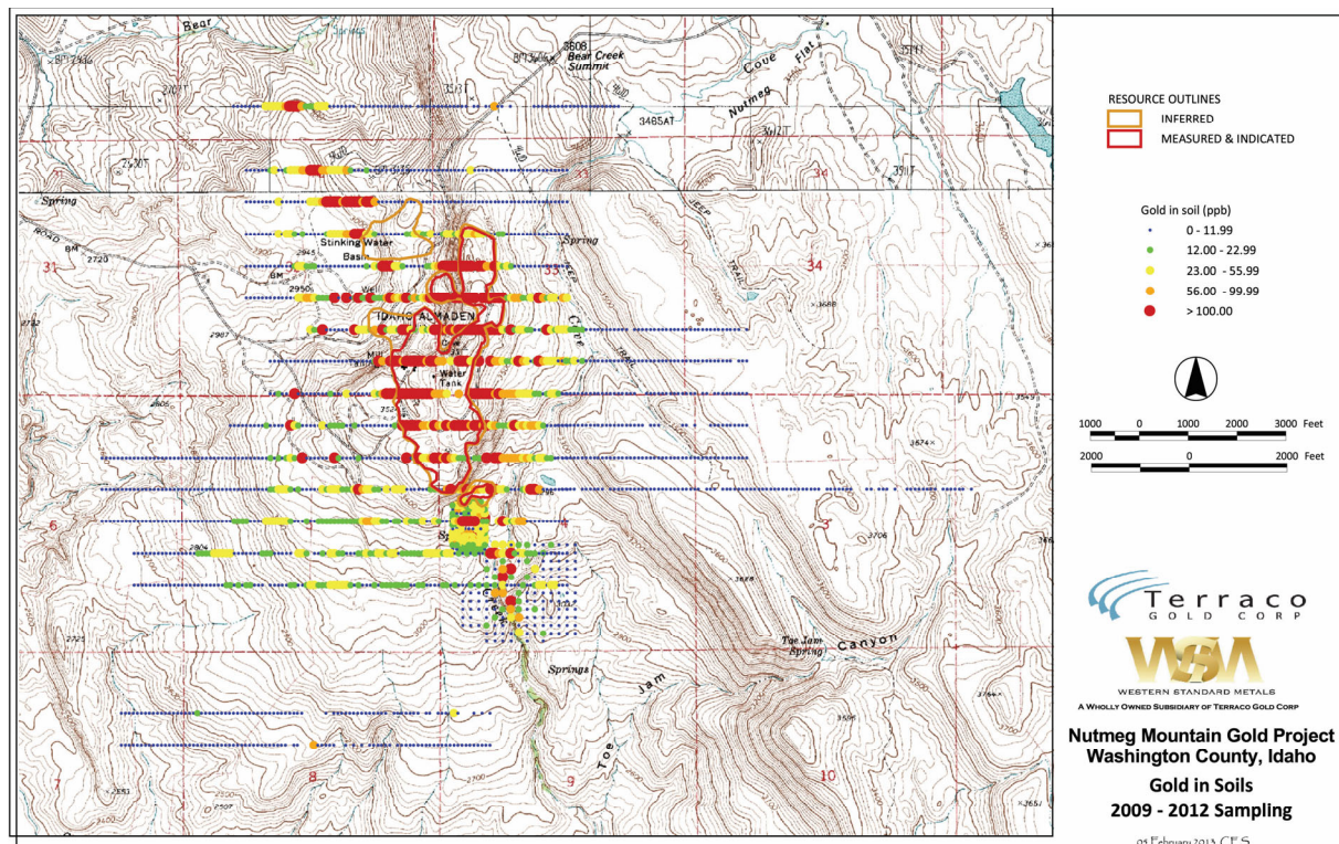
Figure 6.1 Almaden Soil Sampling Grid and Gold Anomalies
