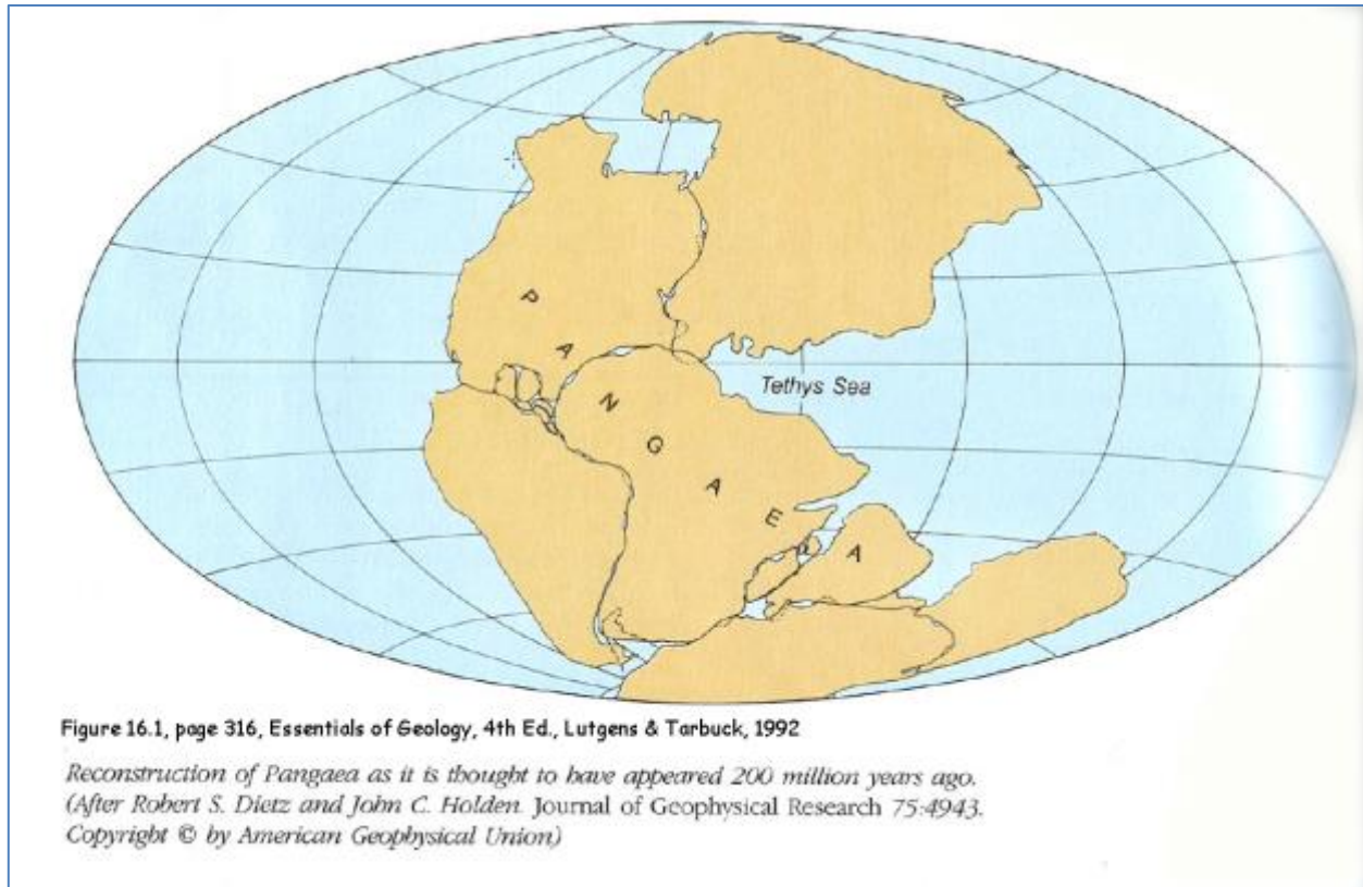
Figure 7-3: The Closure of the Atlantic Creating the Supercontinent Pangea. Meguma Rocks Folded and Stuck to North America. (Lutgens and Tarbuck, 1992)
