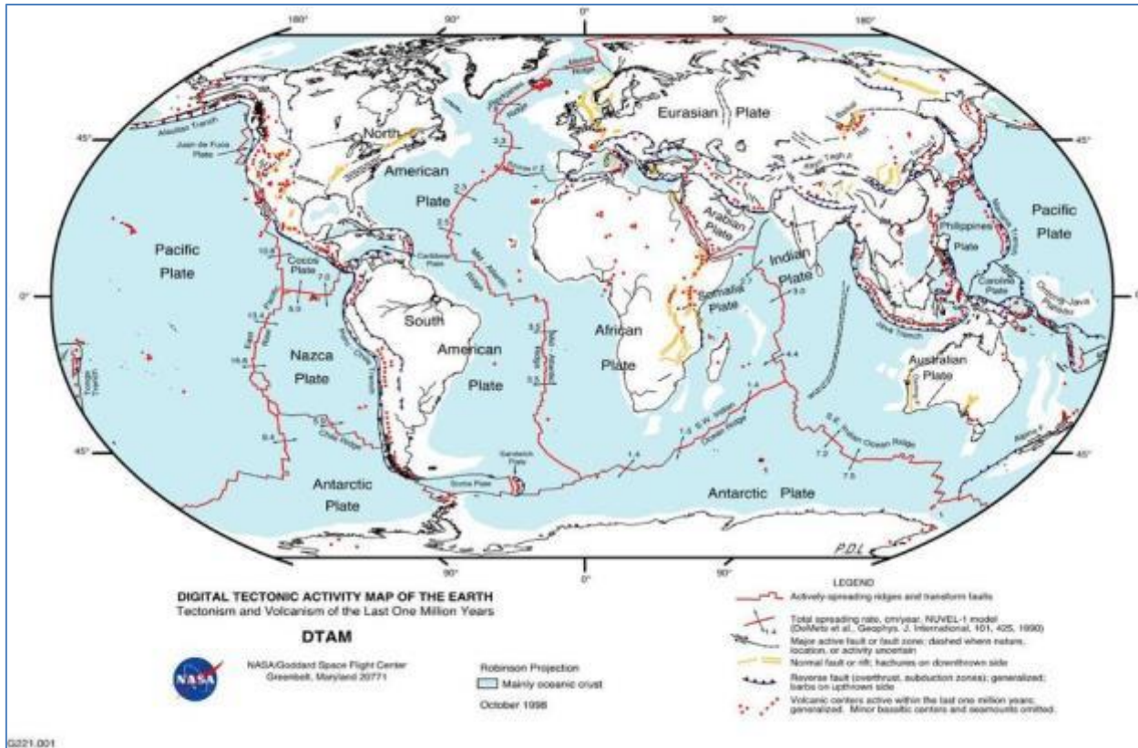
Figure 7-2: Tectonism and Volcanism of the Last Million Years, Tectonic Plate Boundaries (NASA, DTAM, 1998)
