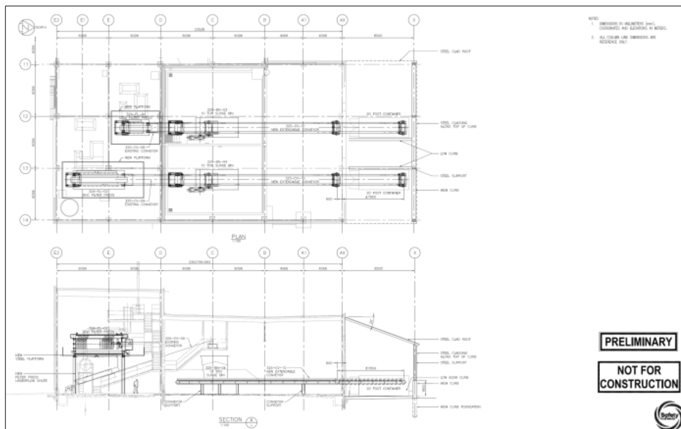
Figure 17-6: Dewatering and Concentrate Handling Section
