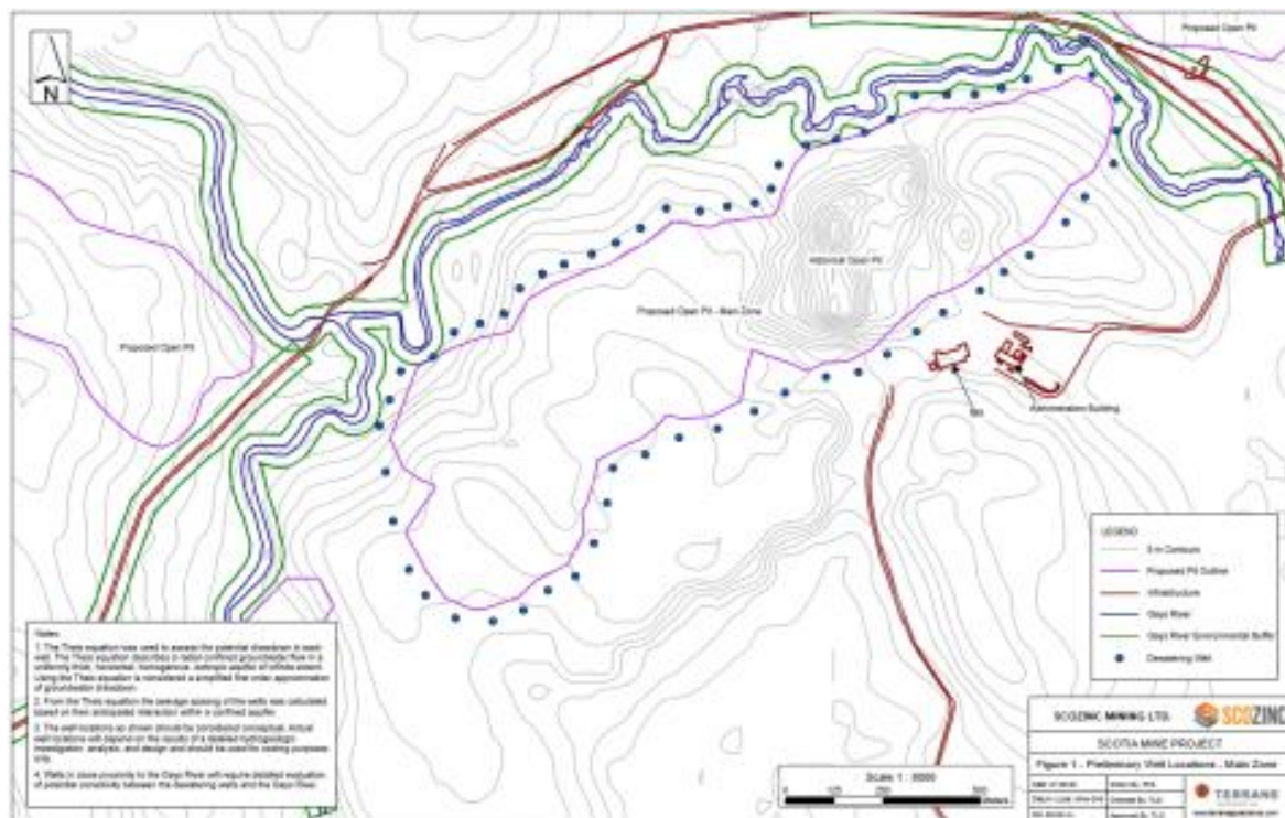
Figure 16-28: Overburden Slope Depressurizing Well Locations
