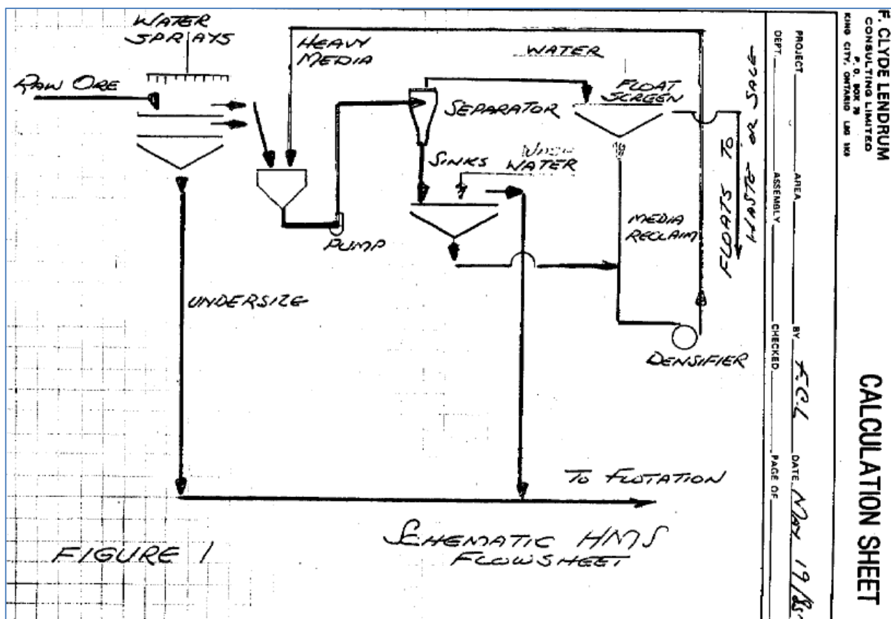
Figure 6-1: Schematic Flowsheet for Sink/Float Testing (from Lane et al, 1986)
