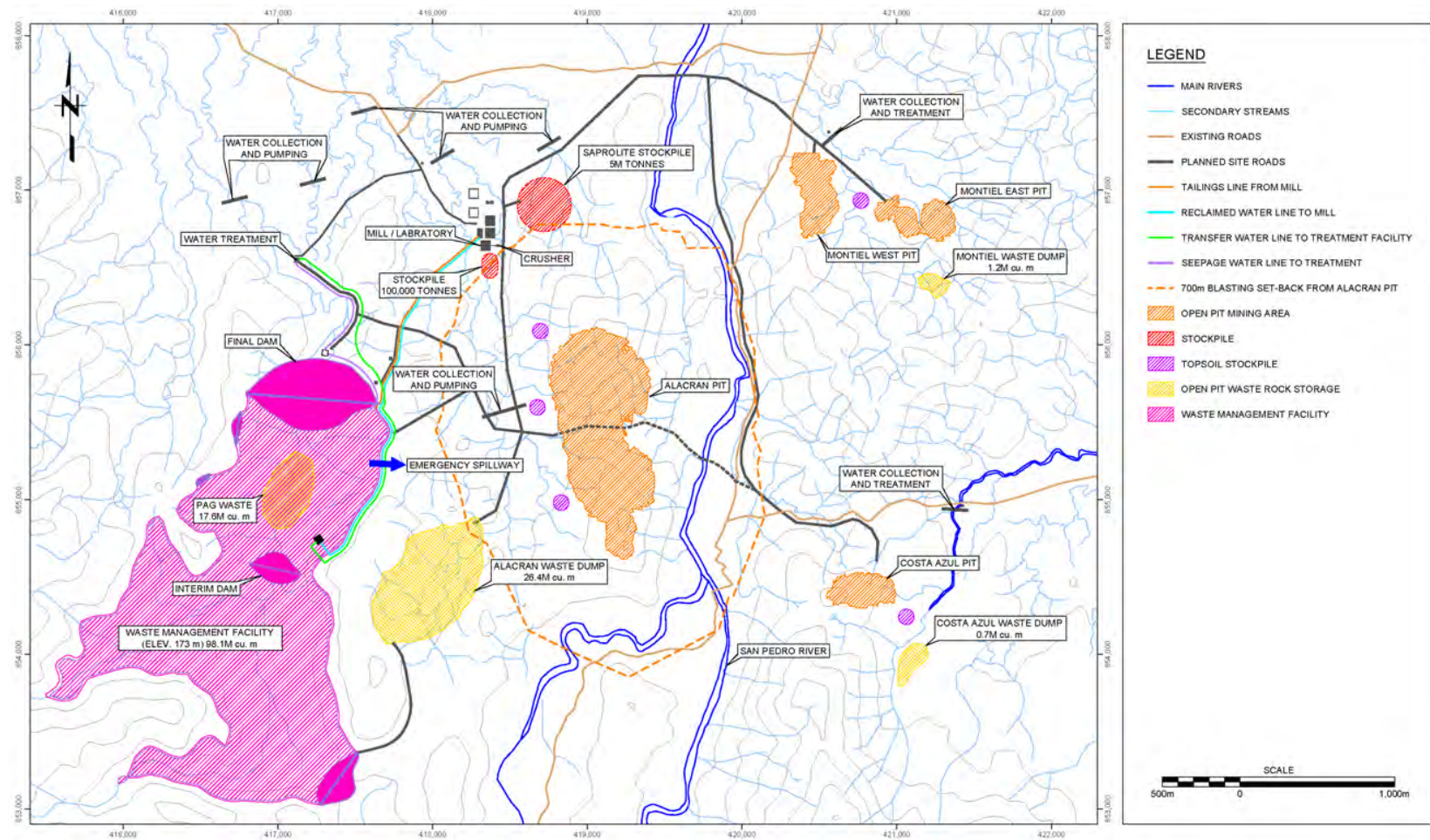
Figure 18-1: Site conceptual general arrangement
