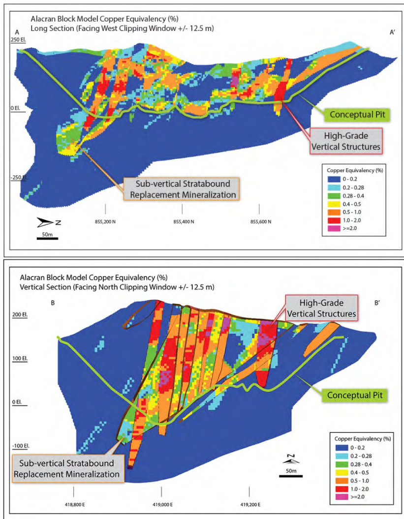
Figure 14-42: July 2019 PEA Alacran conceptual open pit
