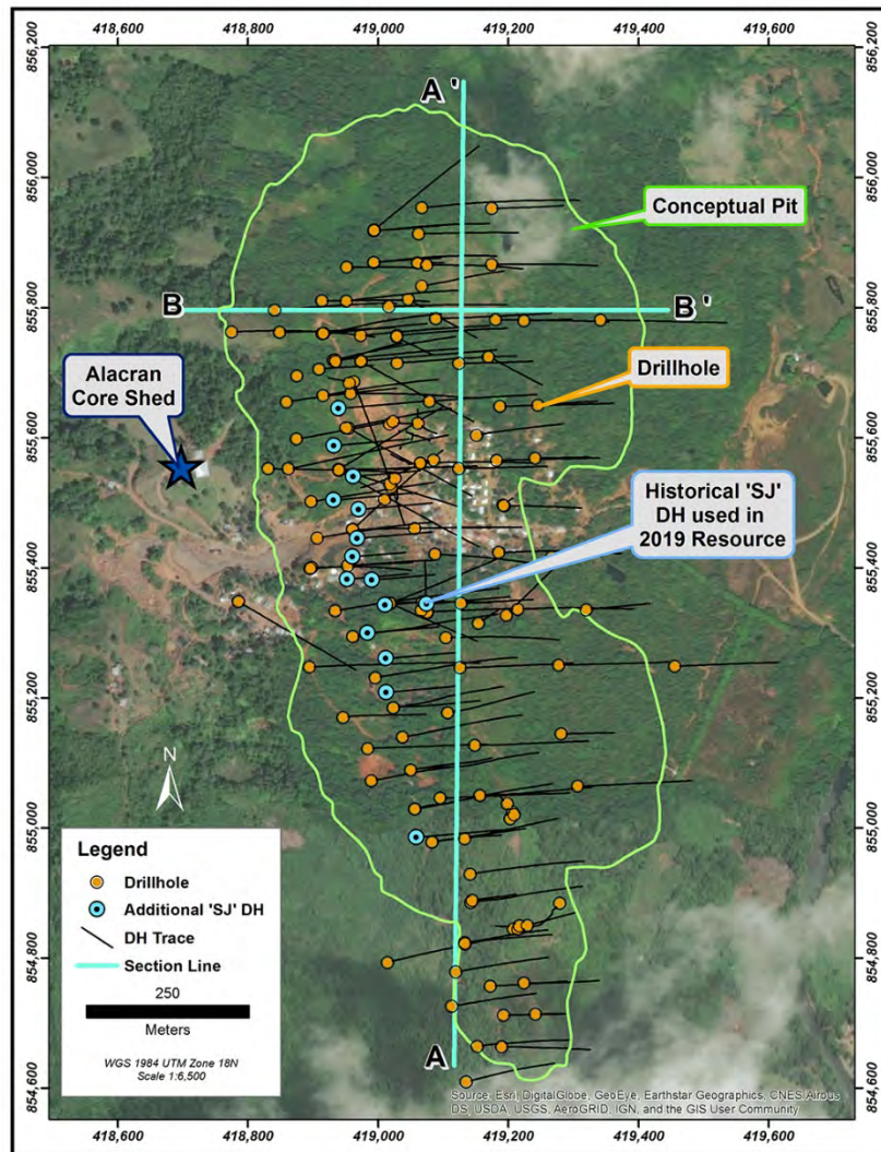
Figure 14-42: July 2019 PEA Alacran conceptual open pit
