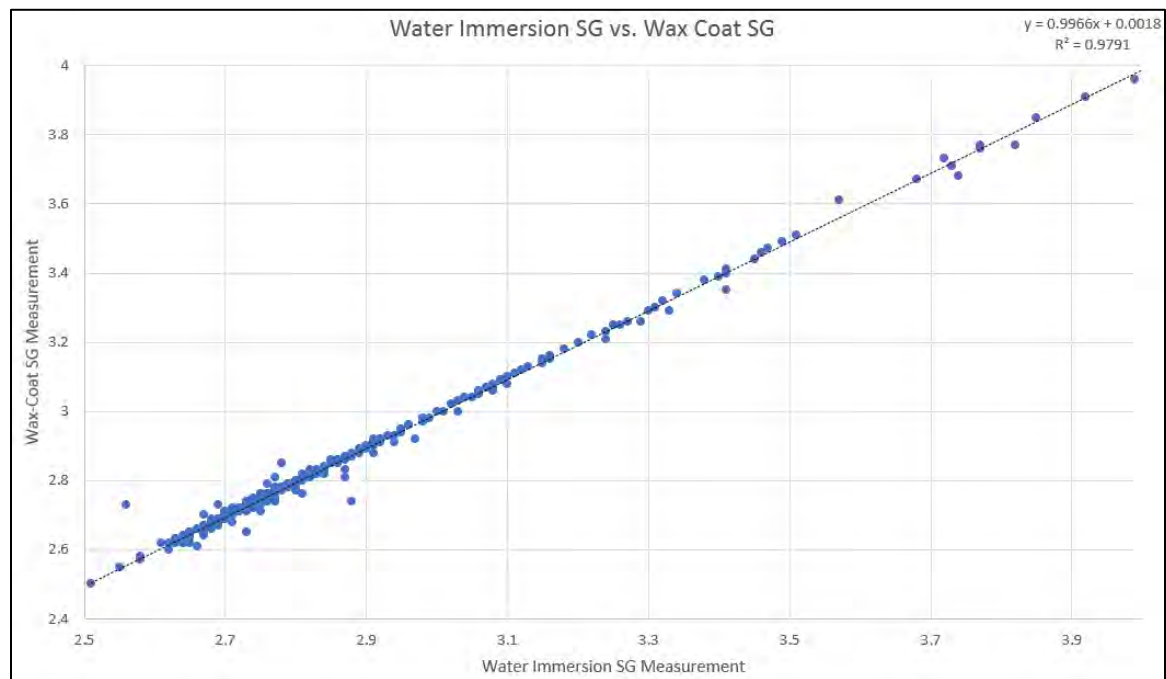
Figure 10-4: Wax Coat SG measurement accuracy analysis
