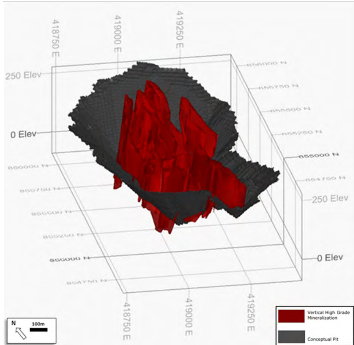
Figure 14-3: Vertical high-grade mineralization wireframes with conceptual open pit
