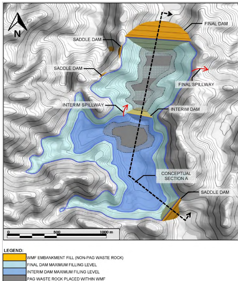
Figure 18-7: WMF conceptual arrangement
