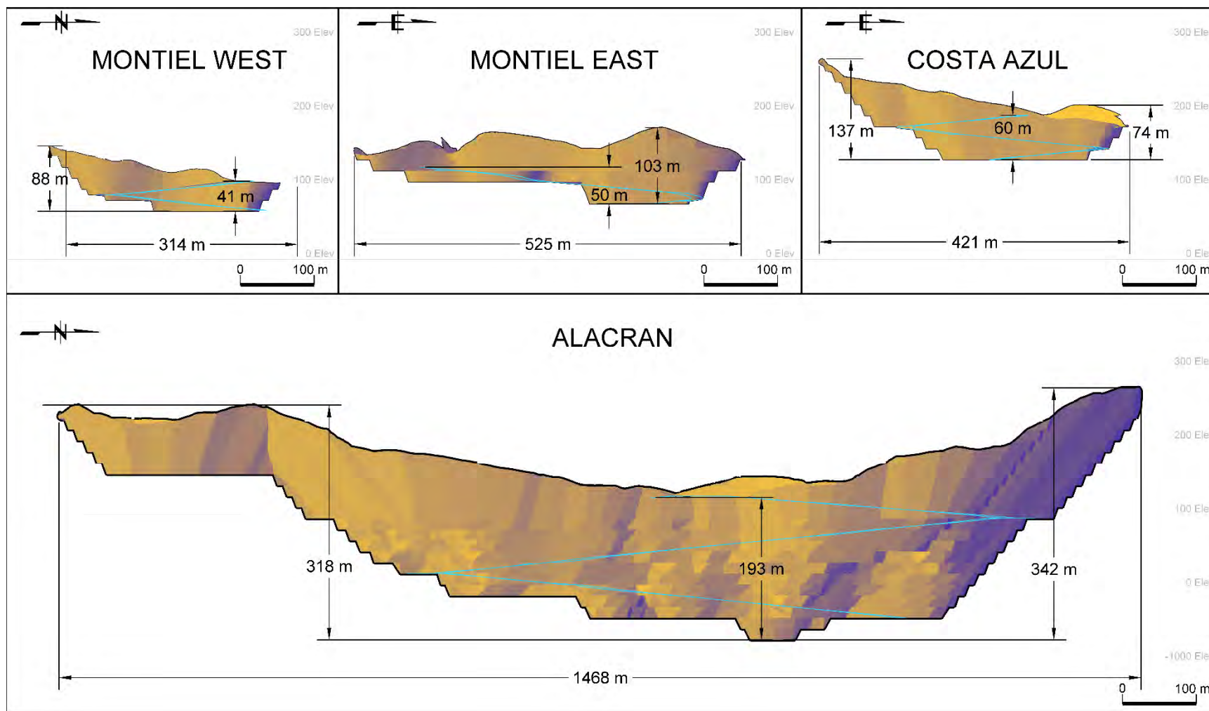
Figure 16-13: Conceptual pit long sections
