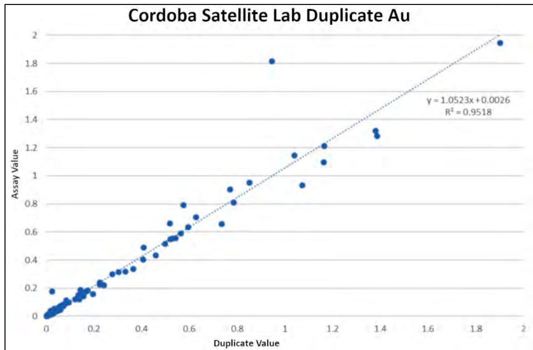
Figure 11-34: Lab duplicates (coarse reject and pulp), for Au (g/t) by Cordoba for the satellite deposits
