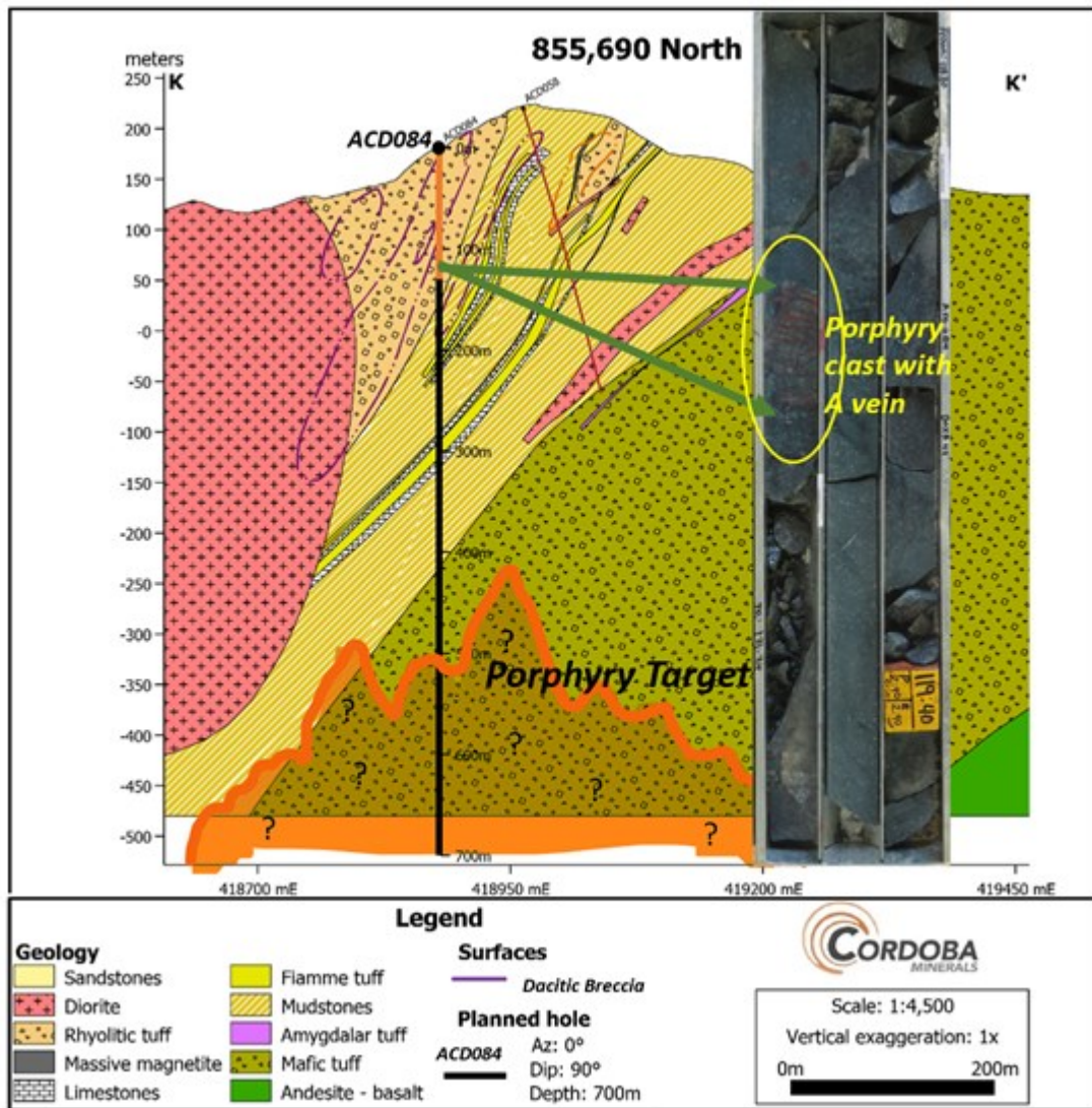
Figure 3: Schematic geological section with evidence of porphyry clasts identified in ACD084 from previous exploration program.
