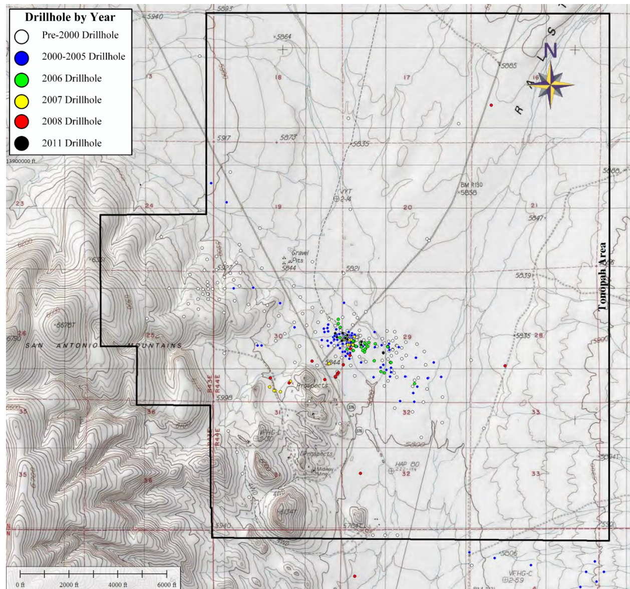
Figure 10-1: Exploration Drilling at the Tonopah Project
