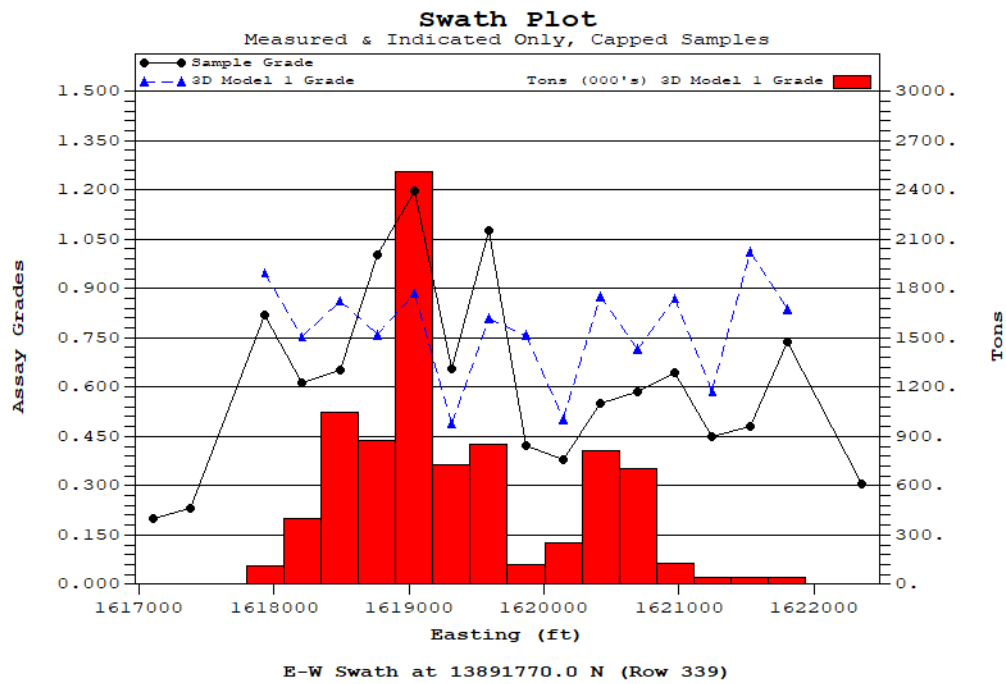
Figure 14-18: Swath Plot by Easting
