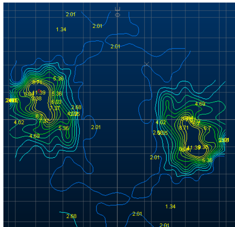
Figure 14-9: CZD variogram map, plan view
