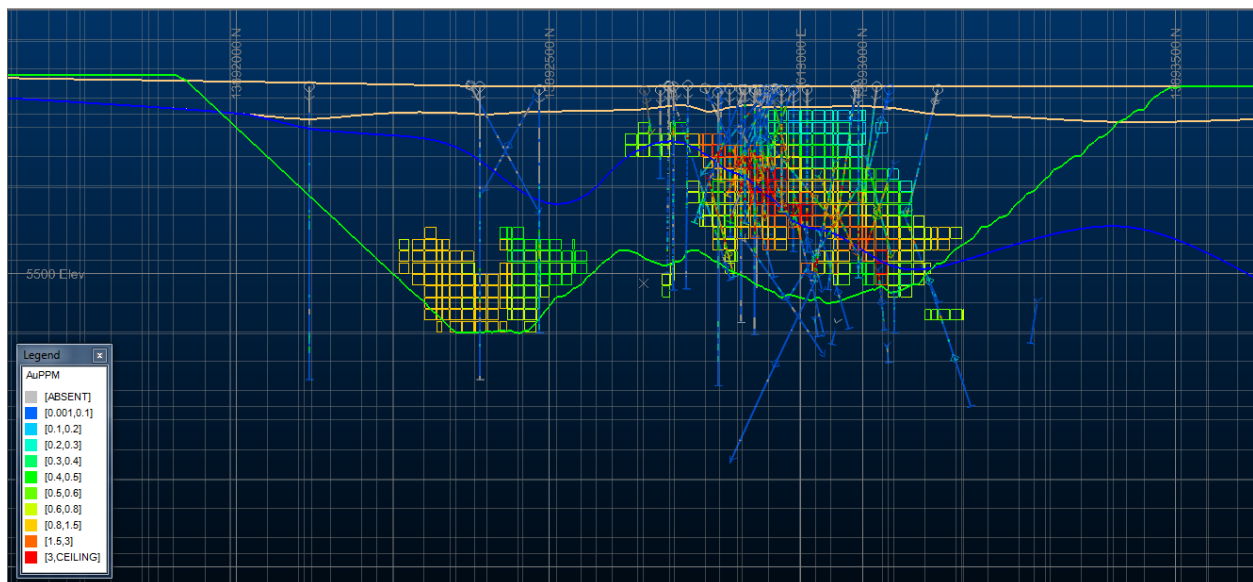
Figure 14-13: Example Cross Section (Looking N60W) through Tonopah block model (Discovery Area). Showing MII blocks and pit trace for reference.
