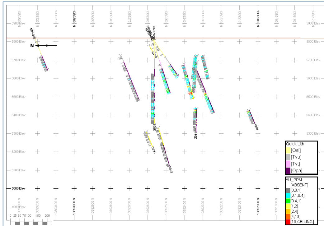
Figure 10-3: NS21 Section, 63-77 / PointLuck
