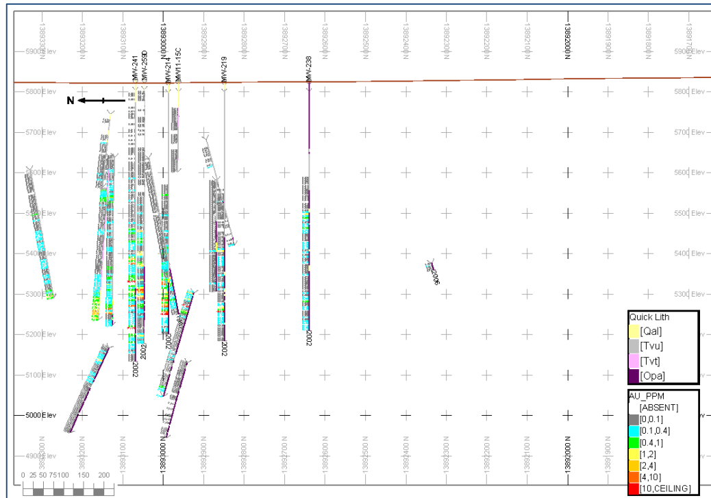
Figure 10-7: NS41 Section, 121 Zone
