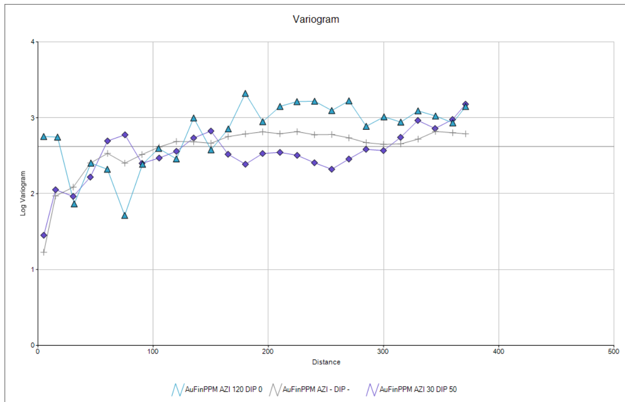
Figure 14-10: Experimental Variograms, PZX zone
