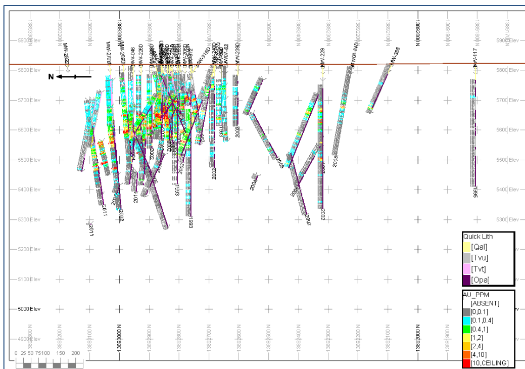
Figure 10-6: NS36 Section, Discovery Zone
