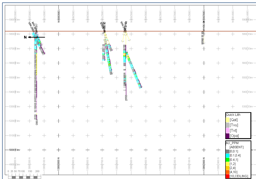
Figure 10-4: NS26 Section, 63-77 Zone
