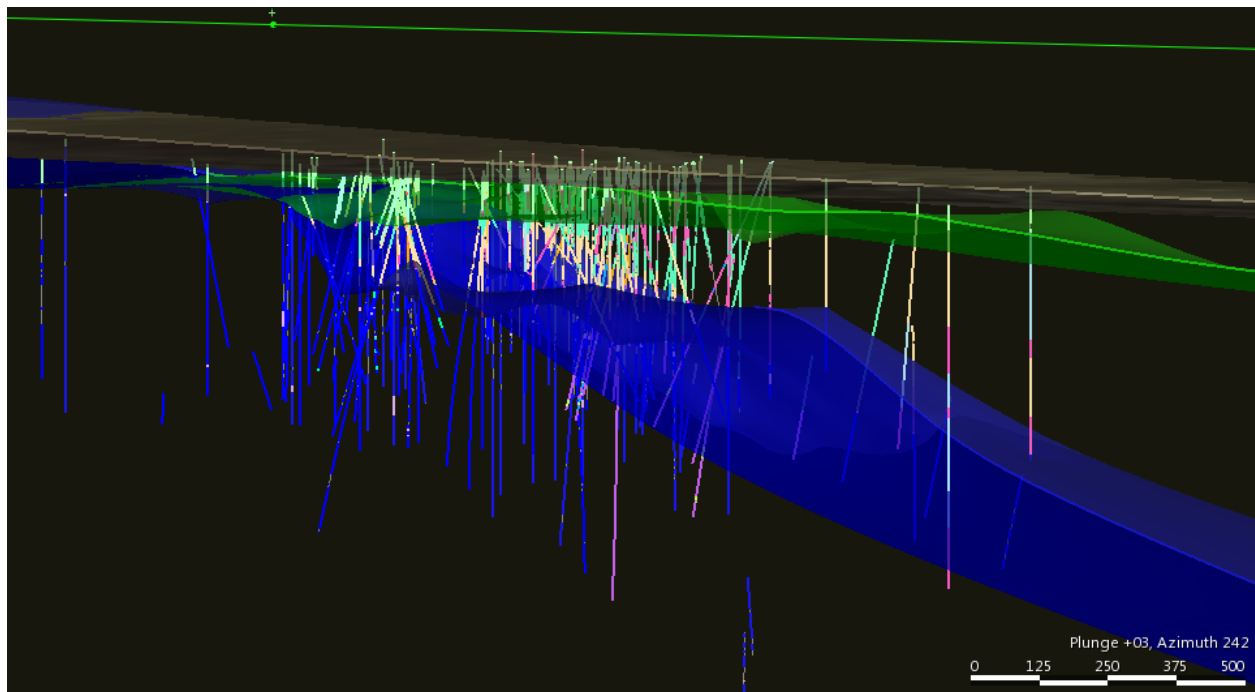
Figure 14-1: Cross section slice showing Opa upper surface (blue) and Tv Upper Surface (green) (Az 242) Scale in feet.
