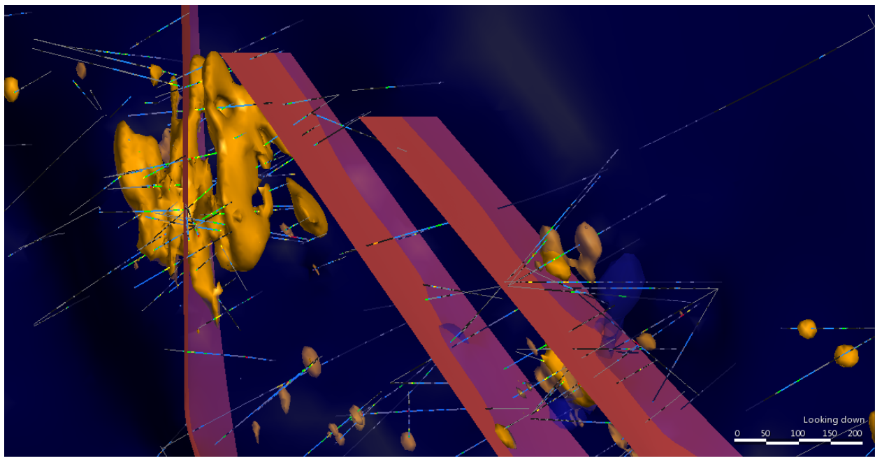
Figure 14-4: Plan view (North is top of page) showing CZD solids (orange) relative to drill data and interpreted conjugate structures. Scale in feet.
