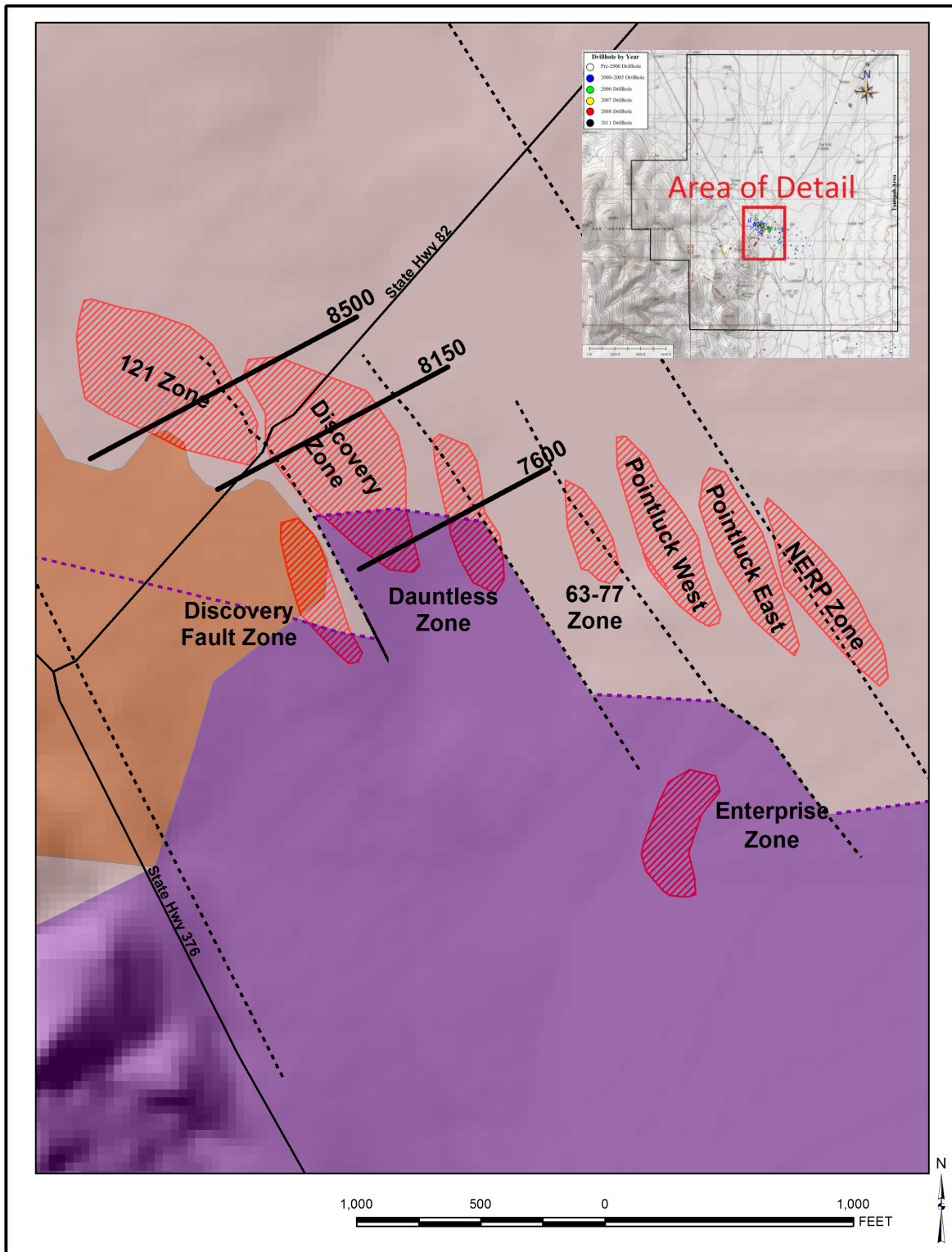
Figure 7-4: Mineralized Zones at the Tonopah project, and cross section traces for Section Lines. Section 8500 corresponds to Figure 7-6Error! Reference source not found. Section 8150 corresponds to Figure 7-5Error! Reference source not found. Section 7600 corresponds to Figure 7-7Error! Reference source not found. (Podratz & LeLacheur, 2014)
