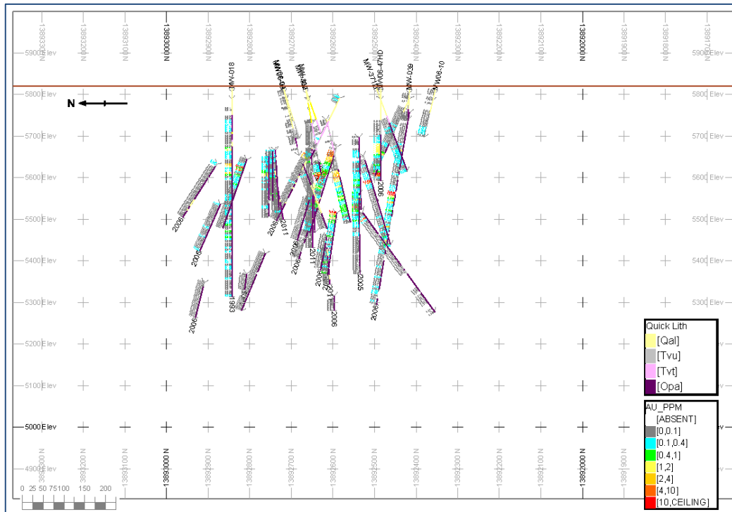
Figure 10-5: NS30 Section, Dauntless Zone
