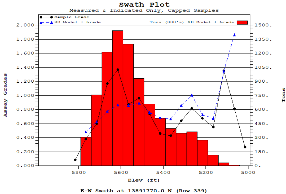
Figure 14-17: Swath Plot by Elevation
