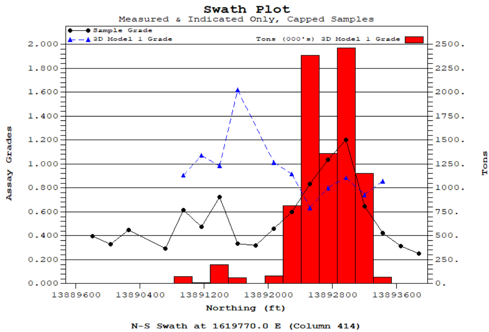
Figure 14-19: Swath Plot by Northing
