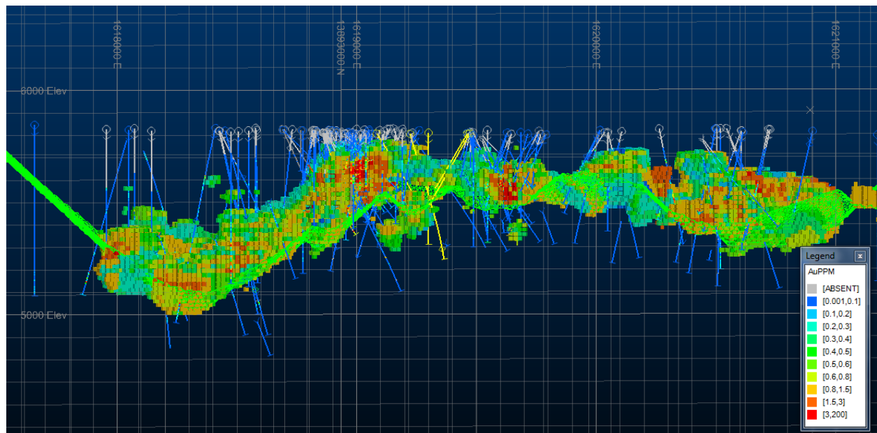
Figure 14-11: Long Section view showing drill holes, estimated blocks, and pit shell used to constrain resource estimate. Blocks outside the pit shell are not included in the resource.
