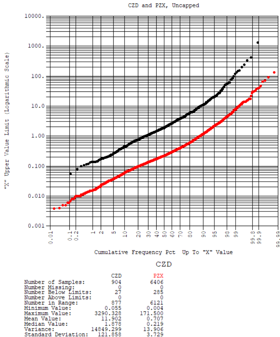
Figure 14-7: CZD and PZX domains Cumulative Frequency Plots
