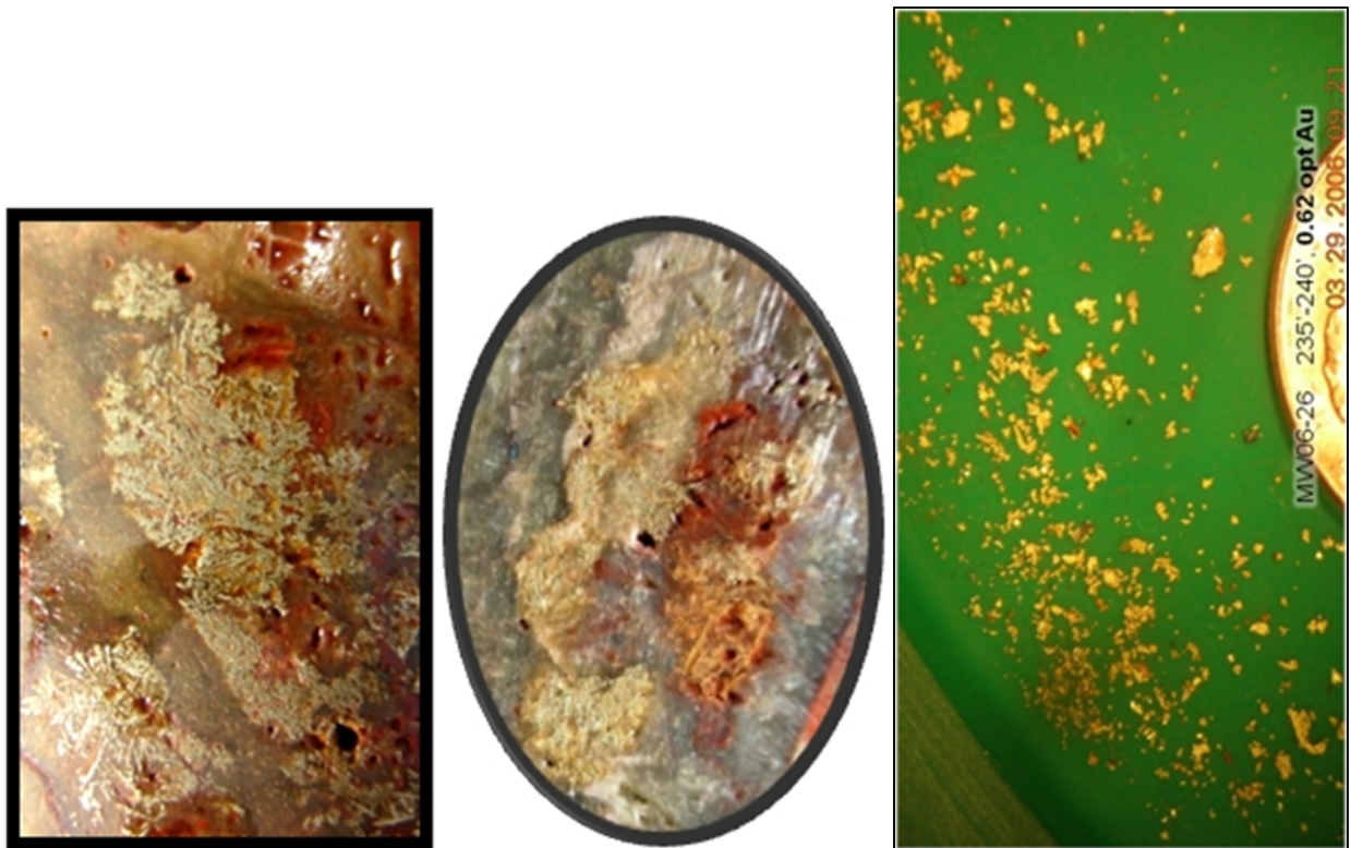
Figure 7-9: Visible Gold from Tonopah Project
