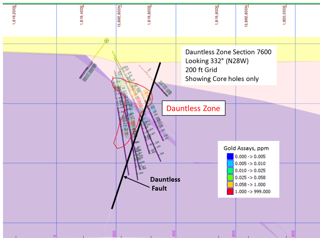
Figure 7-7: Cross Section showing Dauntless Zone Mineralization
