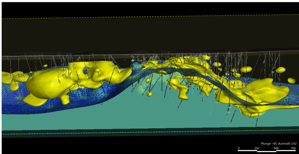
Figure 14-3: Long Section view showing interpreted Primary Zone Domain (PZD, Yellow) log grade shell at 0.150 ppm Au. Azimuth 192, Scale in feet.
