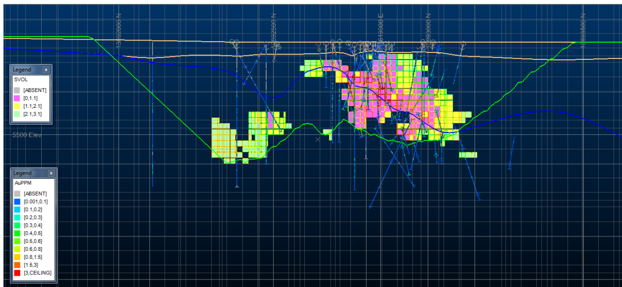
Figure 14-15: Example Cross Section (Looking N60W) through Tonopah Plock Model (Discovery Zone). Showing SVOL (classification) and pit trace for reference.
