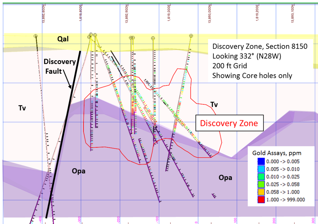
Figure 7-5: Cross Section through Discovery Zone (Section 8150 from Figure 7-4) (Podratz & LeLacheur, 2014)
