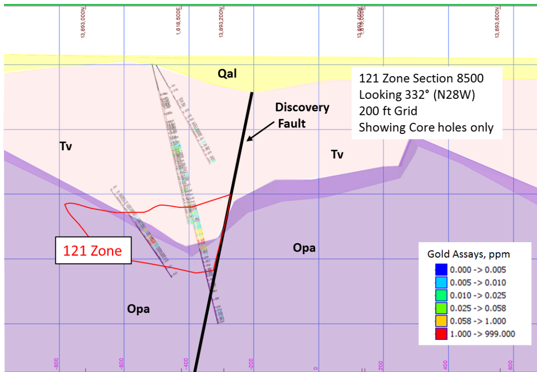
Figure 7-6: Cross Section through 121 zone Mineralization (Section 8500 from Figure 7-4) (Podratz & LeLacheur, 2014)
