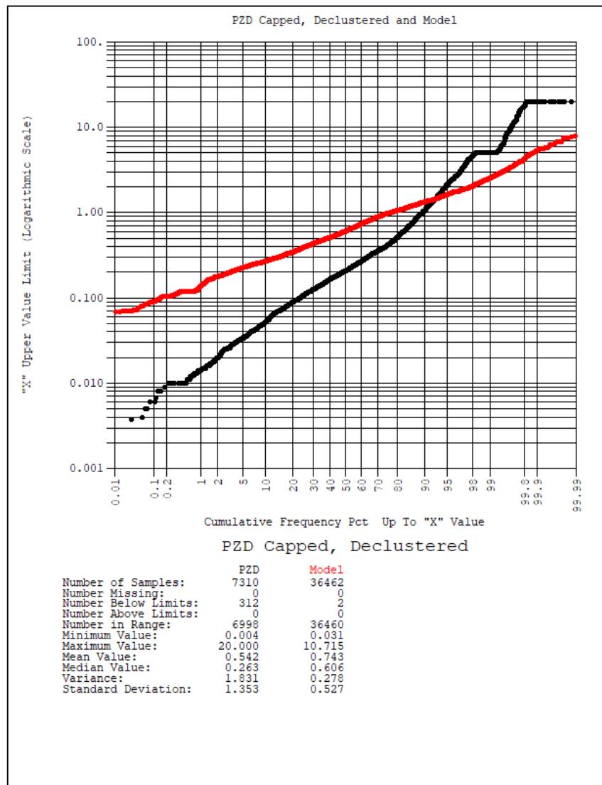
Figure 14-16: PZD composites and MII Resource Block grades, CFP Comparison.
