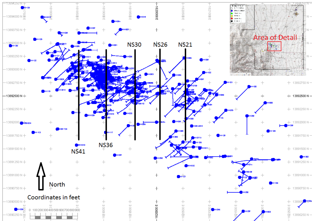
Figure 10-2: Drill Cross Section Traces
