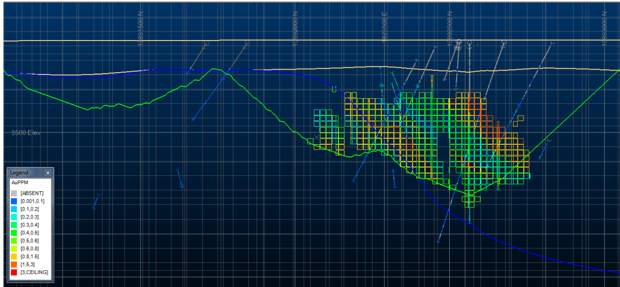
Figure 14-12: Example Cross Section (Looking N60W) through Tonopah block model. Showing MII blocks and pit trace for reference
