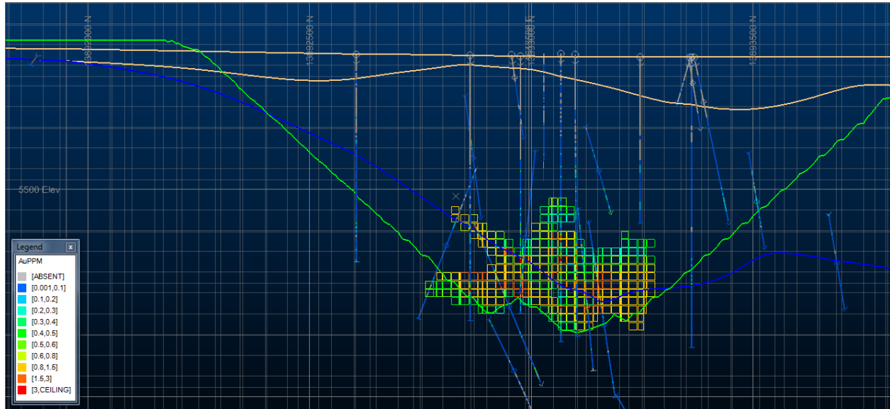
Figure 14-14: Example Cross Section (Looking N60W) through Tonopah block model (121 Area). Showing MII blocks and pit trace for reference
