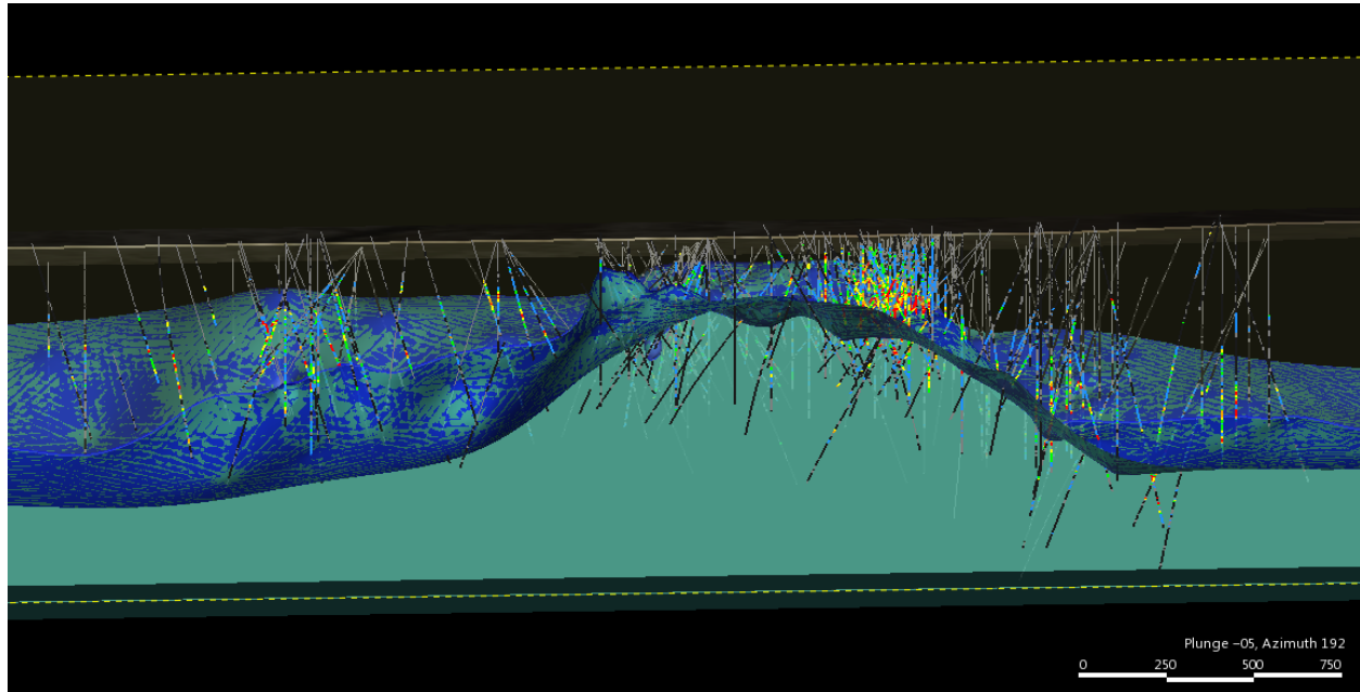
Figure 14-2: Long section view showing mineralization relative to Opa /Tv boundary surface. Az 192. Scale in feet.
