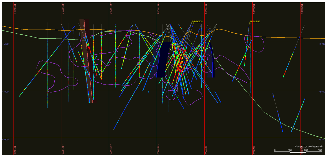
Figure 10-5: Cross Section through Discovery (Left) and Dauntless Zone (Center) Mineralization with 2018-2019 drill holes identified in gold text (Section B-B' from Figure 7-4)
