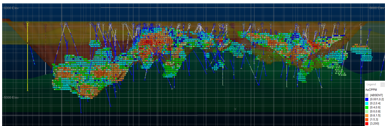
Figure 14-11: Long Section (Looking N20E) view showing drill holes, estimated blocks, and pit shell used to constrain resource estimate. Blocks outside the pit shell are not included in the resource.
