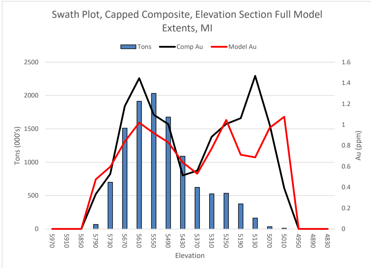
Figure 14-19: Swath Plot by Elevation
