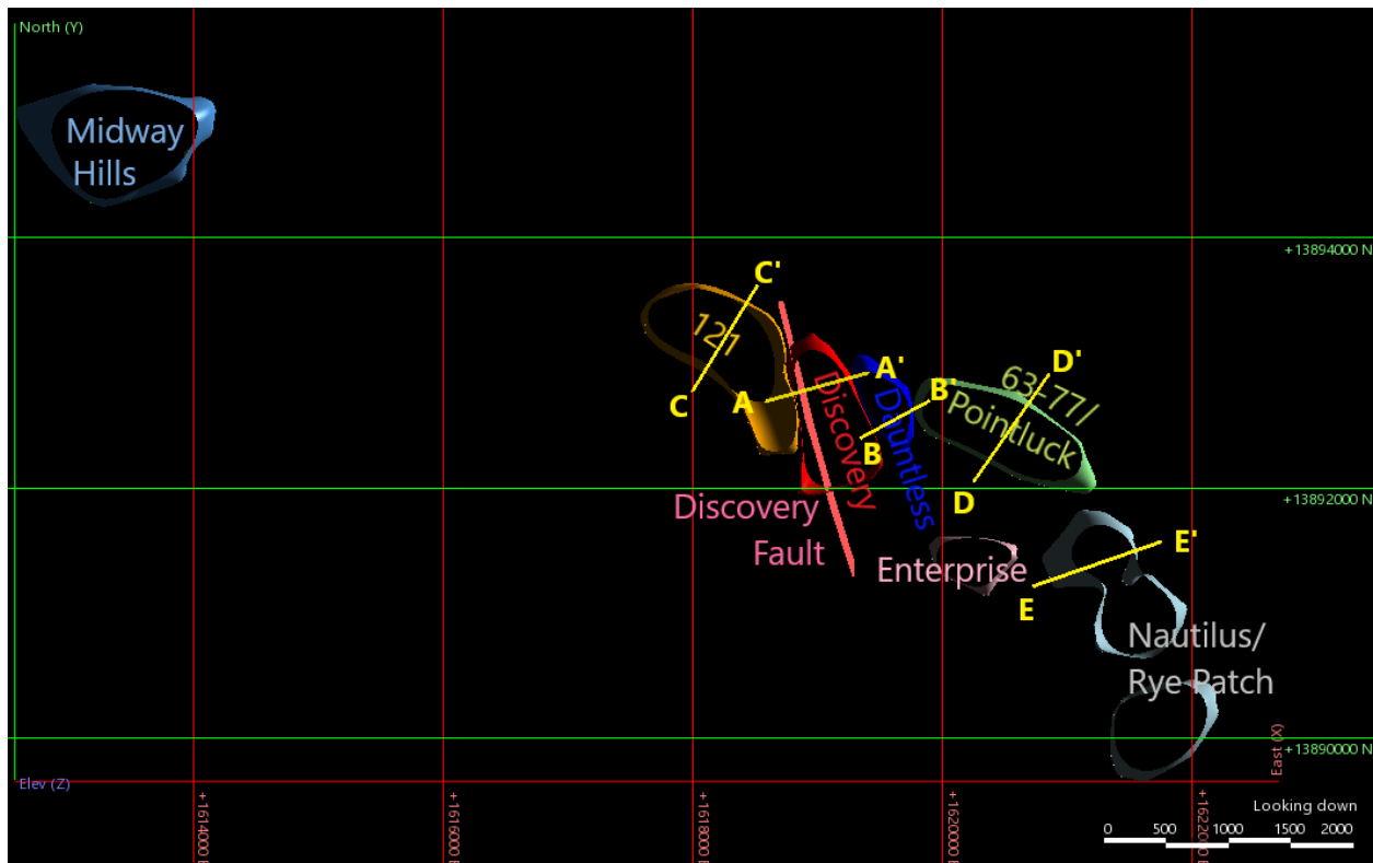
Figure 7-4: Mineralized Zones at the Tonopah project, and cross section traces for Section Lines. Section A-A' corresponds to Figure 10-4 Section B-B' corresponds to Figure 10-5, Section C-C' corresponds to Figure 10-6, Section D-D' corresponds to Figure 10-7, and Section E-E' corresponds to Figure 10-8.
