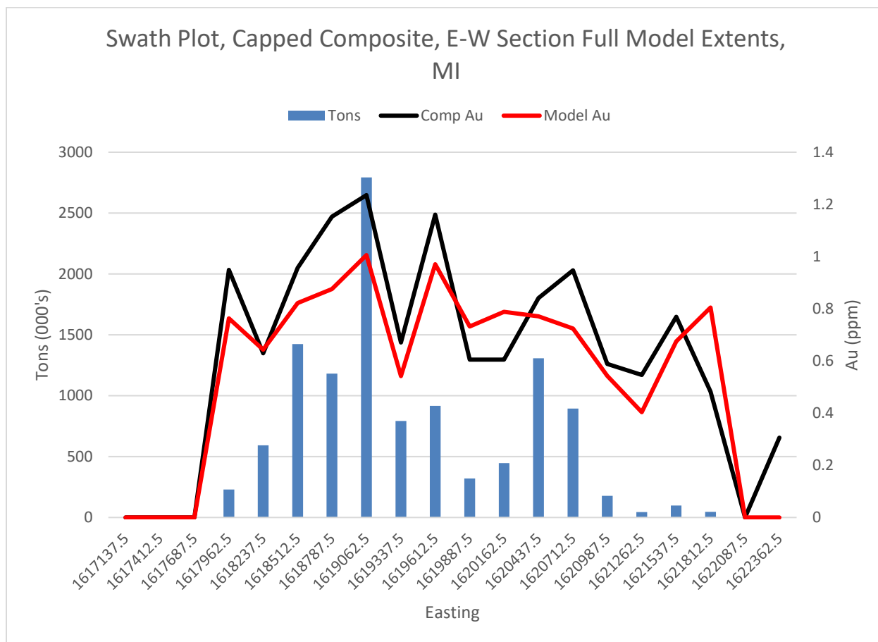
Figure 14-20: Swath Plot by Easting
