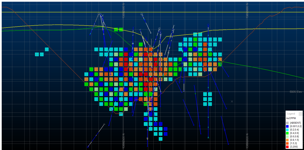
Figure 14-12: Example Cross Section (Looking W) through Tonopah block model (Dauntless Zone). Showing MII blocks and pit trace for reference (Blocks are 20 feet on center)
