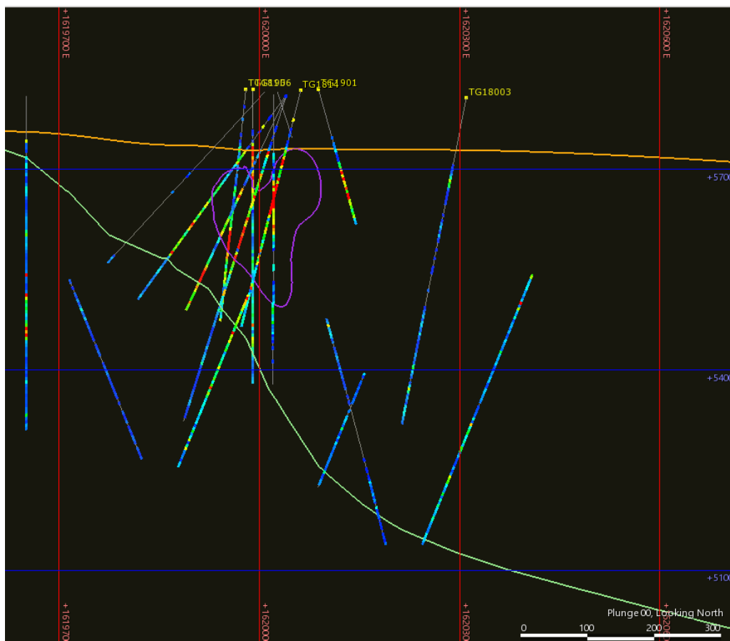
Figure 10-7: Cross Section showing 63-77/Pointluck Zone Mineralization with 2018-2019 drill hole collars identified in gold text. (Section D-D' from Figure 10-3)
