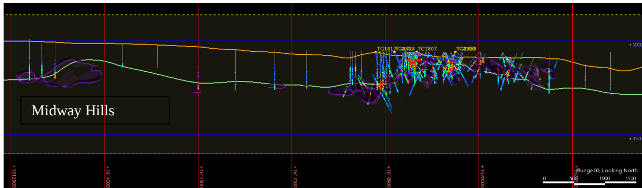
Figure 16-2: Cross section A-A', Looking North showing potential trend of mineralization between Midway Hills (Far left) and the Current resource area (right)
