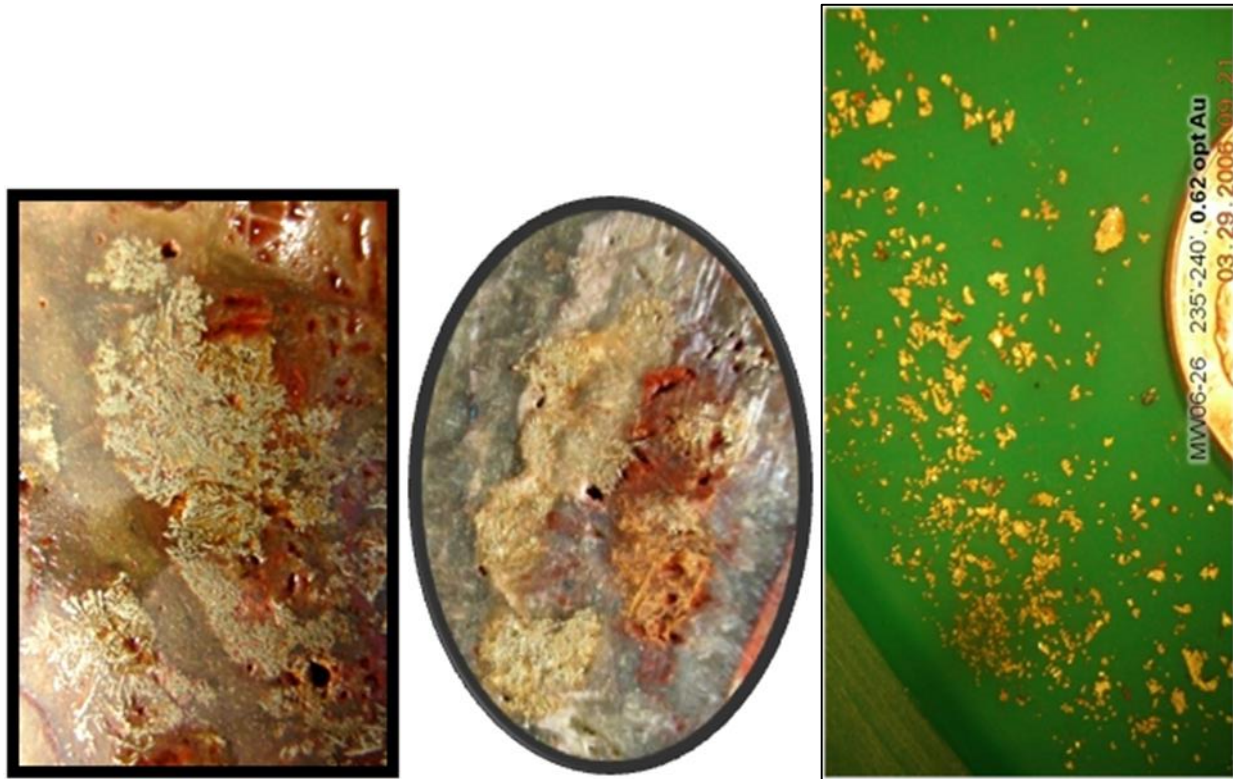
Figure 7-7: Visible Gold from Tonopah Project
