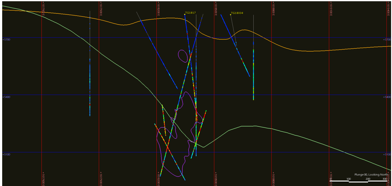
Figure 10-6: Cross Section showing 121 Zone Mineralization with 2018-2019 drill holes identified in gold text. (Section C-C' from Figure 10-3)
