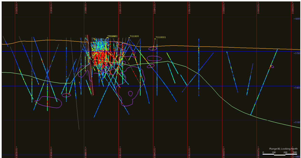
Figure 10-4: Cross Section through Discovery Zone Mineralization (Section A-A' from Figure 10-3)
