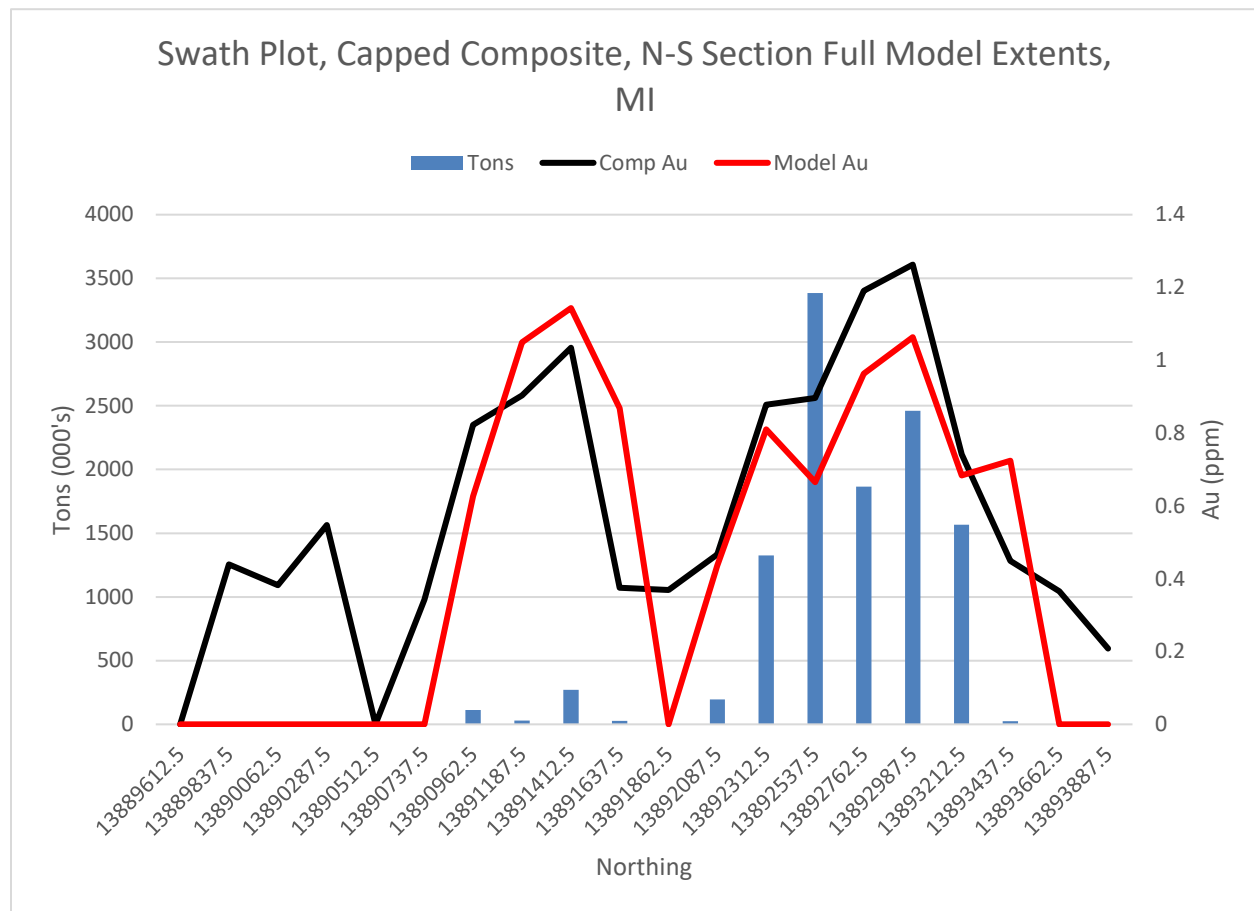
Figure 14-21: Swath Plot by Northing
