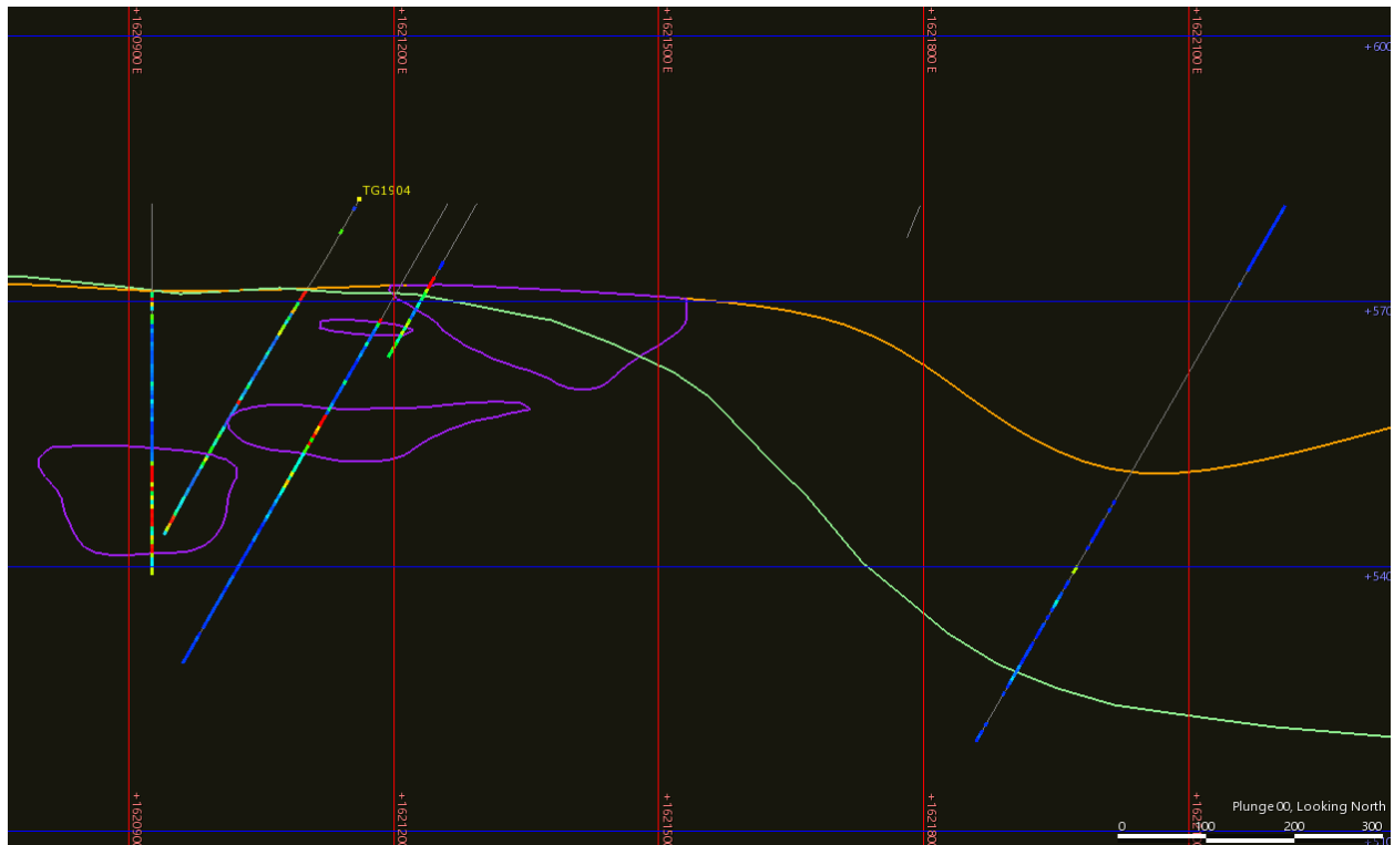
Figure 10-8: Cross Section showing Nautilus/Rye Patch Zone Mineralization with 2018-2019 drilling (Section E-E' from Figure 10-3)
