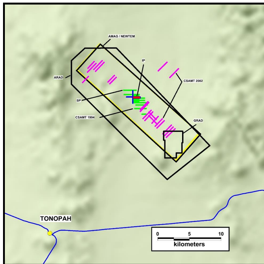
Figure 9-1: Historic Geophysical Survey Index Map (Wright, 2019)
