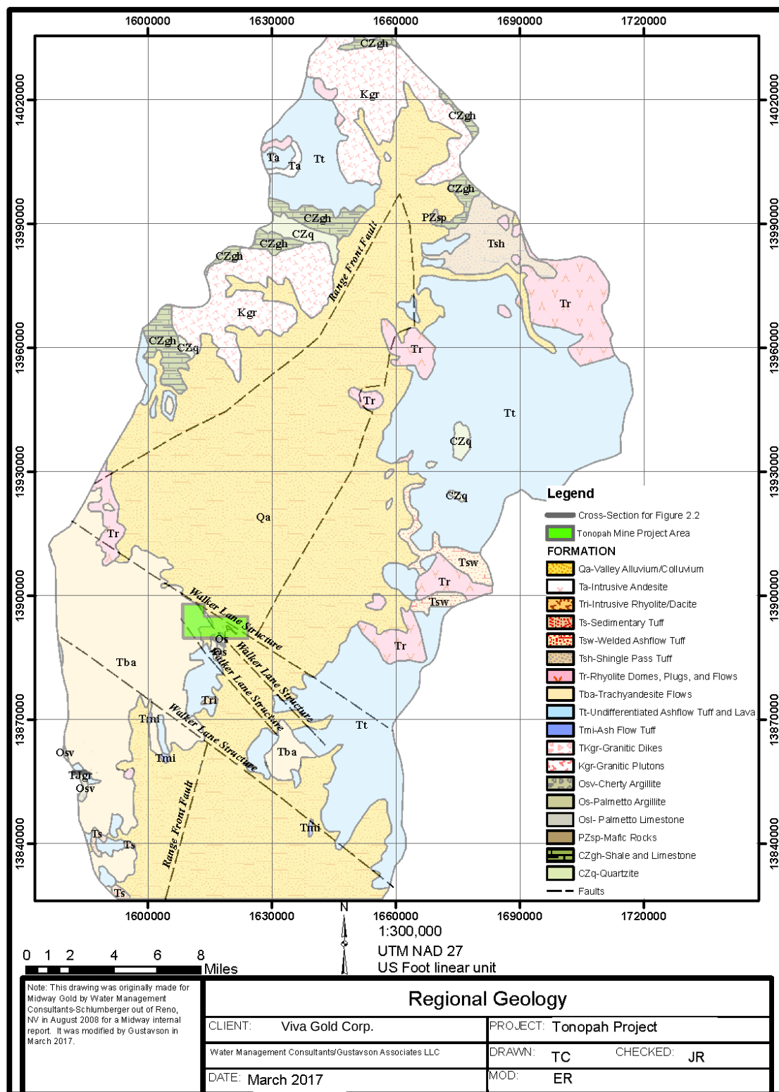
Figure 7-1: Regional Geology
