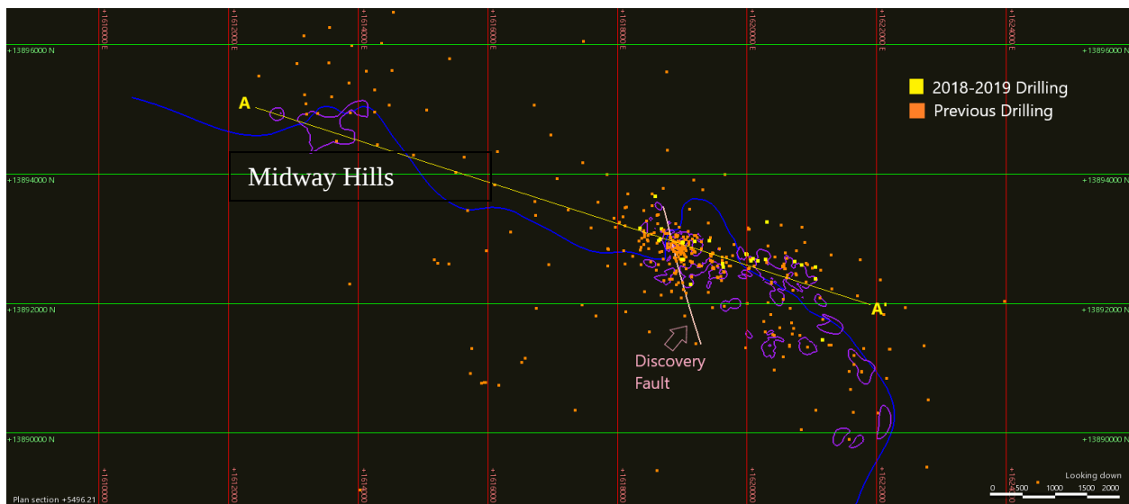
Figure 16-1: Plan view of drilling showing mineralized zones referenced with OPA layer (Section A-A' corresponds to Figure 16-2)
