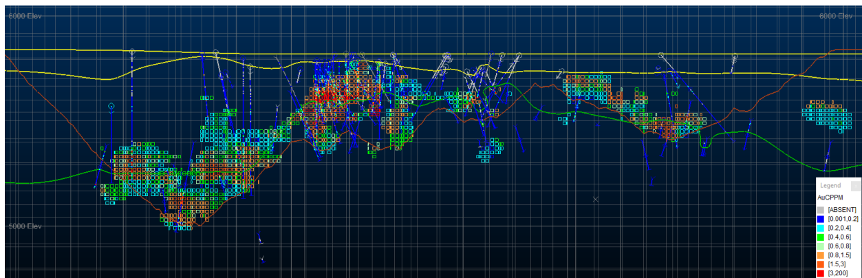
Figure 14-17 Long Section (Looking N20E) showing block grade estimates and pit trace for reference.
