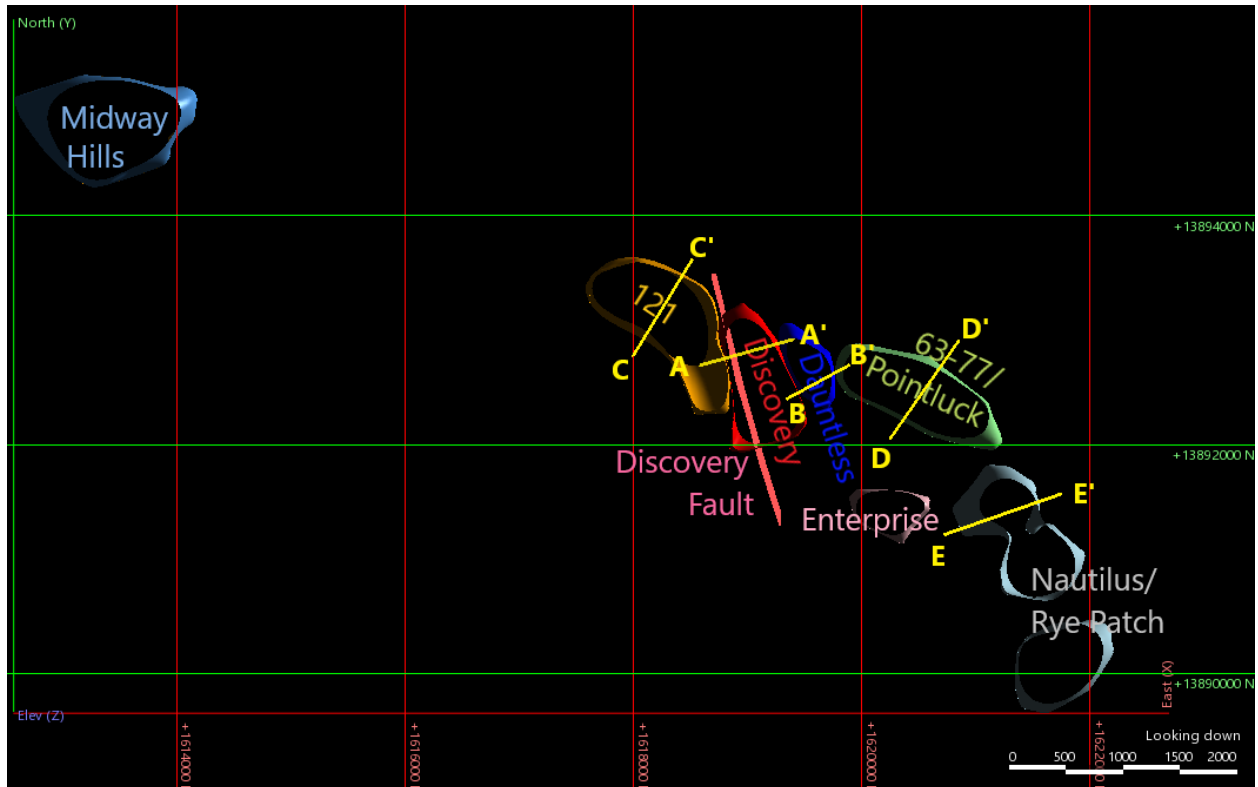
Figure 10-3: Mineralized Zones at the Tonopah project, and cross section traces for Section Lines. Section A-A' corresponds to Error! Reference source not found., Section B-B' corresponds to 10-5, Section C-C' corresponds to Figure 10-6, Section D-D' corresponds to Figure 10-7, and Section E-E' corresponds to Figure 10-8.
