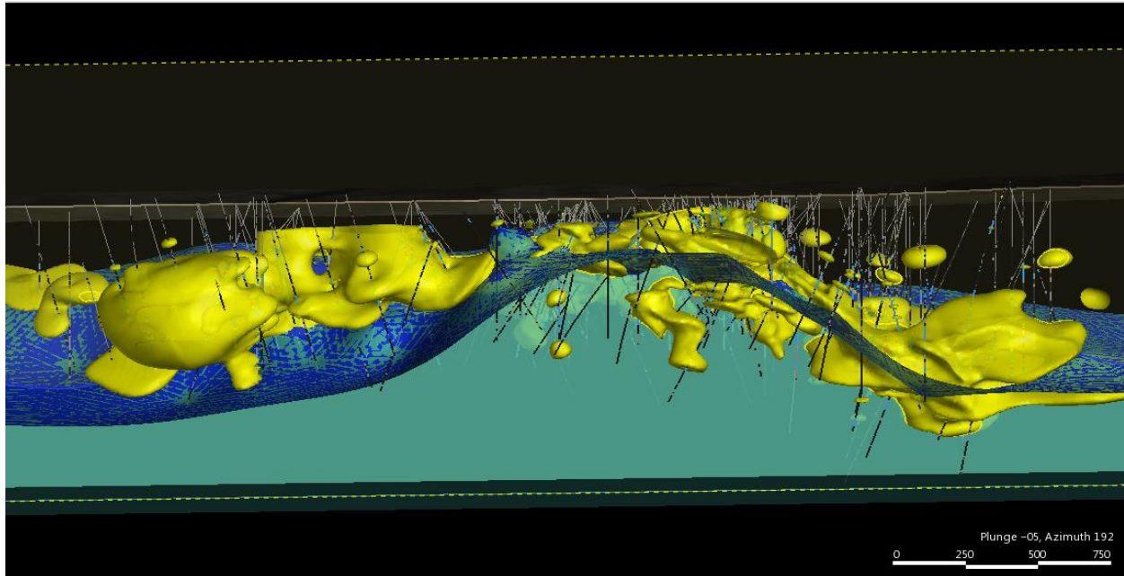
Figure 7-5: Long section looking South (Az 192), showing gold mineralization (gold shell) adjacent to Palmetto argillite contact (blue)
