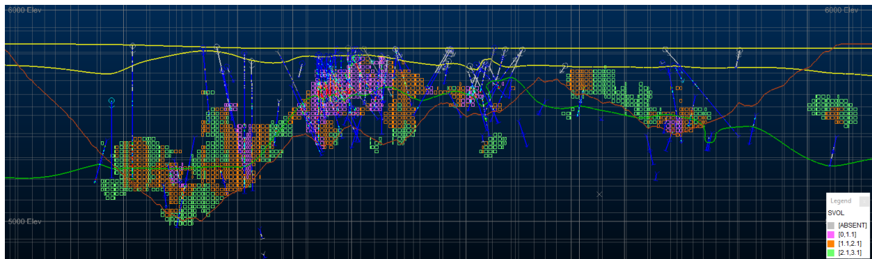
Figure 14-16: Long Section (Looking N20E) through Tonopah Block Model. Showing SVOL (classification) and pit trace for reference.
