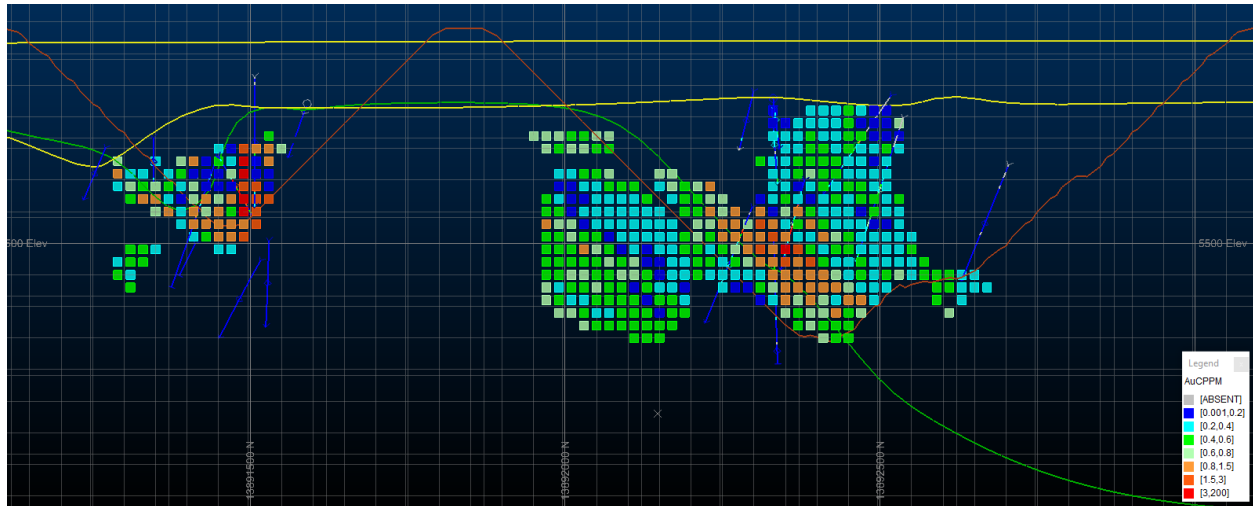
Figure 14-15: Example Cross Section (Looking W) through Enterprise (Left) and 121/Pointluck Zones (right) Showing MII blocks and Pit trace for reference.
