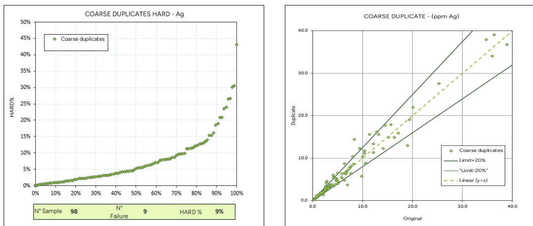
Figure 11-17: Ayawilca Ag Duplicates Plot for Coarse Duplicates – SGS
