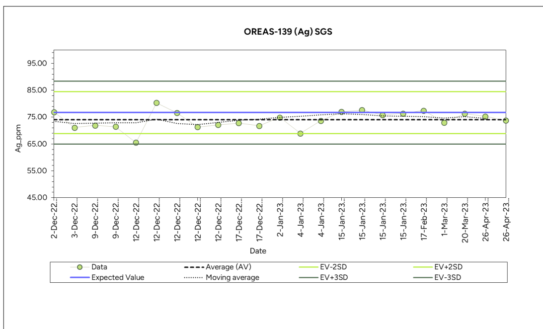
Figure 11-10: Ayawilca Ag Control Chart for OREAS139 – SGS
