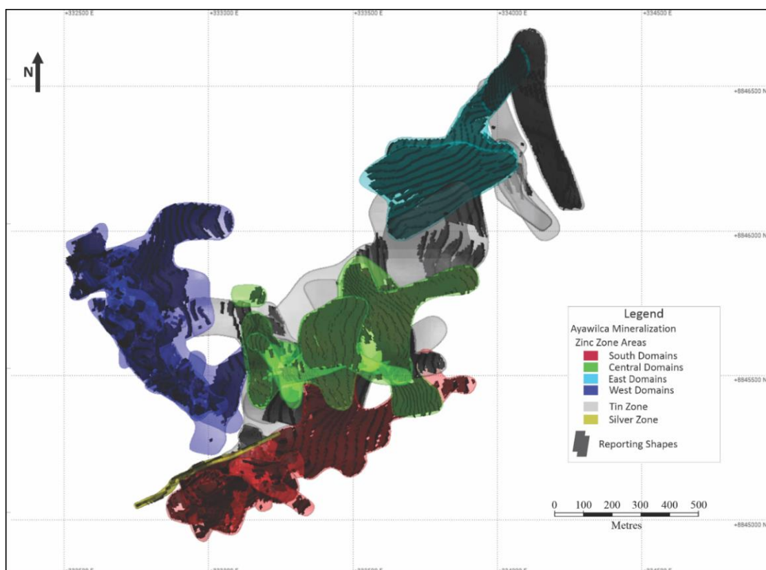
Figure 14-13: Ayawilca Domains and Underground Reporting Shapes in Plan View
