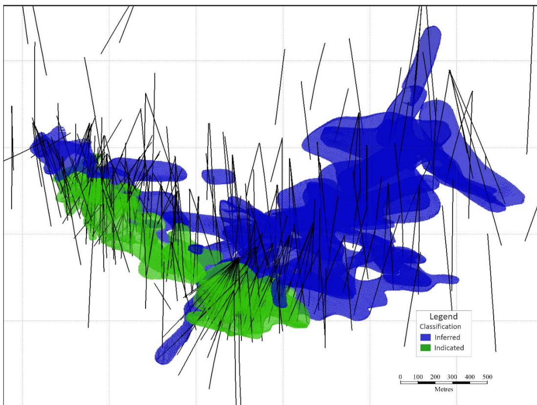
Figure 14-10: Ayawilca Deposit Classification Model and Drilling
