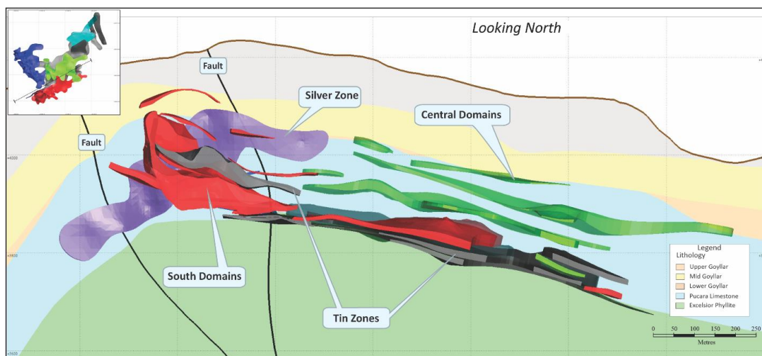
Figure 14-3: Southwest-Northeast Cross Section of the Ayawilca Resource Domains
