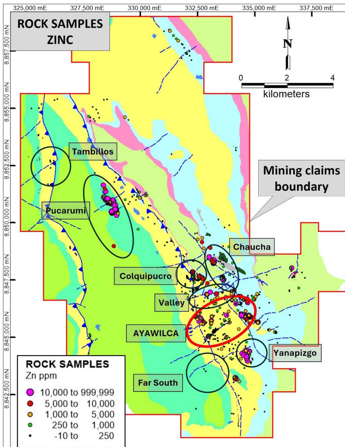
Figure 9-1: Surface Rock Samples Results
