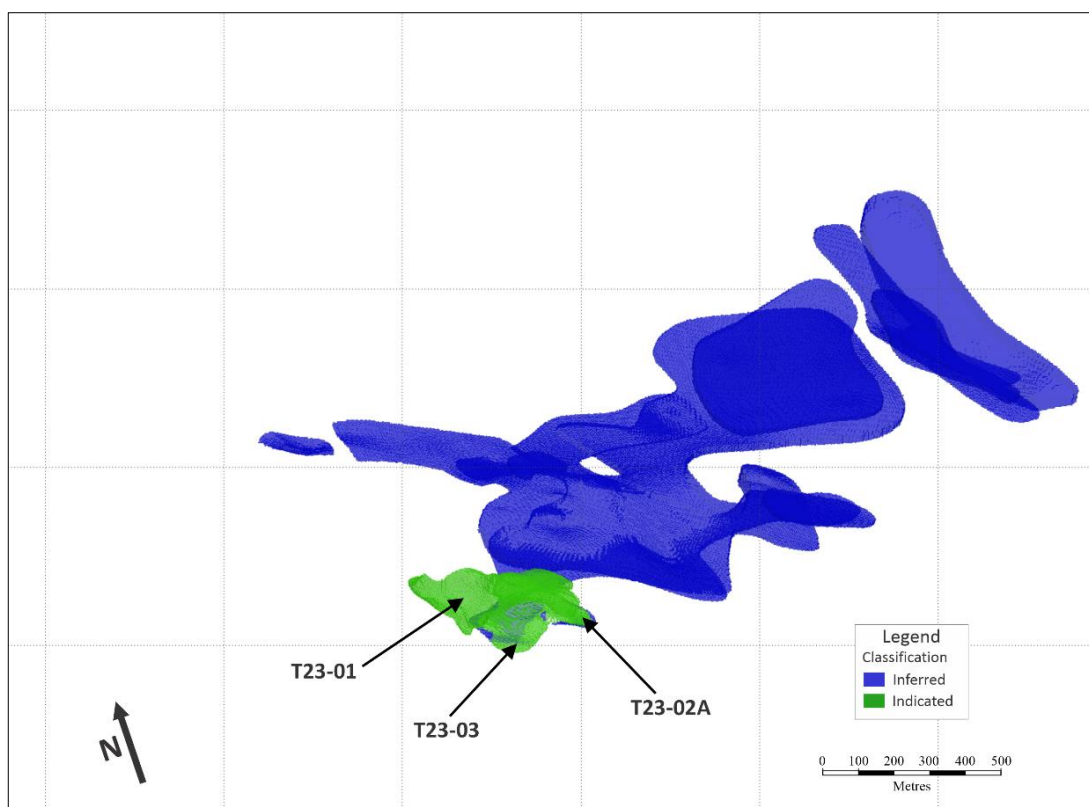
Figure 14-12: Tin Zone Classification Model
