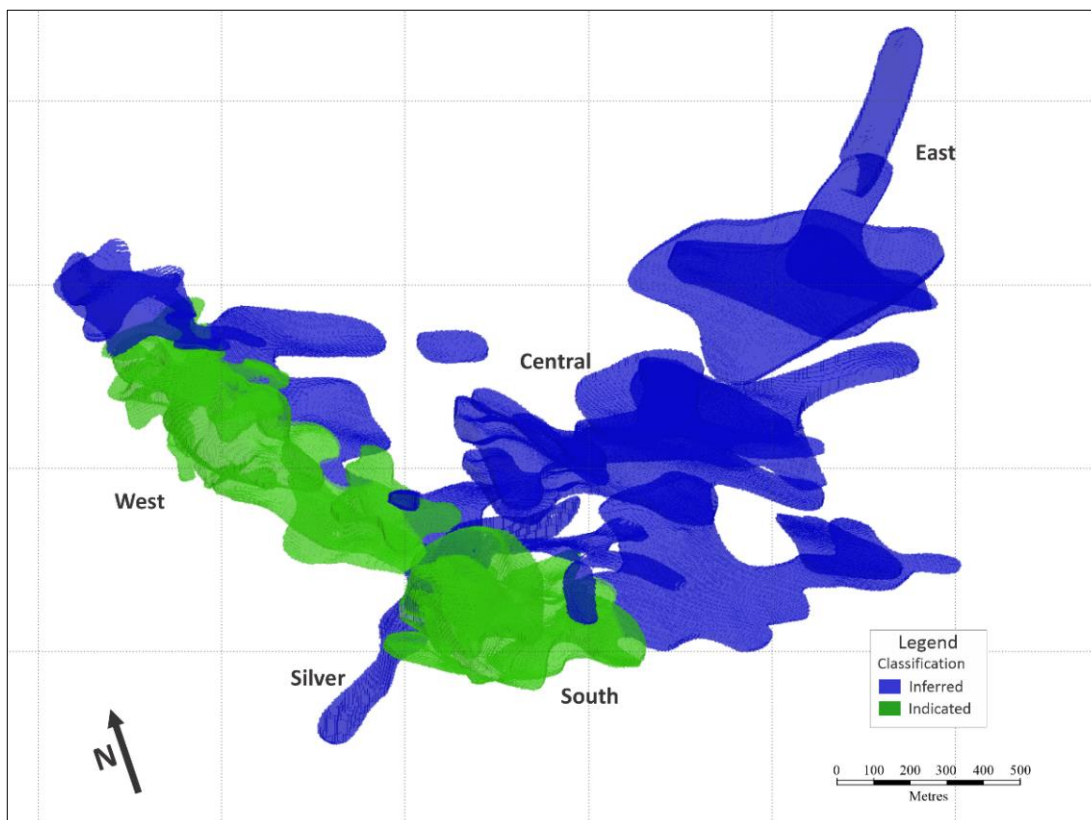
Figure 14-10: Ayawilca Deposit Classification Model and Drilling
