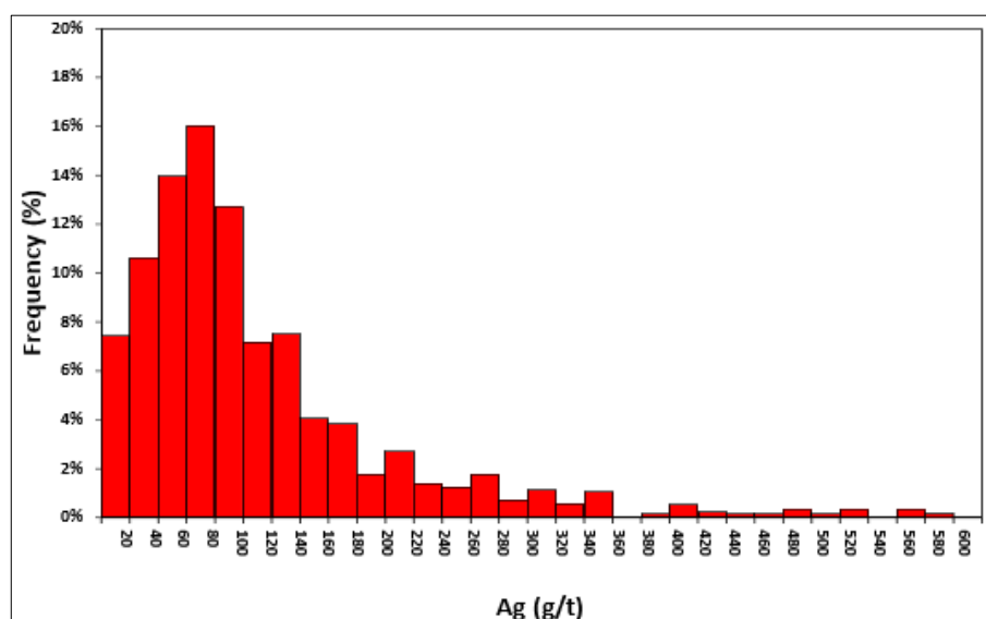
Figure 14-22: Histogram Assays within Colquipucro High-Grade Lenses
