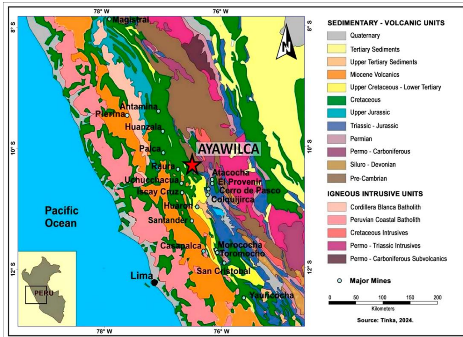
Figure 7-2: Regional Geology
