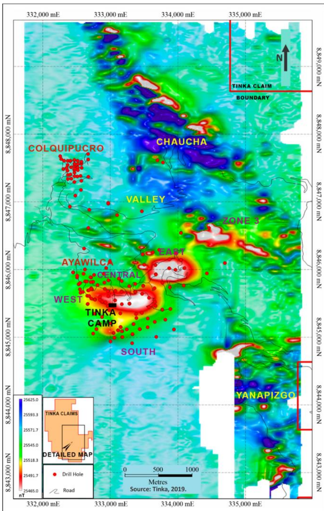
Figure 9-3: RTE Magnetics Map
