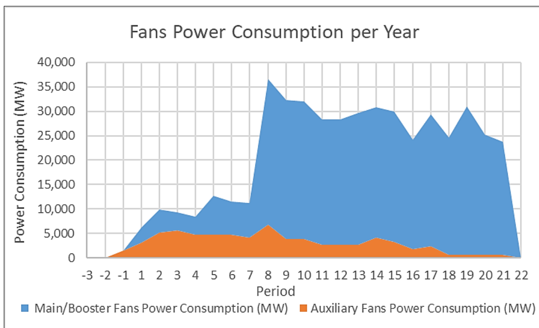
Figure 16-27: Graph Fans Power Consumption Per year
