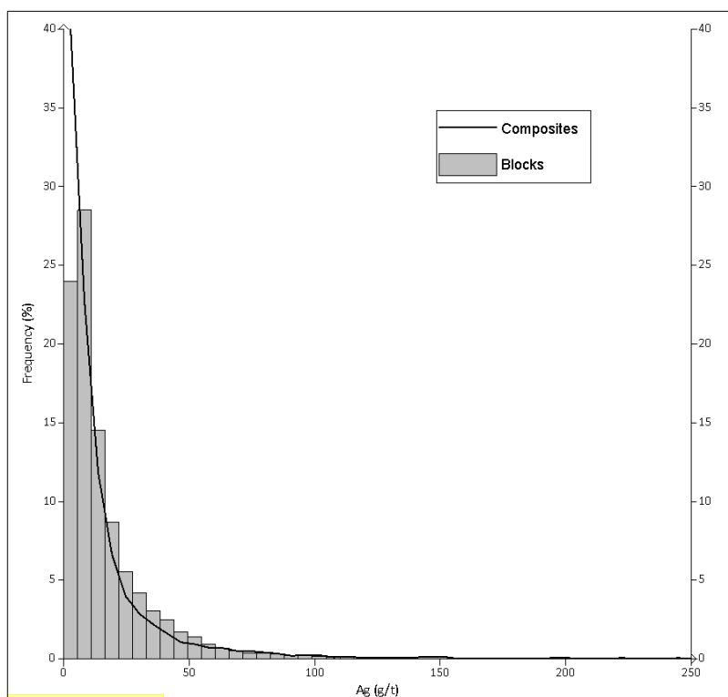
Figure 14-18: Histograms of the Estimated Block Silver Grades – Ayawilca Zinc Zone and Silver Zone
