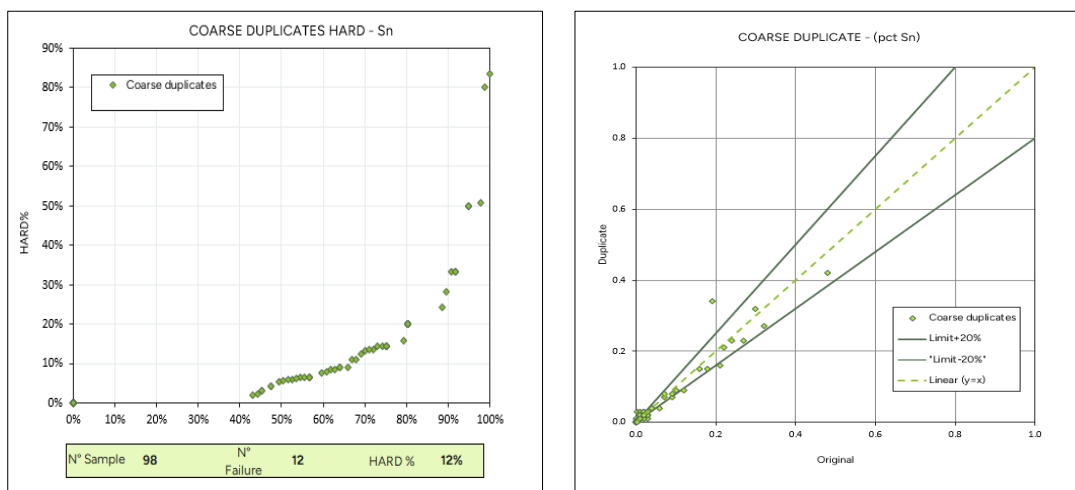
Figure 11-18: Ayawilca Pb Duplicates Plot for Pulp Duplicates – SGS
