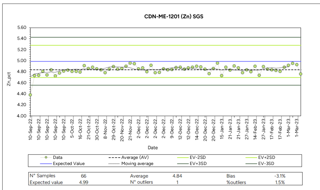
Figure 11-6: Ayawilca Zn Control Chart for CDN-ME-1201 - SGS
