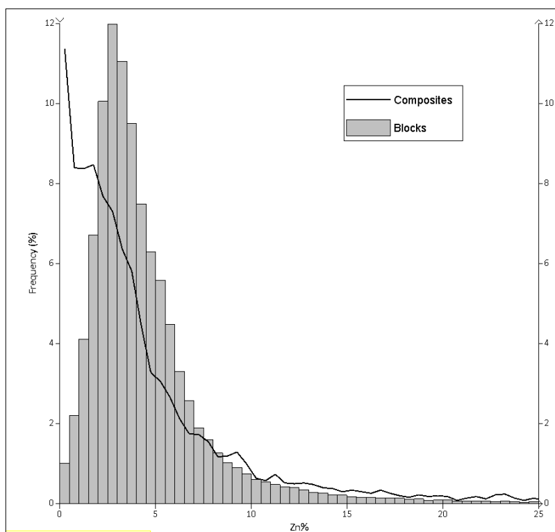
Figure 14-17: Histograms of the Estimated Block Zinc Grades – Ayawilca Zinc Zone and Silver Zone
