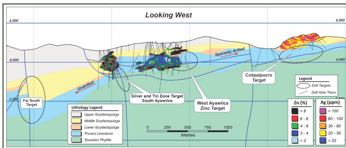
Figure 9-5: Longitudinal Section of Ayawilca Zinc Zone Parallel to the Colquipucro Fault showing Exploration Targets
