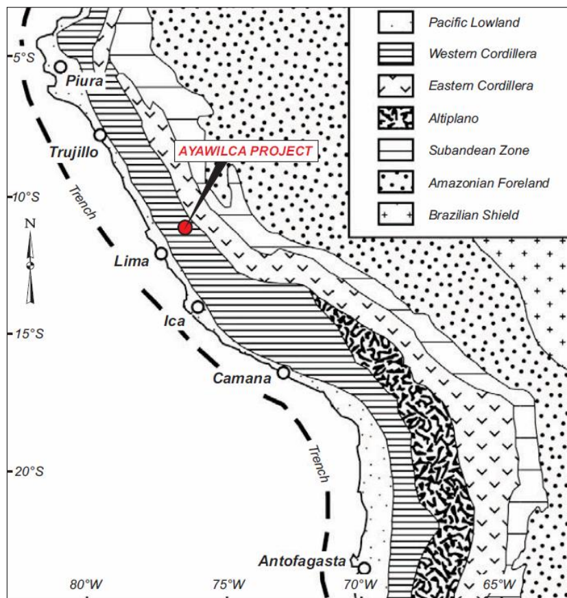
Figure 7-1: Morphostructural Map
