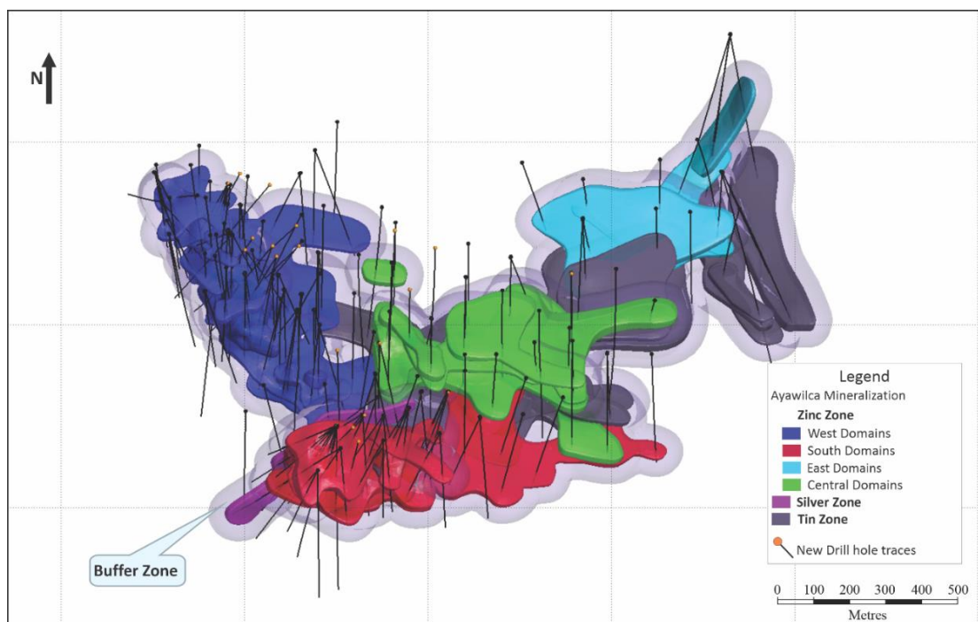
Figure 14-1: Plan View of Ayawilca Resource Domains
