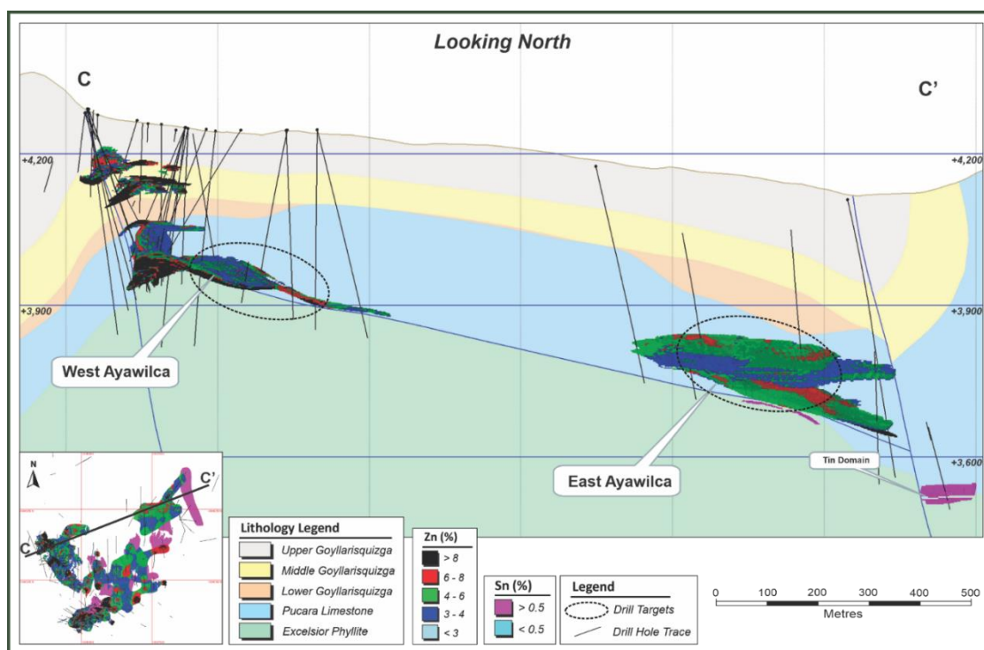
Figure 9-5: Longitudinal Section of Ayawilca Zinc Zone Parallel to the Colquipucro Fault showing Exploration Targets
