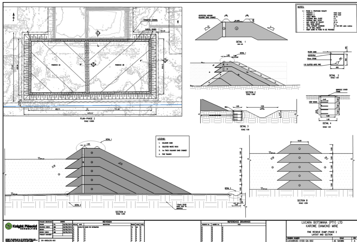
Figure 18-8: Fine Residue Dump - Phase 2 Layout and Section
