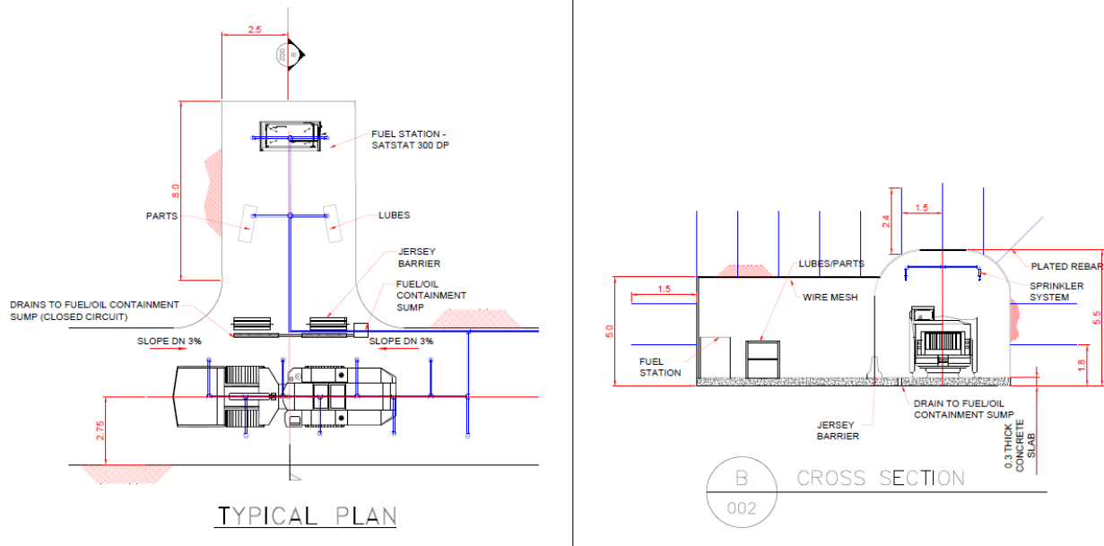
Figure 16-24: Fuel Bay General Arrangement
