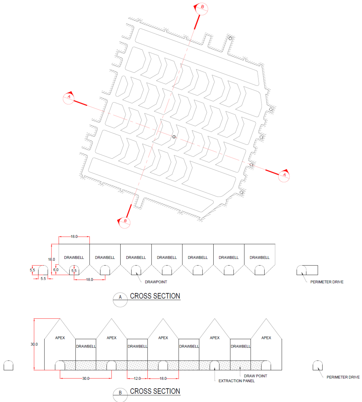
Figure 16-13: Drawbell Geometry
