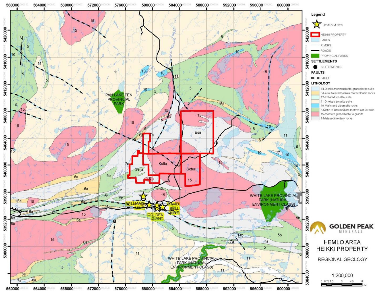
Figure 5: Regional Geology of the Hemlo Area.
