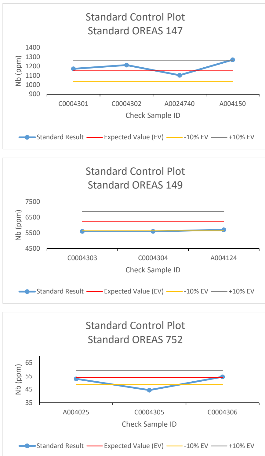
Figure 11-1 Field Standard Control Plots
