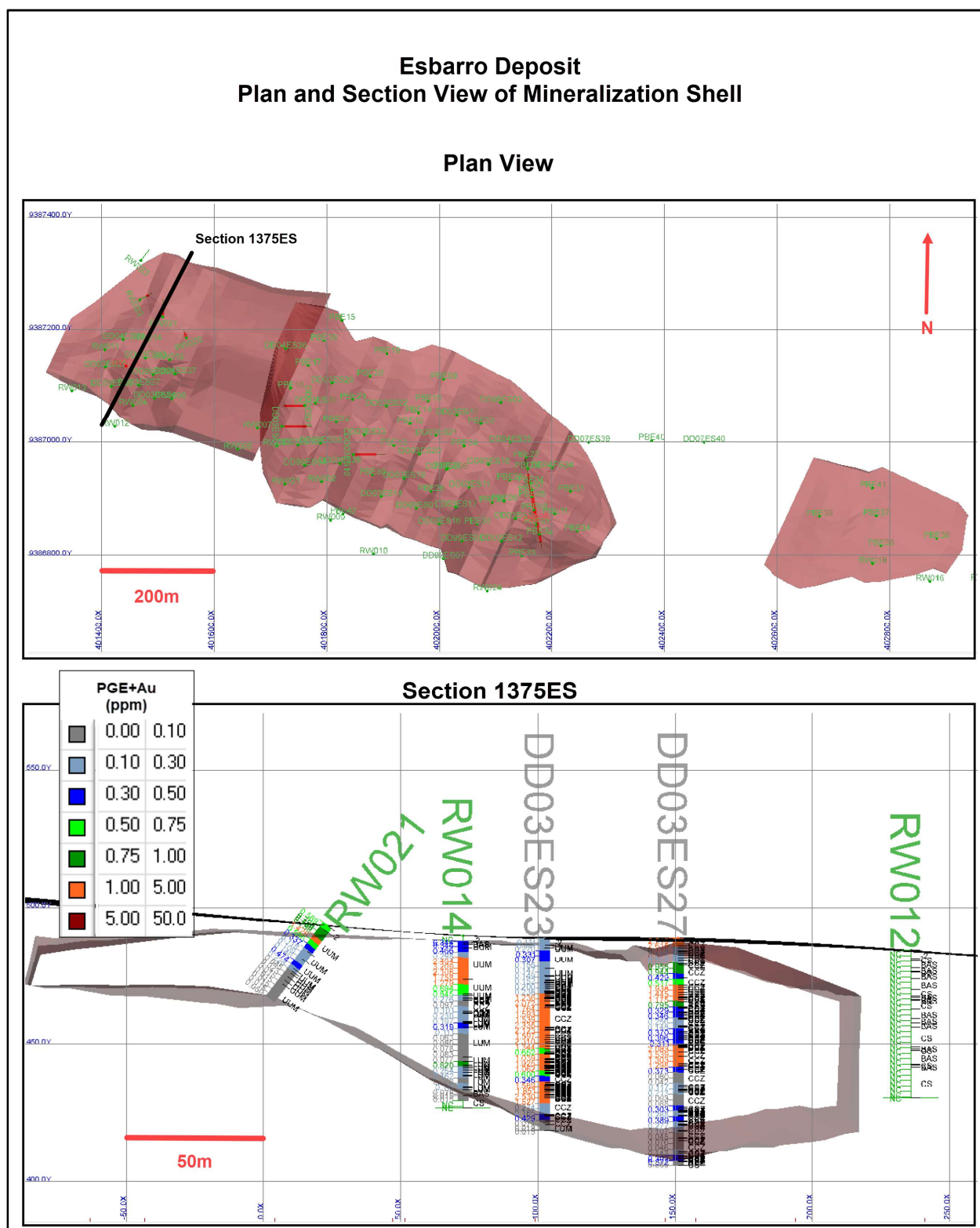
Figure 14-4 Esbarro Deposit, Plan and Section view of Mineralization Shell
