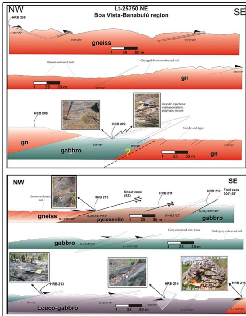
Figure 7-8 Cross Sections from Banabuiu Target Area (GE21, 2018)
