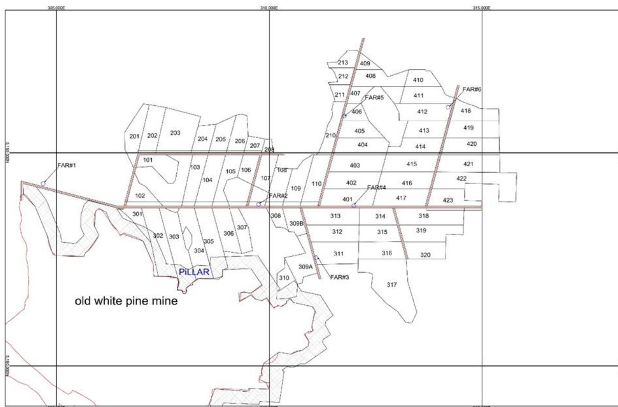
Figure 16.1: Mine Configuration
