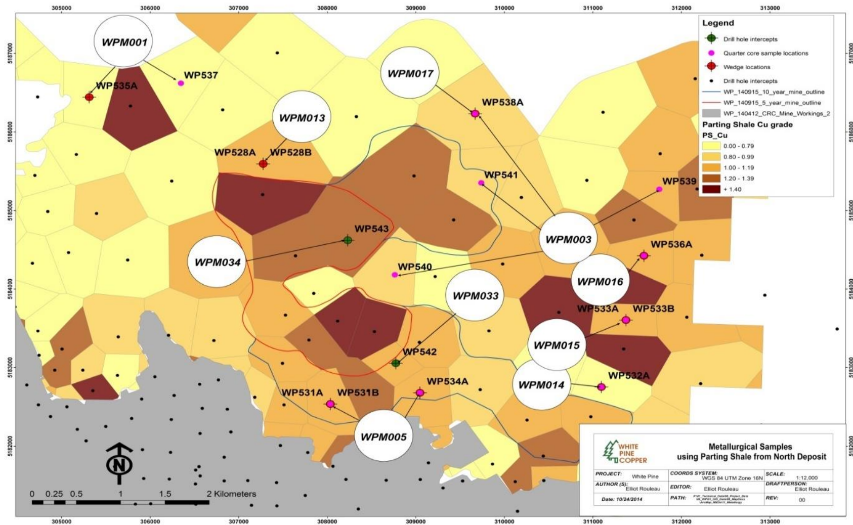
Figure 13.3: Met Samples Used for PS Mineralization Testing
