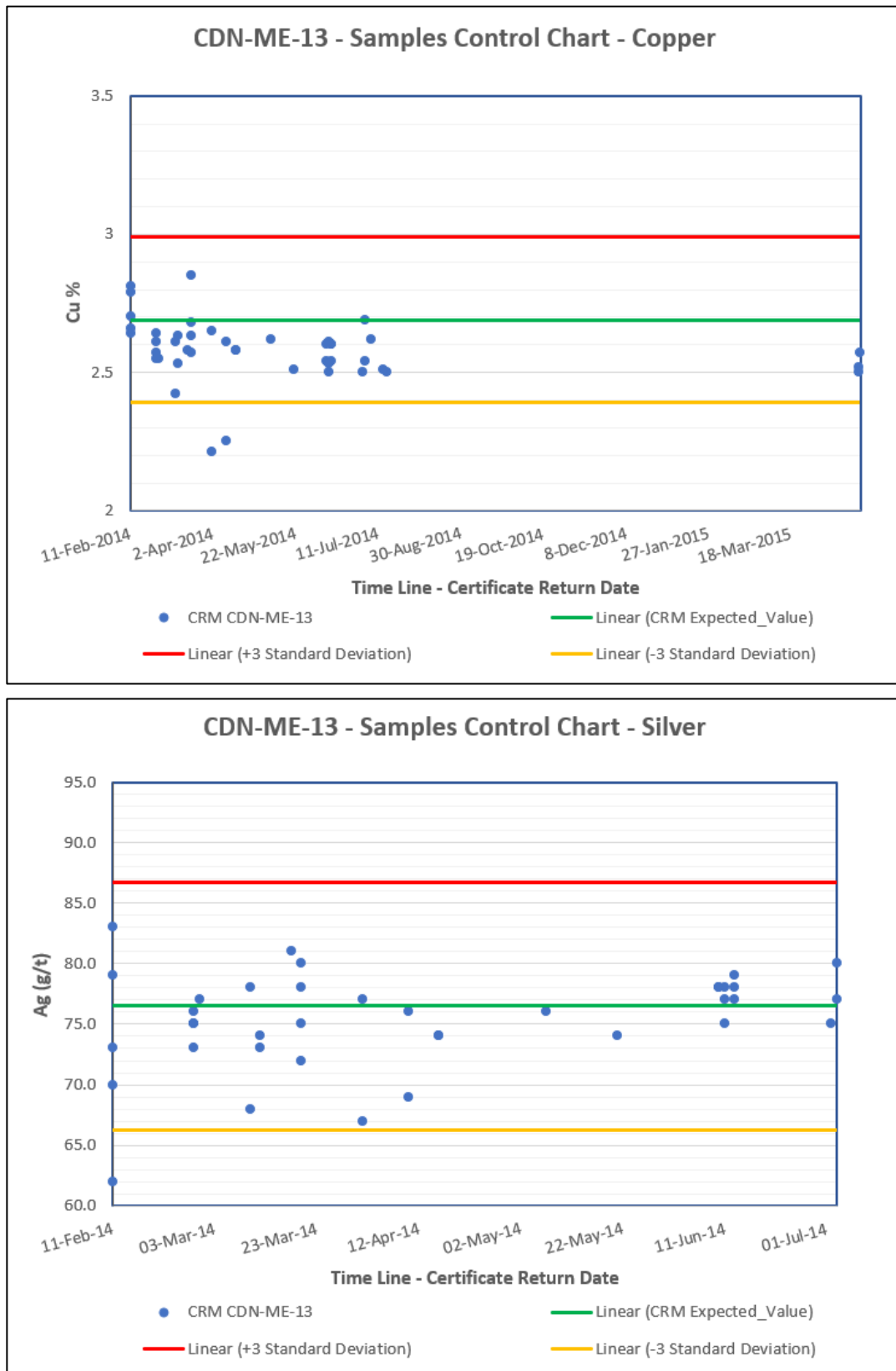
Figure 11.10: Performance of Control Reference Material CDN-ME-13 for Cu (top) and Ag (bottom)
