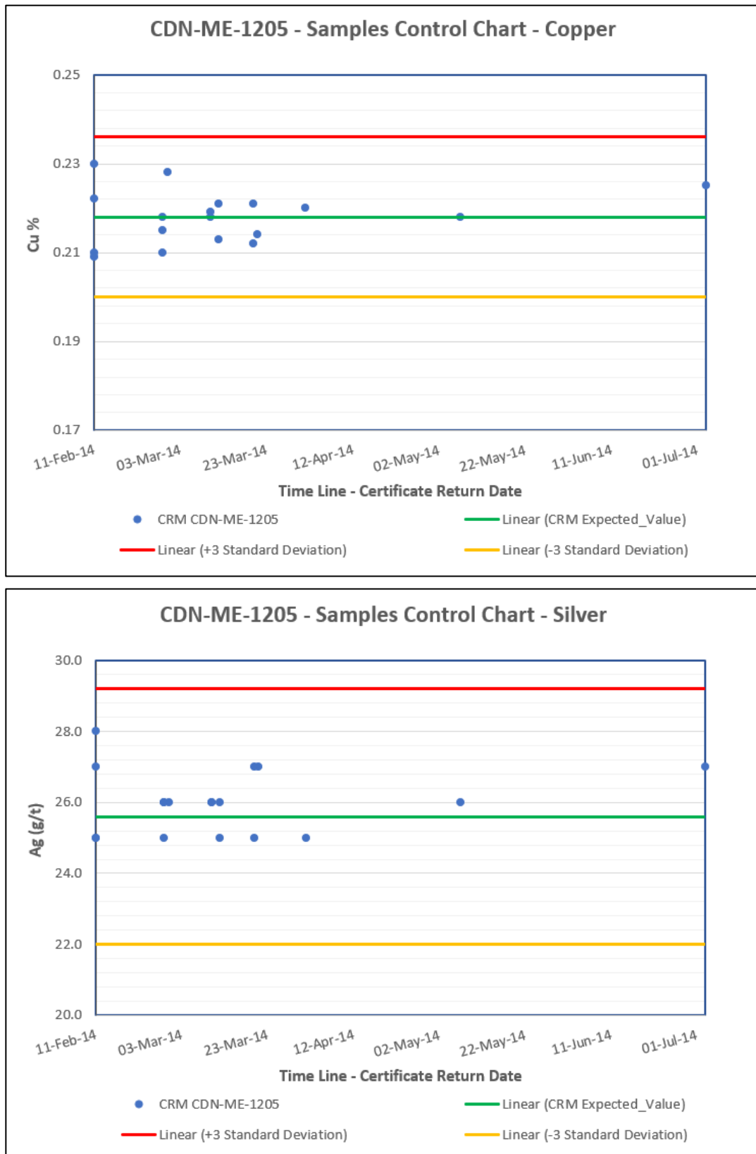
Figure 11.9: Performance of Control Reference Material CDN-ME-1205 for Cu (top) and Ag (bottom)
