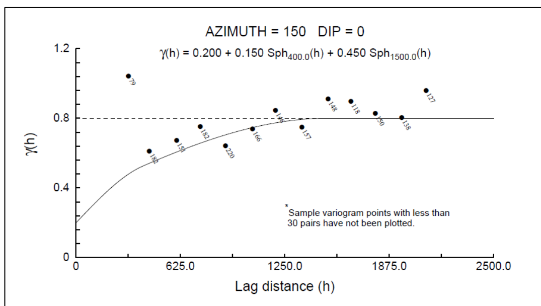
Figure 14.11: Variogram Model Cu% for the Parting Shale (PS) Column
