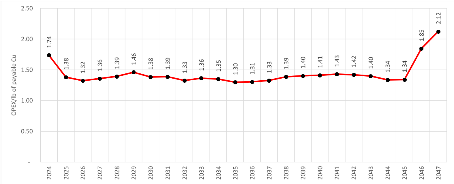
Figure 21.3: Operating Cost per lb of Payable Copper
