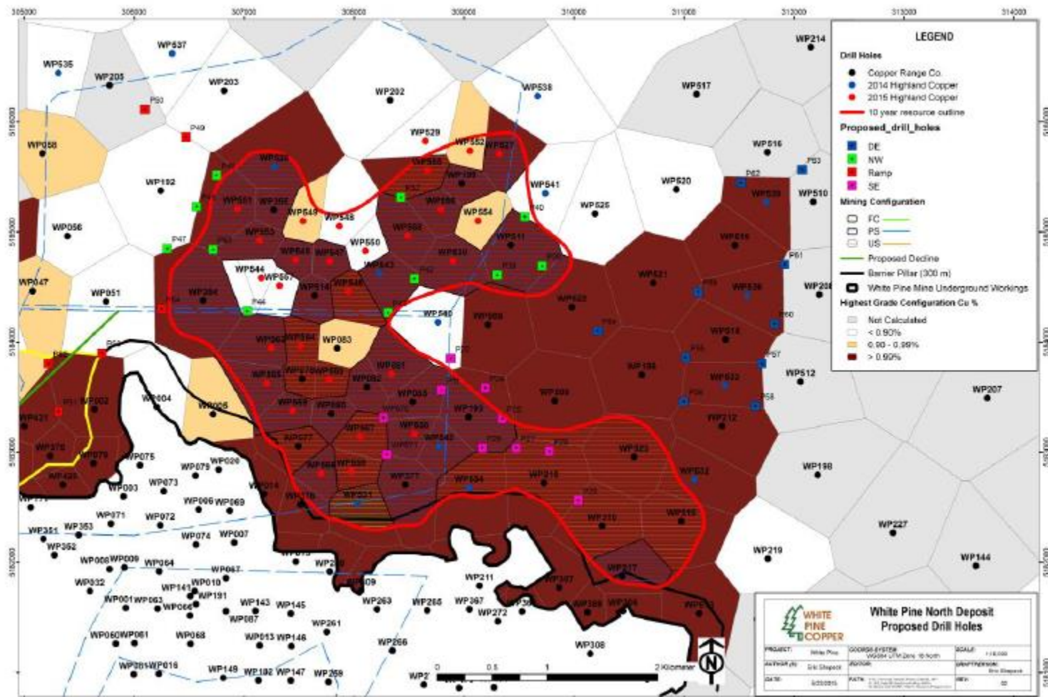
Figure 13.6: White Pine North Deposit Proposed Drill Holes
