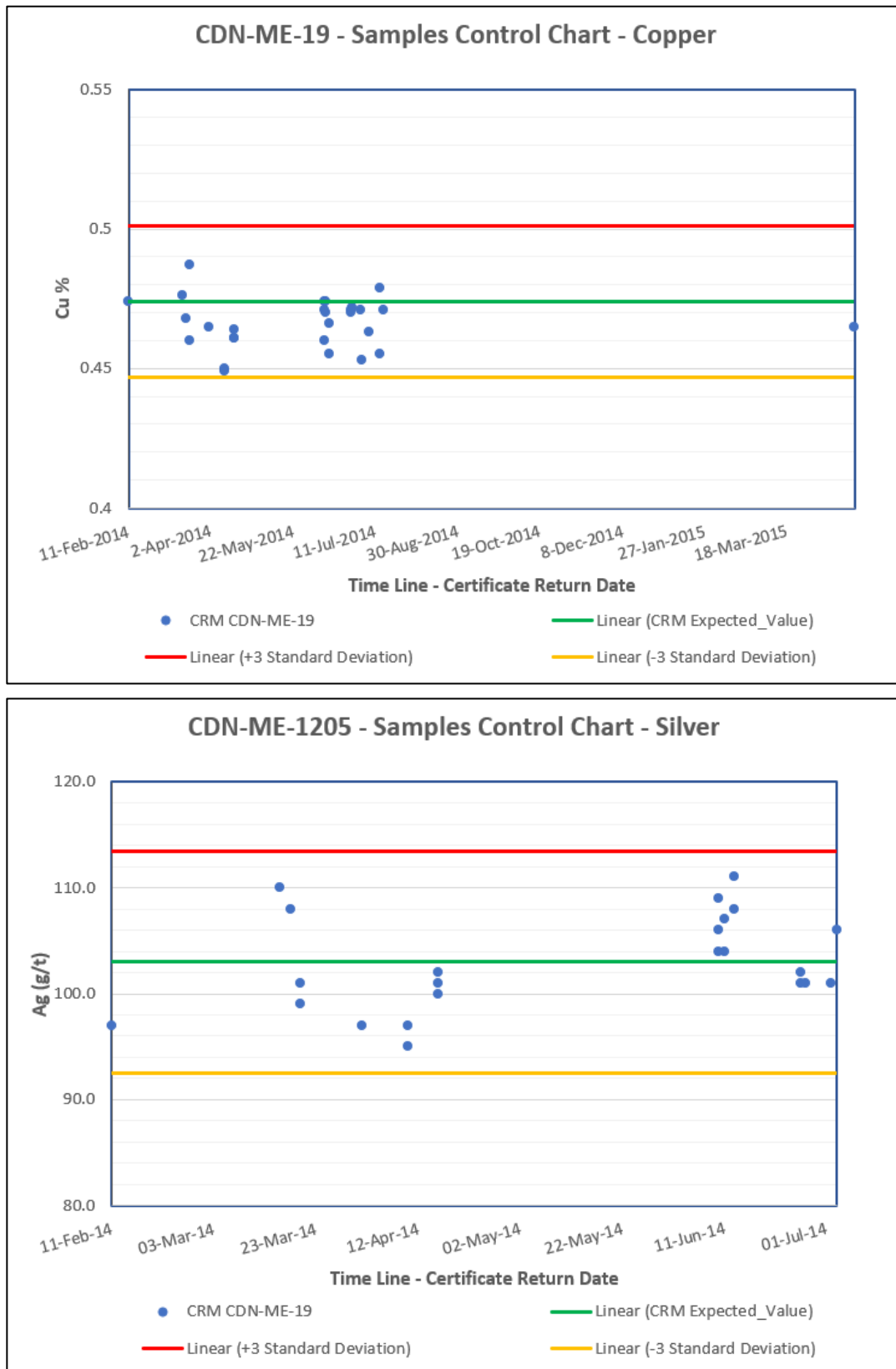
Figure 11.11: Performance of Control Reference Material CDN-ME-19 for Cu (top) and Ag (bottom)
