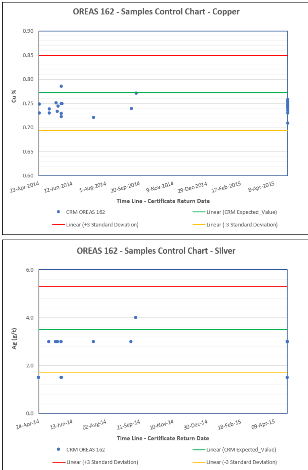
Figure 11.6: Performance of Control Reference Material OREAS 162 for Cu (top) and Ag (bottom)
