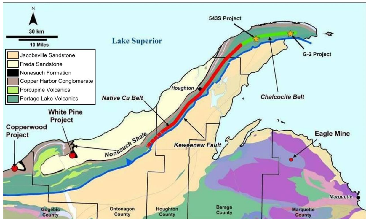
Figure 7.1: Regional Geology – Upper Peninsula of Michigan
