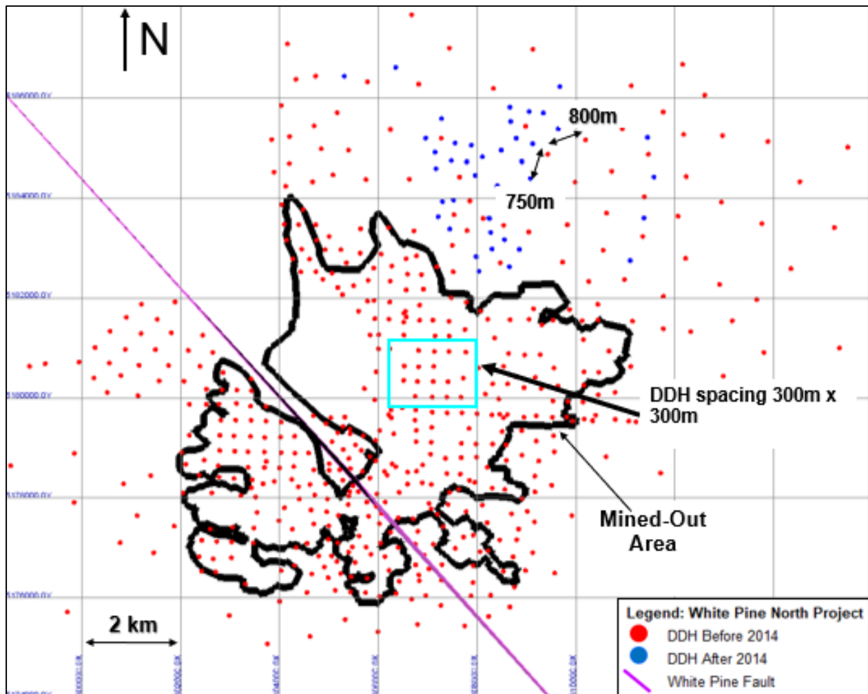
Figure 14.1: Plan View of Drill Hole Collars – White Pine North Project
