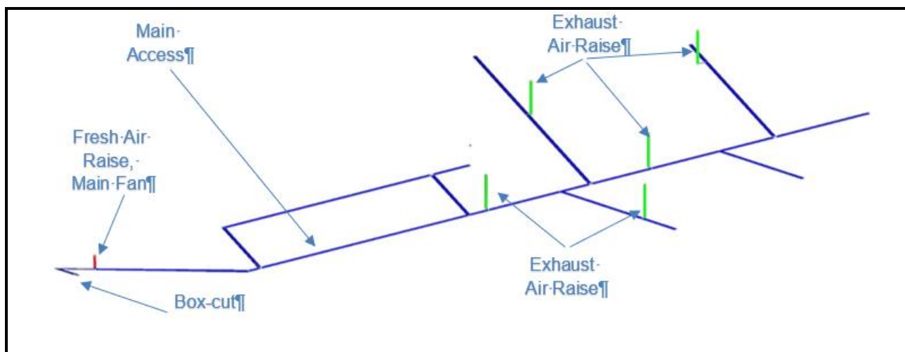
Figure 16.13: Ventilation Layout during Production Period
