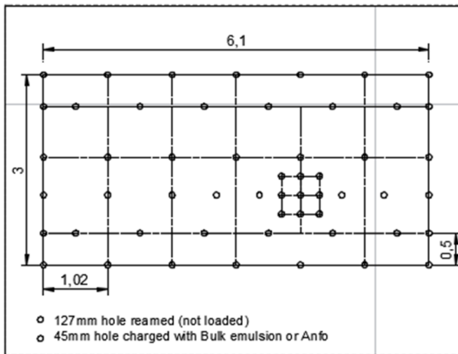
Figure 16.7: Drilling Pattern for the Development Drift
