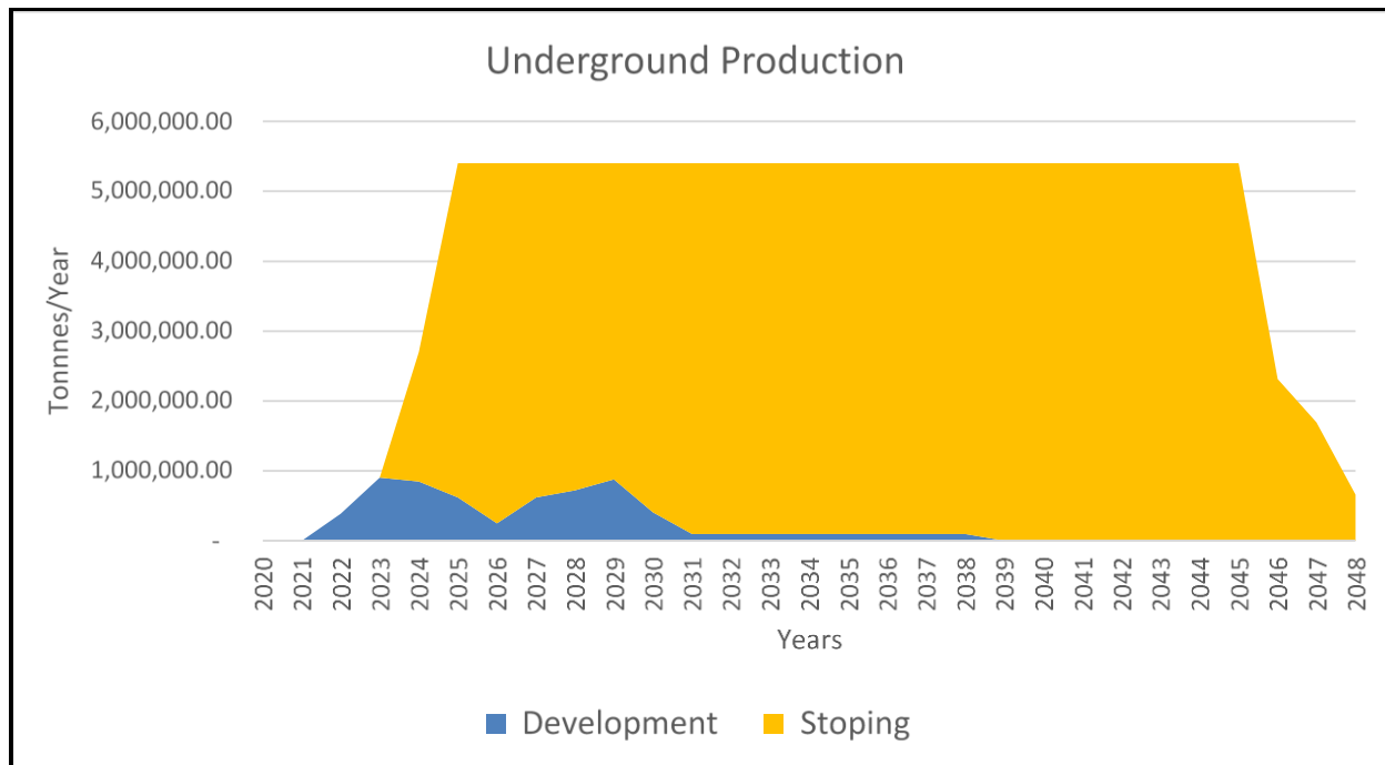
Figure 16.12: Production Schedule
