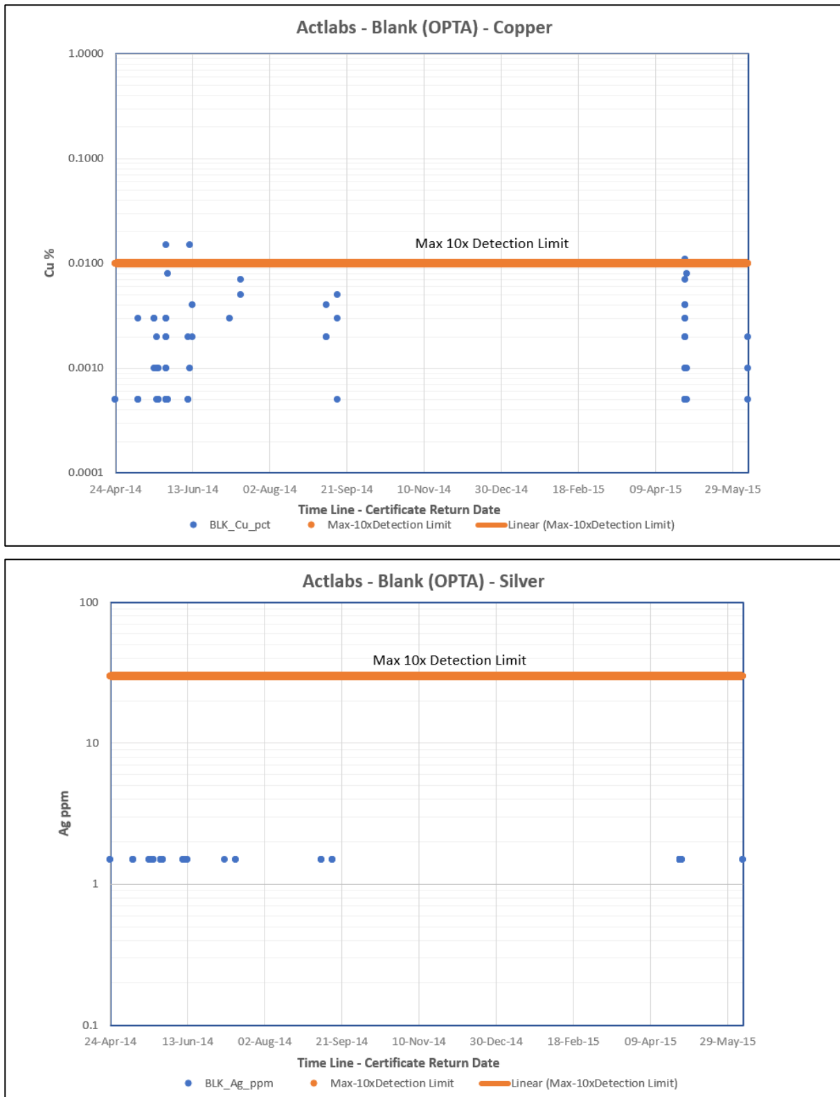
Figure 11.1: Blank Material (OPTA) Time Plots with Analytical Results for Copper (top) and Silver (bottom)
