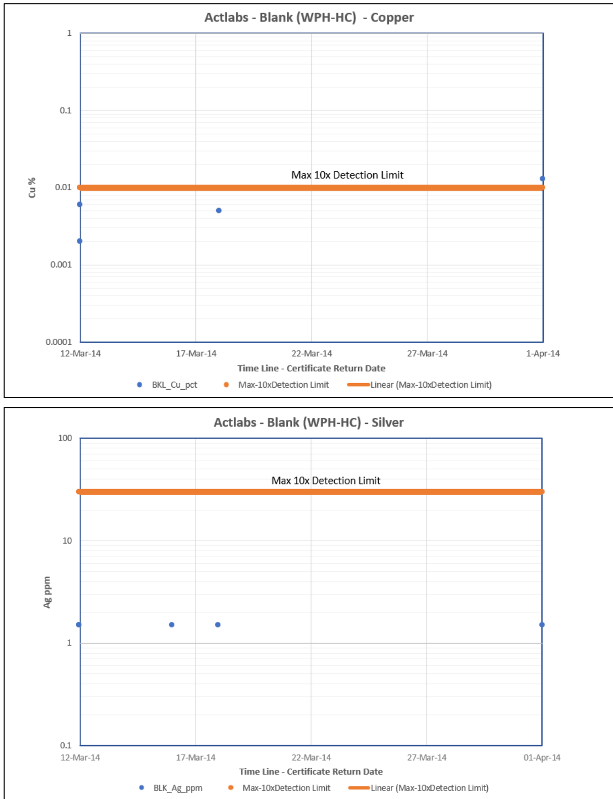
Figure 11.3: Blank Material (WPH-HC) Time Plots with Analytical Results for Copper (top) and Silver (bottom)
