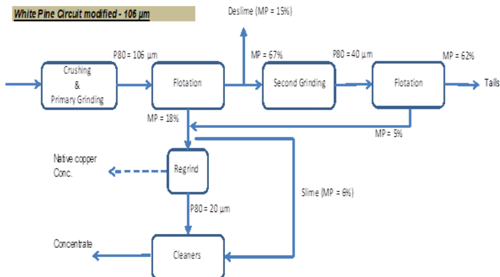
Figure 13.4: White Pine Circuit – 106 \mu\text{m}
