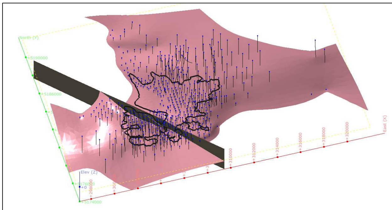
Figure 14.4: Parting Shale and White Pine Fault – Leapfrog 3D Model
