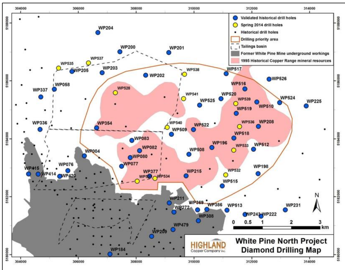
Figure 9.1: Location Map of Holes Completed During 2014 Drilling Program and Historical Diamond Drill Holes Used in Highland's Validation Sampling Program
