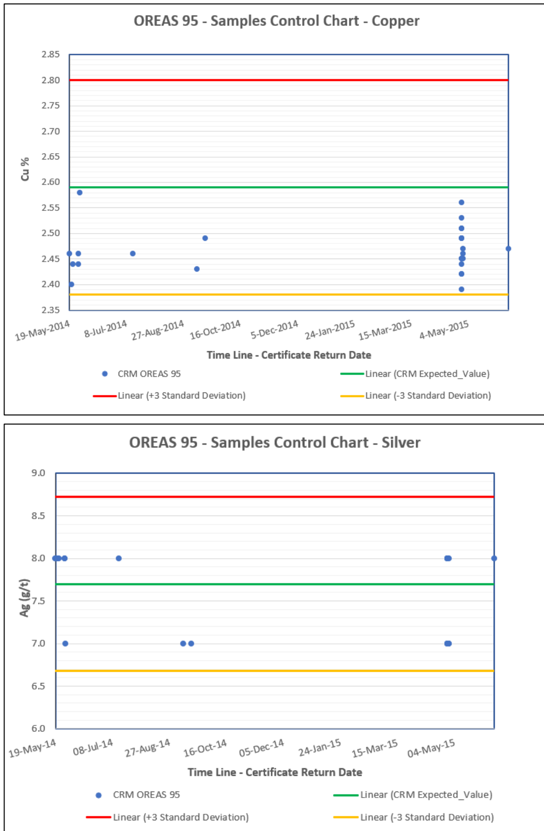
Figure 11.7: Performance of Control Reference Material OREAS 95 for Cu (top) and Ag (bottom)
