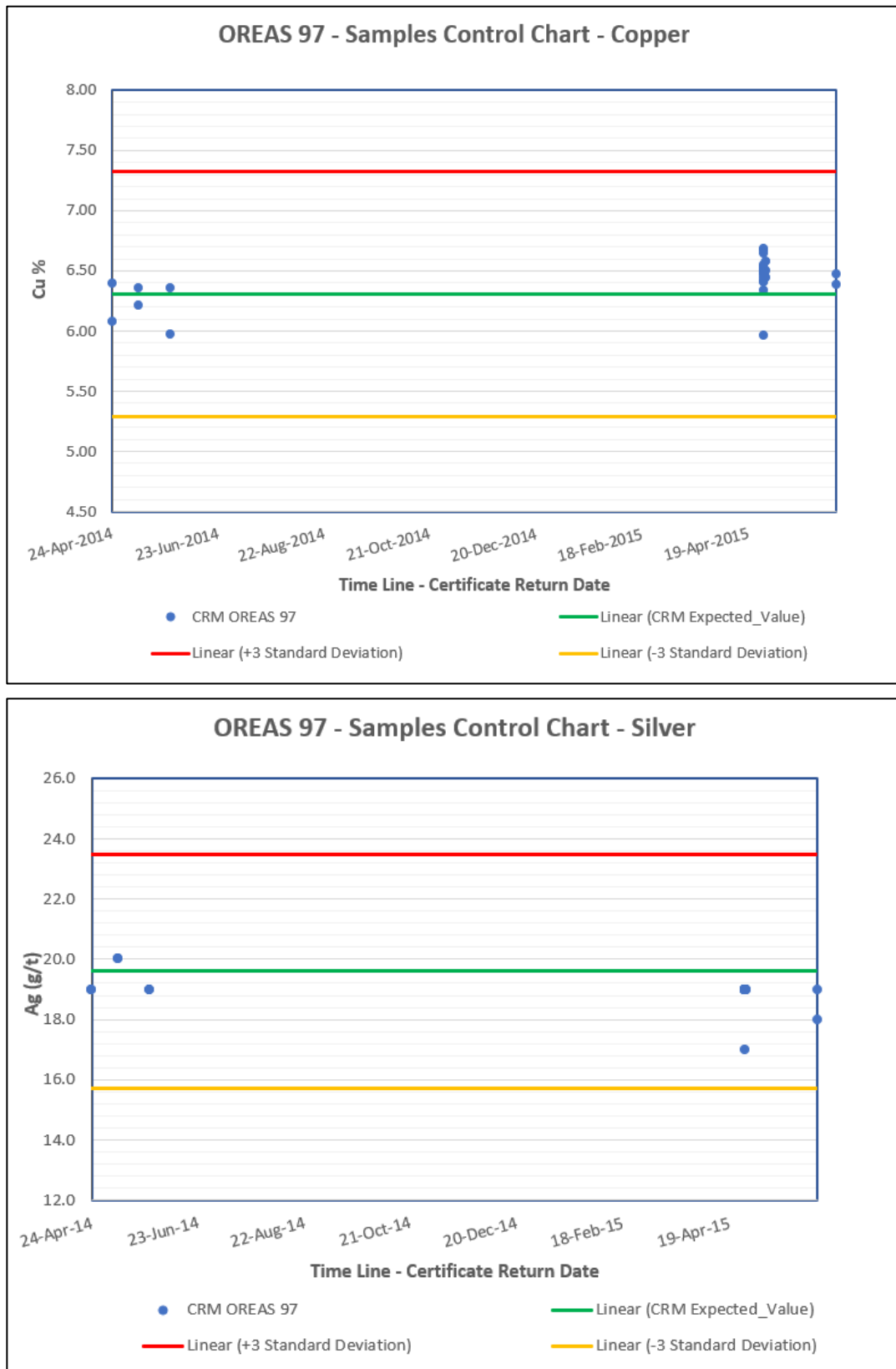
Figure 11.8: Performance of Control Reference Material OREAS 97 for Cu (top) and Ag (bottom)
