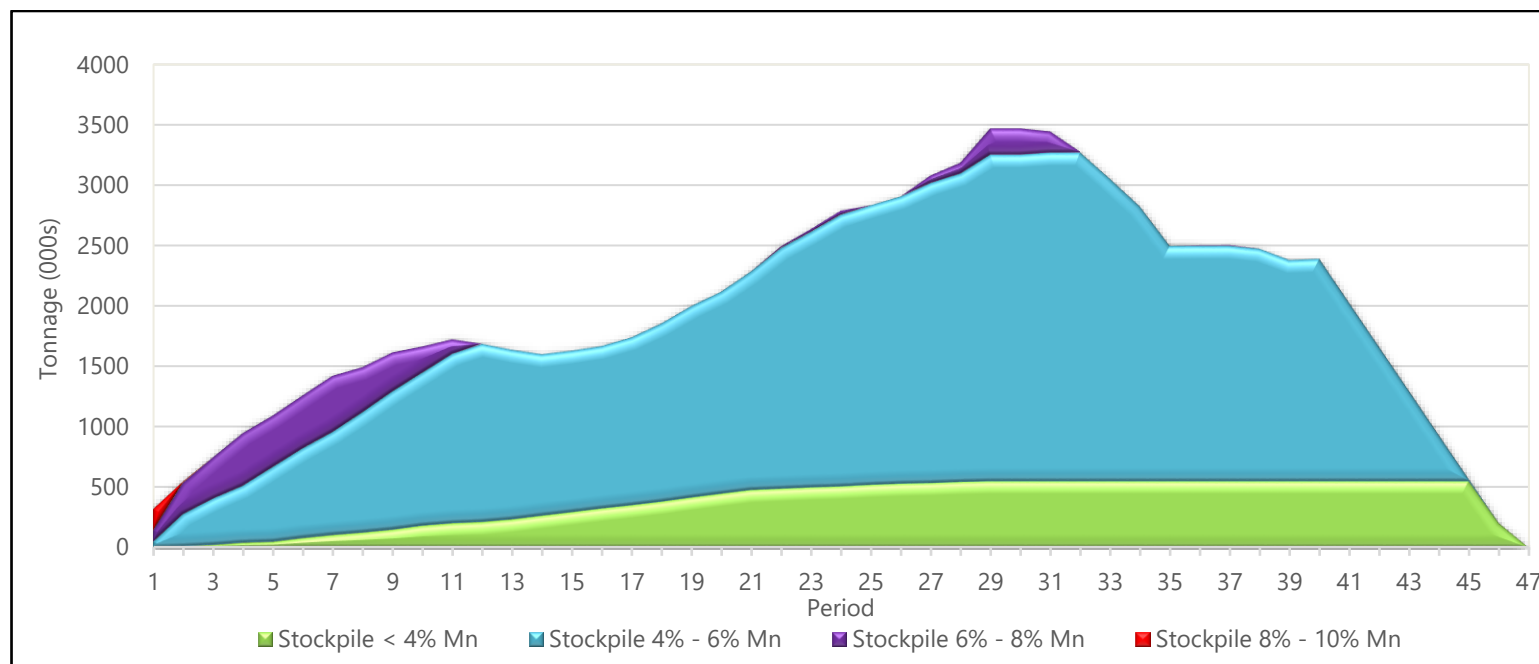
Figure 16-7: Conceptual Stockpile Grade Summary
