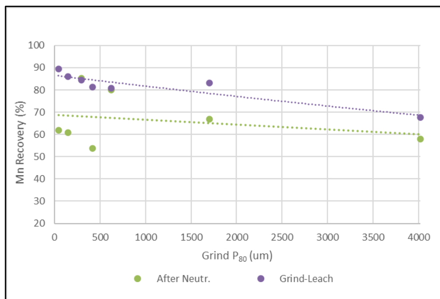
Figure 13-4: Effect of Grind Size on Manganese Extraction, in Leach and after Neutralization
