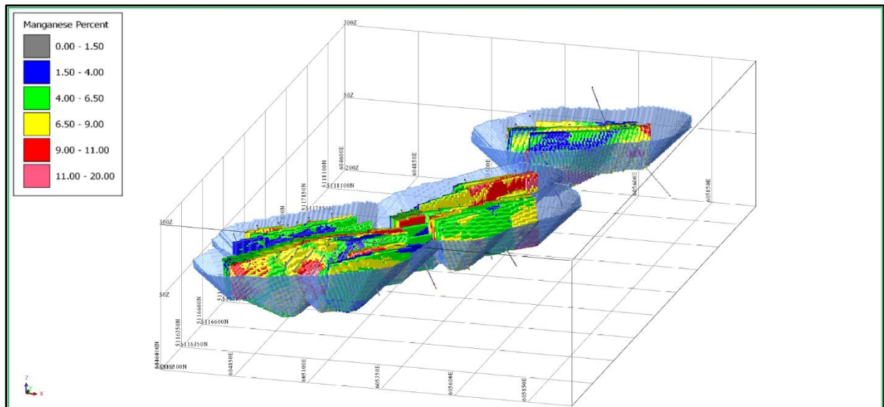
Figure 14-27: Oblique View Looking Northwest of the Optimized Pit Shell
