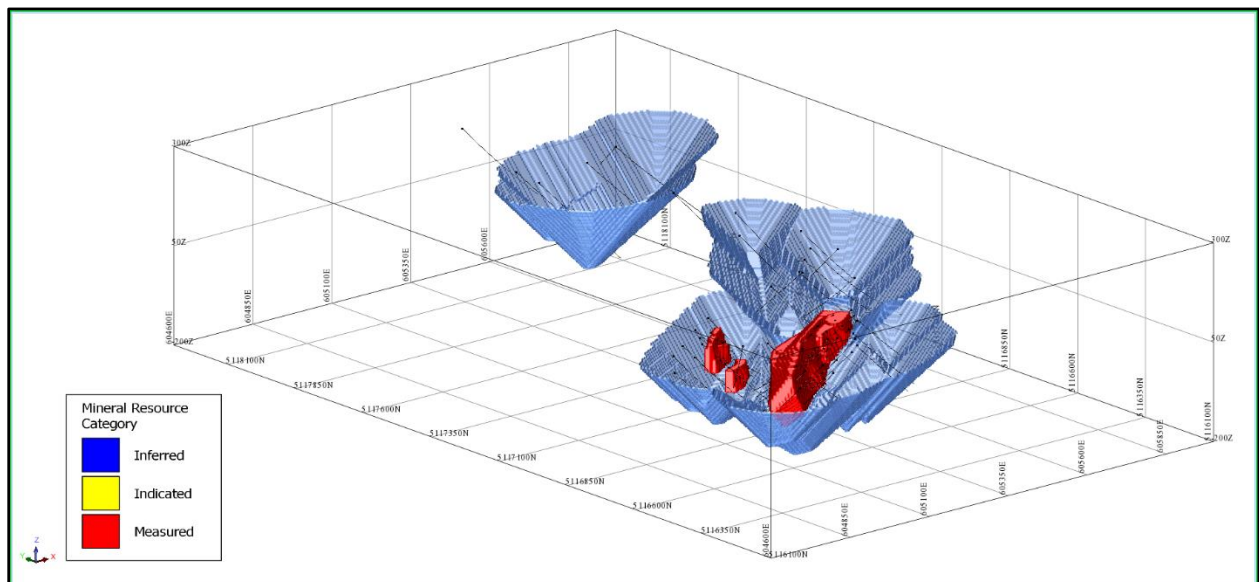
Figure 14-31: Oblique View Looking Northeast of the Measured Mineral Resource within the Optimized Pit Shell
