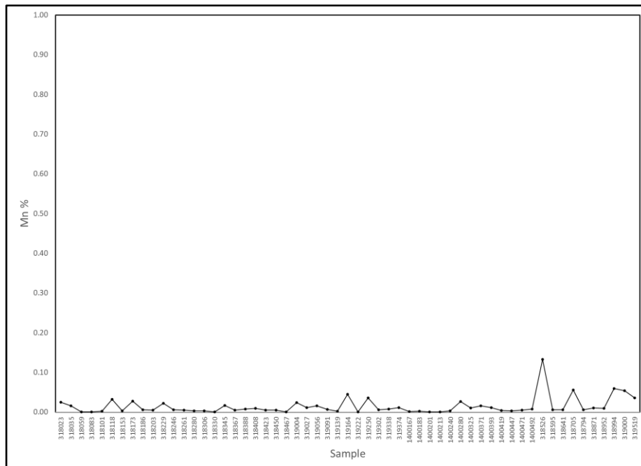
Figure 11-10: 2016 and 2017 Drilling Program Blank Results for Mn (N = 57)
