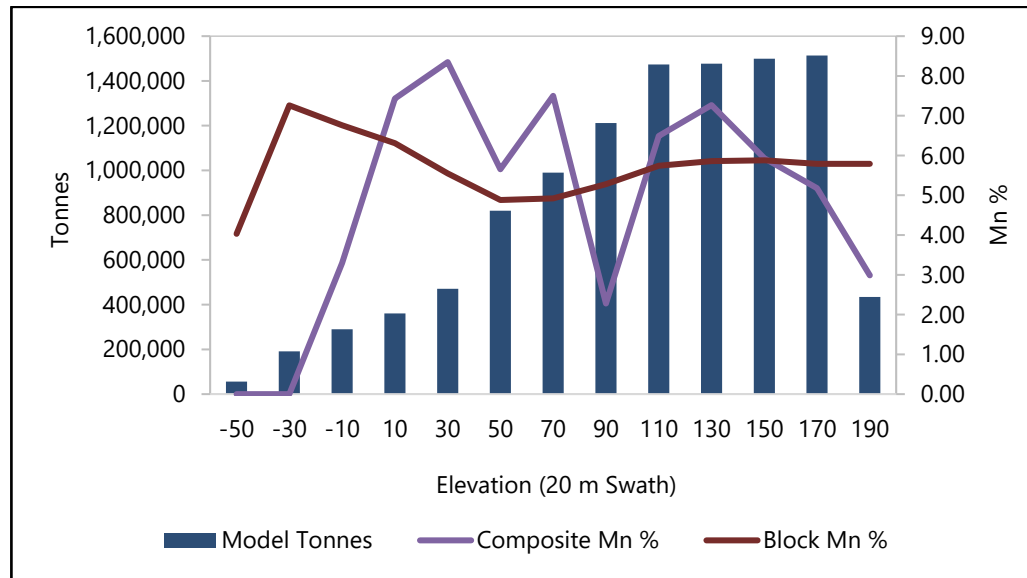
Figure 14-25: Iron Hill Area Elevation Swath Plot of Mineral Resource and 3.0 m Composite Mn % Grades
