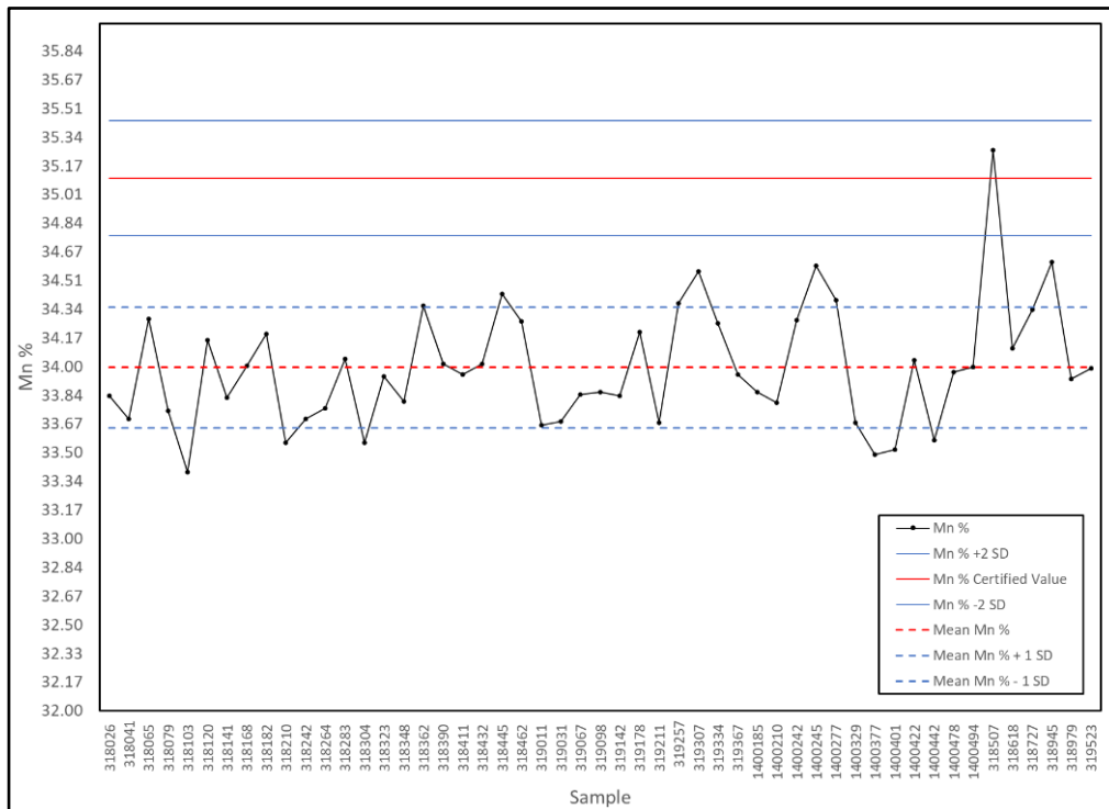
Figure 11-2: 2016 and 2017 Drilling Programs CRM OREAS 171 Results for Mn (N = 51)
