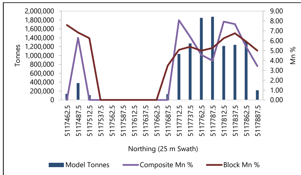
Figure 14-23: Iron Hill Area South-North Swath Plot of Mineral Resource and 3.0 m Composite Mn % Grades
