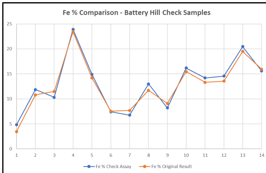
Figure 12-2: Fe% Witness Sample Results 2016, 2017, and 2020 Drilling Programs
