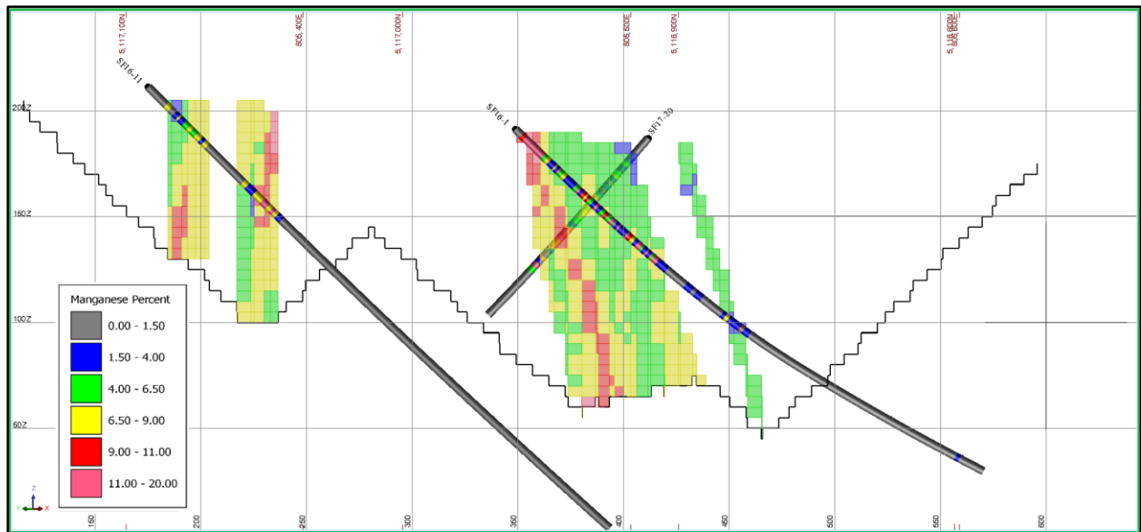
Figure 14-16: Representative Cross-Section looking Northeast of the Sharpe Farm Area Comparing OK Blocks and Assay Manganese Values (Optimized Pit Shell in Black)
