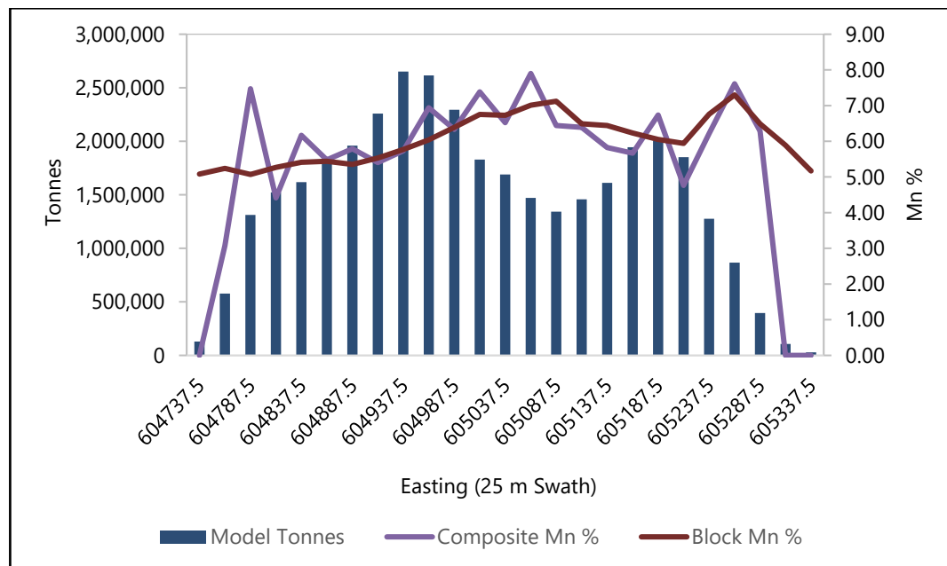
Figure 14-18: Moody Hill Area West-East Swath Plot of Mineral Resource and 3.0 m Composite Mn % Grades
