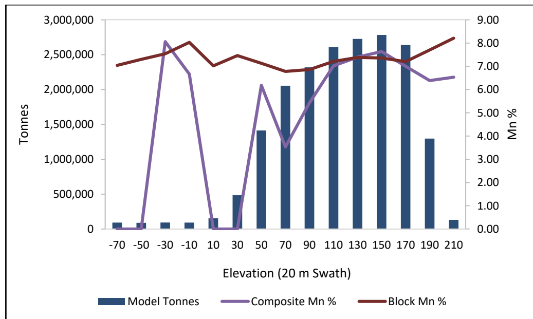
Figure 14-22: Sharpe Farm Area Elevation Swath Plot of Mineral Resource and 3.0 m Composite Mn % Grades
