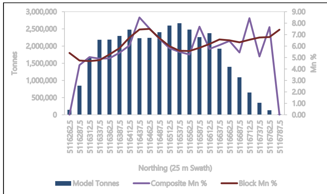
Figure 14-17: Moody Hill Area South-North Swath Plot of Mineral Resource and 3 m Composite Mn % Grades
