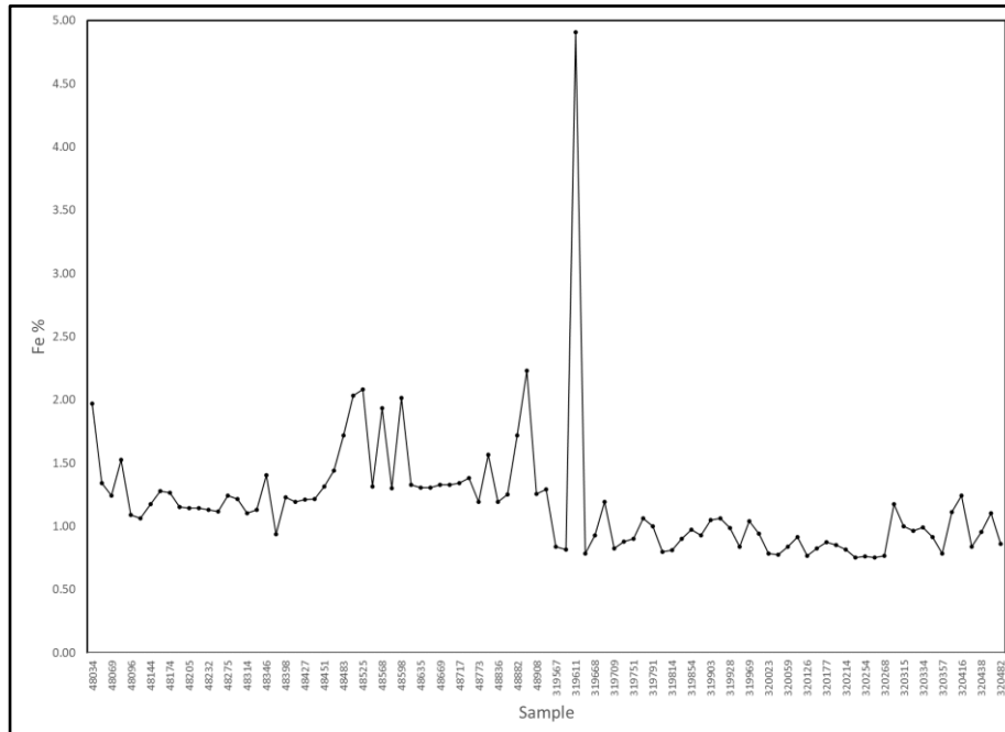
Figure 11-11: 2020 Drilling Program Blank Results for Fe (N = 95)
