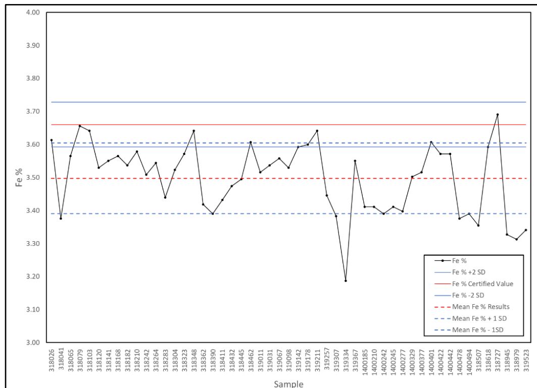
Figure 11-1: 2016 and 2017 Drilling Programs CRM OREAS 171 Results for Fe (N = 51)
