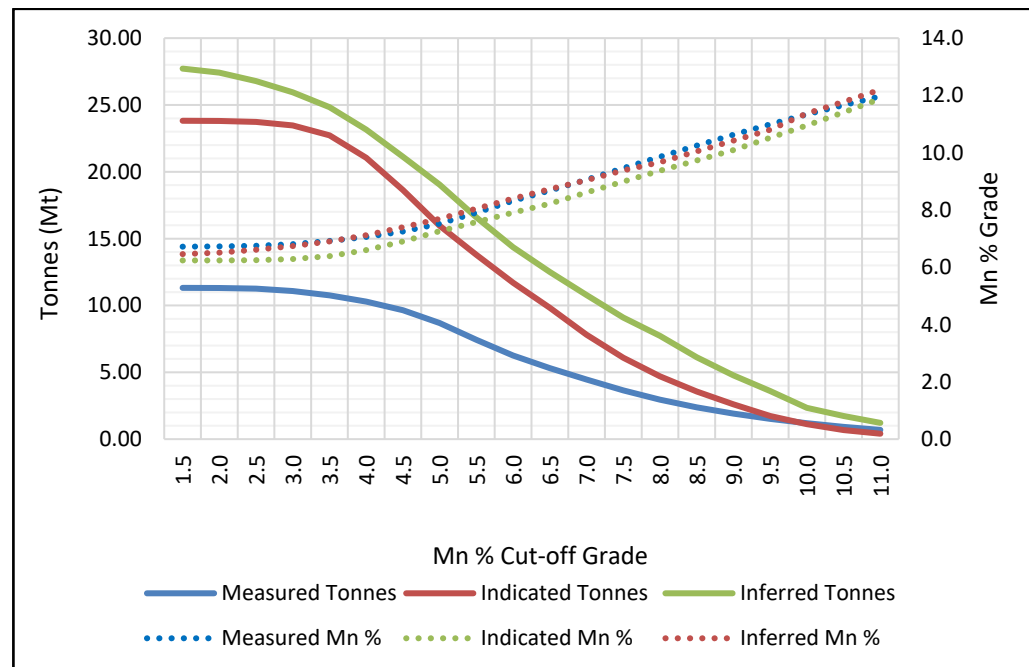
Figure 14-32: Tonnage/Grade Relationship Within Mineral Resources
