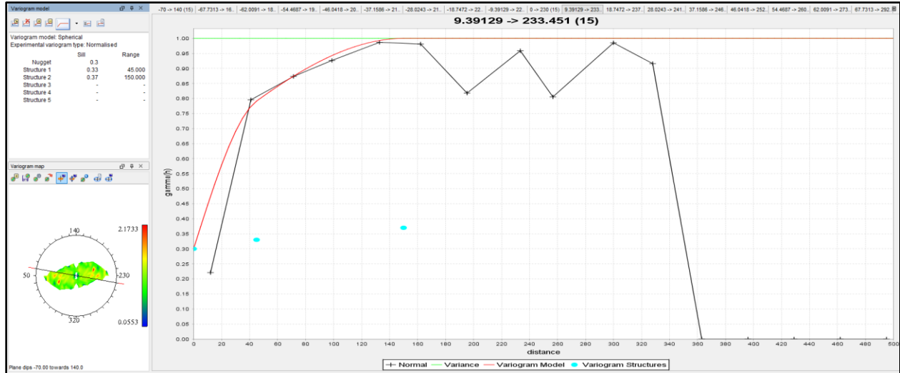
Figure 14-8: Manganese Variogram Model for the Major Axis of Continuity
