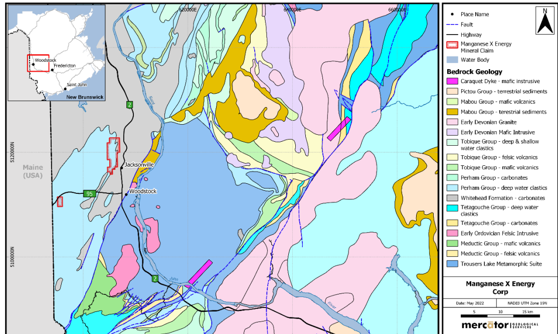
Figure 7-1: Regional Geological Map of Woodstock Area
