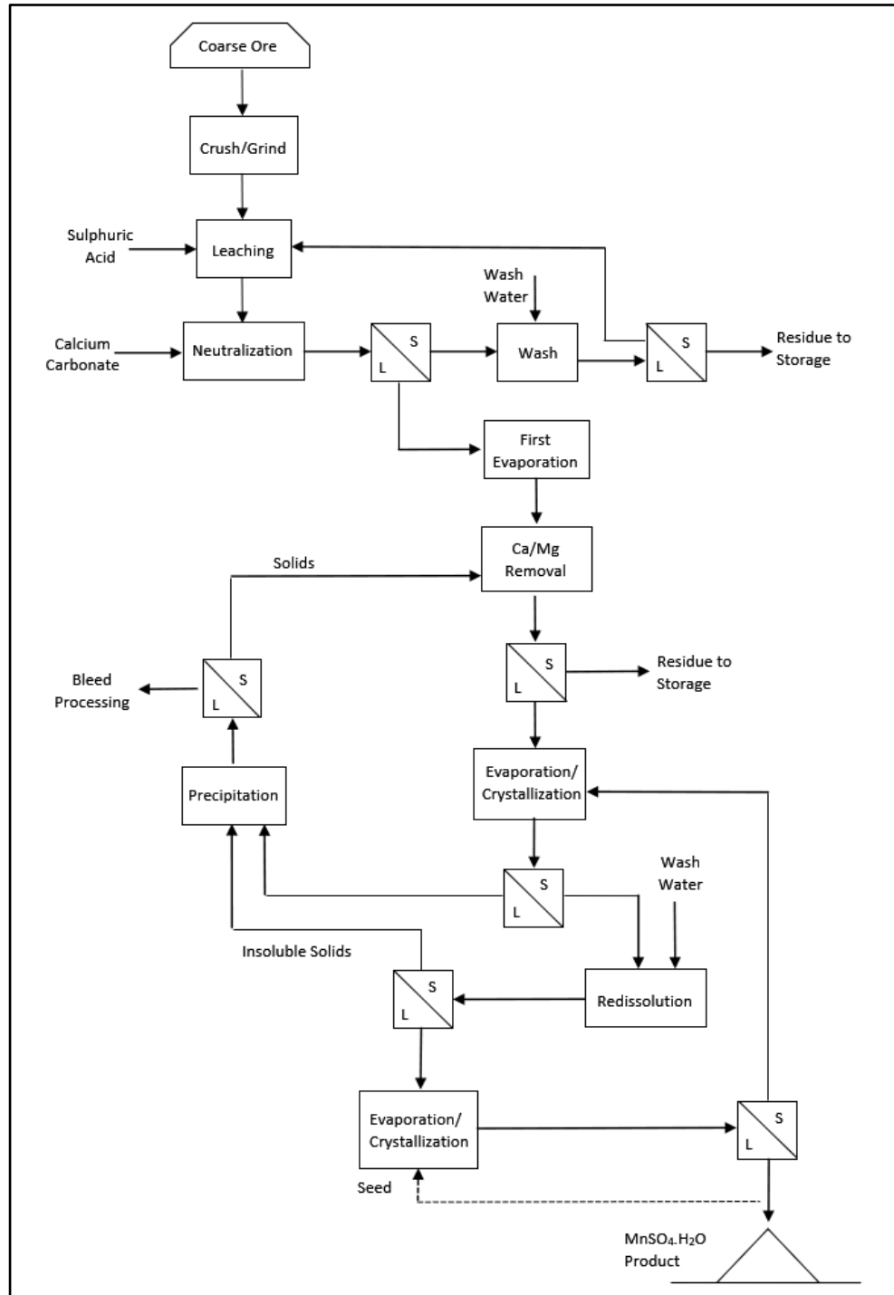
Figure 17-1: Process Block Flow Diagram
