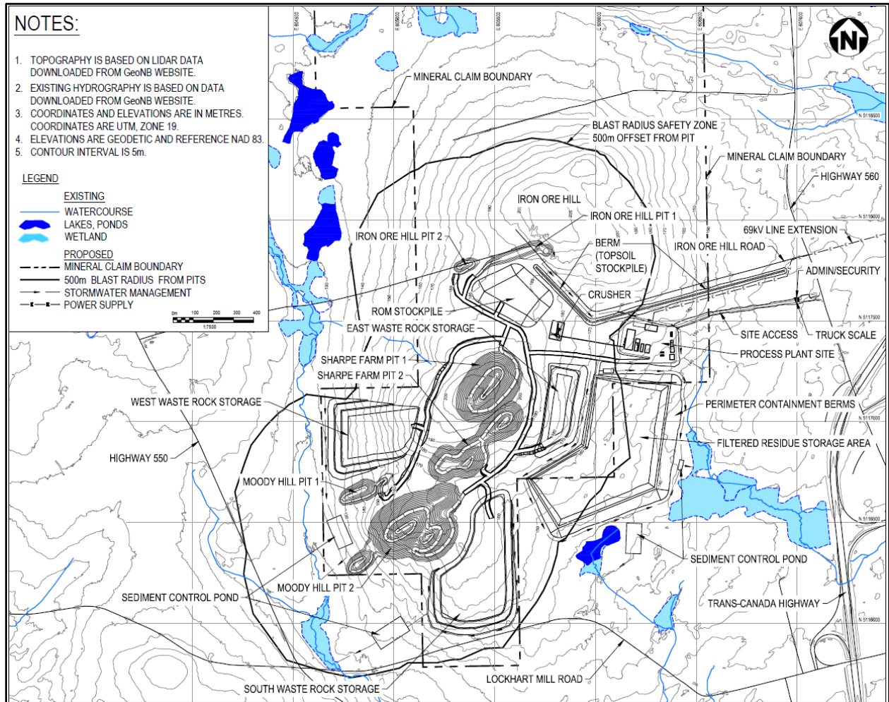
Figure 1-1: Site Plan Layout
