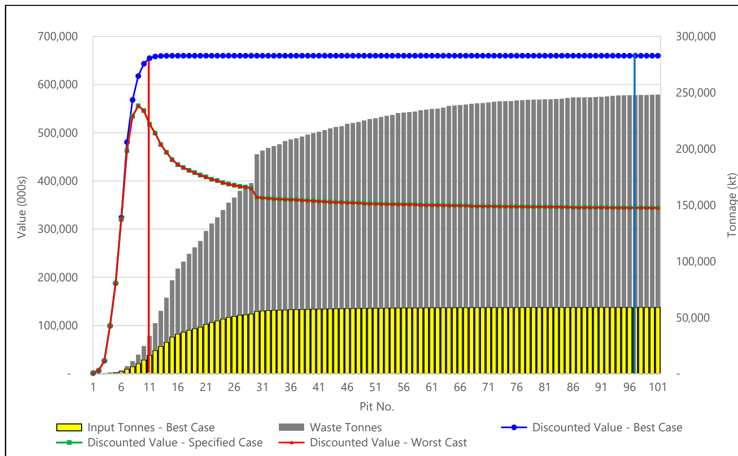
Figure 16-1: Pit Optimization Results, Pit-by-Pit Grade-Tonnage Graph
