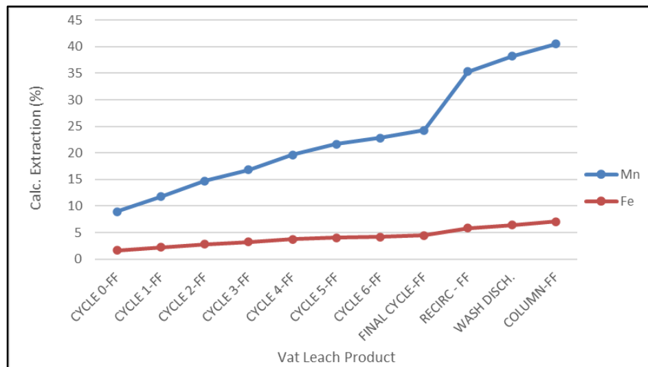
Figure 13-3: Vat Leach Test – Kinetic Extraction Curves for Manganese and Iron
