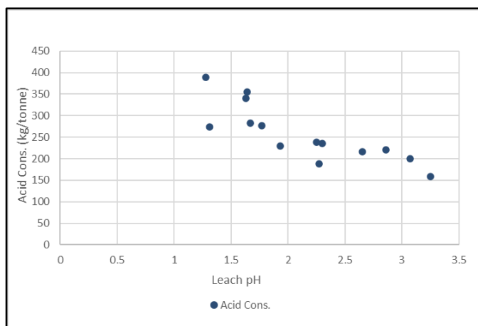
Figure 13-5: Acid Consumption vs. Leach pH on Moody Central Composite
