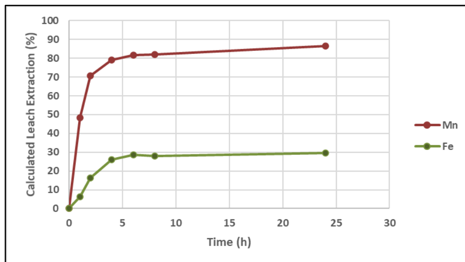
Figure 13-2: Bulk Leach Test – Kinetic Extraction Curves for Manganese and Iron
