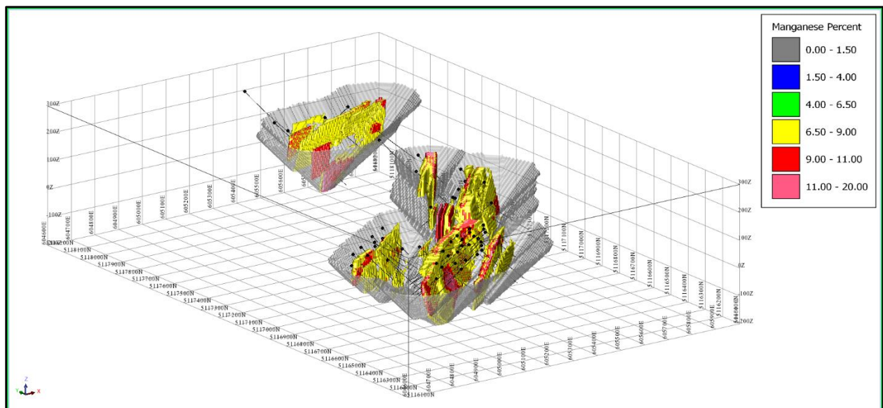
Figure 14-13: Oblique View Looking Northeast of Manganese Values Above a 6.5% Mn Cut-off within the Optimized Pit Shell (Grey)
