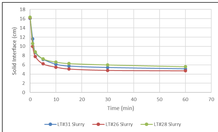
Figure 13-6: Best Settling Curves for Each Composite
