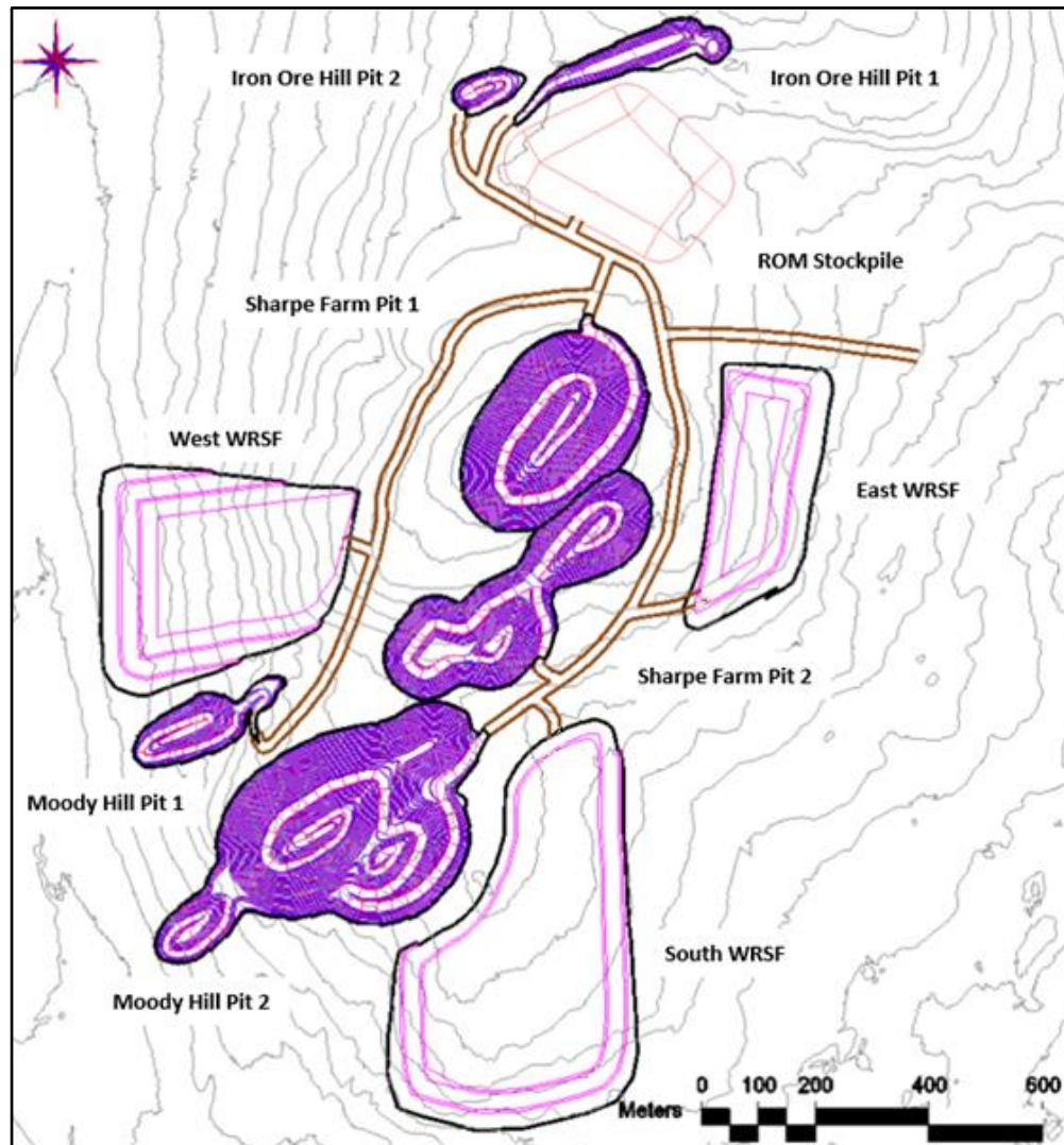
Figure 16-4: Conceptual Layout Plan – Pits, Waste Rock Storage Facilities, and ROM Stockpile
