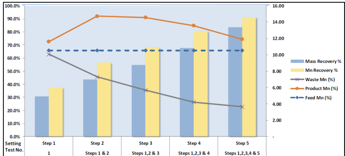
Figure 13-1: Ore Sorting Preliminary Scoping – Step 1 to 5 Manganese Grade Recovery
