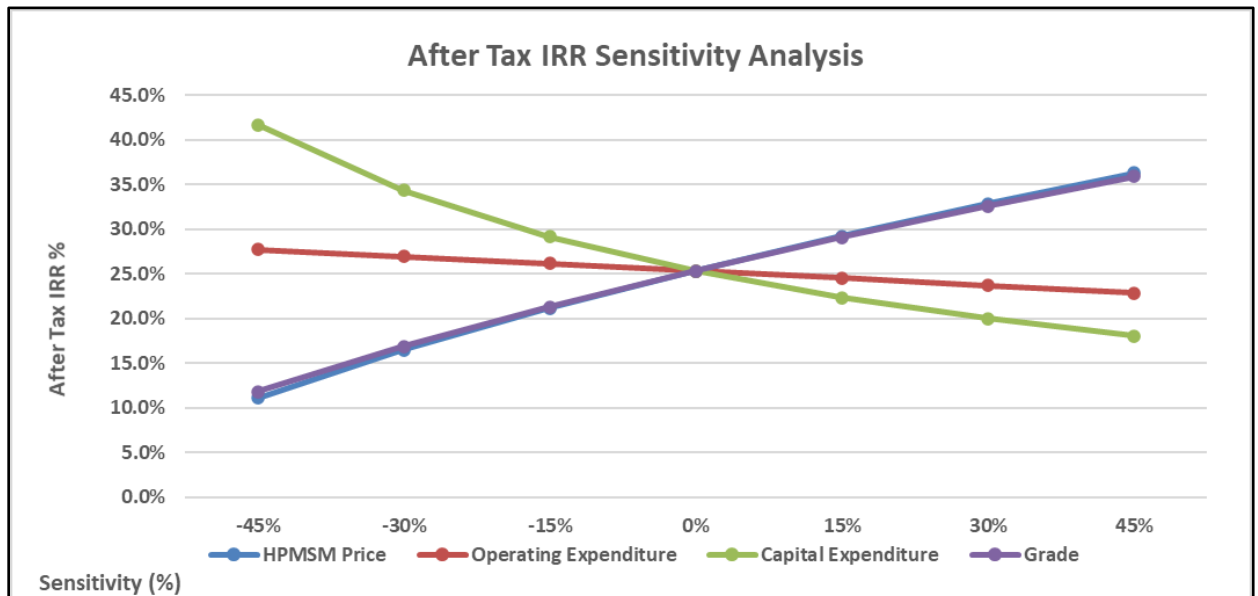
Figure 22-6: After-Tax IRR Sensitivity
