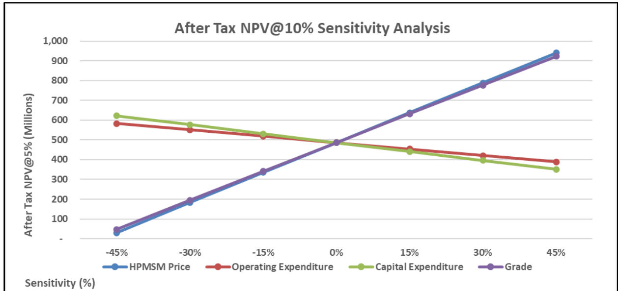
Figure 22-5: After-Tax NPV 10 Sensitivity
