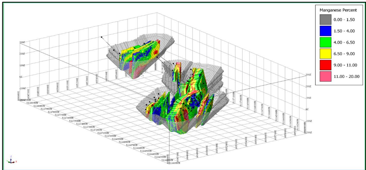
Figure 14-12: Oblique View Looking Northeast of Manganese Values Above a 1.5% Mn Cut-off within the Optimized Pit Shell (Grey)
