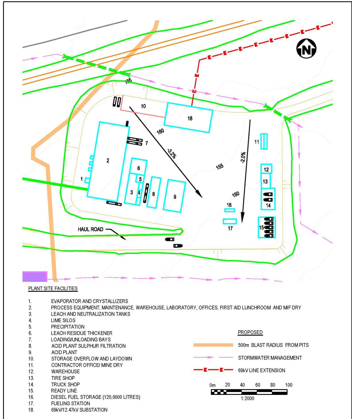
Figure 18-2: Process Plant Site Layout
