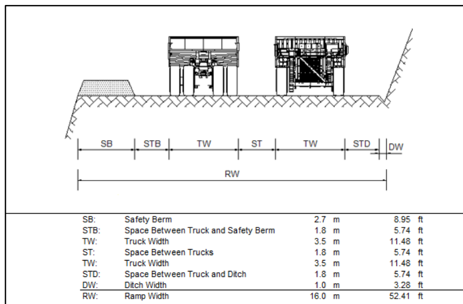
Figure 16-3: Typical Ramp Cross-Section
