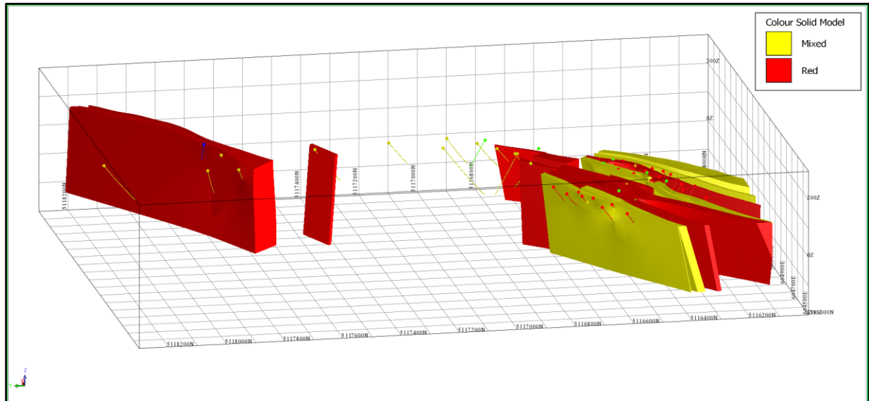
Figure 14-6: Isometric View (East) of the Red and Mixed Colour Solid Models
