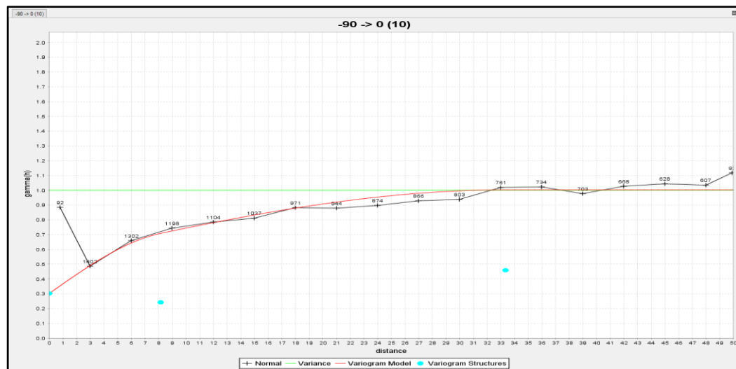
Figure 14-7: Downhole Manganese Variogram
