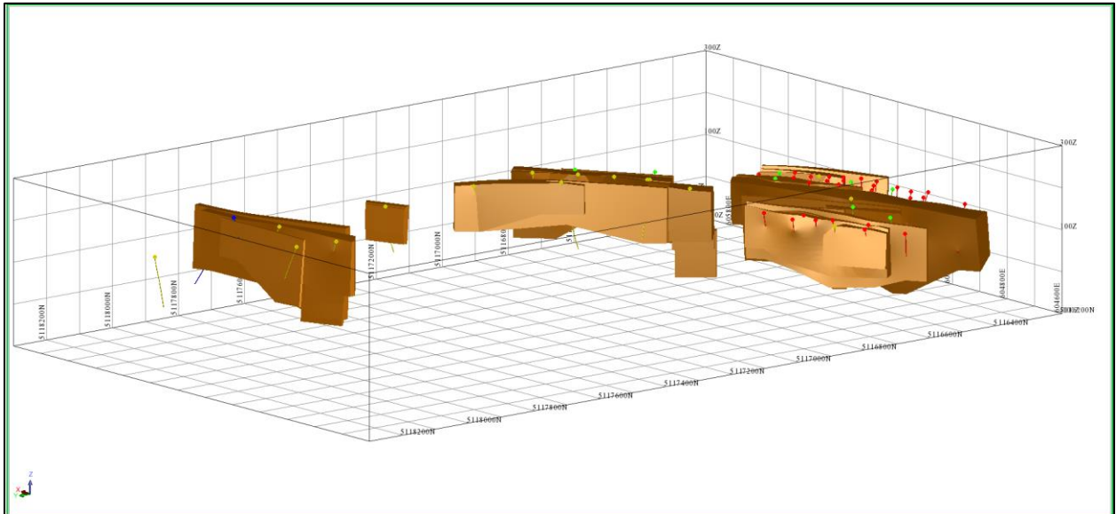
Figure 14-3: Isometric View (Southeast) of the Grade Domain Solid Models
