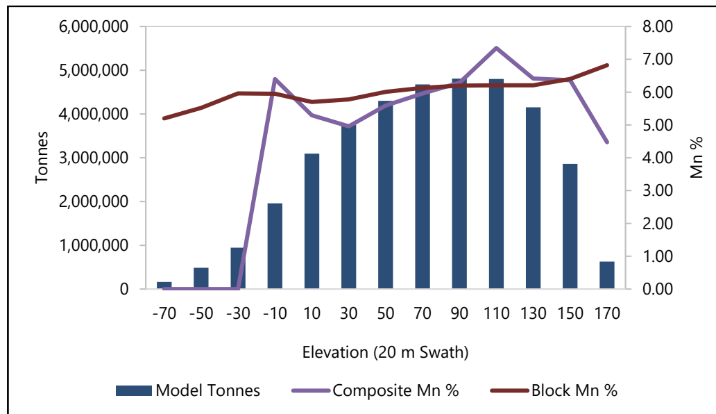
Figure 14-19: Moody Hill Area Elevation Swath Plot of Mineral Resource and 3.0 m Composite Mn % Grades
