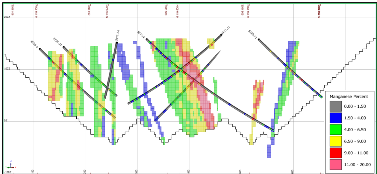
Figure 14-15: Representative Cross-Section Looking Northeast of the Moody Hill Area Comparing OK Blocks and Assay Manganese Values (Optimized Pit Shell in Black)
