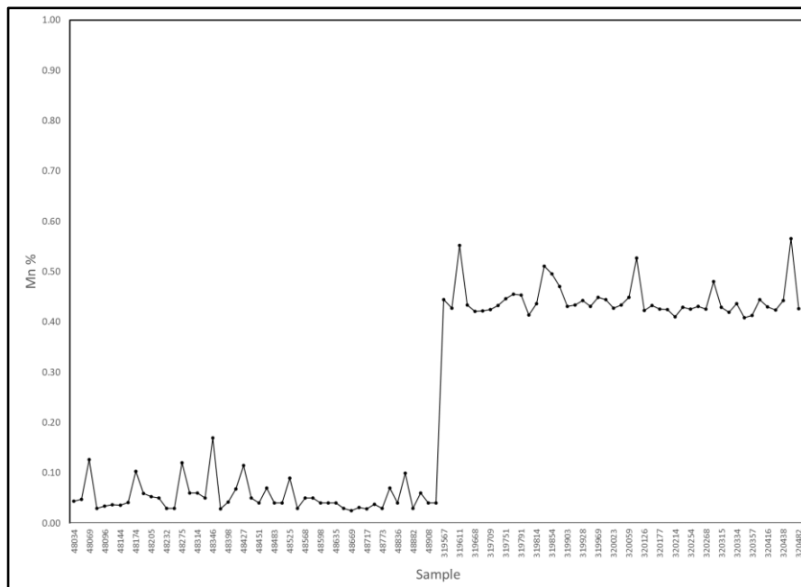
Figure 11-12: 2020 Drilling Program Blank Results for Mn (N = 95)
