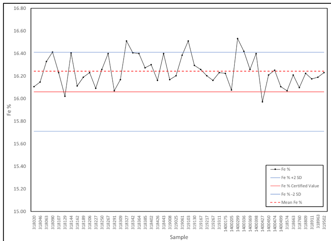
Figure 11-3: 2016 and 2017 Drilling Programs CRM OREAS 700 Results for Fe (N = 48)
