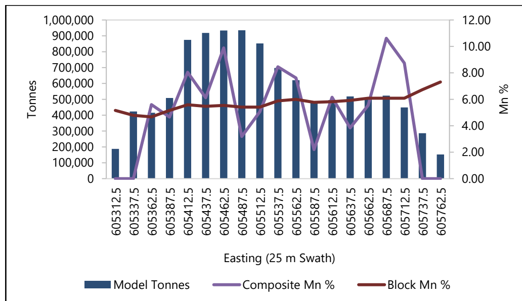
Figure 14-24: Iron Hill Area West-East Swath Plot of Mineral Resource and 3.0 m Composite Mn % Grades
