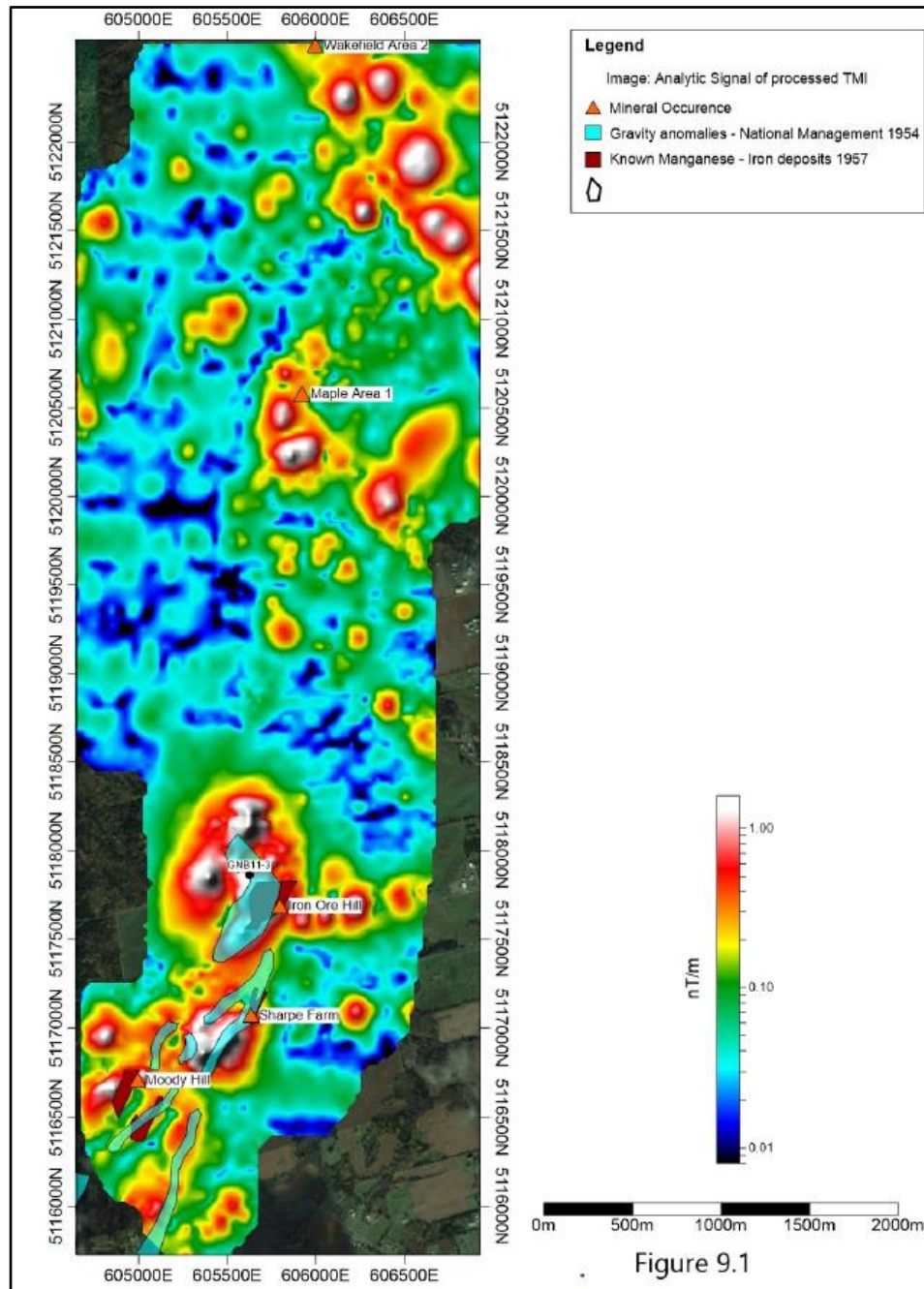
Figure 9-1: 2016 Ground Magnetometer Survey Results
