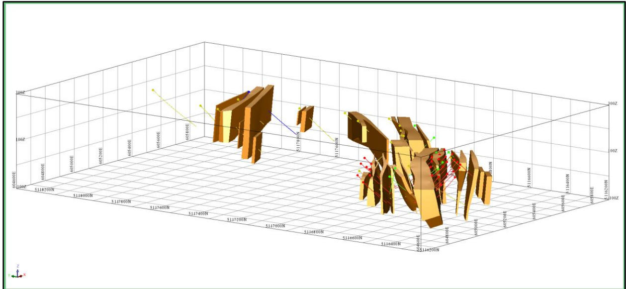
Figure 14-5: Isometric View (Northeast) of the Grade Domain Solid Models
