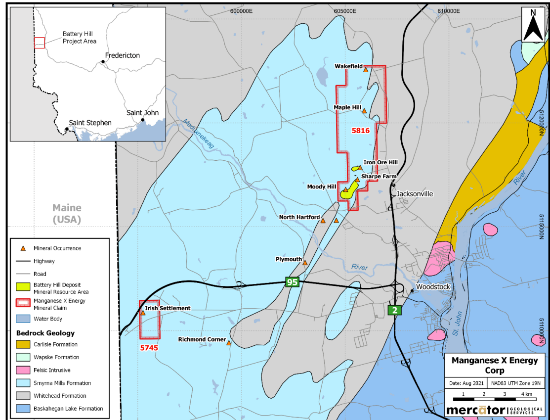
Figure 7-2: Geology of the Battery Hill Manganese Property
