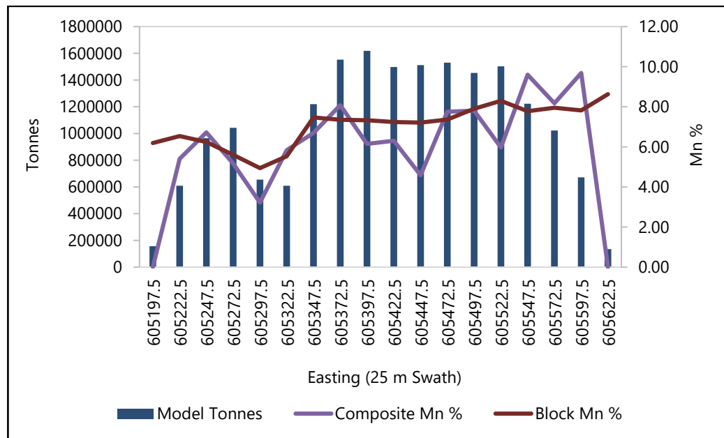
Figure 14-21: Sharpe Farm Area West-East Swath Plot of Mineral Resource and 3.0 m Composite Mn % Grades
