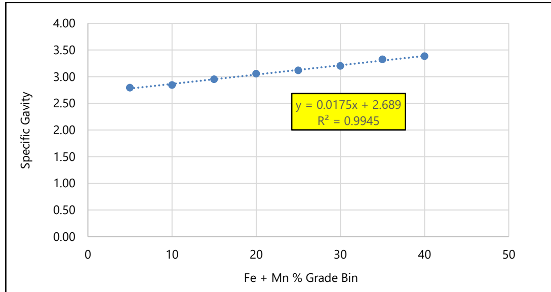
Figure 14-11: Regression Curve between Specific Gravity and Manganese Plus Iron Grade
