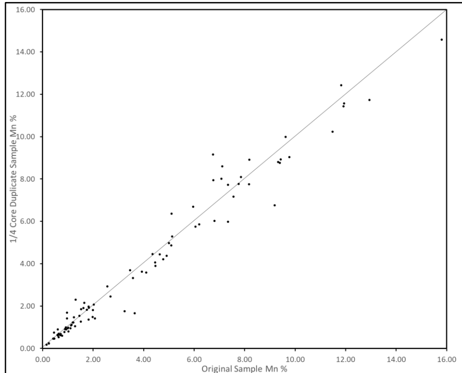
Figure 11-16: 2020 Duplicate ¼ Core Sample Results for Mn (N = 93)
