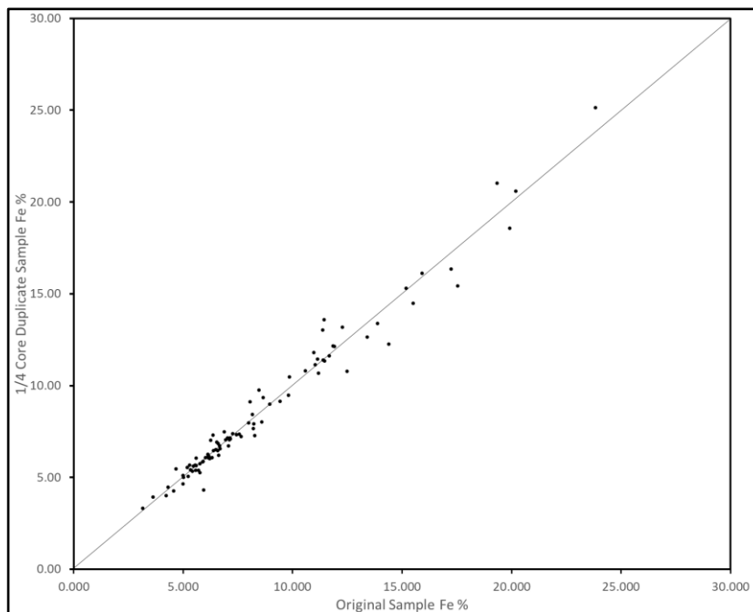
Figure 11-15: 2020 Duplicate ¼ Core Sample Results for Fe (N = 93)
