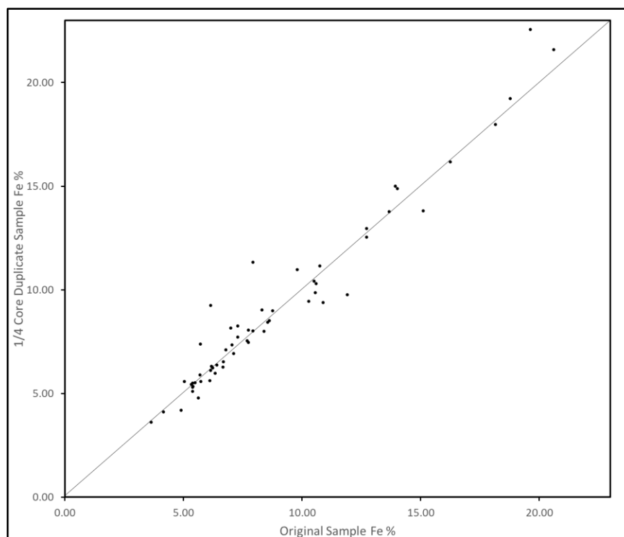
Figure 11-13: 2016 and 2017 Duplicate 1/4 Core Sample Results for Fe (N = 58)
