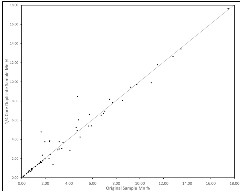
Figure 11-14: 2016 and 2017 Duplicate ¼ Core Sample Results for Mn (N = 58)
