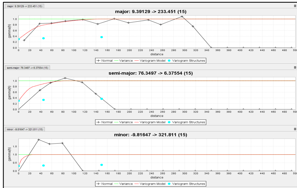
Figure 14-10: Manganese Variogram Model
