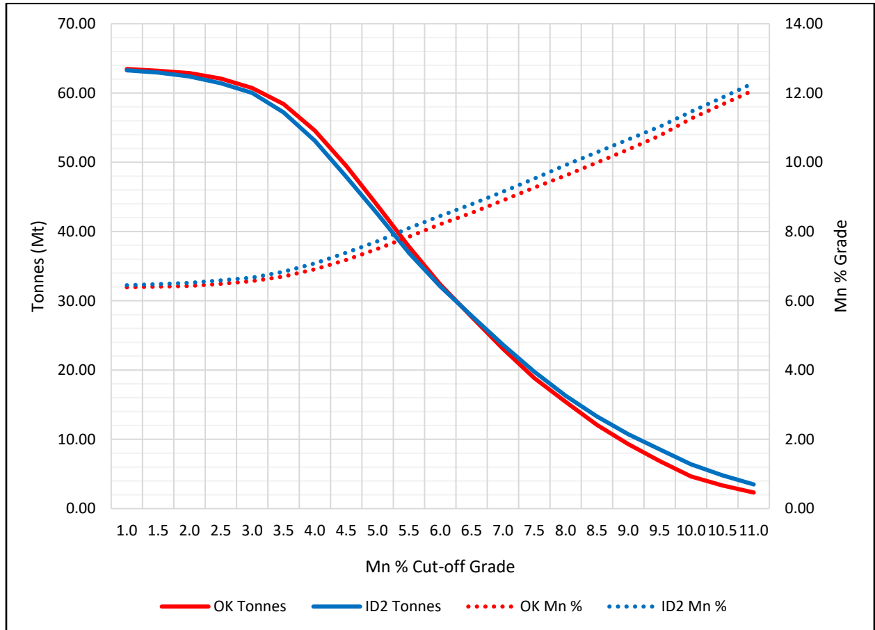
Figure 14-26: Grade and Tonnage Relationship of OK and ID2 Interpolation Methodologies
