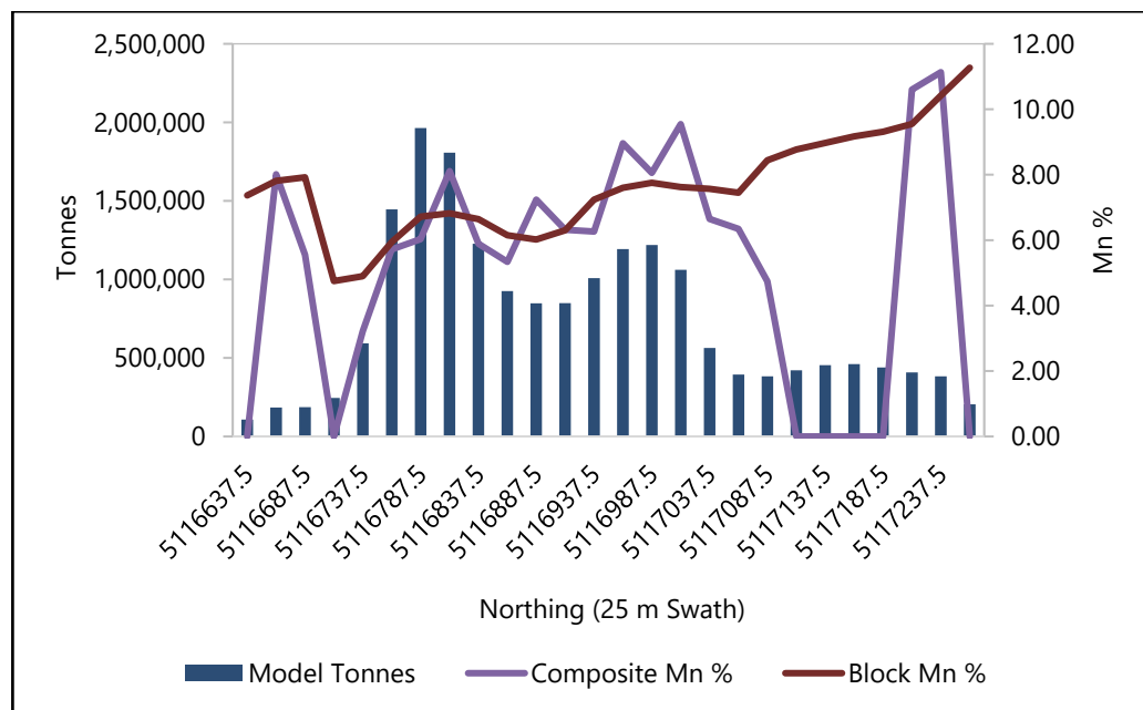
Figure 14-20: Sharpe Farm Area South-North Swath Plot of Mineral Resource and 3.0 m Composite Mn % Grades
