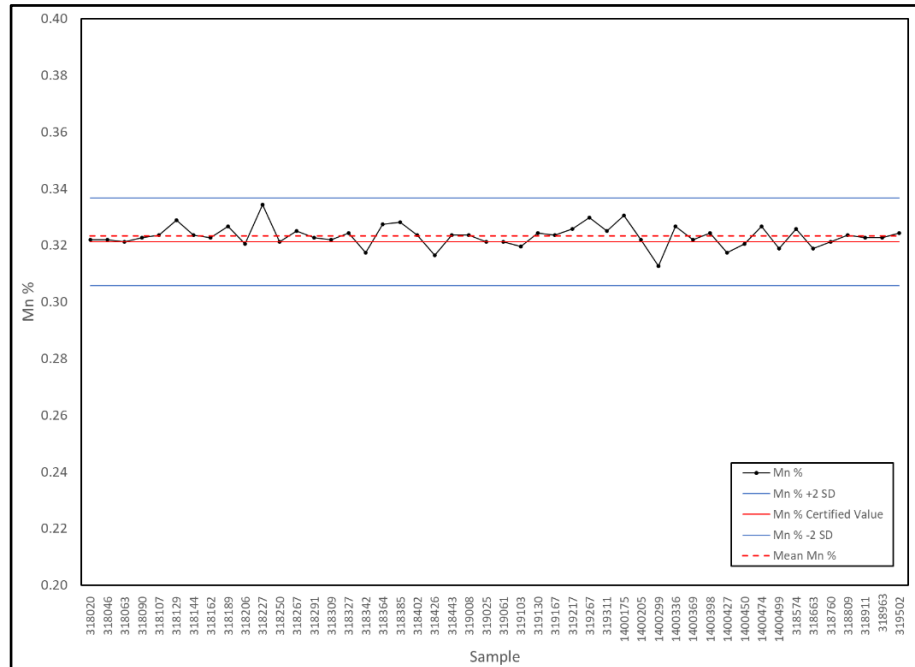
Figure 11-4: 2016 and 2017 Drilling Programs CRM OREAS 700 Results for Mn (N = 48)
