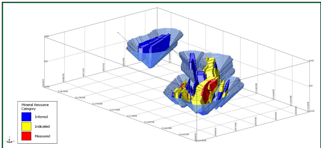
Figure 14-29: Oblique View Looking Northeast of the Mineral Resource Categorization within the Optimized Pit Shell (Blue)
