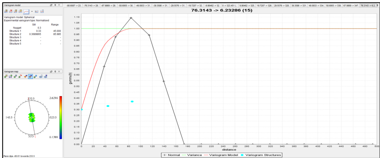
Figure 14-9: Manganese Variogram Model for the Semi-Major Axis of Continuity
