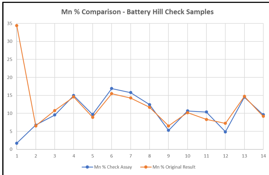
Figure 12-1: Mn% Witness Sample Results 2016, 2017, and 2020 Drilling Programs
