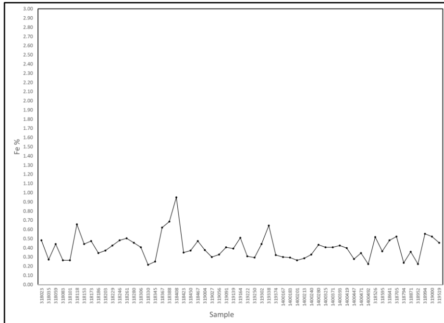
Figure 11-9: 2016 and 2017 Drilling Program Blank Results for Fe (N = 57)
