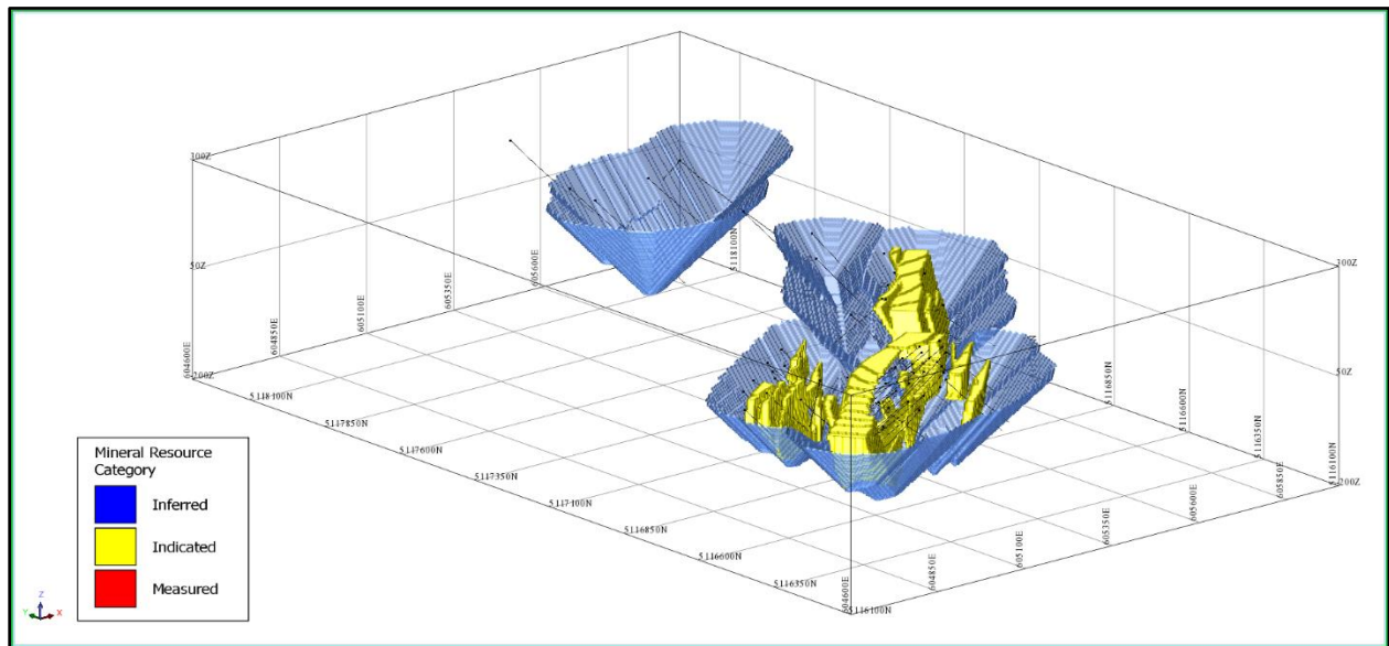
Figure 14-30: Oblique View Looking Northeast of the Indicated Mineral Resource within the Optimized Pit Shell (Blue)
