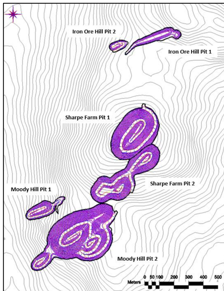
Figure 16-2: Ultimate Pits Moody Hill, Sharpe Farm, and Iron Ore Hill Zones
