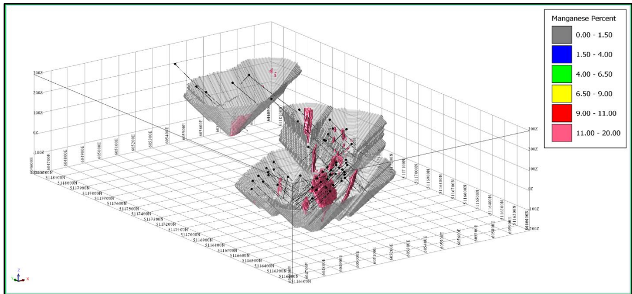
Figure 14-14: Oblique View Looking Northeast of Manganese Values Above a 11% Mn Cut-off within the Optimized Pit Shell (Grey)
