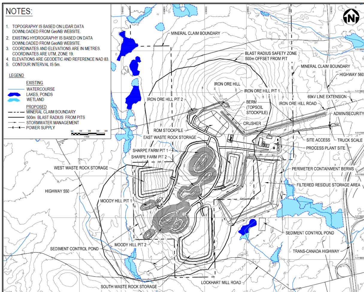
Figure 18-1: Project Site Layout
