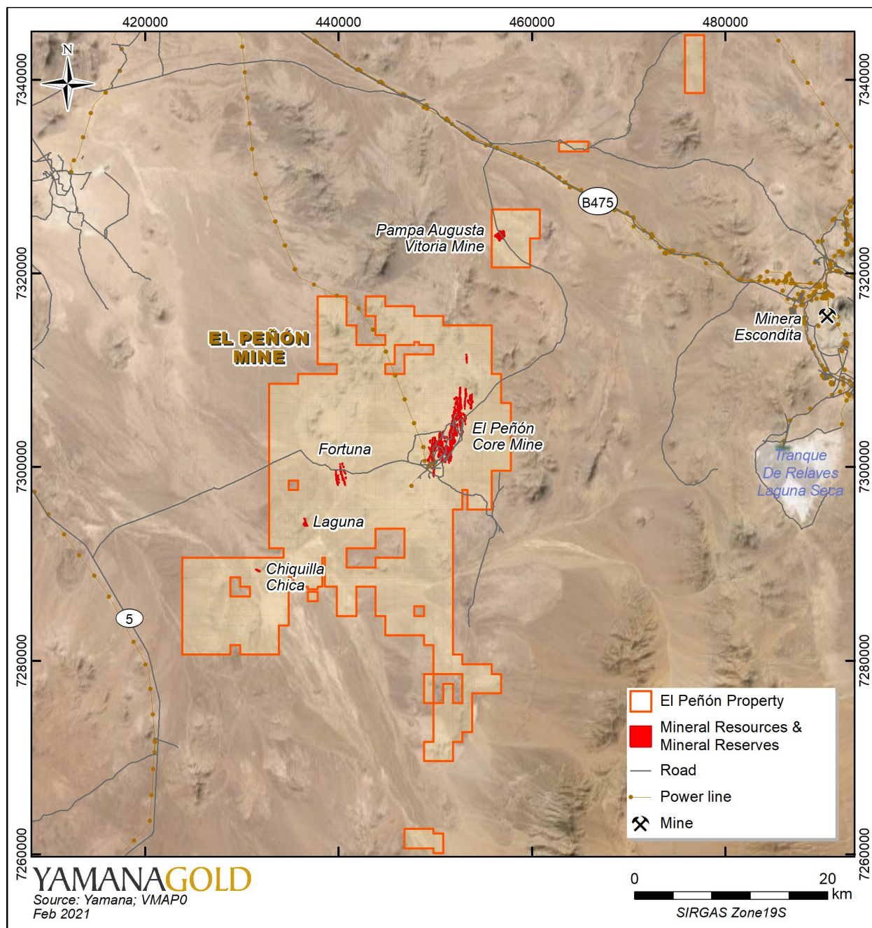
Figure 4-2: Map of mineral tenure
